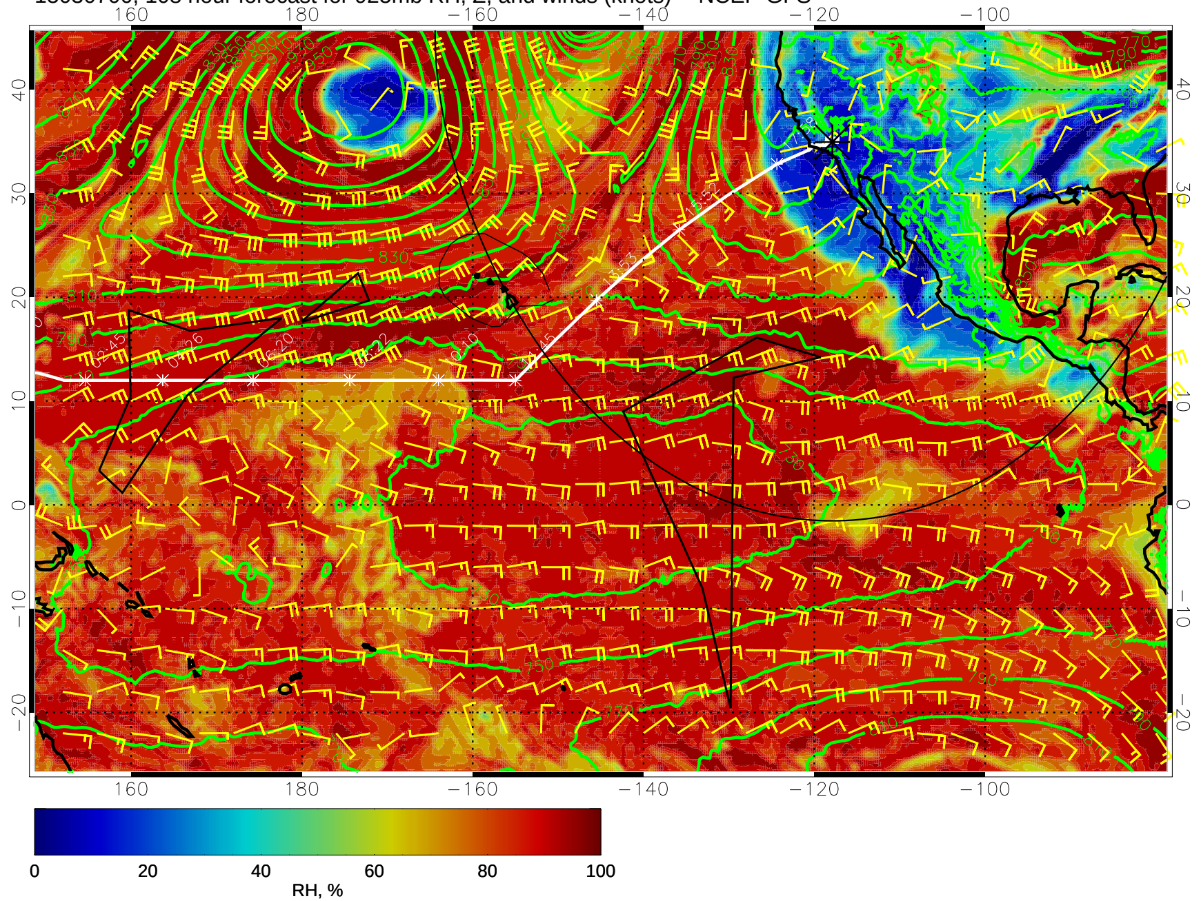
15030700, 108 hour forecast for 925mb RH, Z, and winds (knots) -- NCEP GFS
