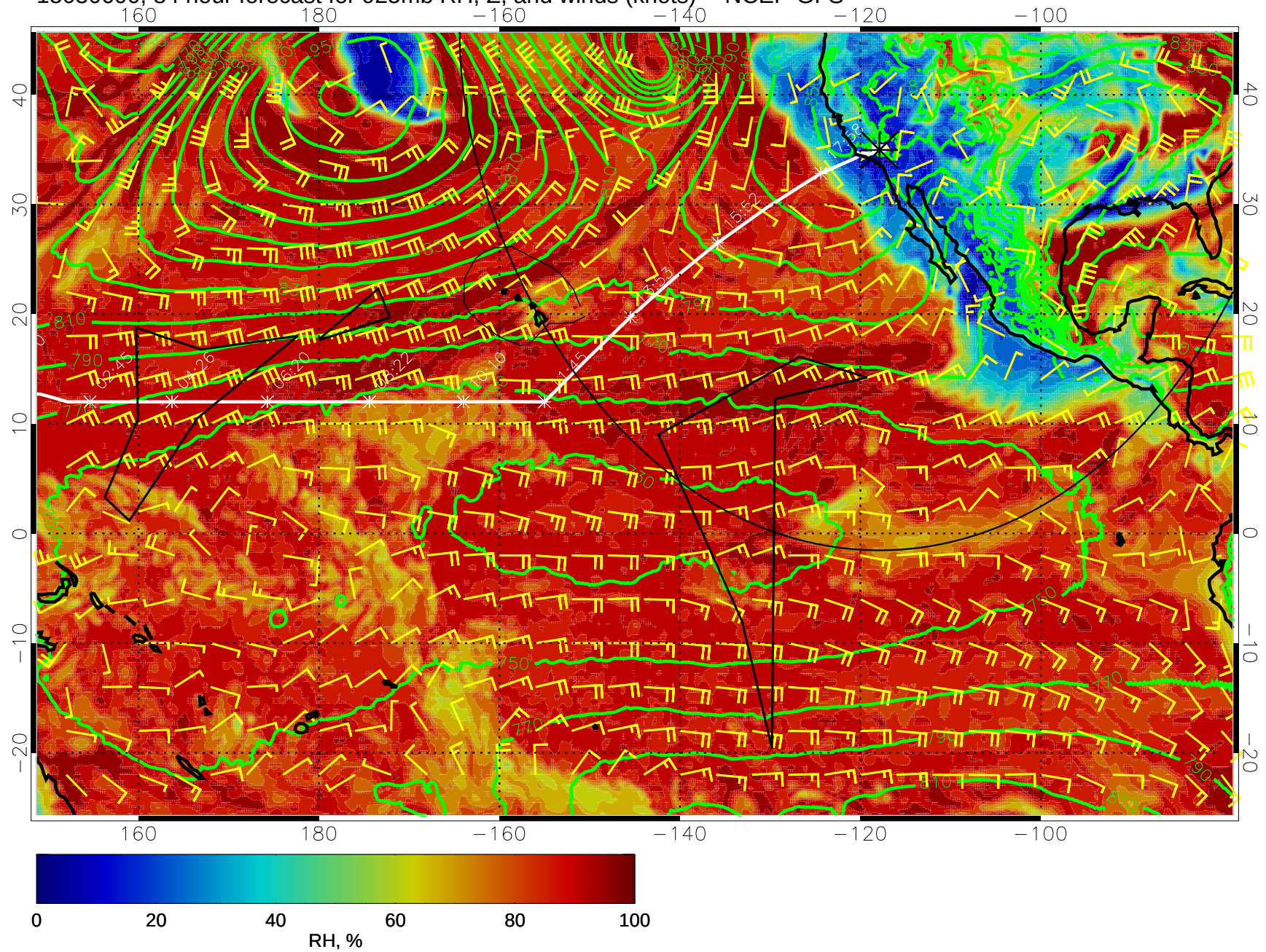
15030600, 84 hour forecast for 925mb RH, Z, and winds (knots) -- NCEP GFS
