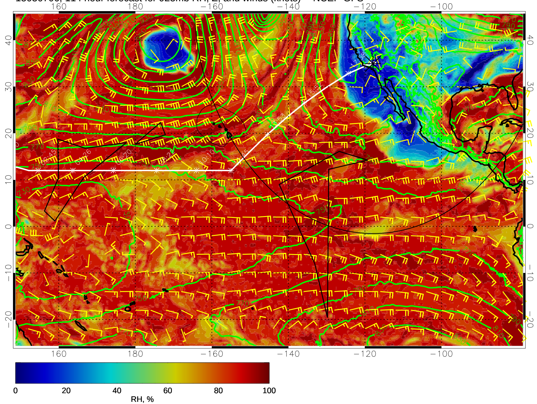
15030706, 114 hour forecast for 925mb RH, Z, and winds (knots) -- NCEP GFS
