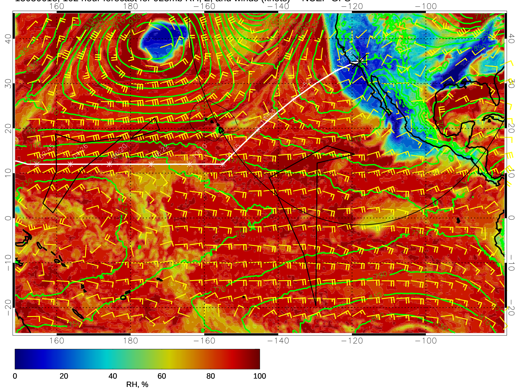
15030618, 102 hour forecast for 925mb RH, Z, and winds (knots) -- NCEP GFS
