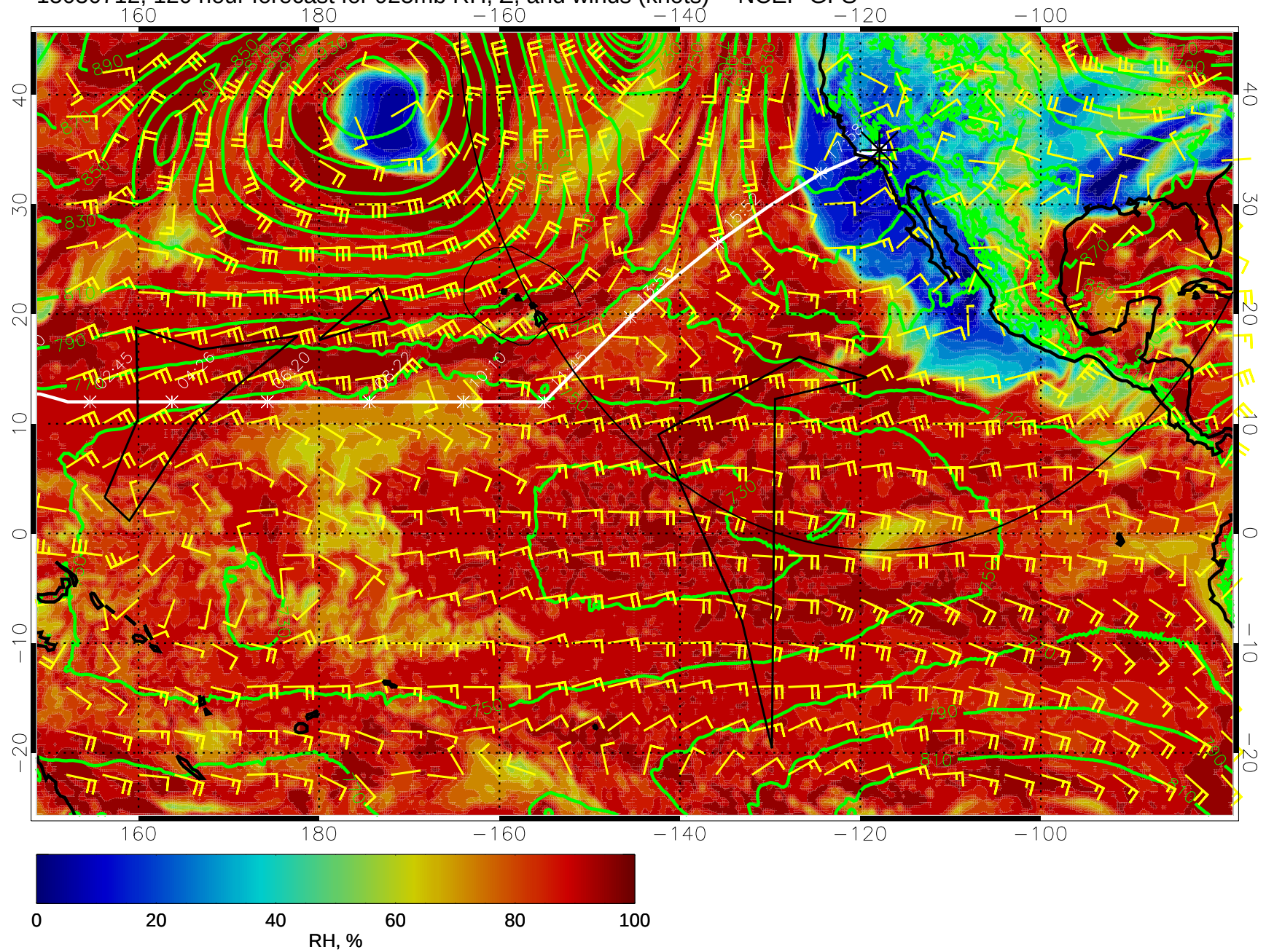
15030712, 120 hour forecast for 925mb RH, Z, and winds (knots) -- NCEP GFS
