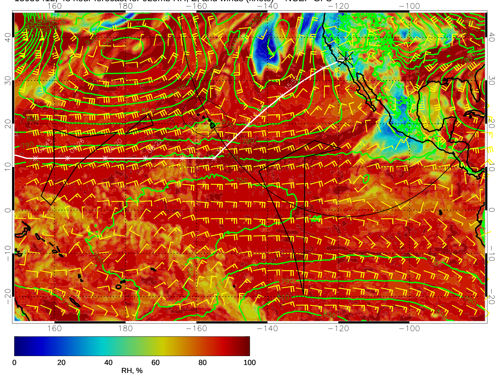
15030412, 48 hour forecast for 925mb RH, Z, and winds (knots) -- NCEP GFS
