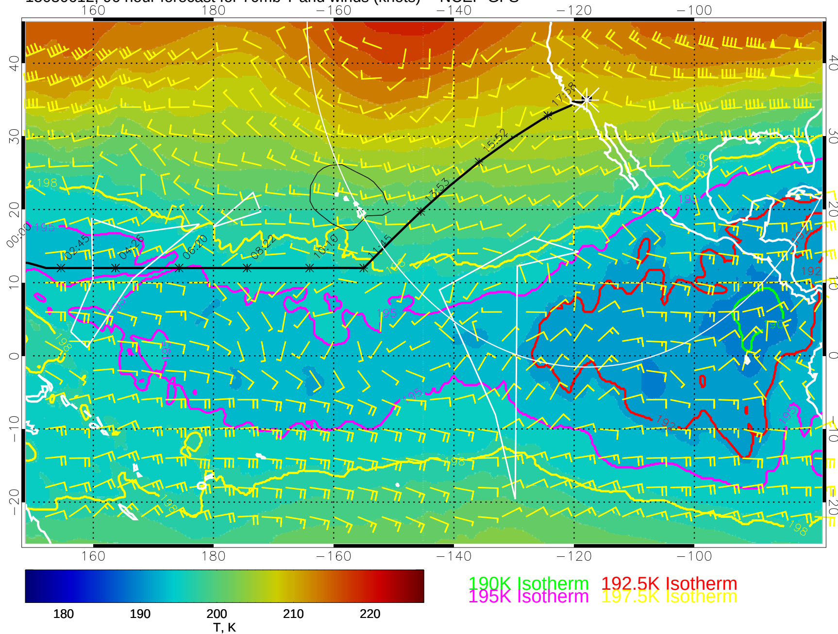
15030612, 96 hour forecast for 70mb T and winds (knots) -- NCEP GFS
