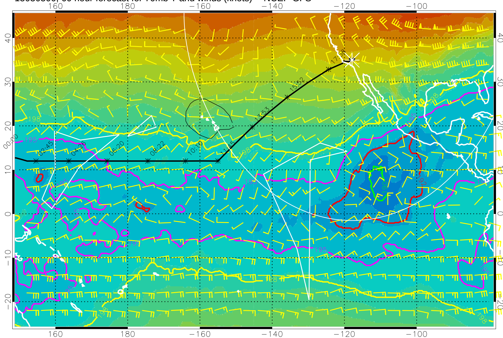
15030500, 60 hour forecast for 70mb T and winds (knots) -- NCEP GFS
