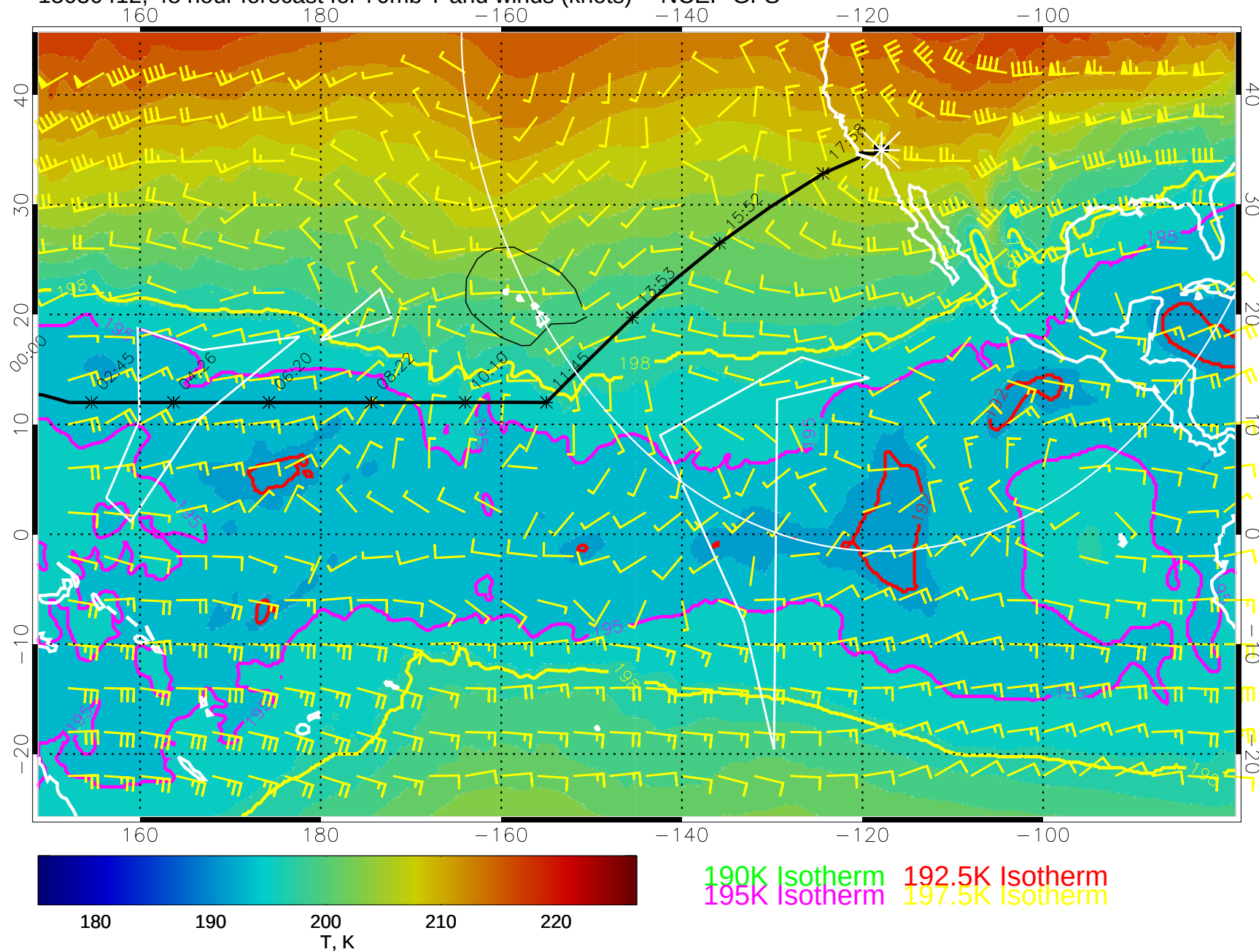
15030412, 48 hour forecast for 70mb T and winds (knots) -- NCEP GFS
