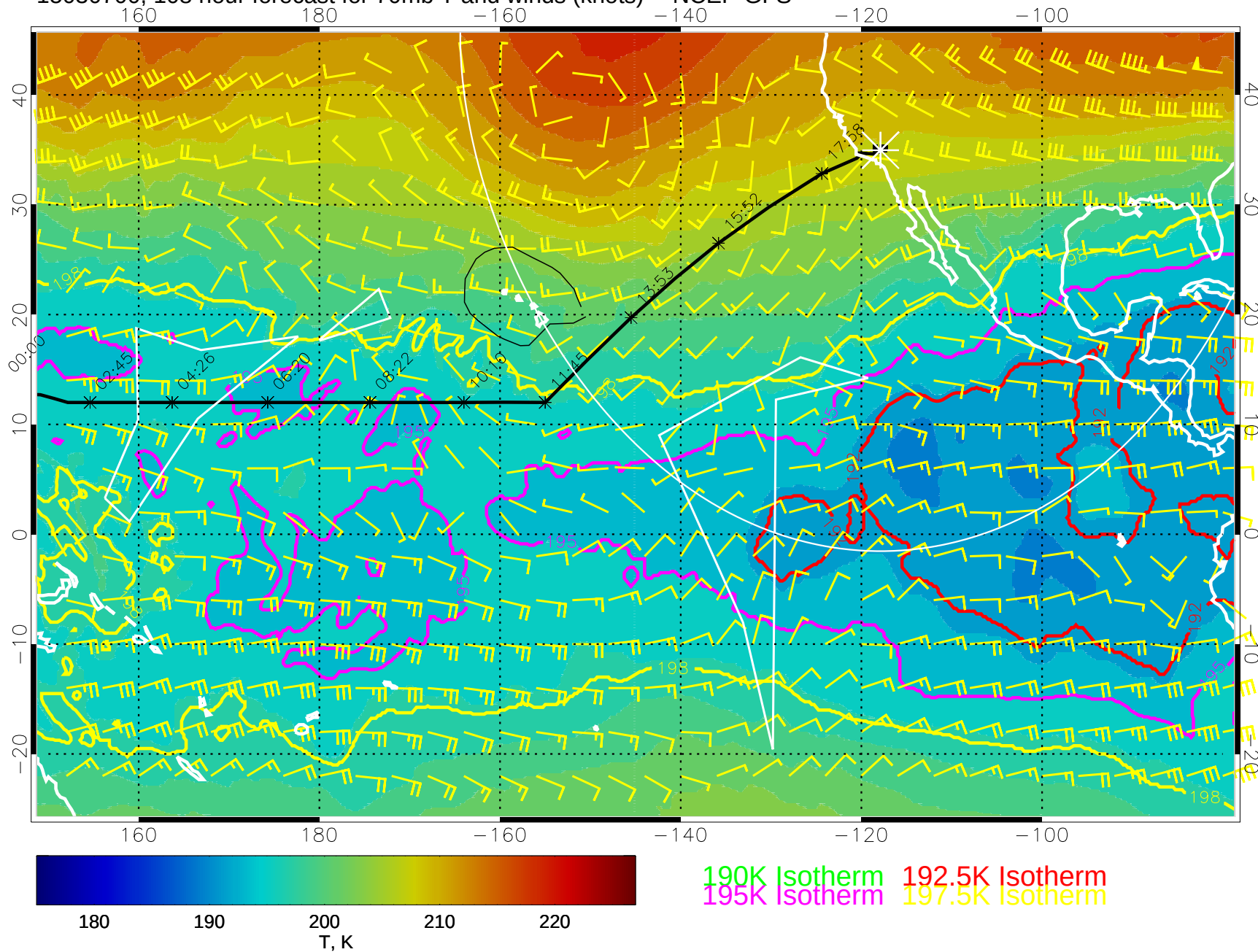
15030700, 108 hour forecast for 70mb T and winds (knots) -- NCEP GFS
