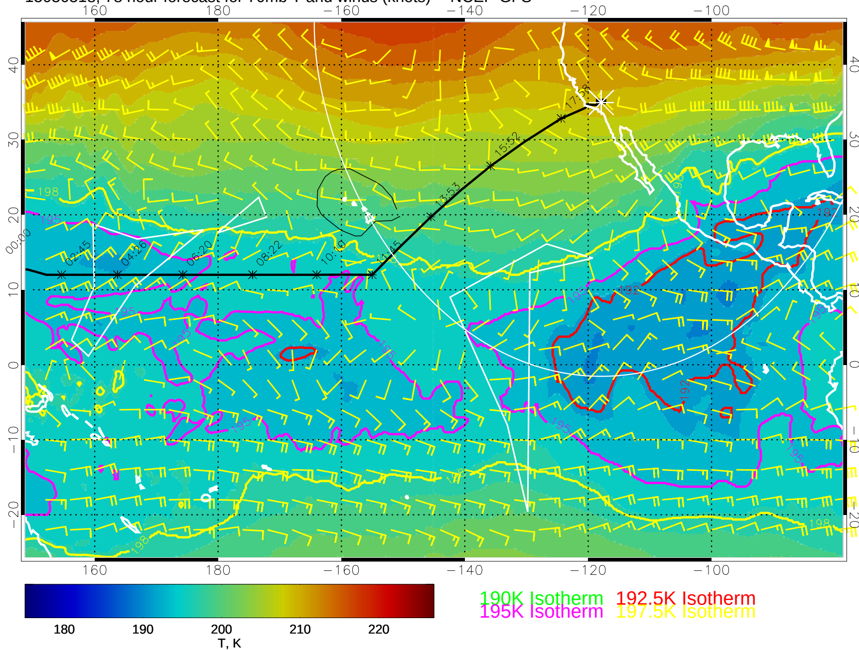
15030518, 78 hour forecast for 70mb T and winds (knots) -- NCEP GFS
