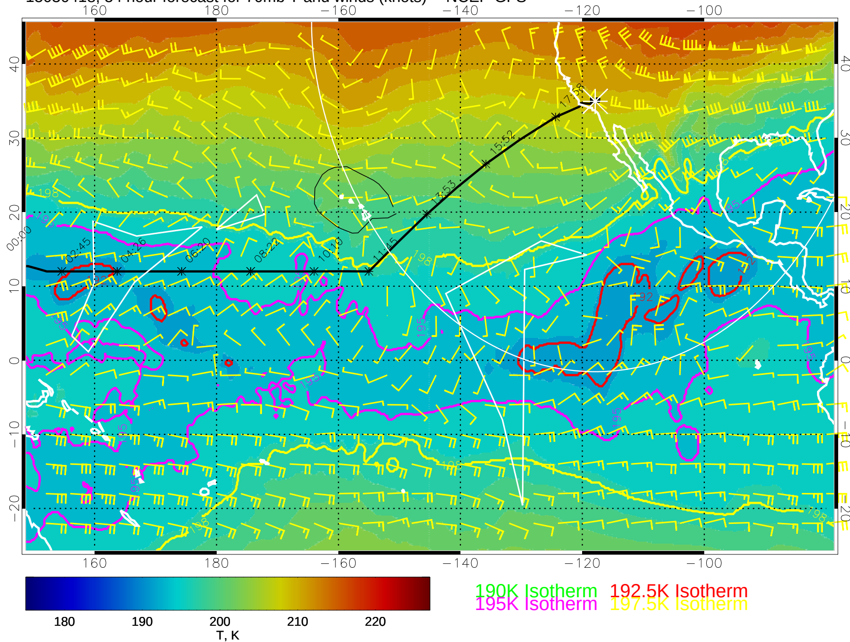
15030418, 54 hour forecast for 70mb T and winds (knots) -- NCEP GFS
