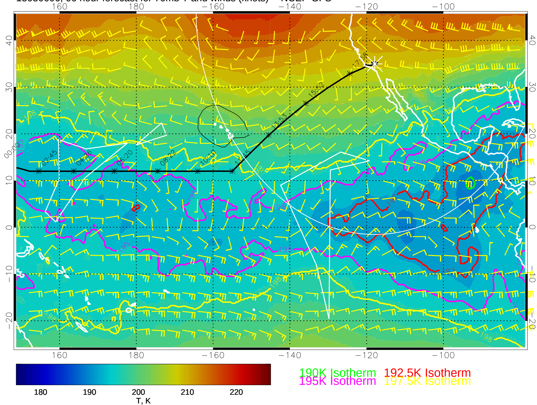
15030606, 90 hour forecast for 70mb T and winds (knots) -- NCEP GFS
