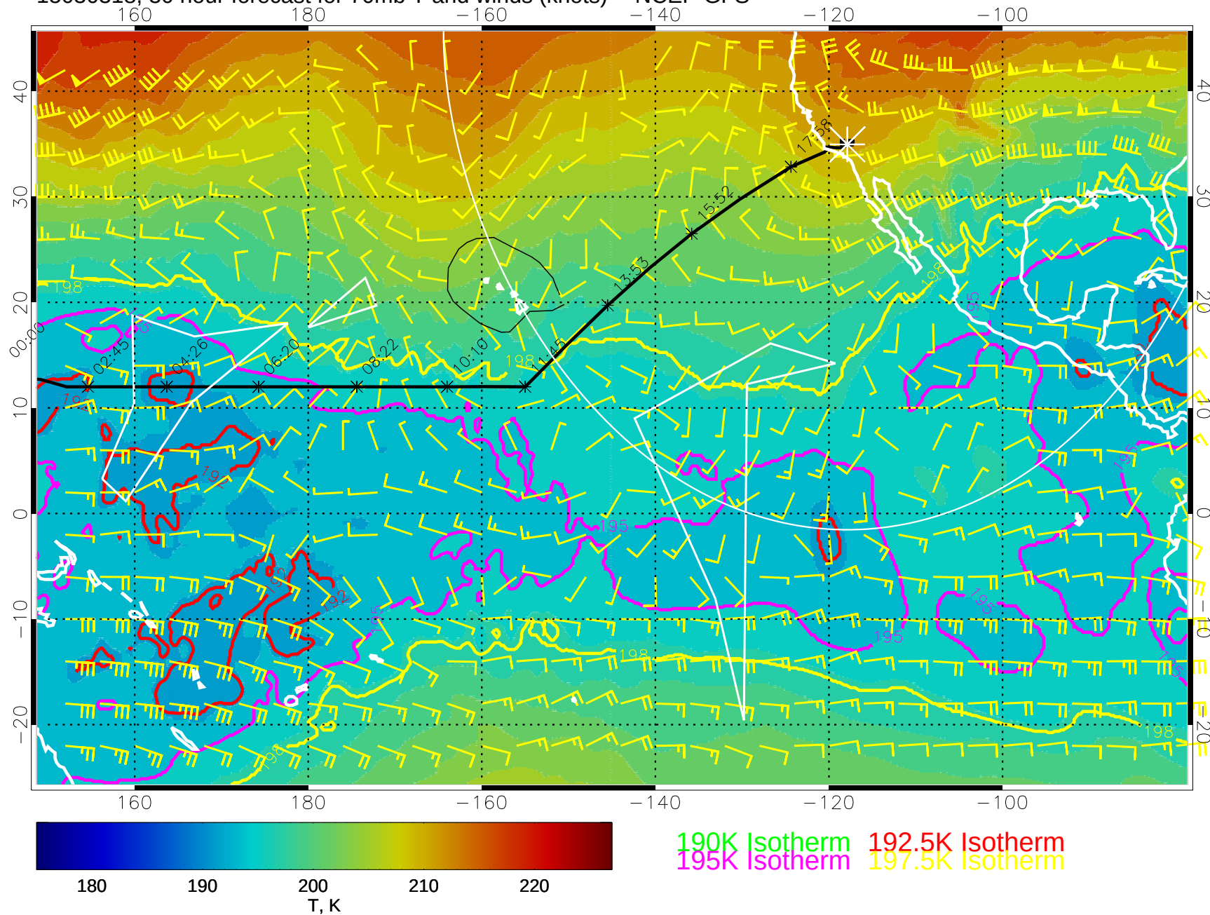
15030318, 30 hour forecast for 70mb T and winds (knots) -- NCEP GFS
