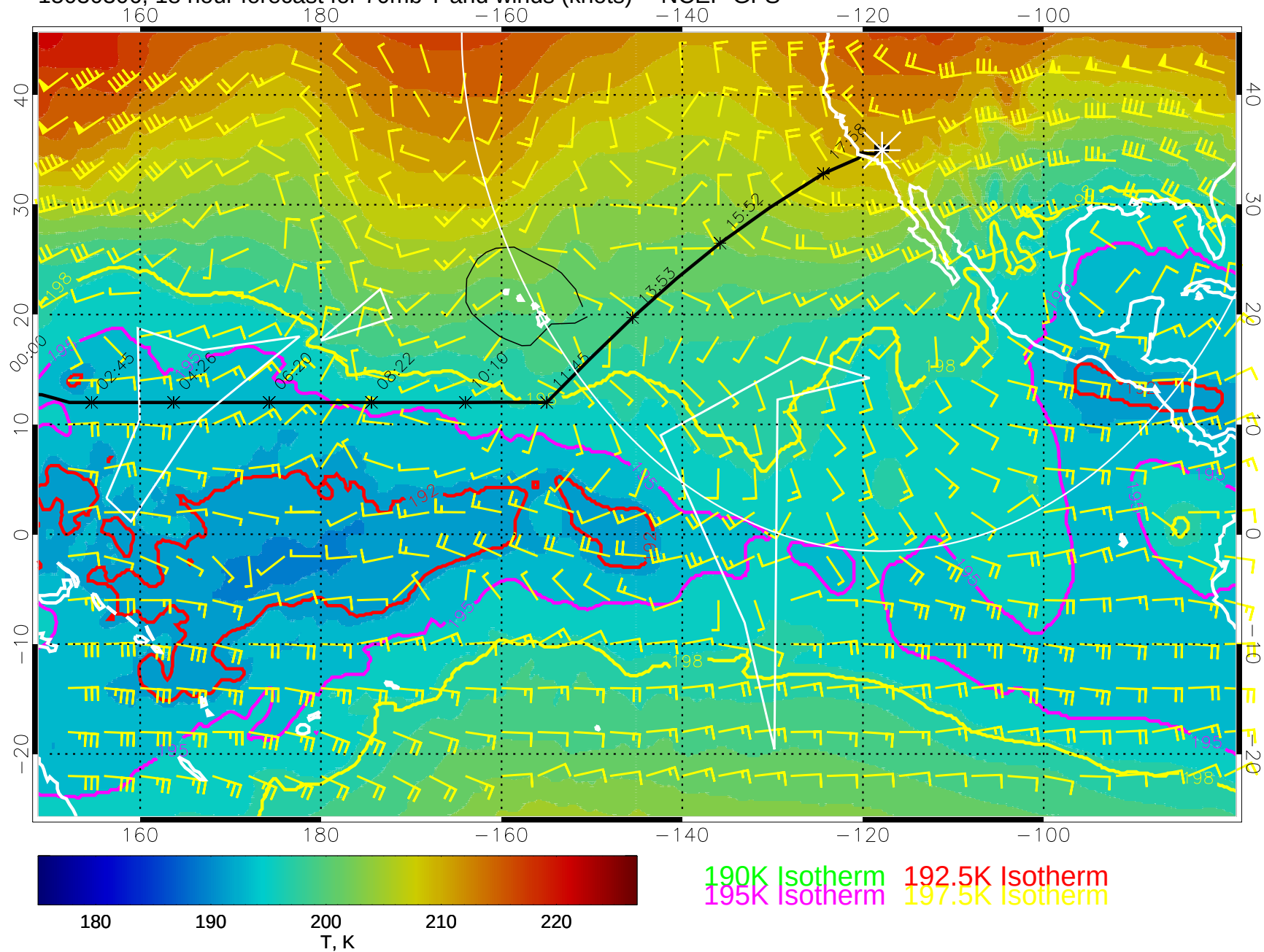
15030306, 18 hour forecast for 70mb T and winds (knots) -- NCEP GFS
