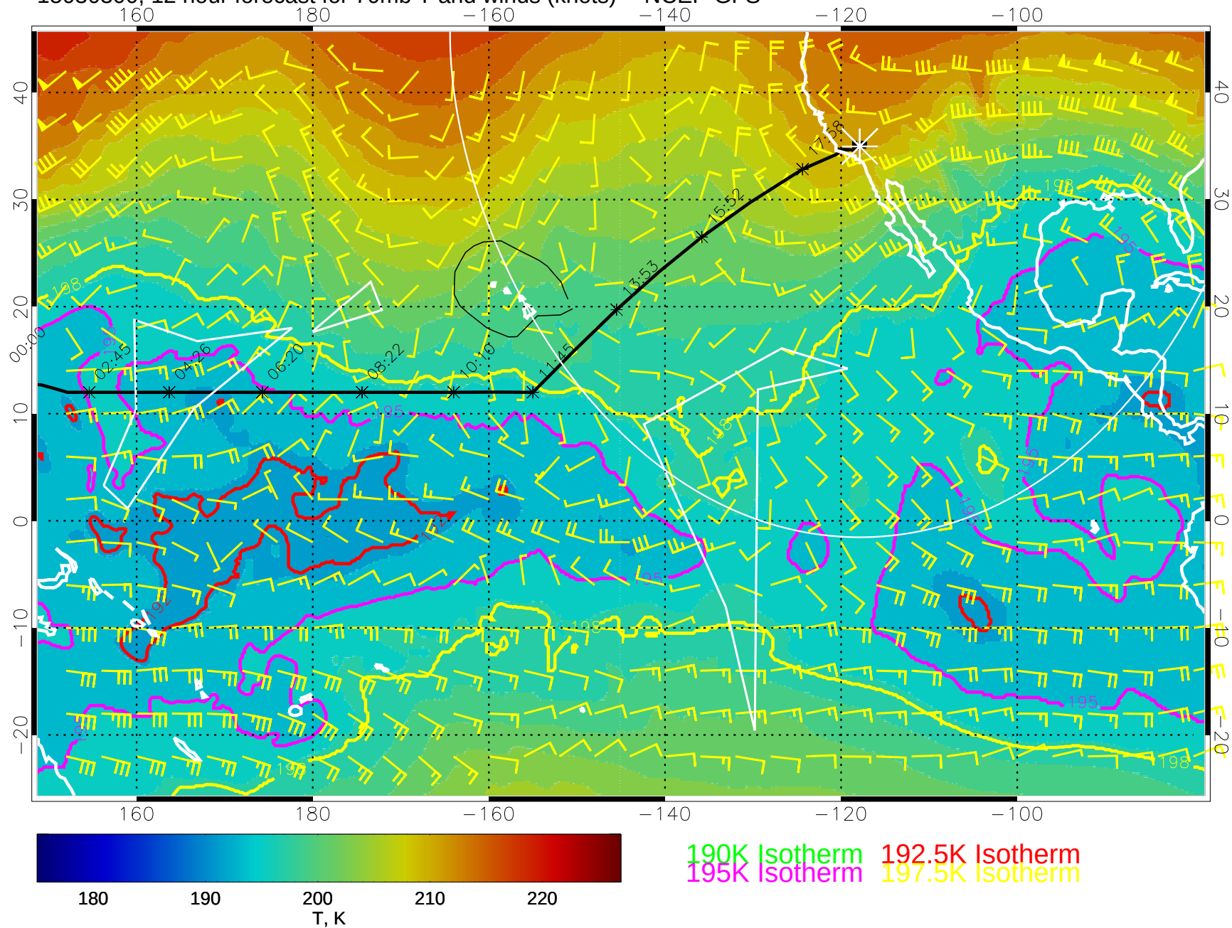
15030300, 12 hour forecast for 70mb T and winds (knots) -- NCEP GFS
