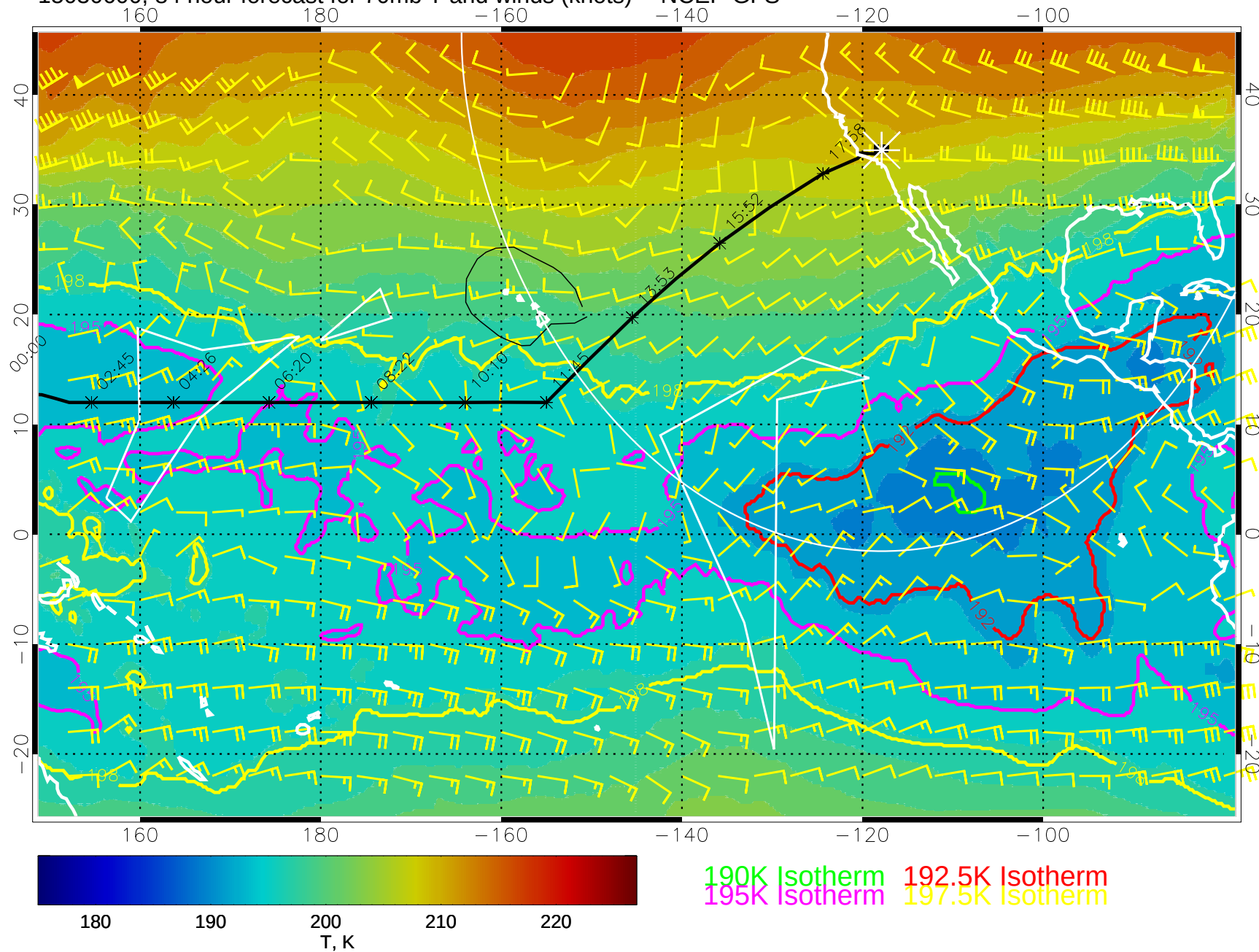
15030600, 84 hour forecast for 70mb T and winds (knots) -- NCEP GFS
