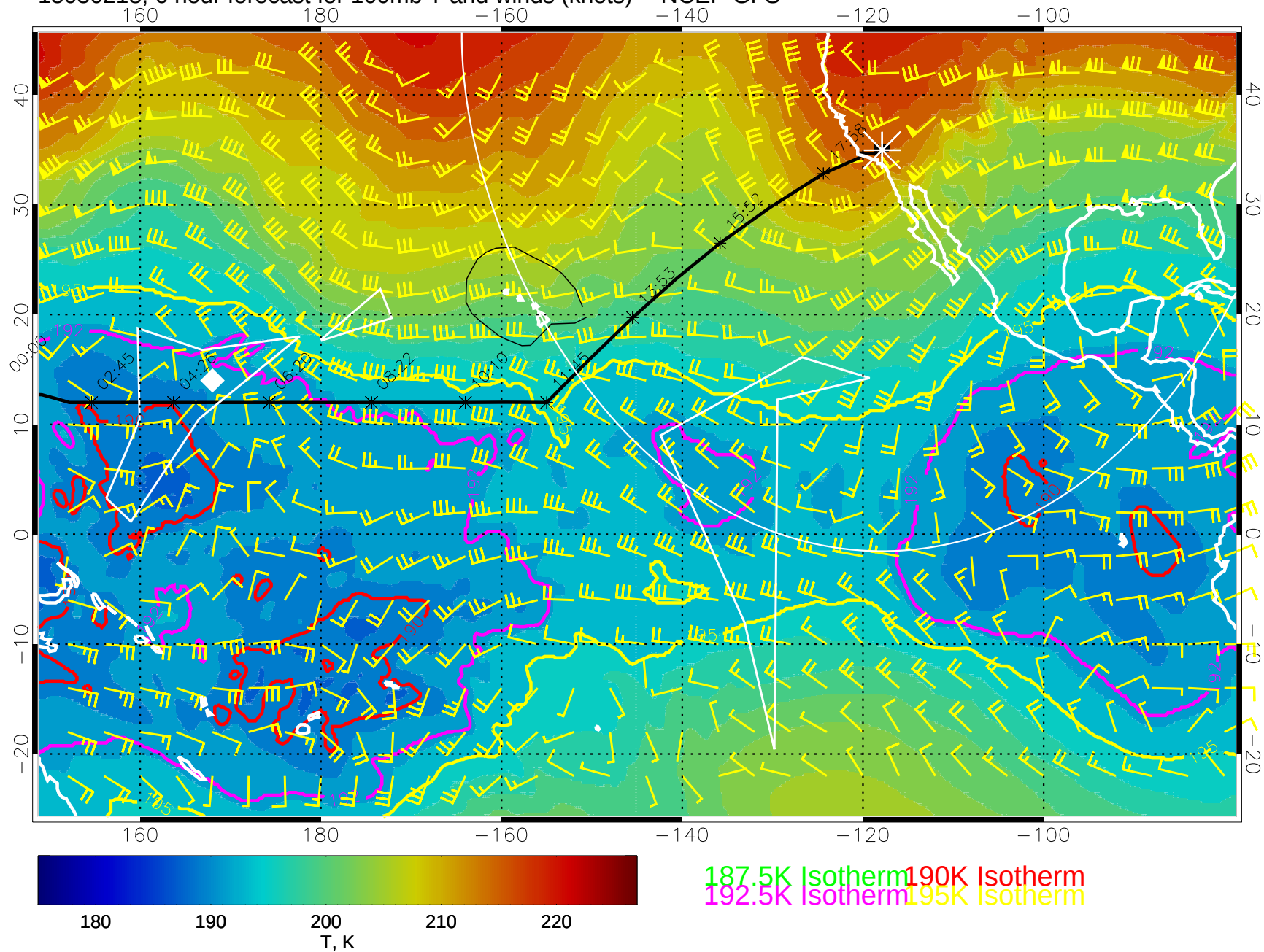
15030218, 6 hour forecast for 100mb T and winds (knots) -- NCEP GFS
