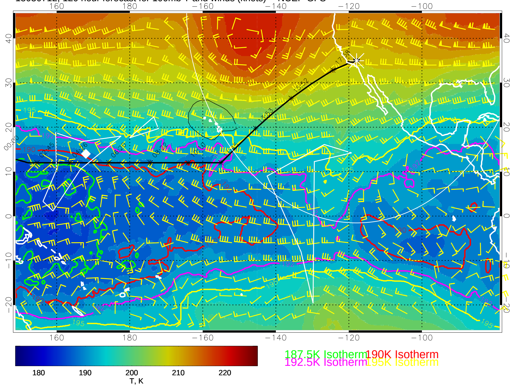
15030712, 120 hour forecast for 100mb T and winds (knots) -- NCEP GFS
