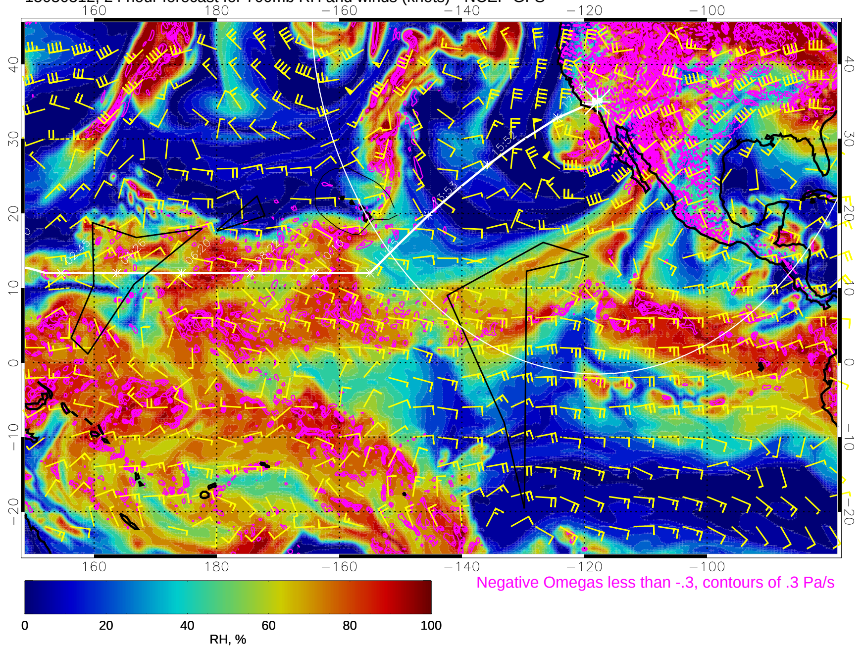
15030312, 24 hour forecast for 700mb RH and winds (knots) - NCEP GFS
