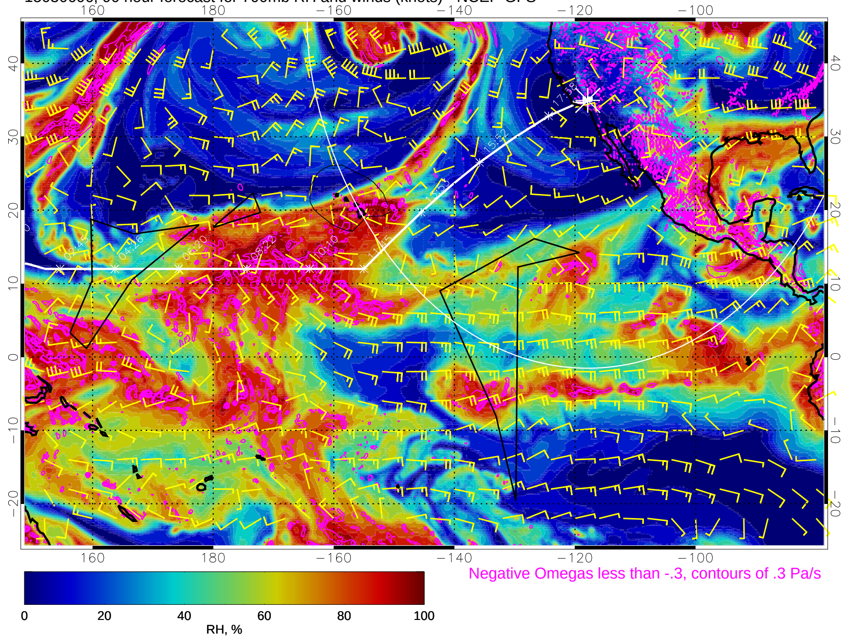
15030606, 90 hour forecast for 700mb RH and winds (knots) - NCEP GFS
