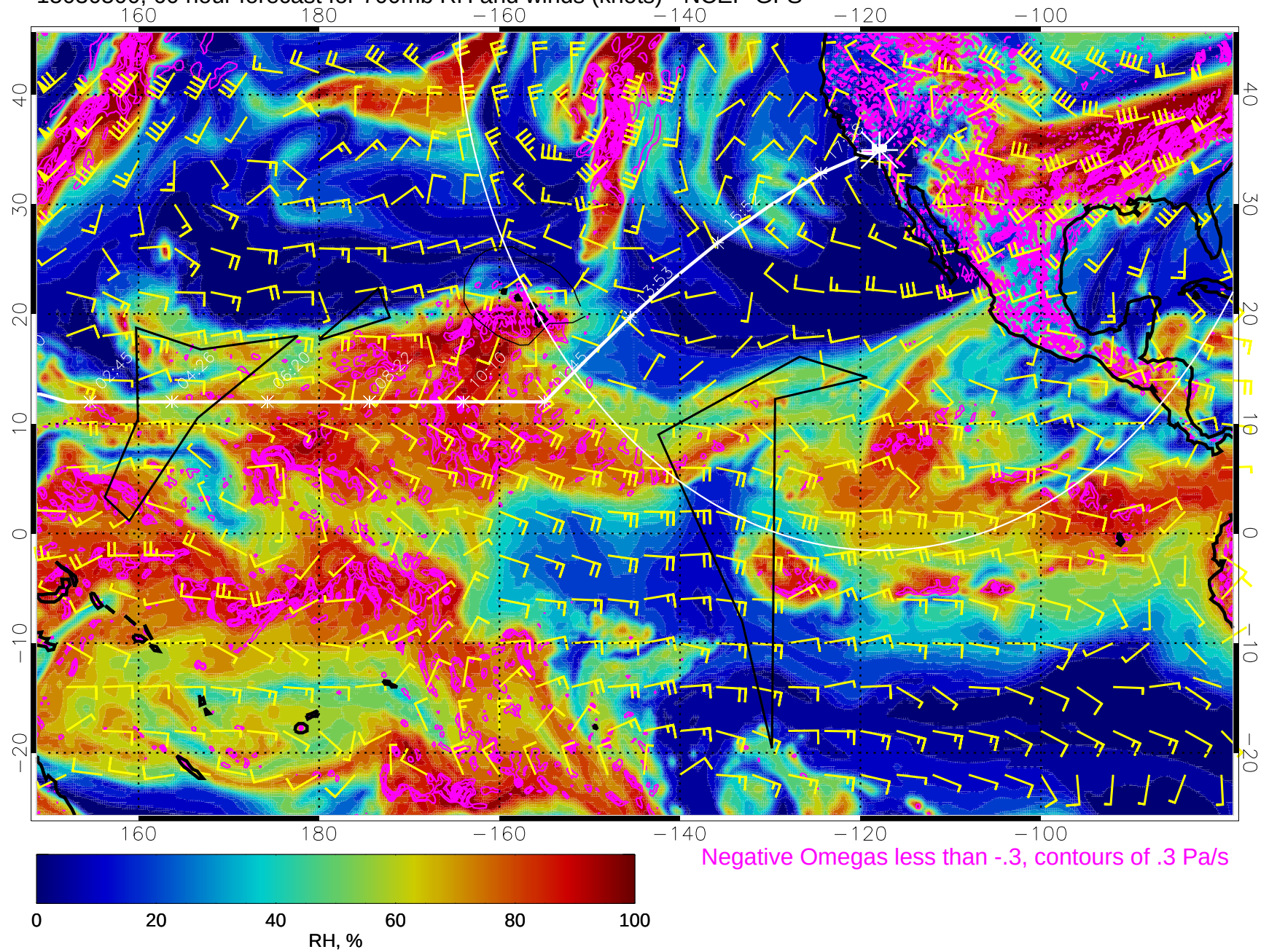
15030500, 60 hour forecast for 700mb RH and winds (knots) - NCEP GFS
