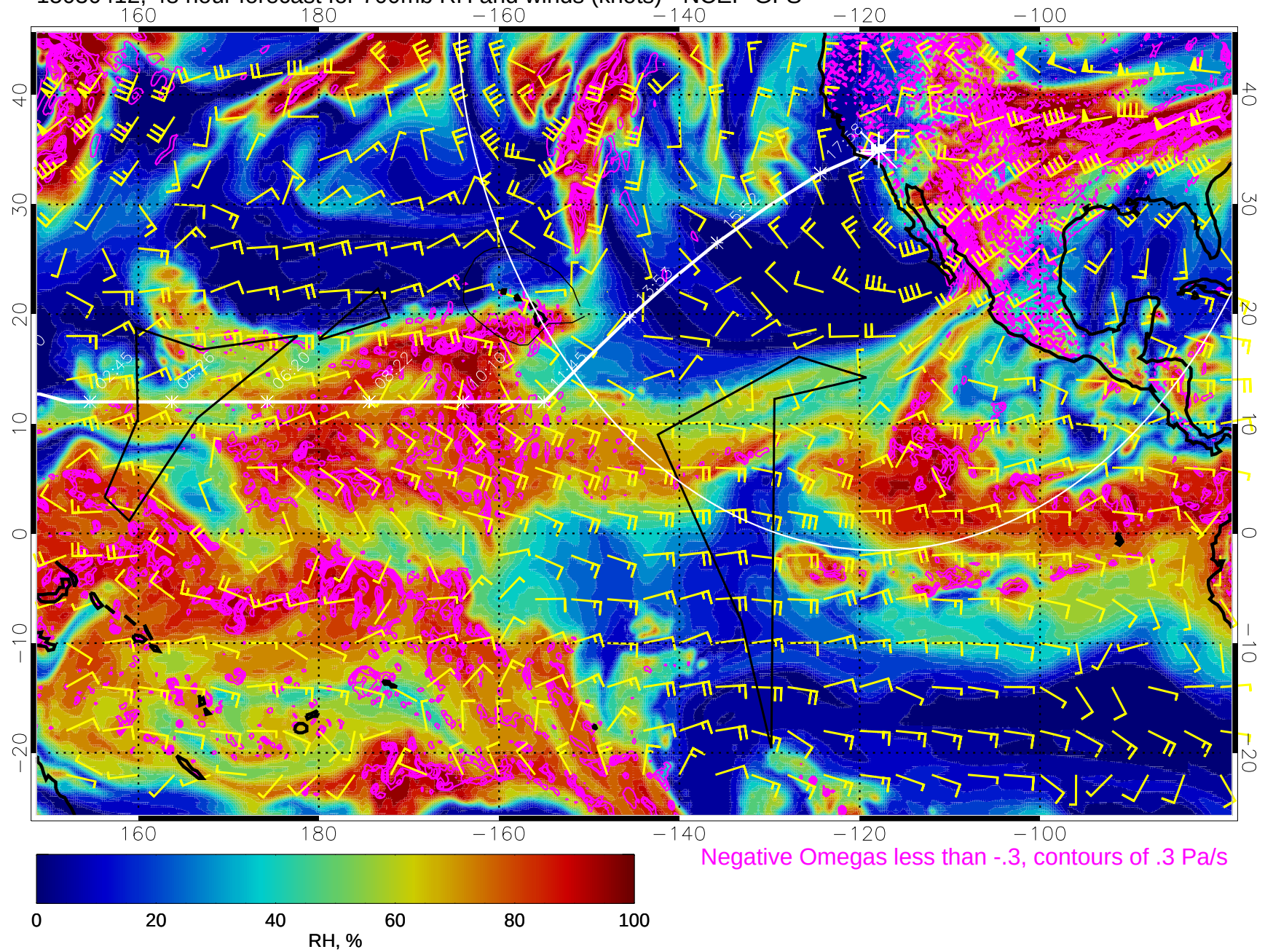
15030412, 48 hour forecast for 700mb RH and winds (knots) - NCEP GFS
