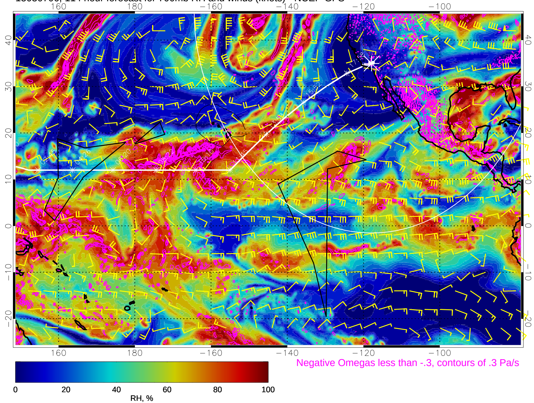
15030706, 114 hour forecast for 700mb RH and winds (knots) - NCEP GFS
