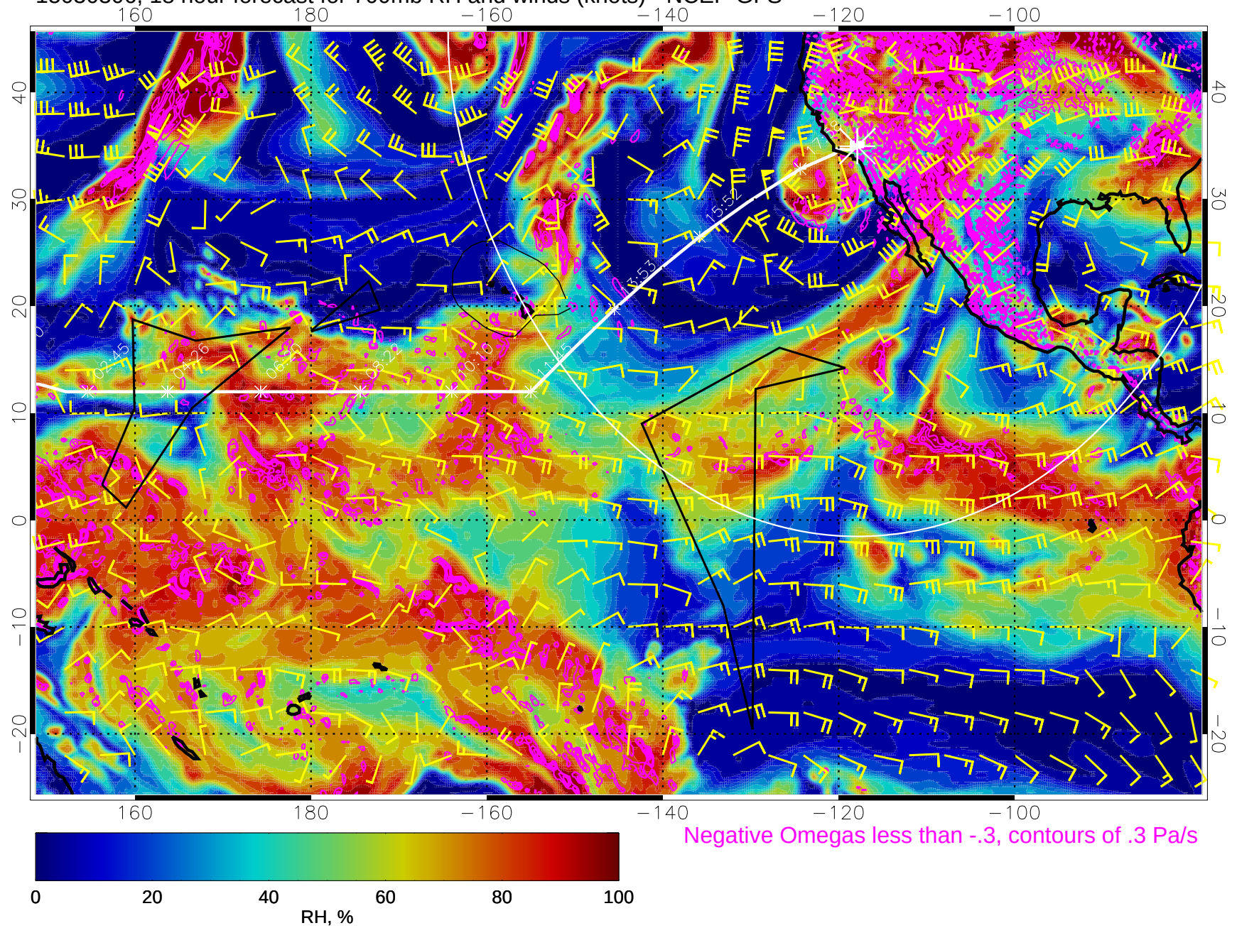
15030306, 18 hour forecast for 700mb RH and winds (knots) - NCEP GFS
