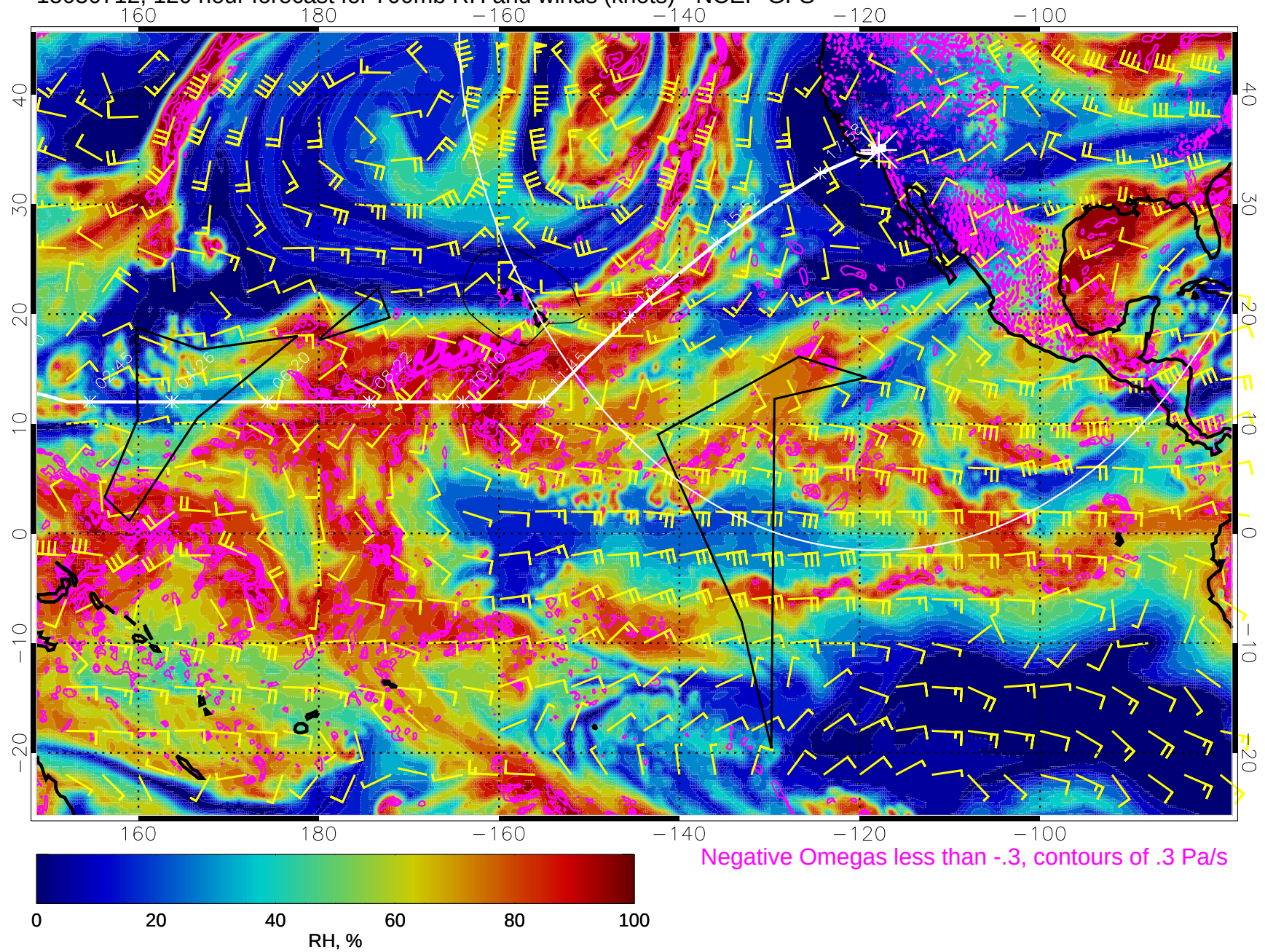
15030712, 120 hour forecast for 700mb RH and winds (knots) - NCEP GFS
