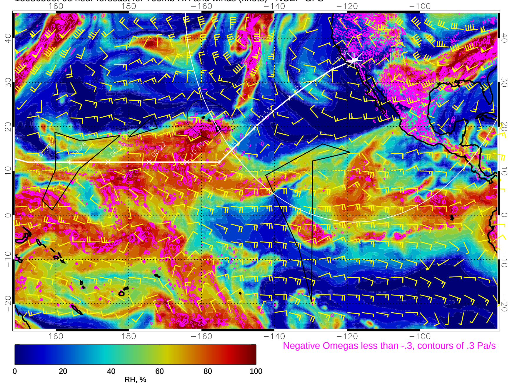
15030506, 66 hour forecast for 700mb RH and winds (knots) - NCEP GFS
