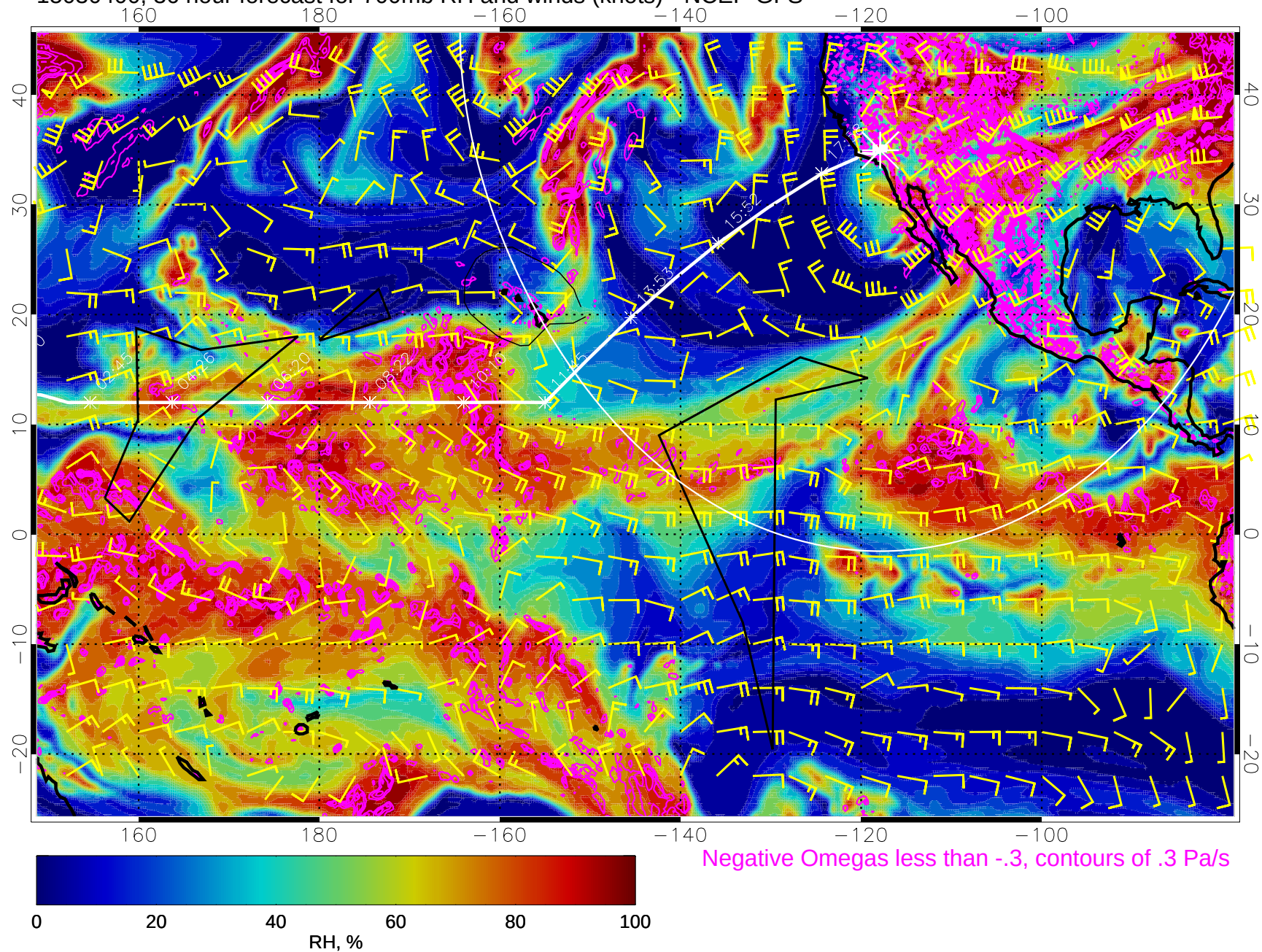
15030400, 36 hour forecast for 700mb RH and winds (knots) - NCEP GFS
