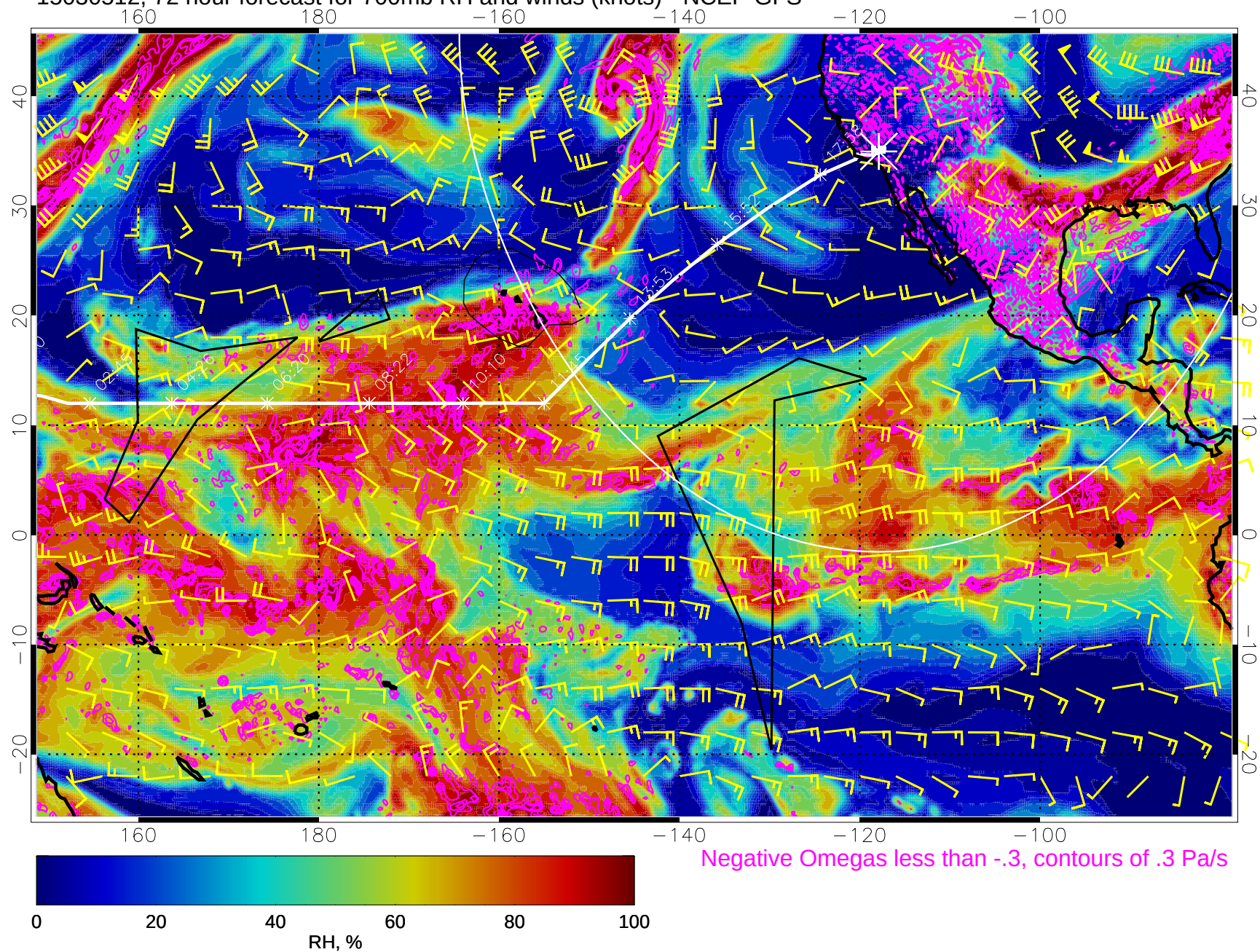
15030512, 72 hour forecast for 700mb RH and winds (knots) - NCEP GFS
