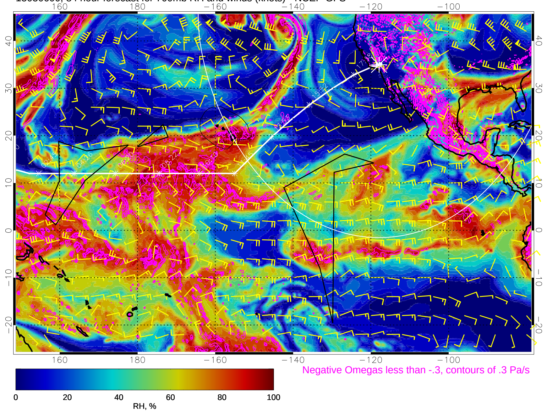
15030600, 84 hour forecast for 700mb RH and winds (knots) - NCEP GFS
