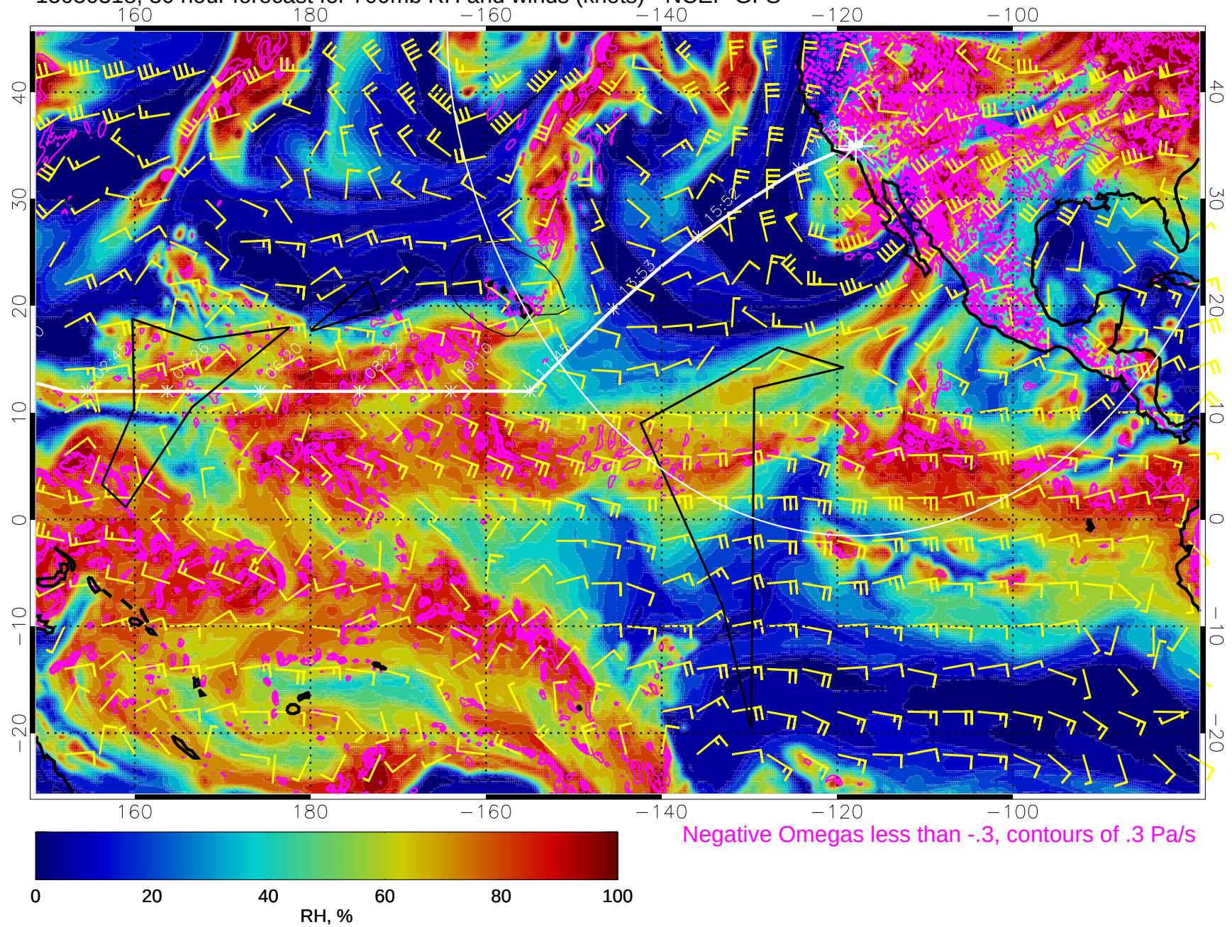
15030318, 30 hour forecast for 700mb RH and winds (knots) - NCEP GFS
