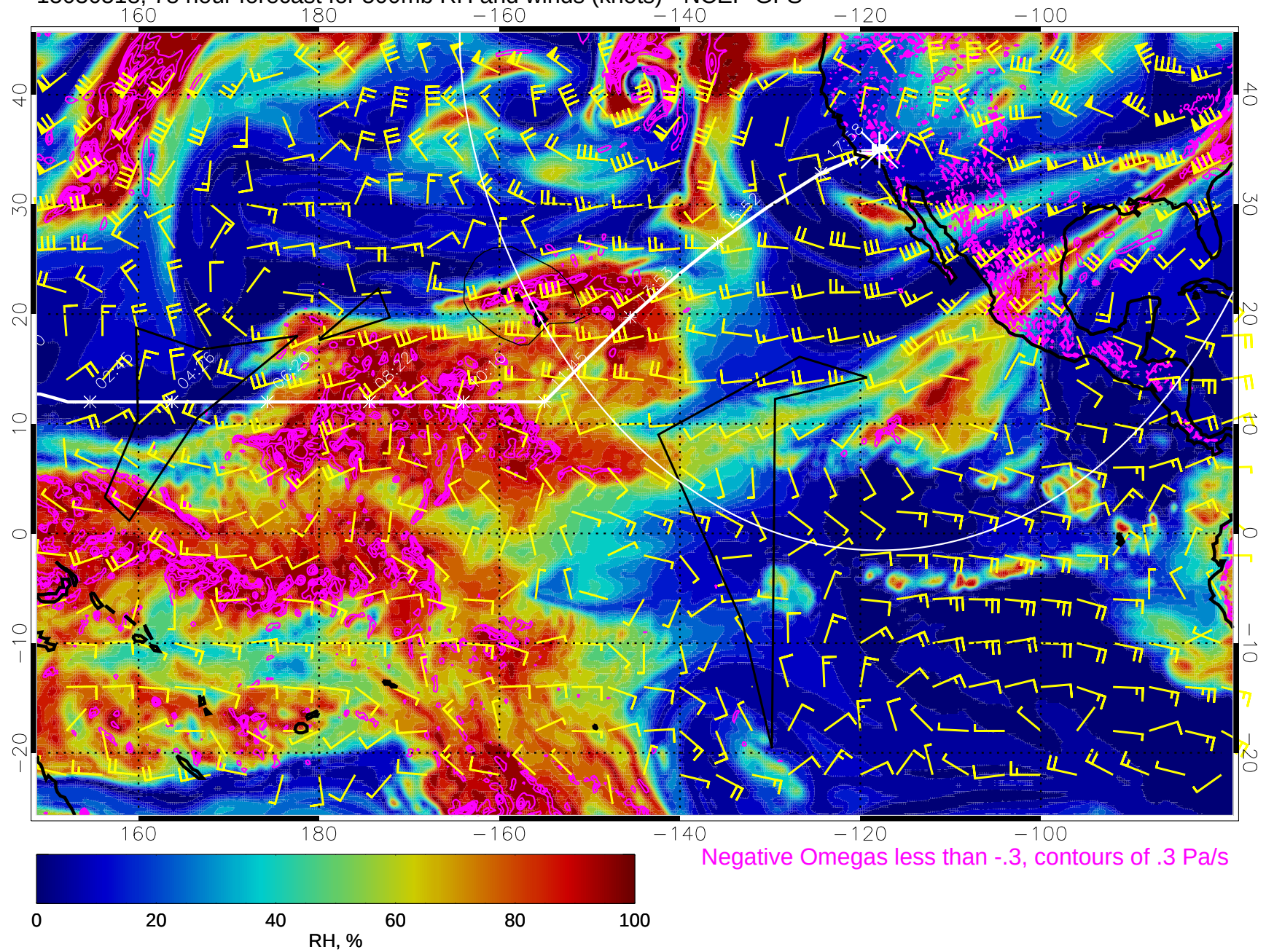
15030518, 78 hour forecast for 500mb RH and winds (knots) - NCEP GFS
