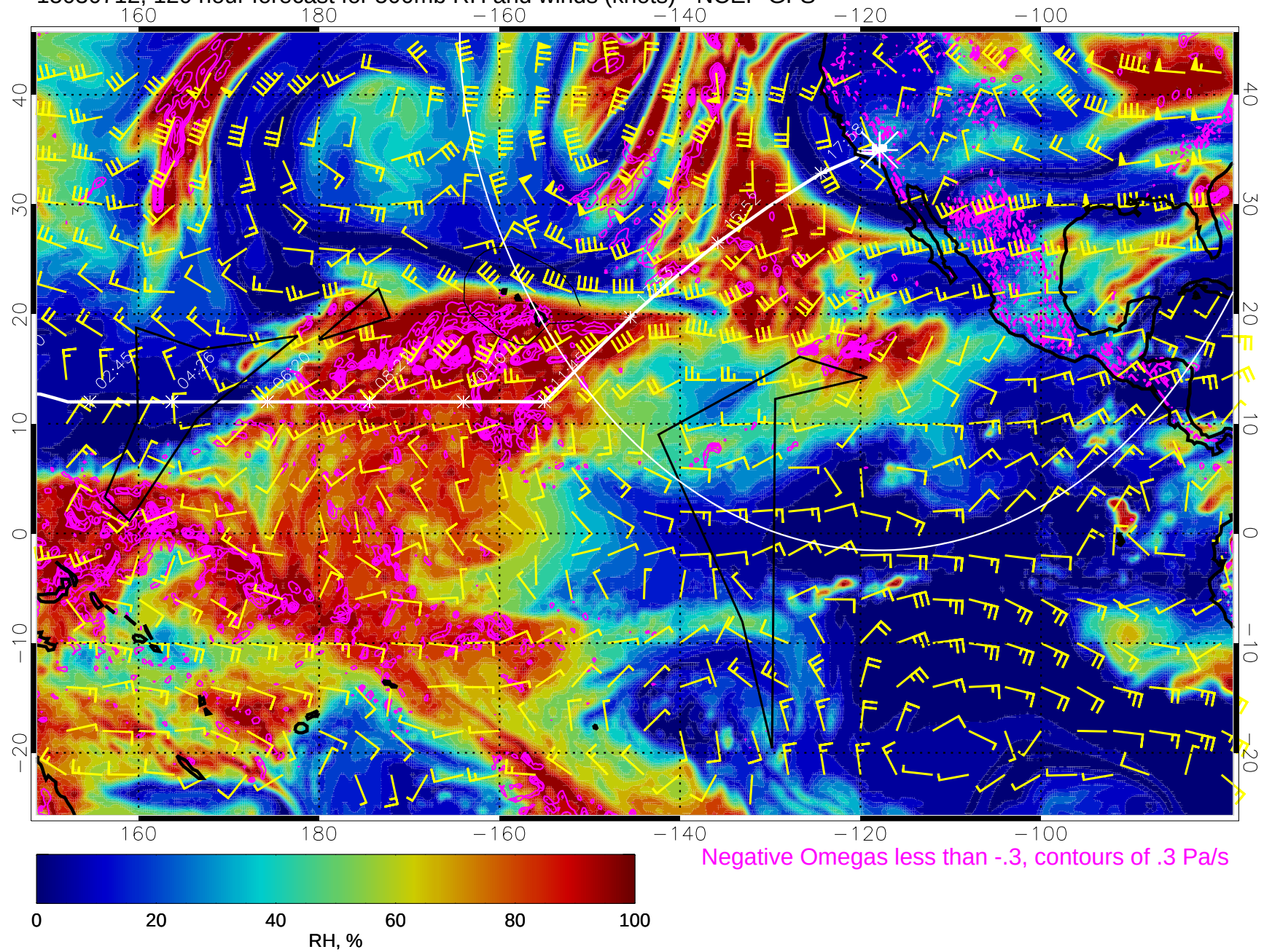
15030712, 120 hour forecast for 500mb RH and winds (knots) - NCEP GFS
