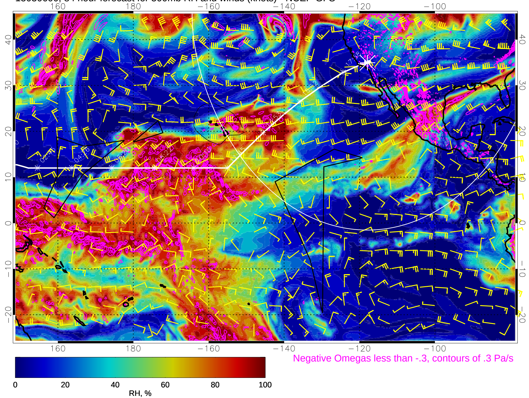
15030600, 84 hour forecast for 500mb RH and winds (knots) - NCEP GFS
