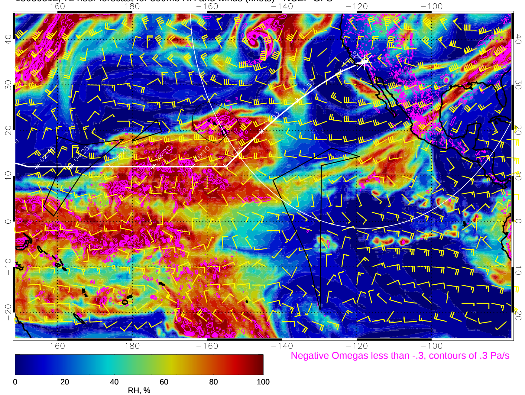
15030512, 72 hour forecast for 500mb RH and winds (knots) - NCEP GFS
