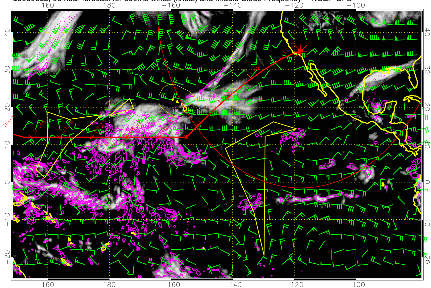
15030612, 96 hour forecast for 500mb winds (knots) and Middle Cloud Frequency -- NCEP GFS
