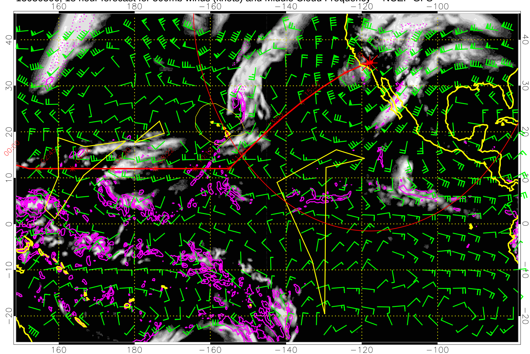
15030306, 18 hour forecast for 500mb winds (knots) and Middle Cloud Frequency -- NCEP GFS
