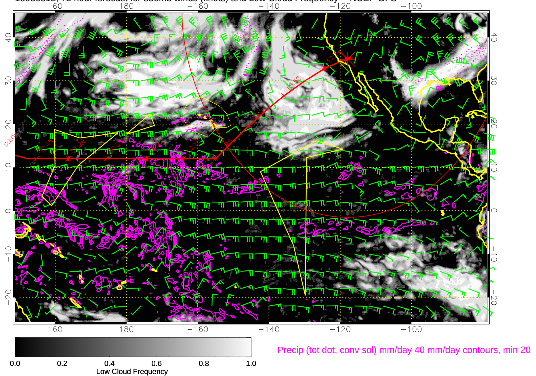
15030512, 72 hour forecast for 850mb winds (knots) and Low Cloud Frequency -- NCEP GFS
