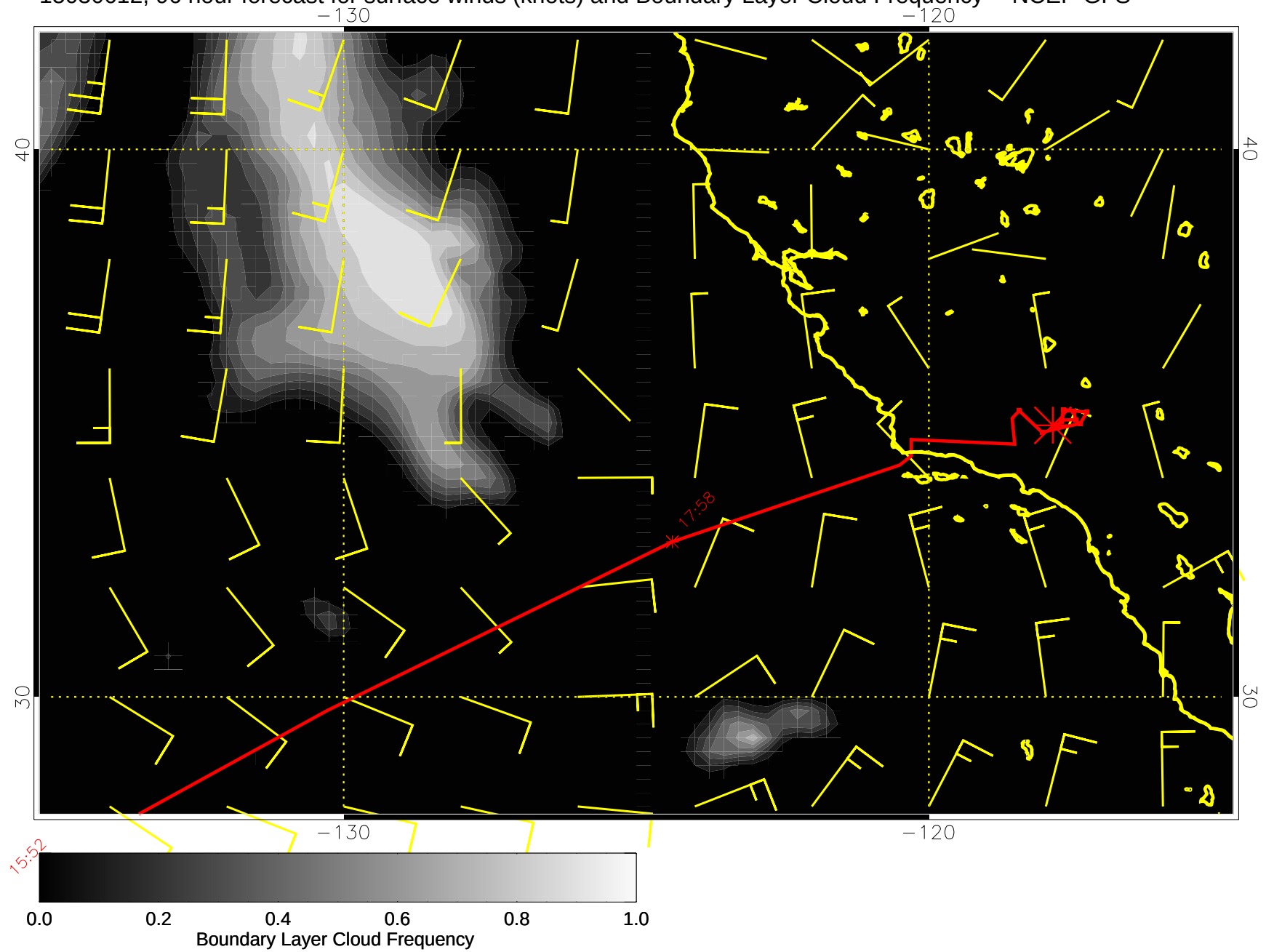
15030612, 96 hour forecast for surface winds (knots) and Boundary Layer Cloud Frequency -- NCEP GFS
