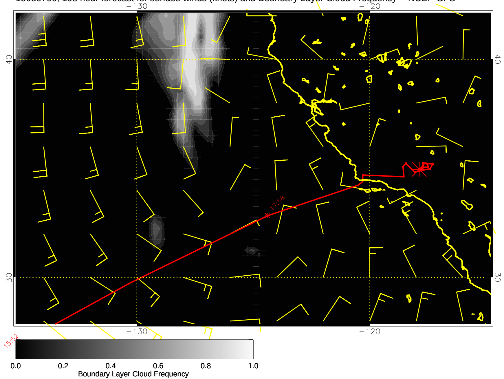
15030700, 108 hour forecast for surface winds (knots) and Boundary Layer Cloud Frequency -- NCEP GFS
