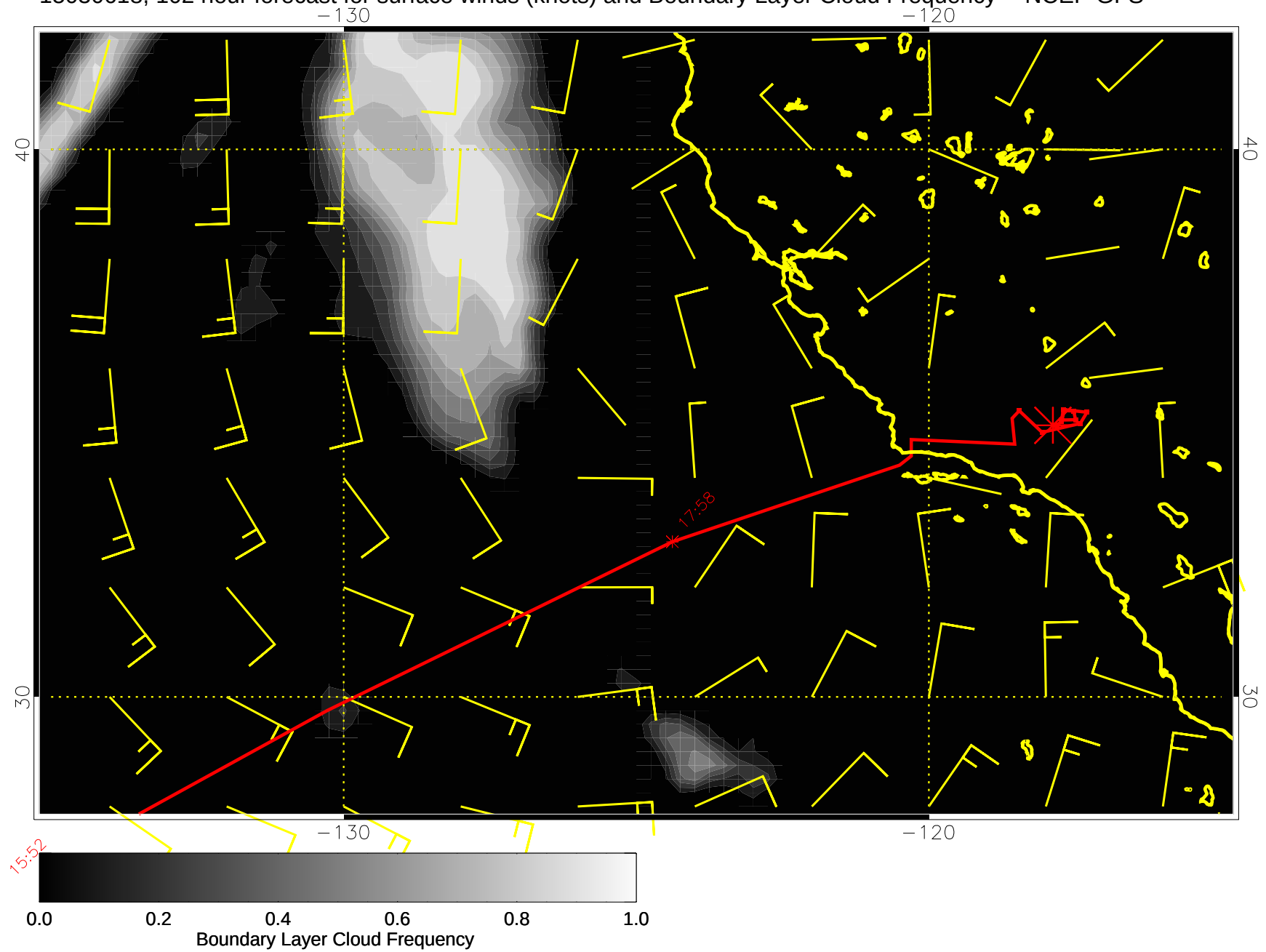
15030618, 102 hour forecast for surface winds (knots) and Boundary Layer Cloud Frequency -- NCEP GFS
