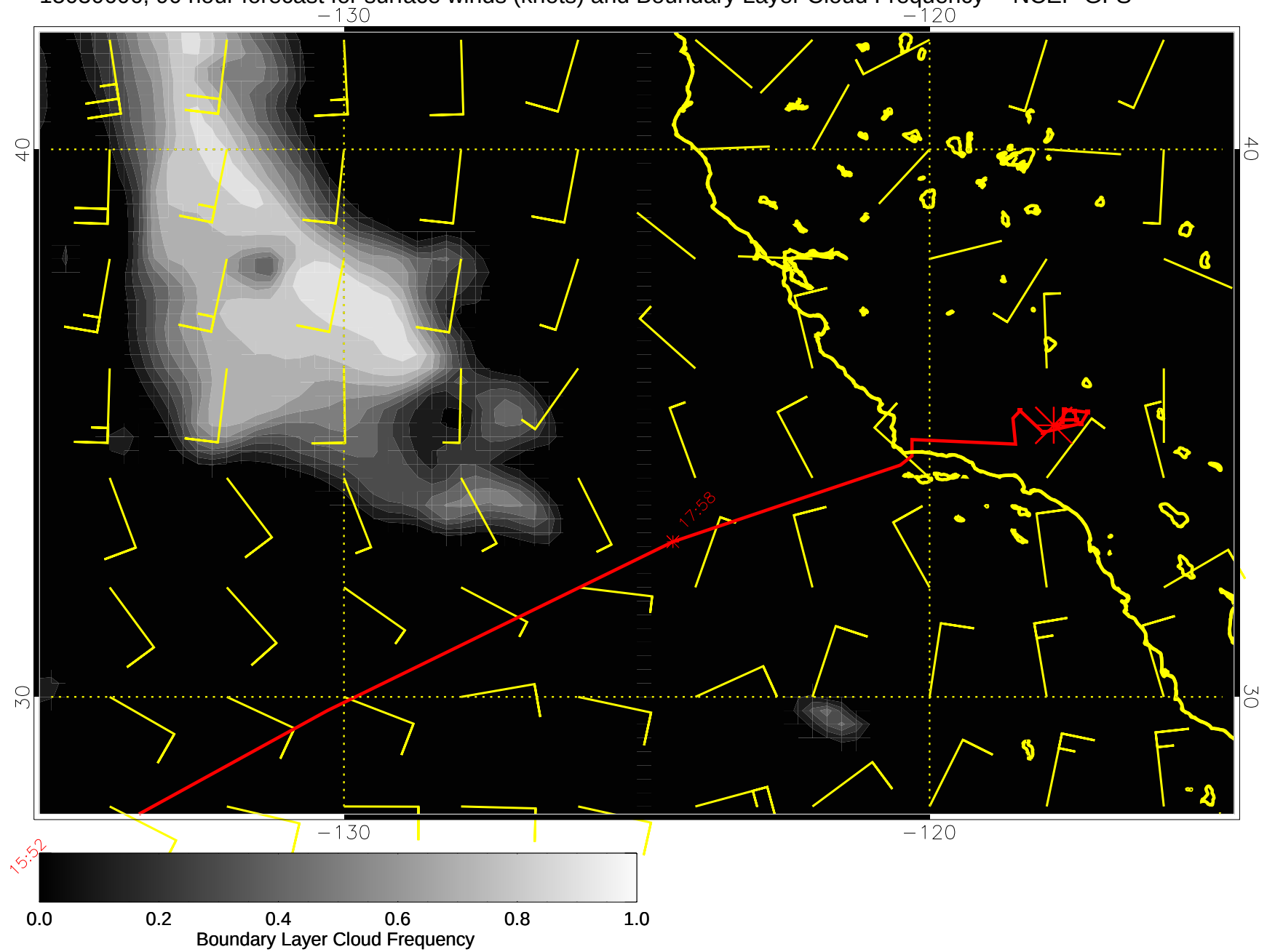
15030606, 90 hour forecast for surface winds (knots) and Boundary Layer Cloud Frequency -- NCEP GFS
