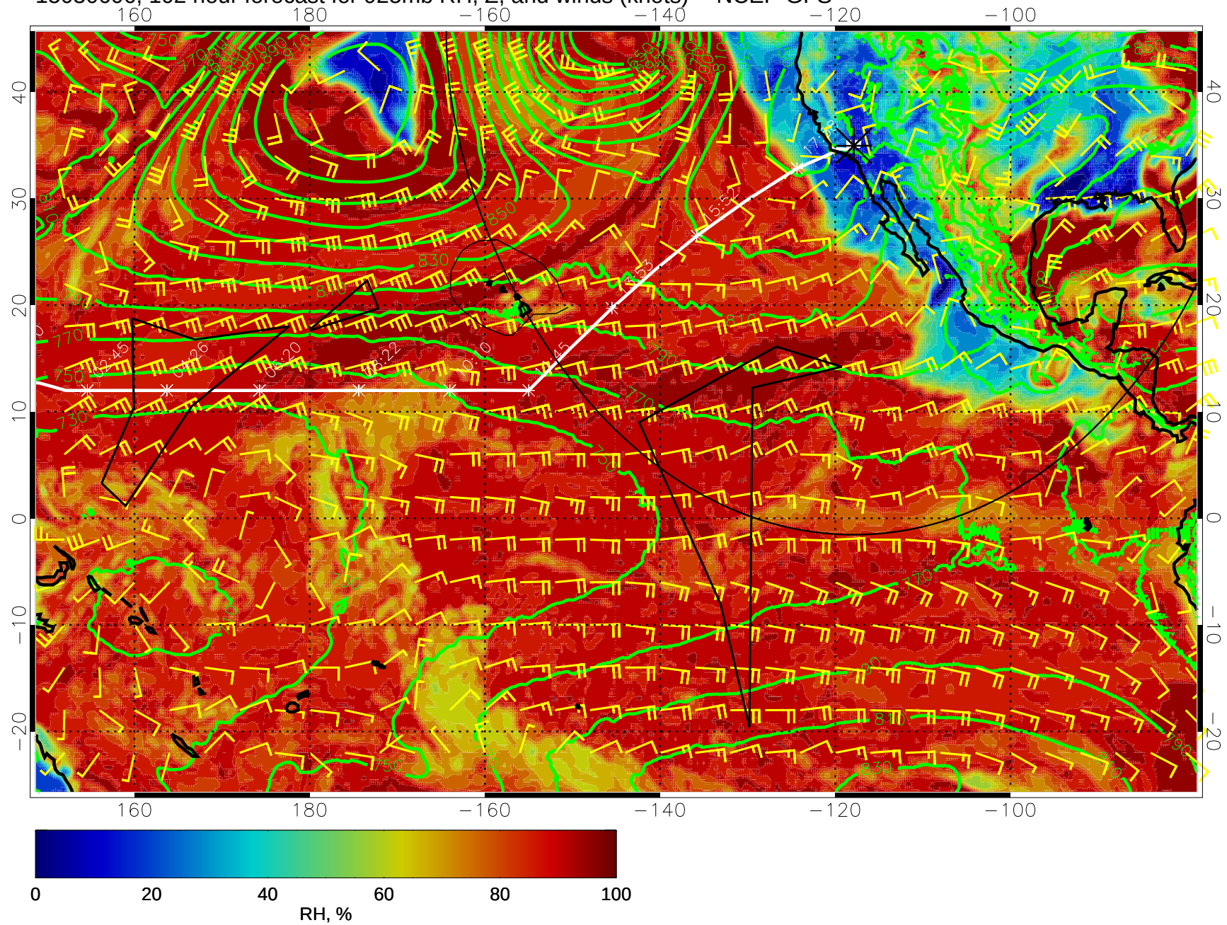
15030606, 102 hour forecast for 925mb RH, Z, and winds (knots) -- NCEP GFS
