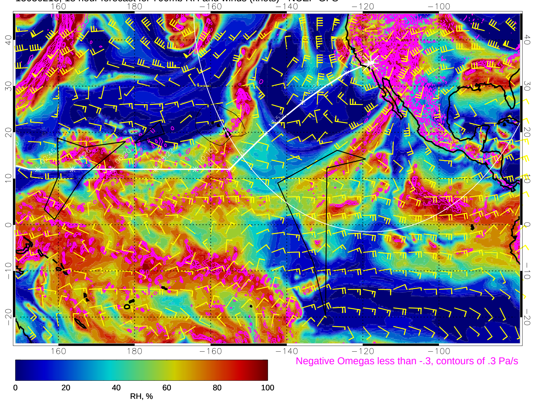
15030218, 18 hour forecast for 700mb RH and winds (knots) - NCEP GFS
