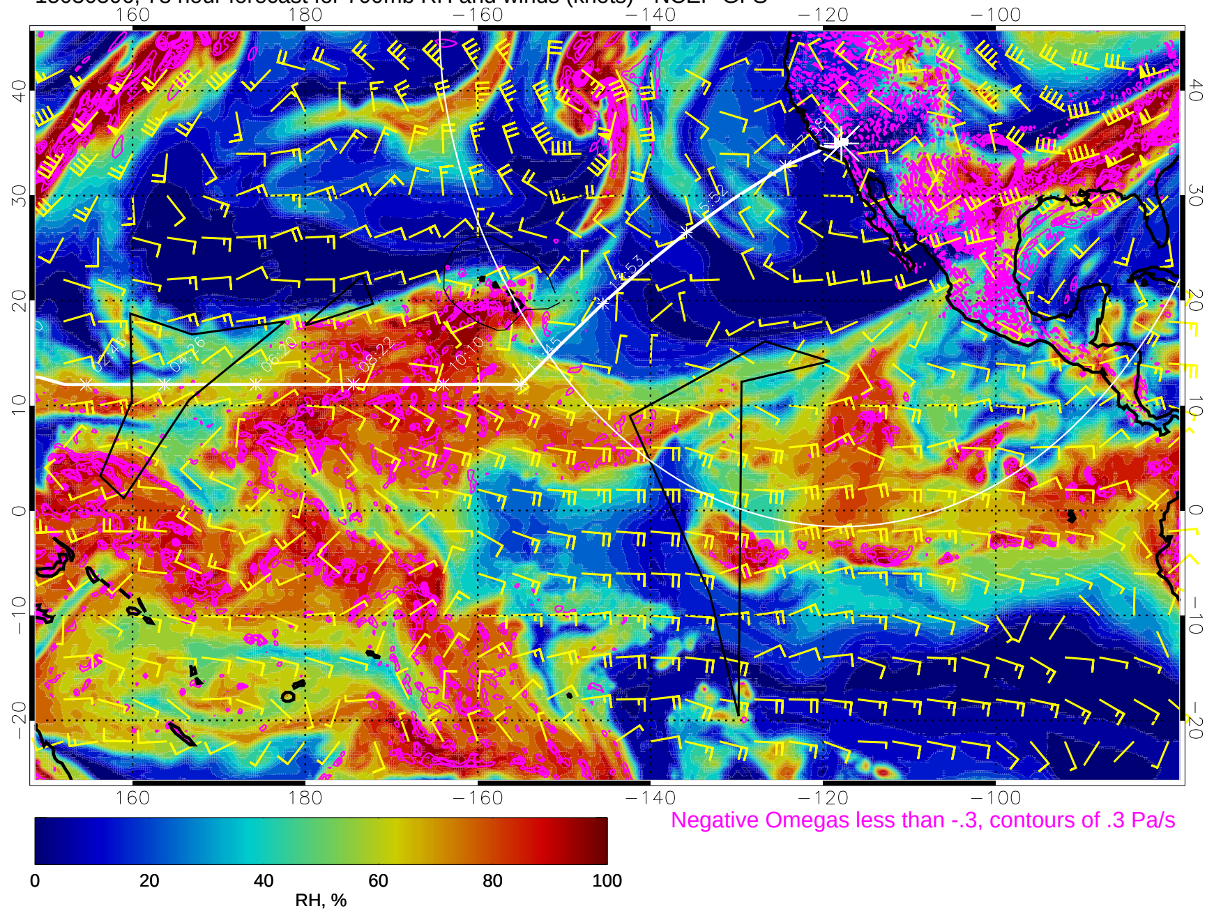
15030506, 78 hour forecast for 700mb RH and winds (knots) - NCEP GFS
