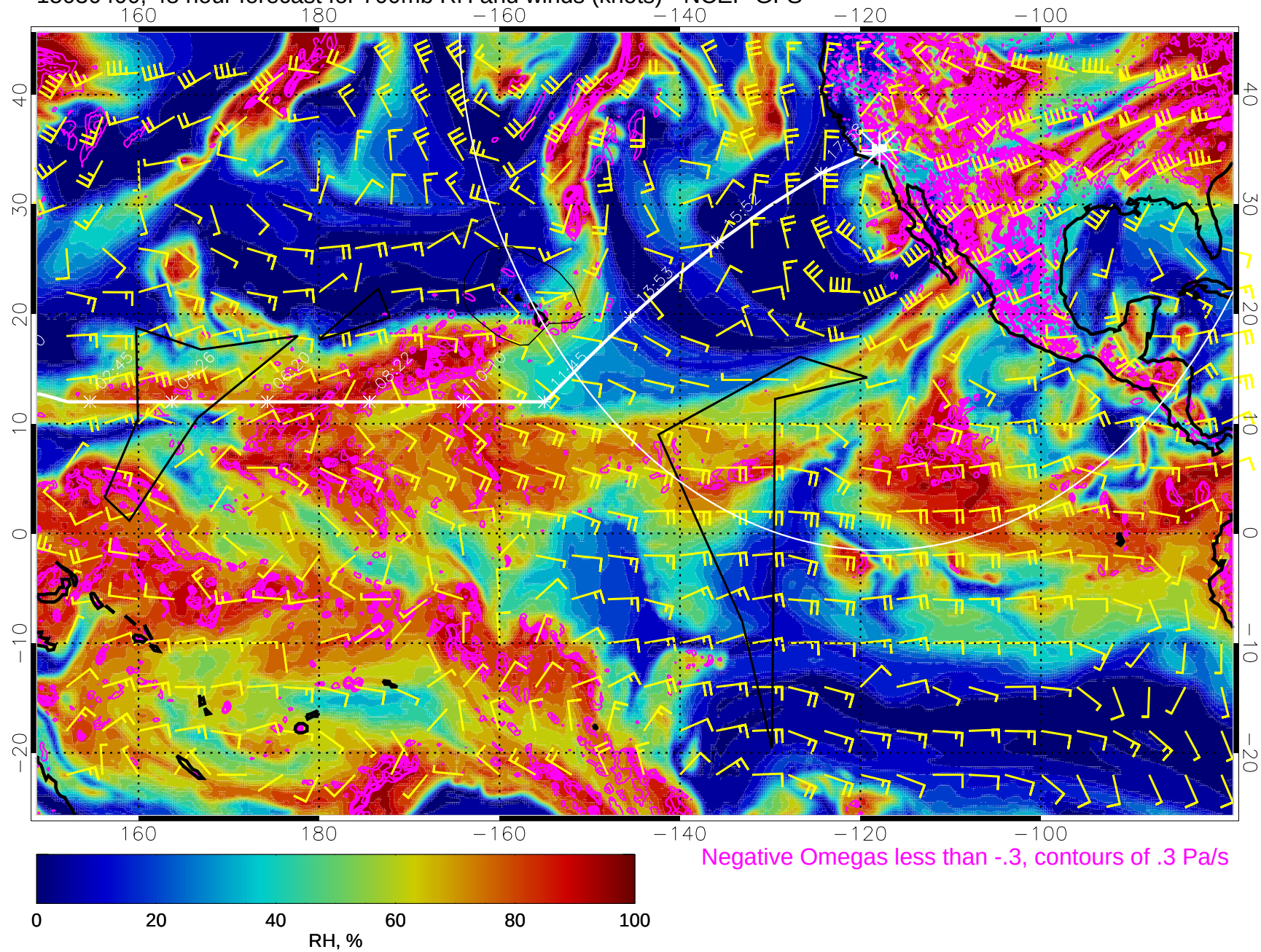
15030400, 48 hour forecast for 700mb RH and winds (knots) - NCEP GFS
