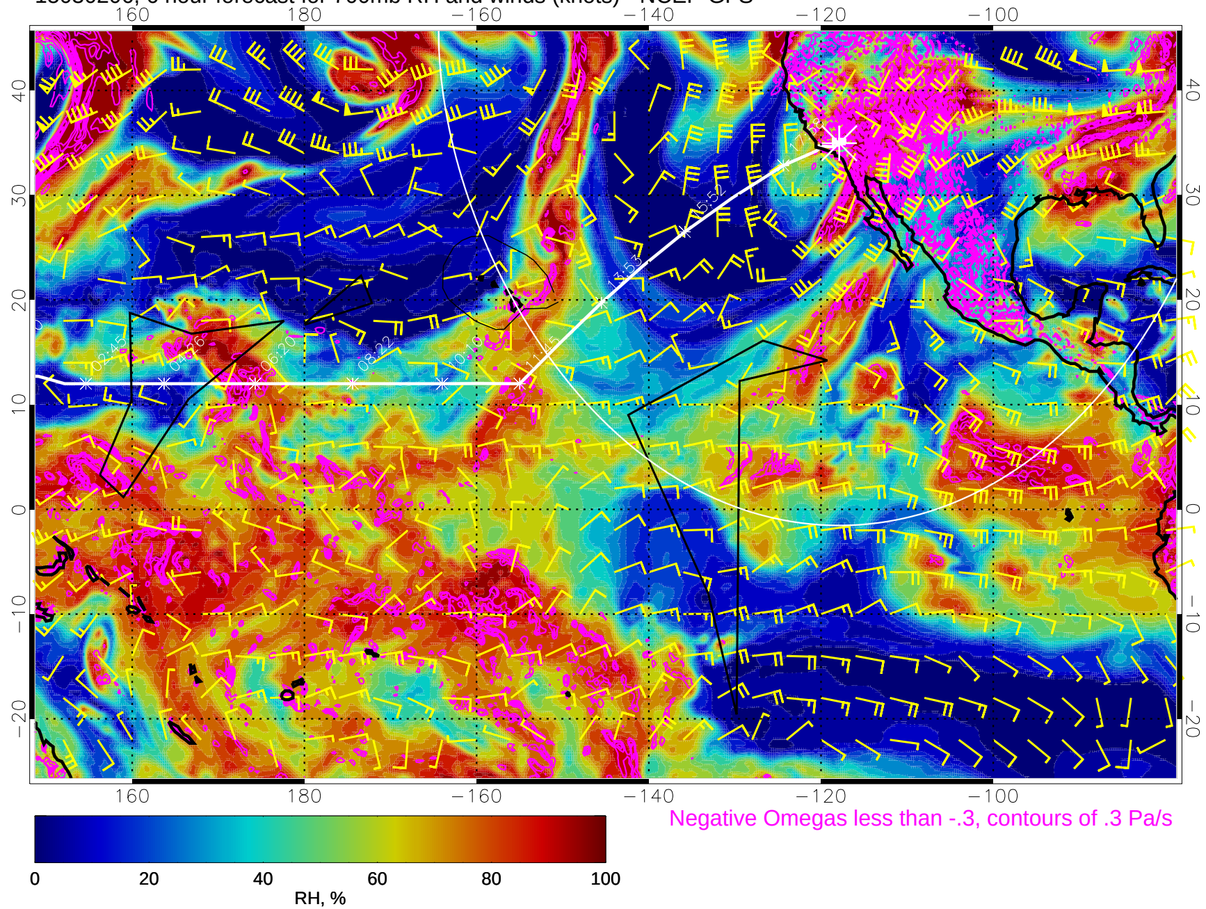
15030206, 6 hour forecast for 700mb RH and winds (knots) - NCEP GFS
