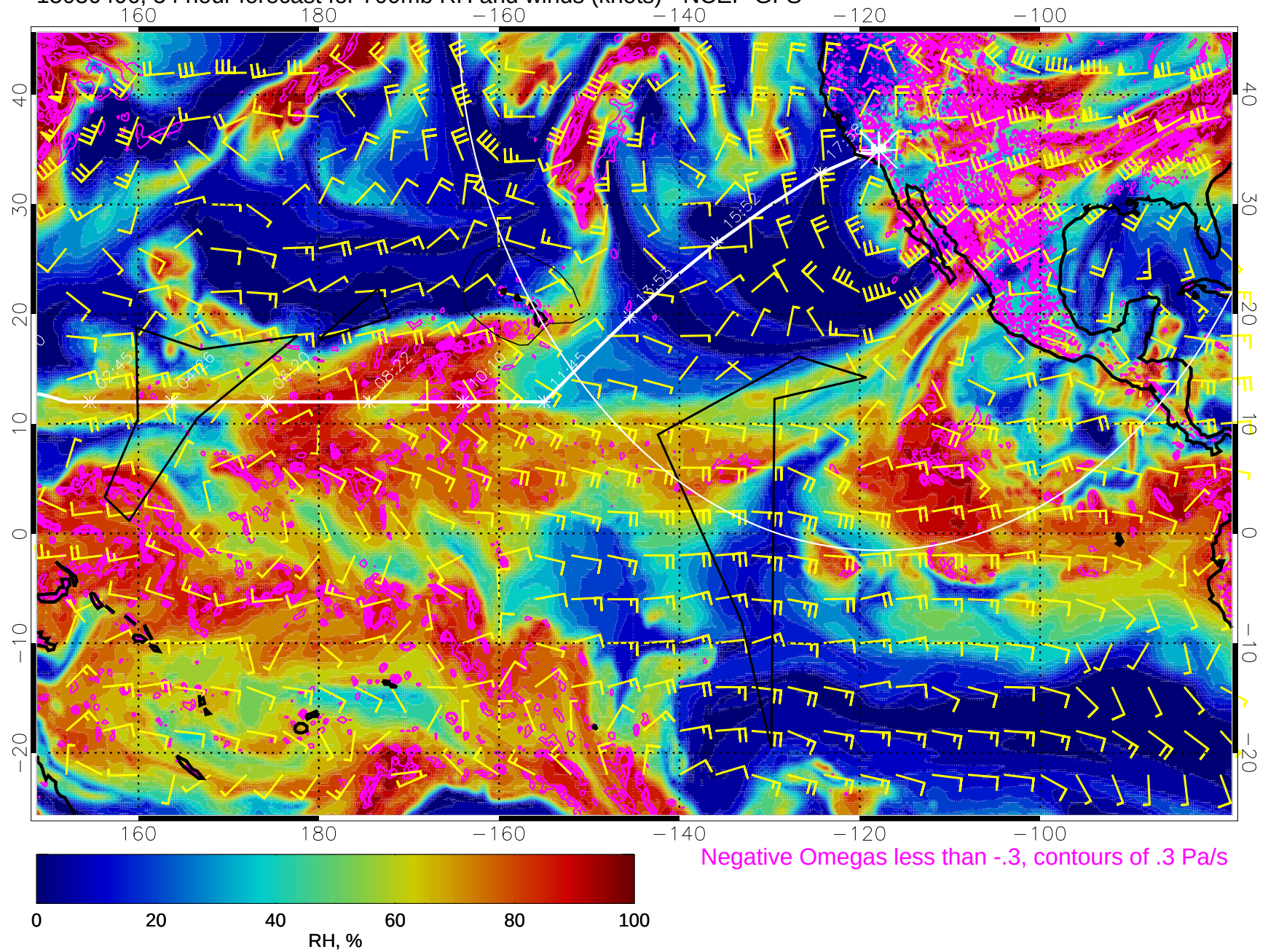
15030406, 54 hour forecast for 700mb RH and winds (knots) - NCEP GFS
