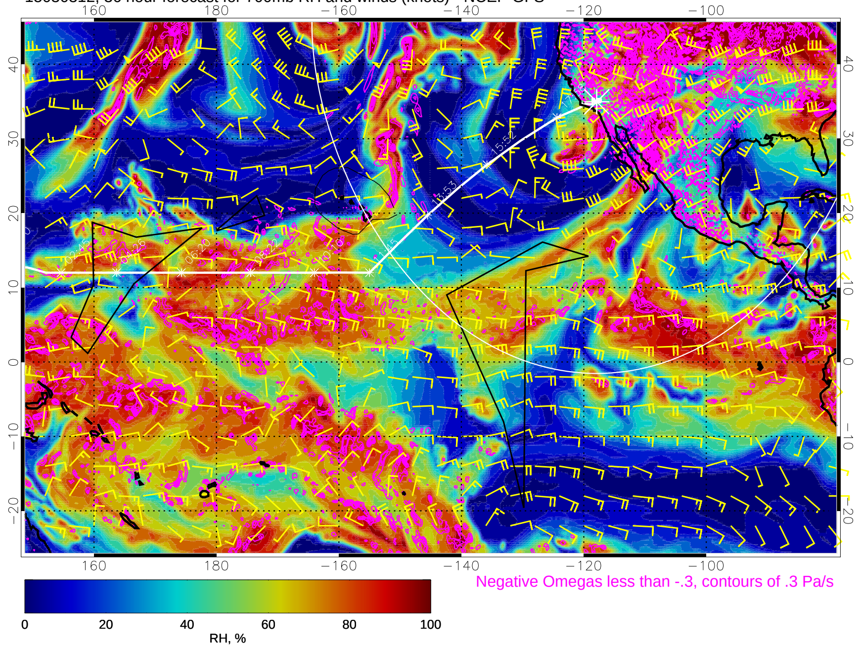
15030312, 36 hour forecast for 700mb RH and winds (knots) - NCEP GFS
