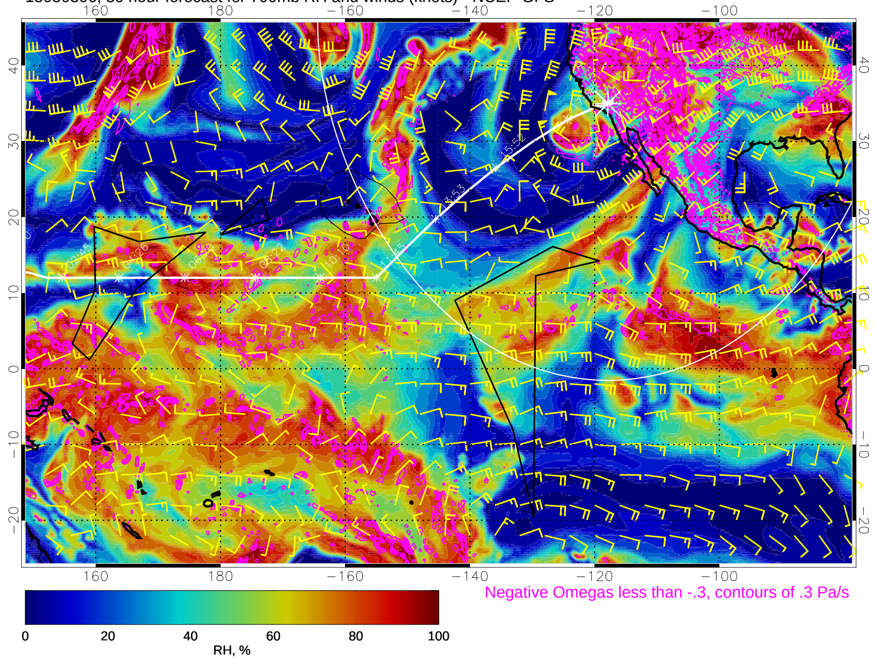
15030306, 30 hour forecast for 700mb RH and winds (knots) - NCEP GFS
