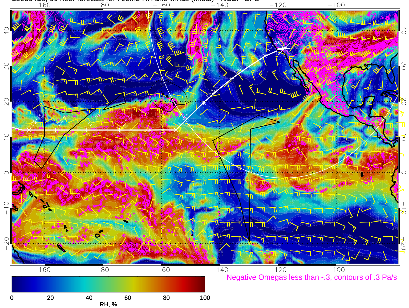
15030418, 66 hour forecast for 700mb RH and winds (knots) - NCEP GFS
