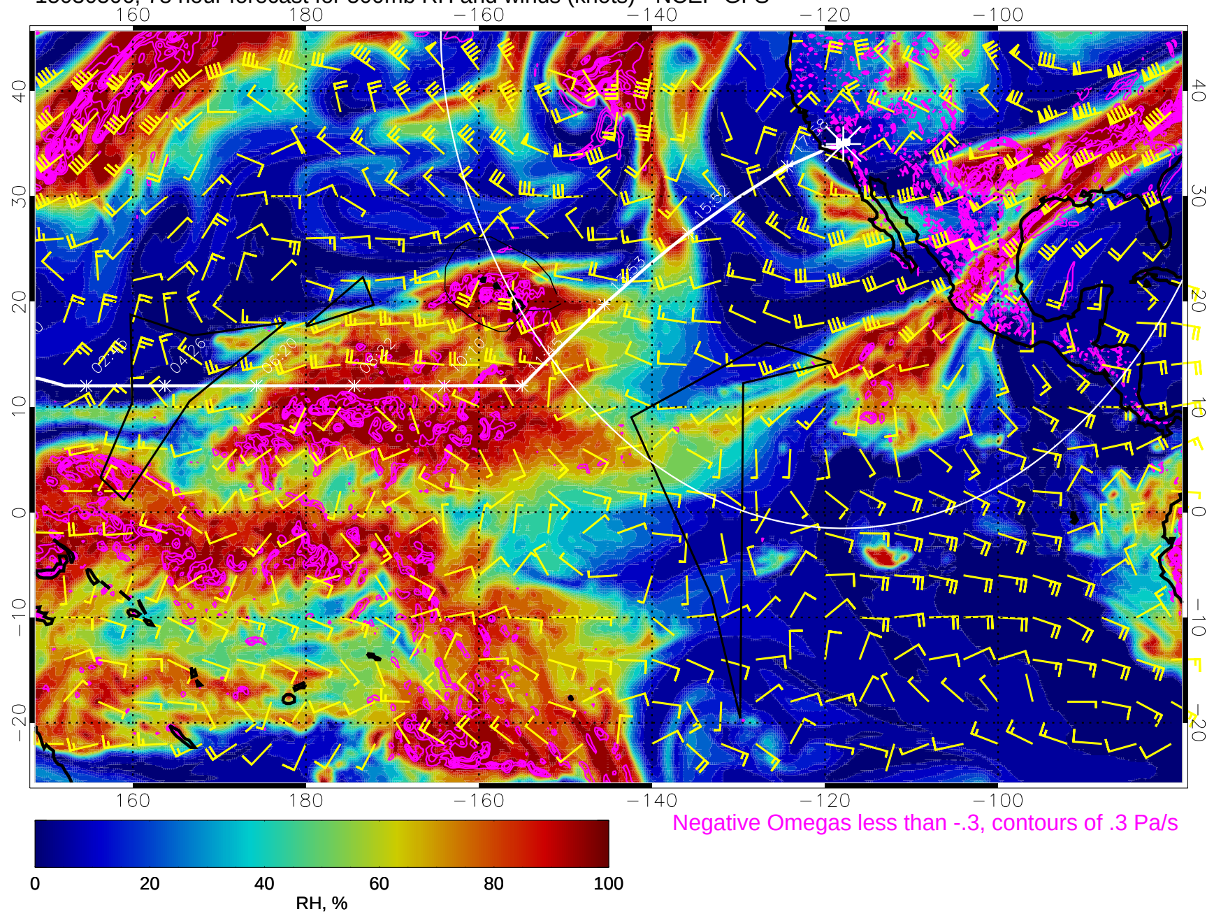
15030506, 78 hour forecast for 500mb RH and winds (knots) - NCEP GFS
