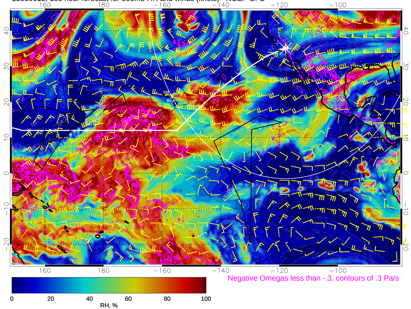
15030612, 108 hour forecast for 500mb RH and winds (knots) - NCEP GFS
