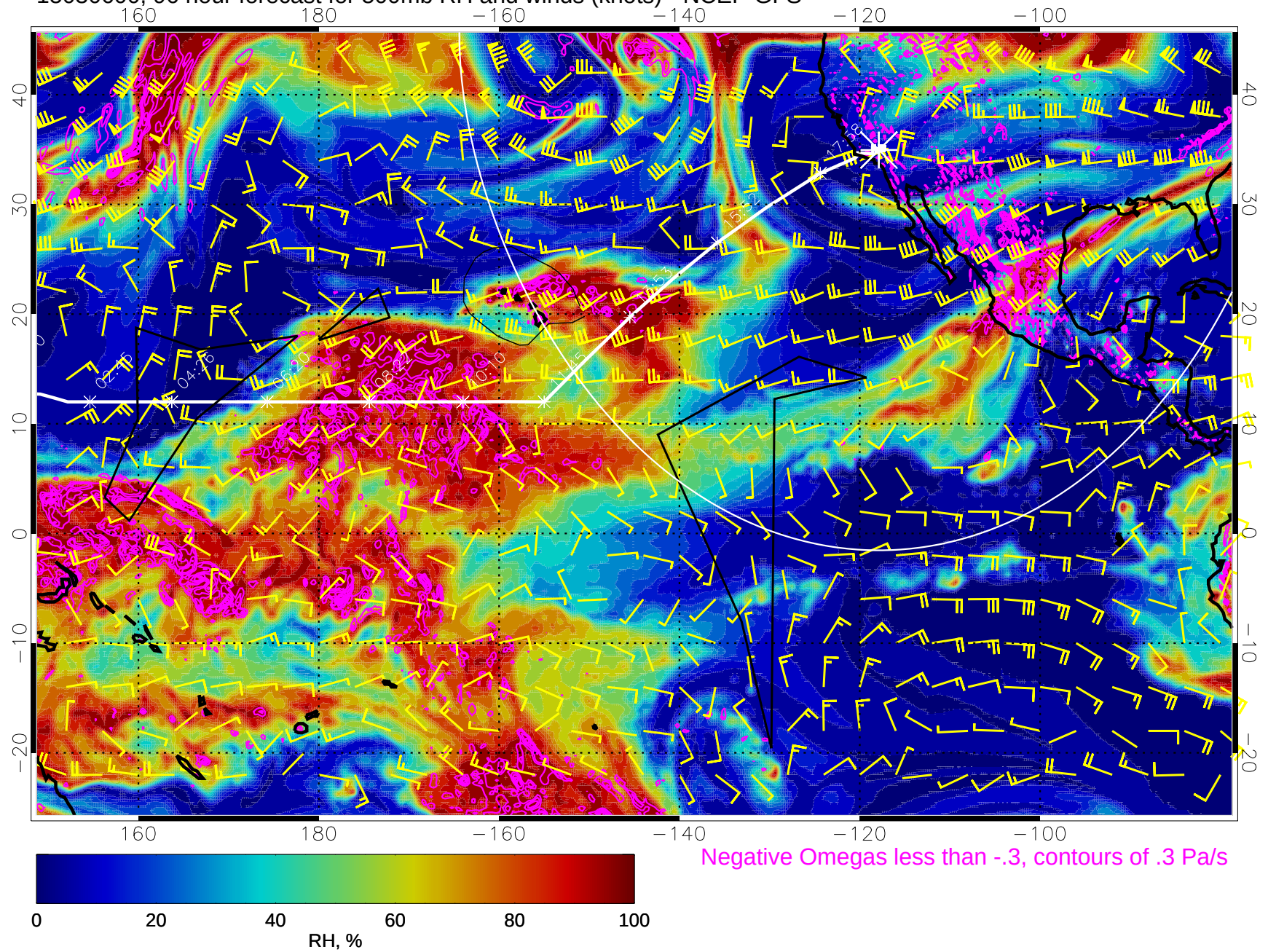
15030600, 96 hour forecast for 500mb RH and winds (knots) - NCEP GFS
