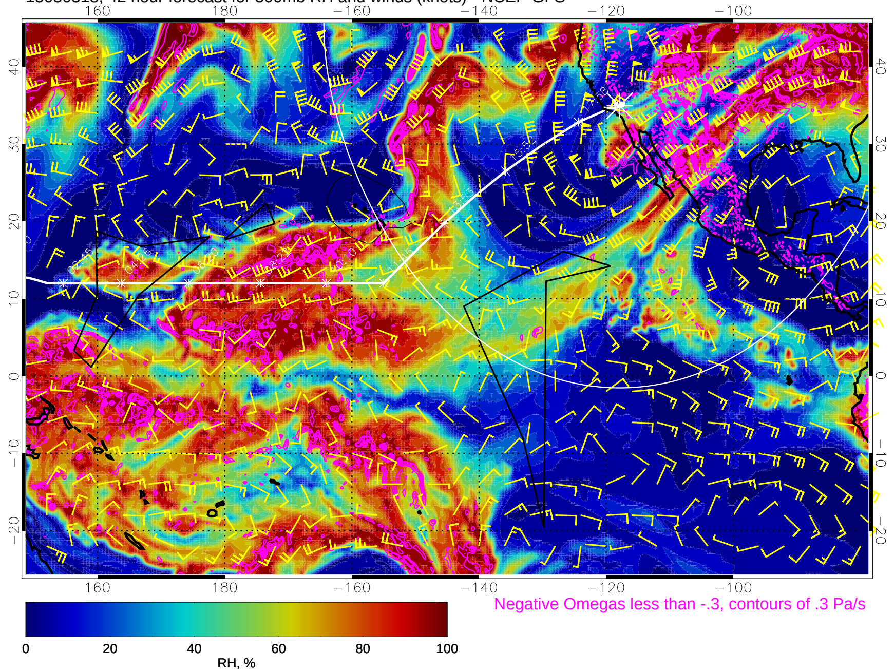
15030318, 42 hour forecast for 500mb RH and winds (knots) - NCEP GFS
