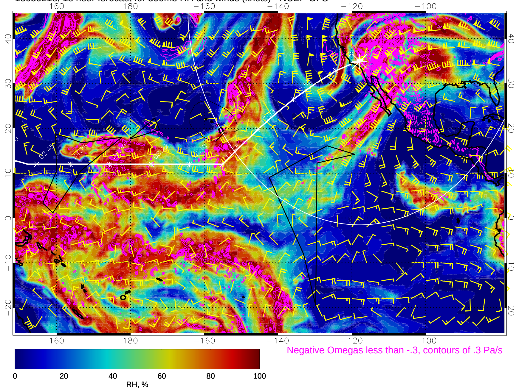
15030218, 18 hour forecast for 500mb RH and winds (knots) - NCEP GFS
