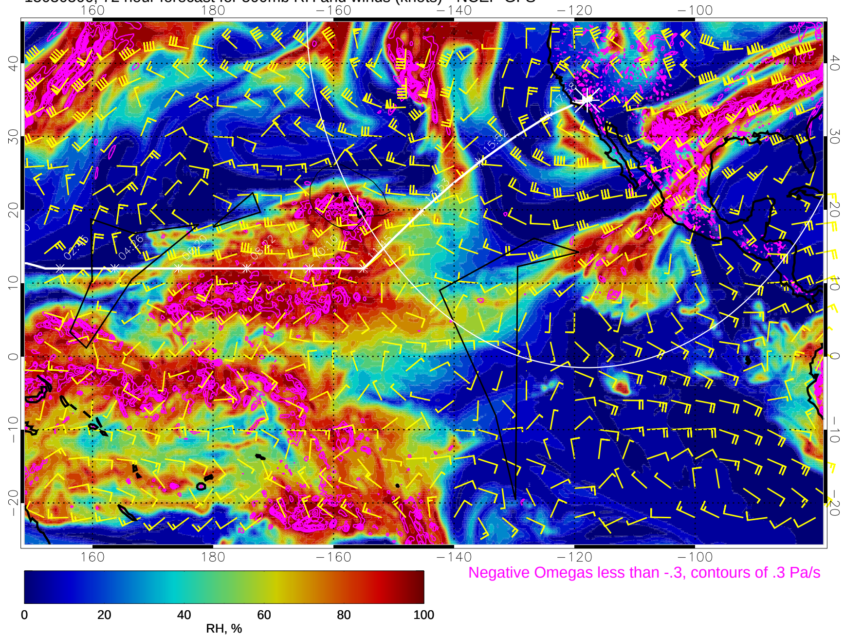
15030500, 72 hour forecast for 500mb RH and winds (knots) - NCEP GFS
