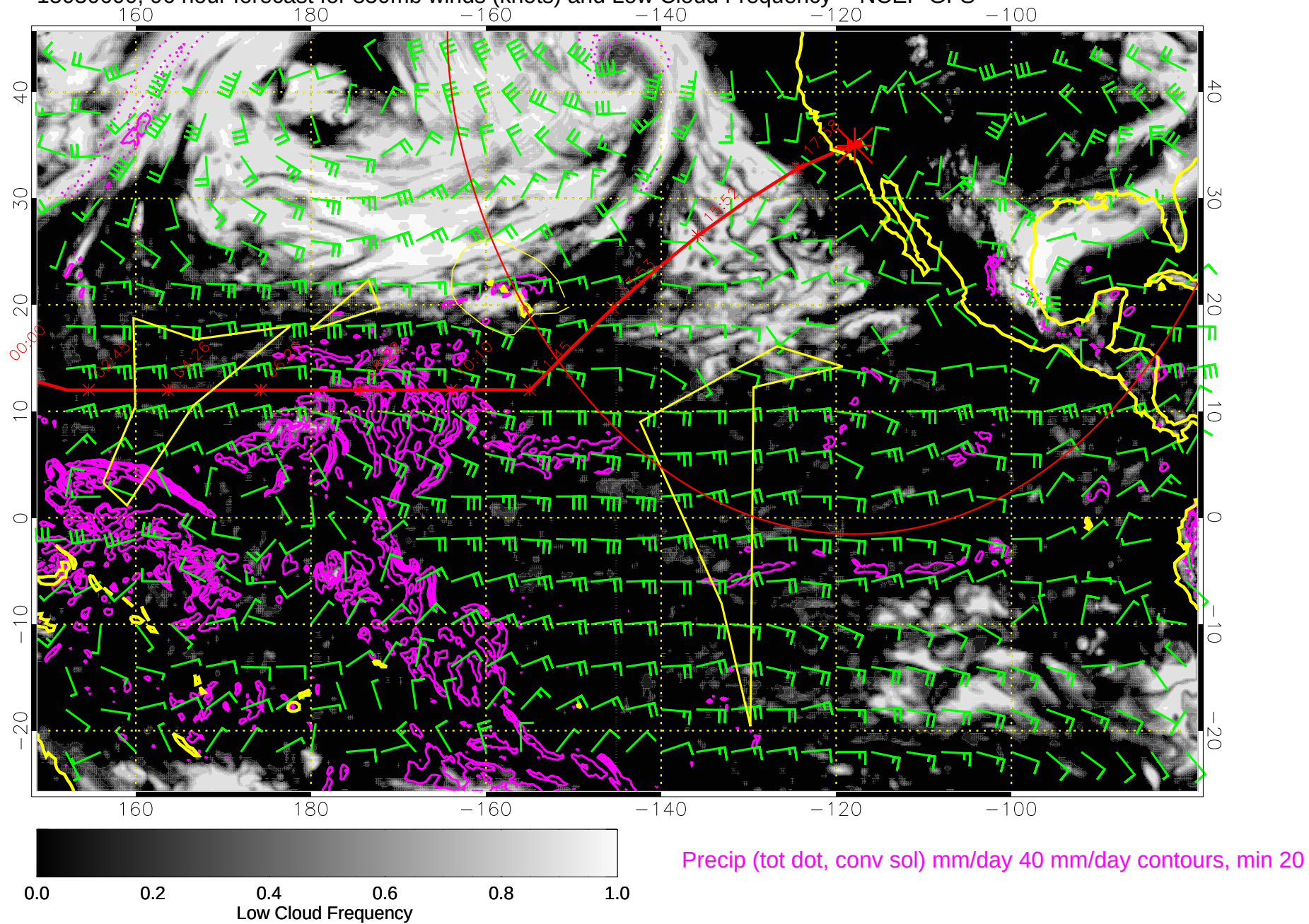
15030600, 96 hour forecast for 850mb winds (knots) and Low Cloud Frequency -- NCEP GFS
