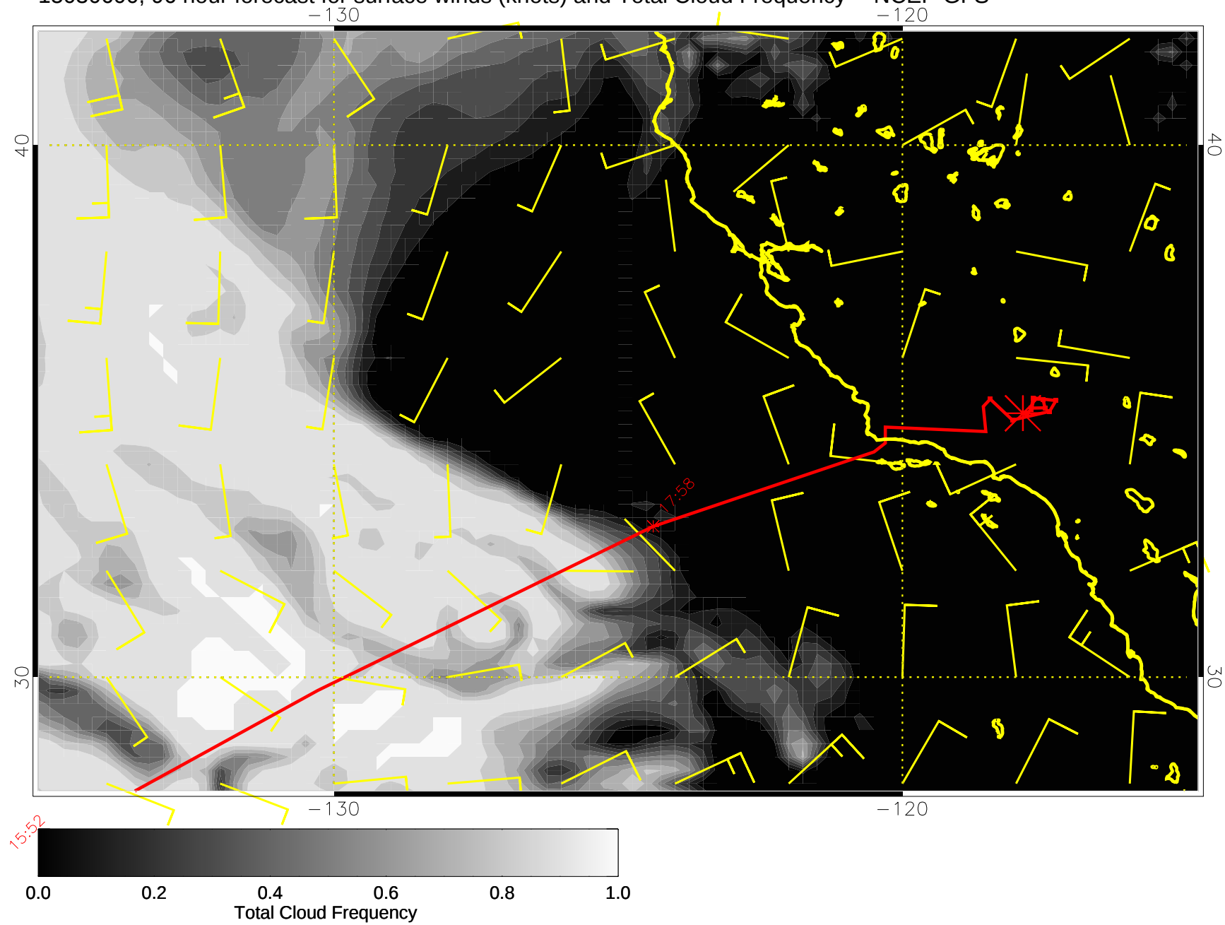
15030600, 96 hour forecast for surface winds (knots) and Total Cloud Frequency -- NCEP GFS
