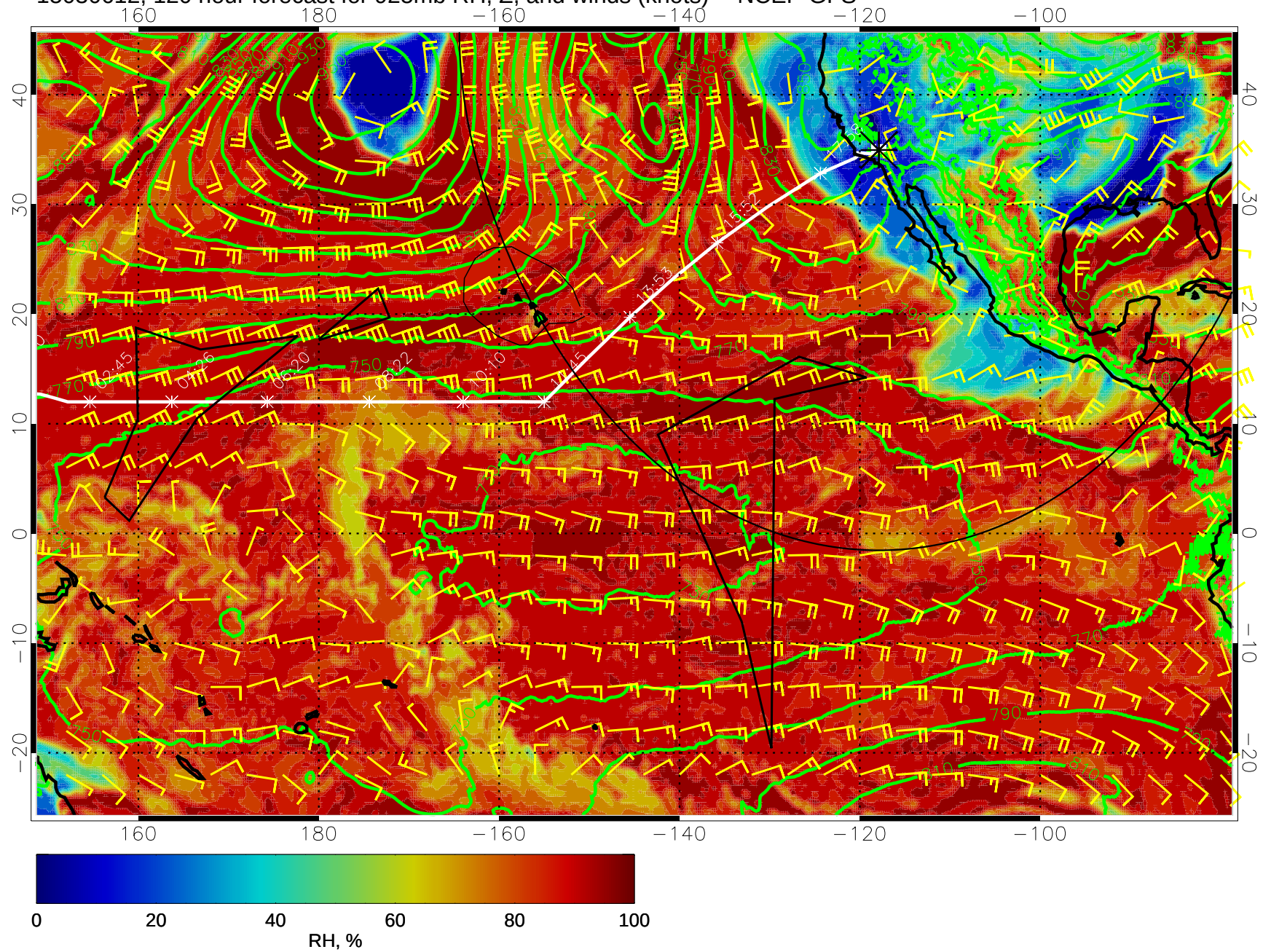
15030612, 120 hour forecast for 925mb RH, Z, and winds (knots) -- NCEP GFS
