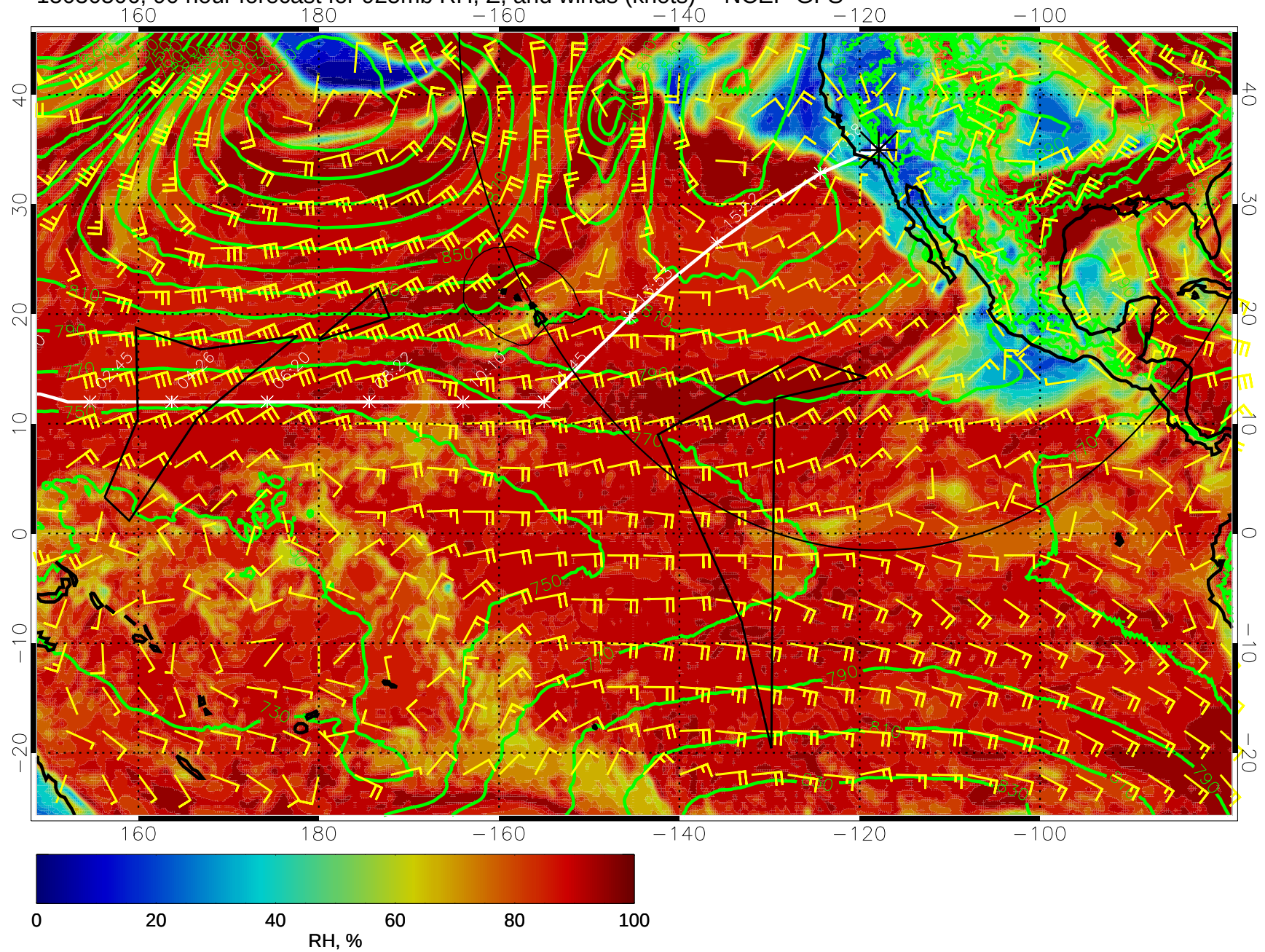
15030506, 90 hour forecast for 925mb RH, Z, and winds (knots) -- NCEP GFS
