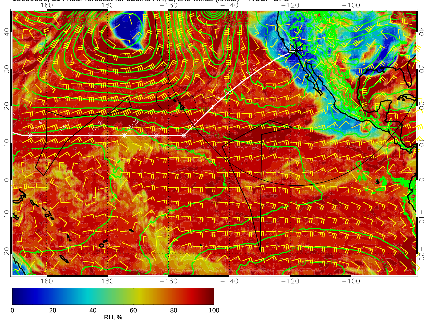
15030606, 114 hour forecast for 925mb RH, Z, and winds (knots) -- NCEP GFS
