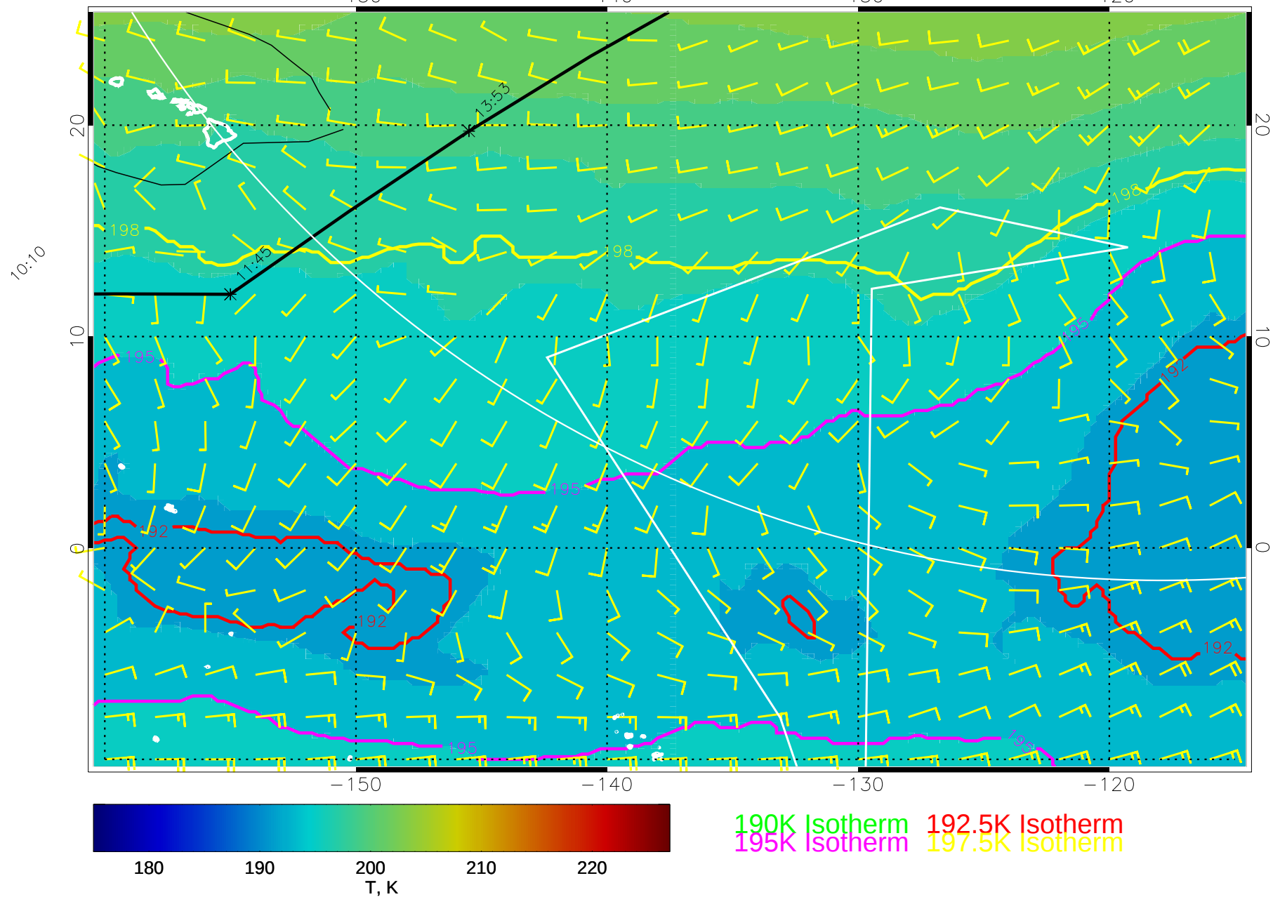
15030506, 90 hour forecast for 70mb T and winds (knots) -- NCEP GFS
