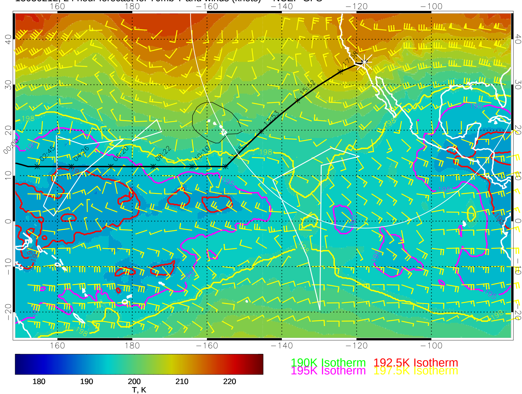
15030212, 24 hour forecast for 70mb T and winds (knots) -- NCEP GFS
