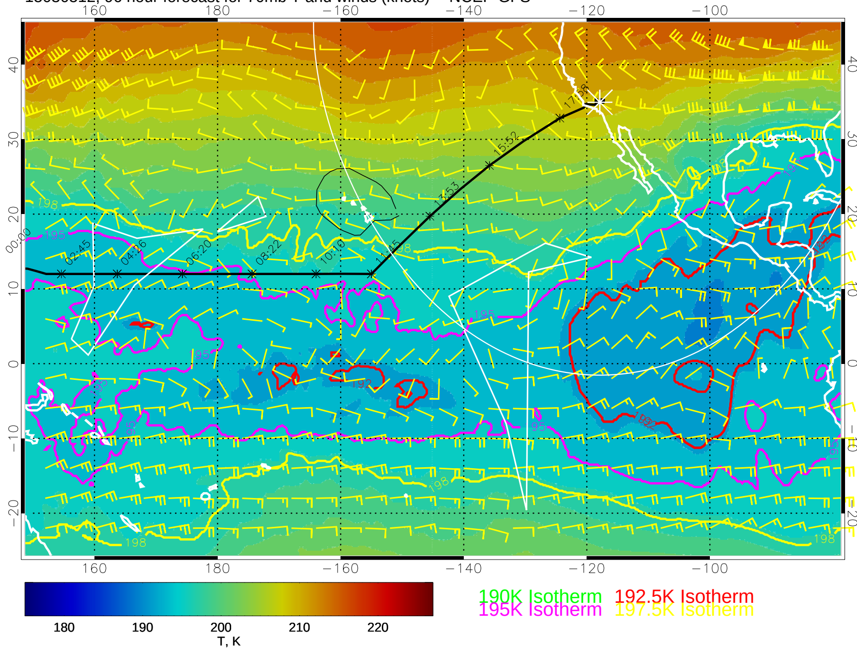
15030512, 96 hour forecast for 70mb T and winds (knots) -- NCEP GFS
