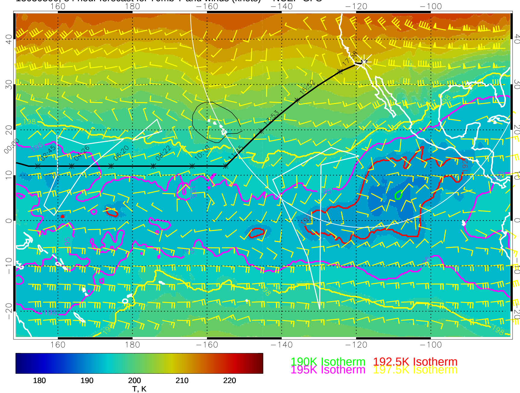
15030500, 84 hour forecast for 70mb T and winds (knots) -- NCEP GFS
