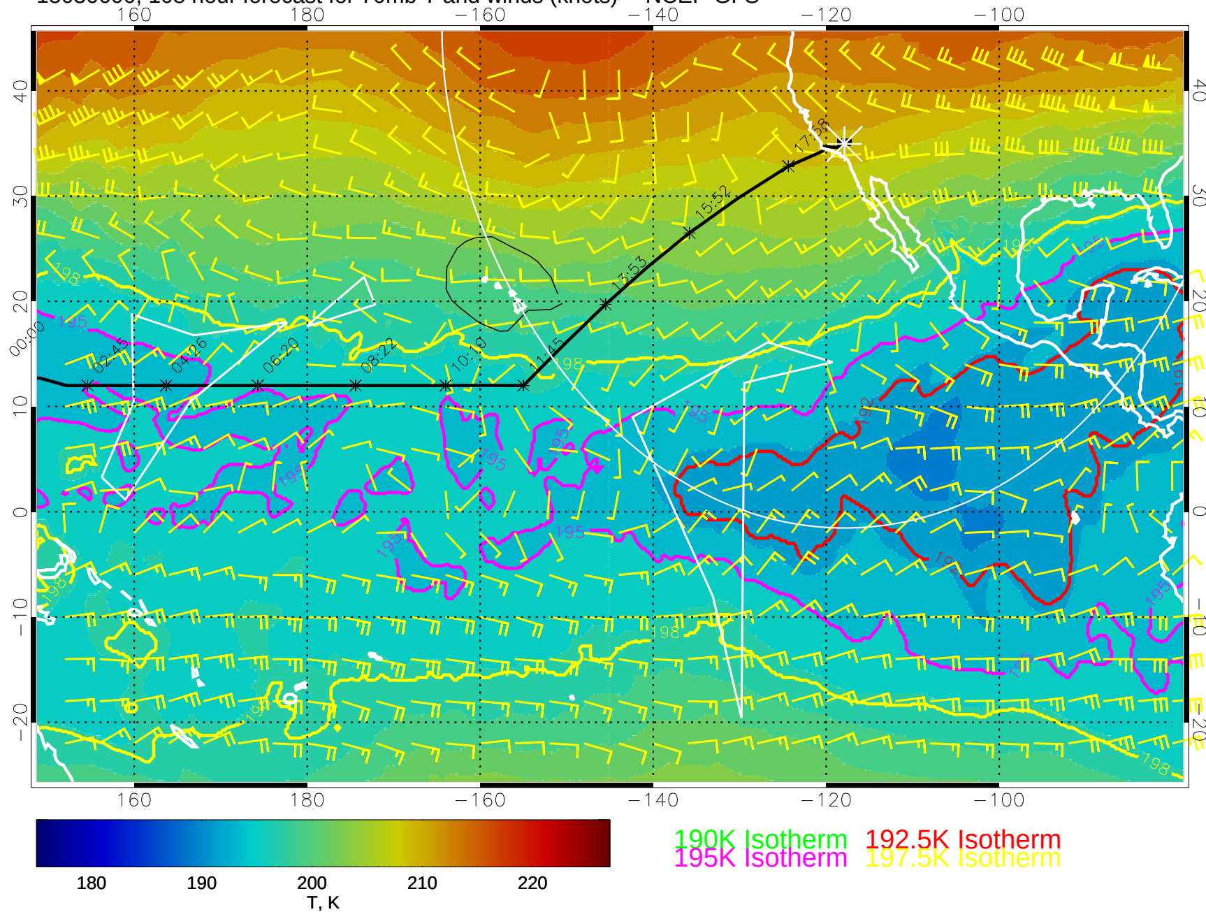
15030600, 108 hour forecast for 70mb T and winds (knots) -- NCEP GFS
