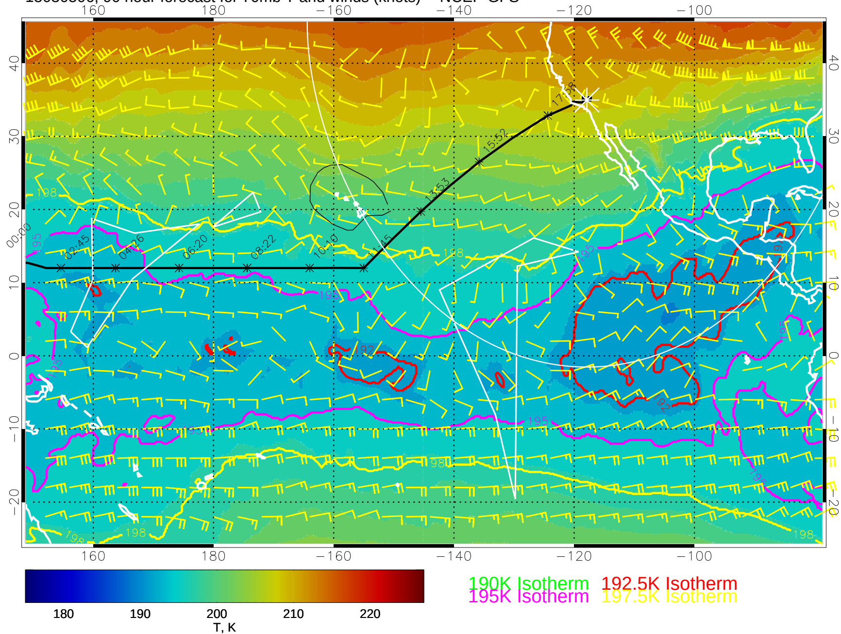
15030506, 90 hour forecast for 70mb T and winds (knots) -- NCEP GFS
