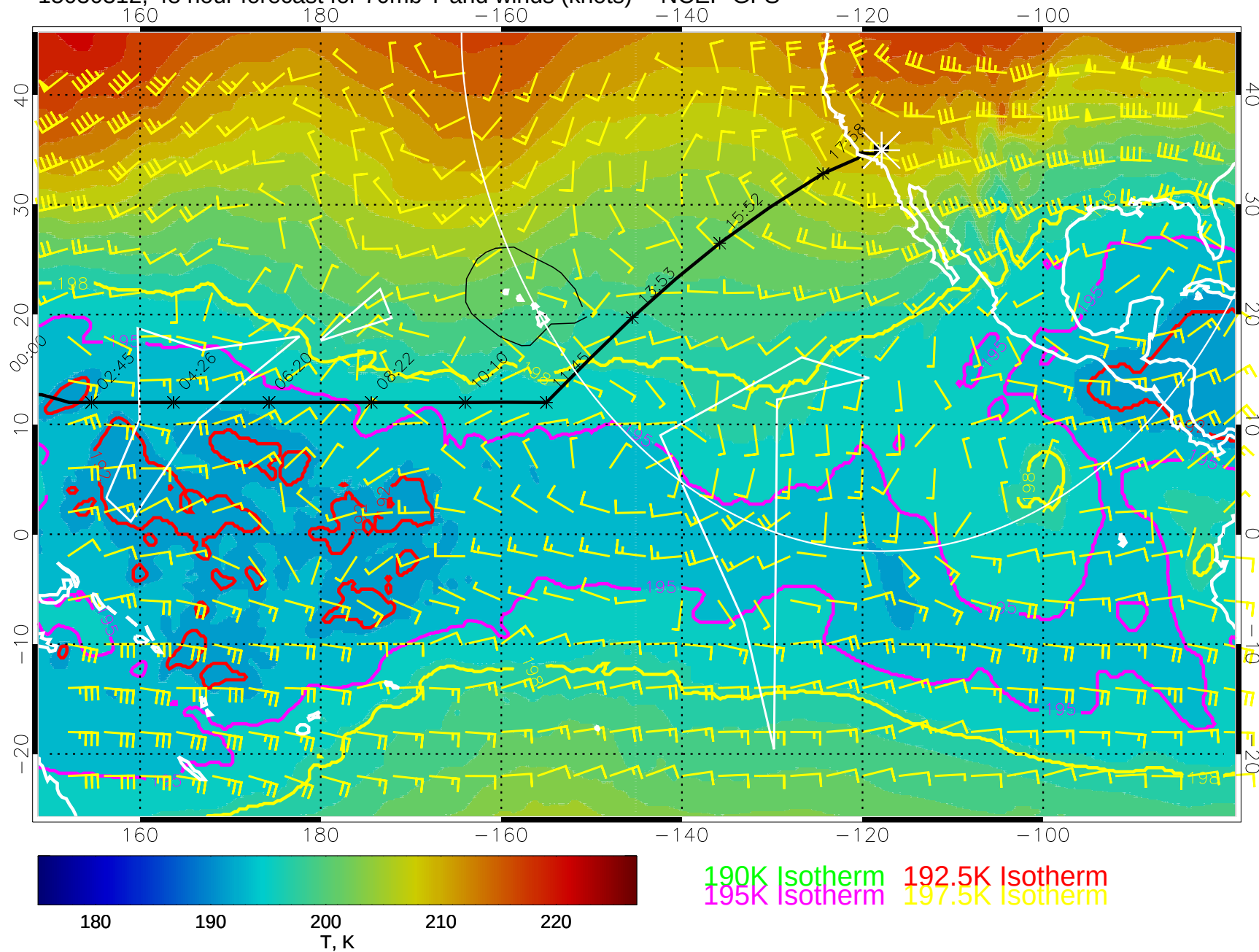
15030312, 48 hour forecast for 70mb T and winds (knots) -- NCEP GFS
