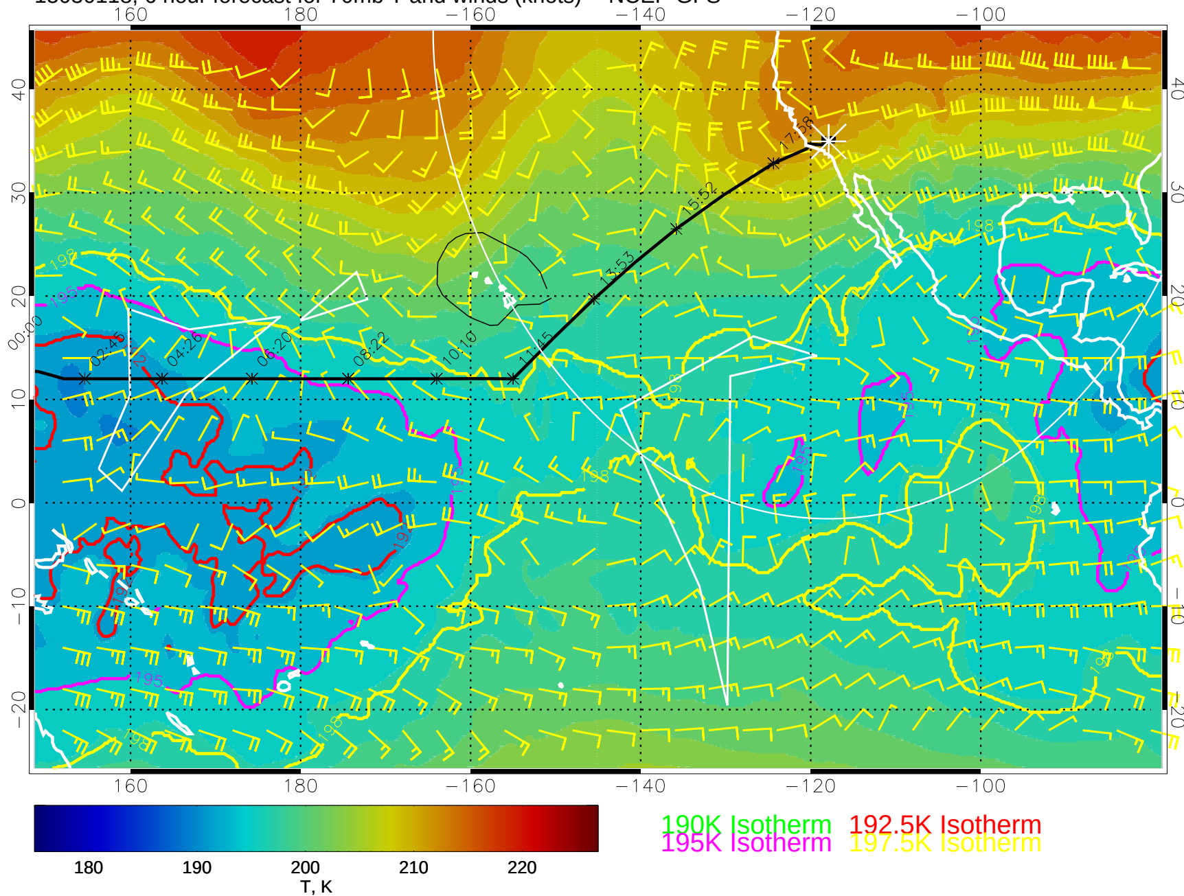
15030118, 6 hour forecast for 70mb T and winds (knots) -- NCEP GFS
