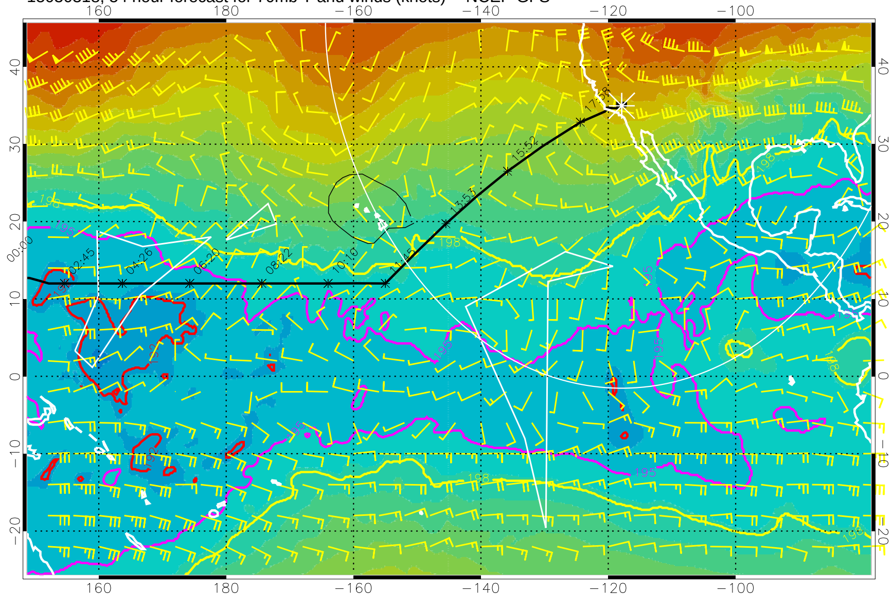
15030318, 54 hour forecast for 70mb T and winds (knots) -- NCEP GFS
