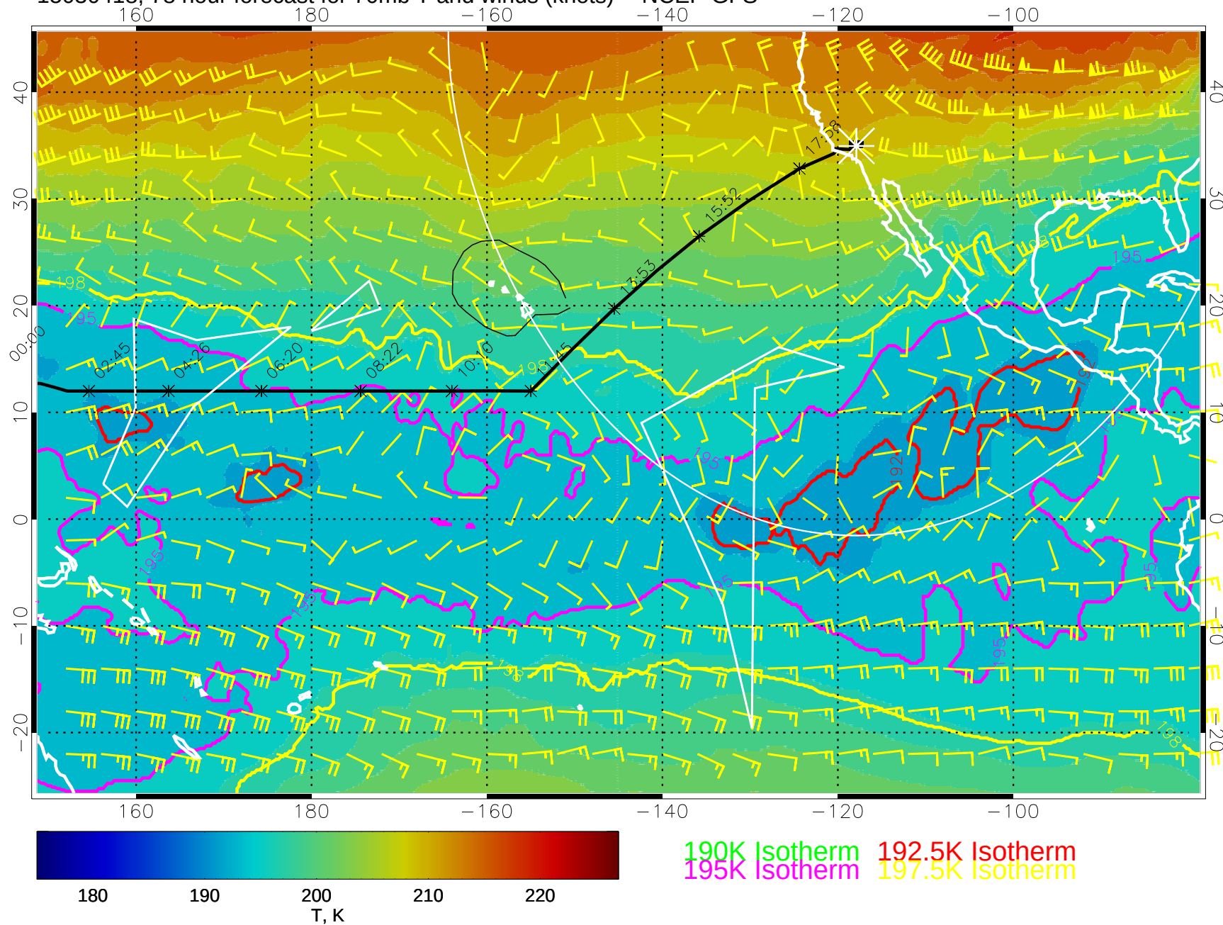
15030418, 78 hour forecast for 70mb T and winds (knots) -- NCEP GFS
