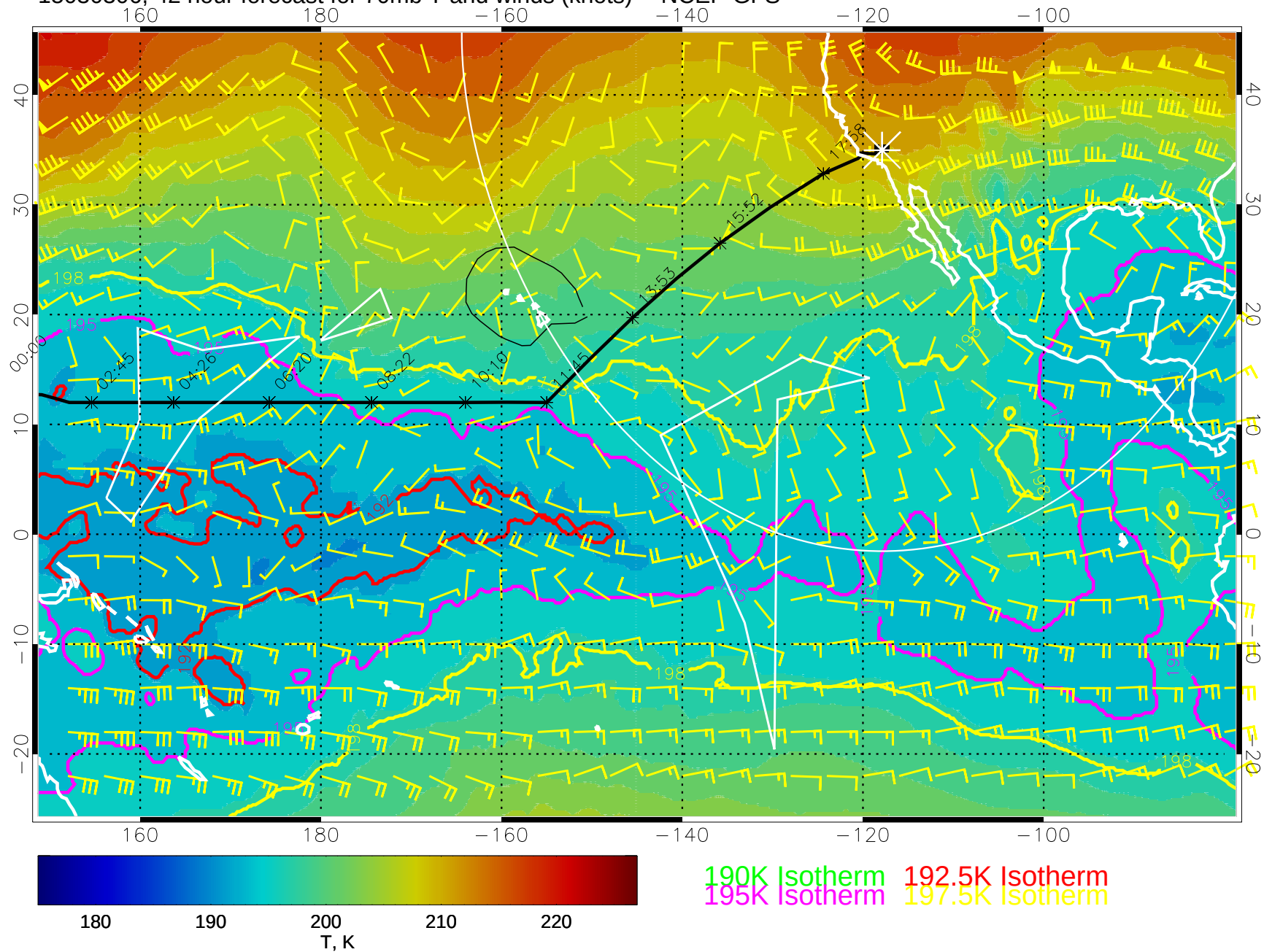
15030306, 42 hour forecast for 70mb T and winds (knots) -- NCEP GFS
