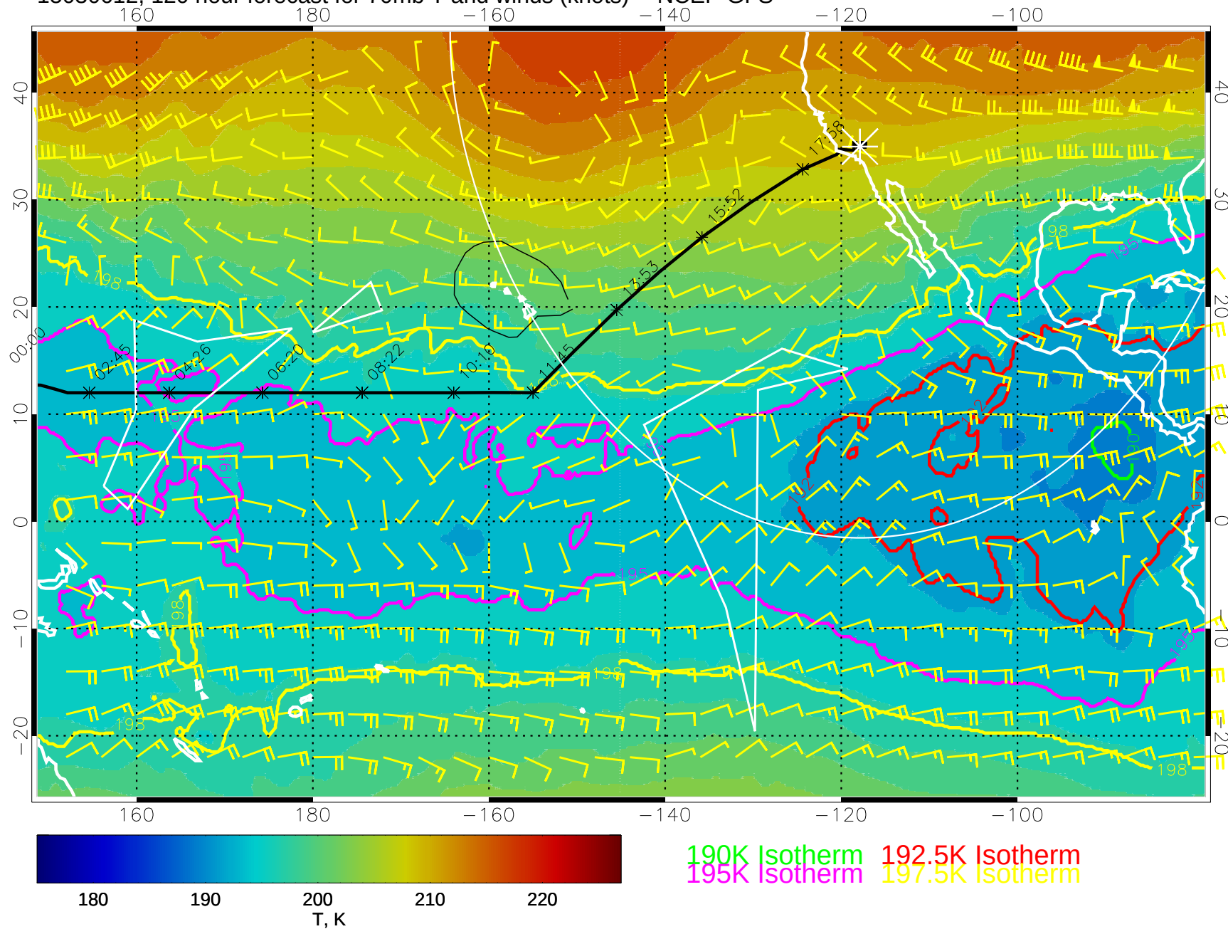
15030612, 120 hour forecast for 70mb T and winds (knots) -- NCEP GFS
