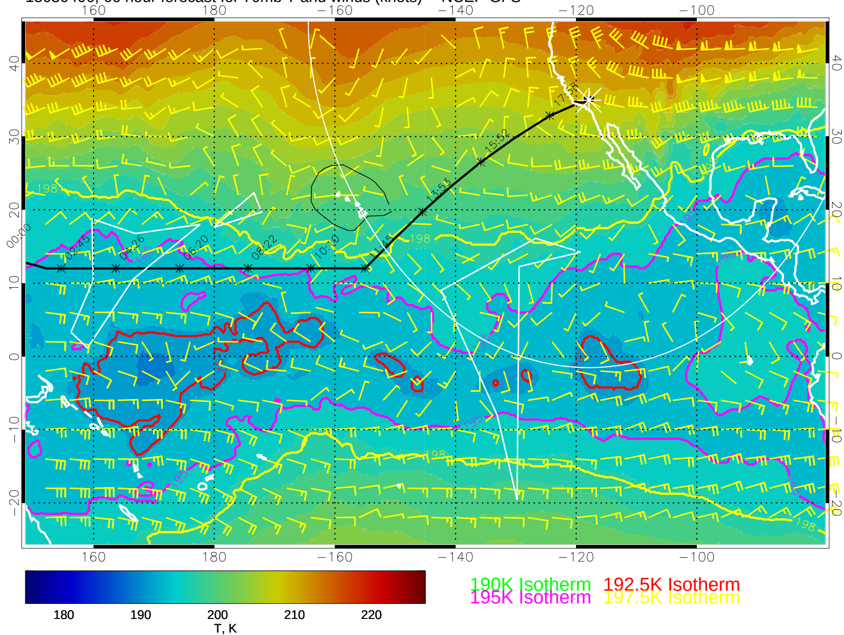
15030406, 66 hour forecast for 70mb T and winds (knots) -- NCEP GFS
