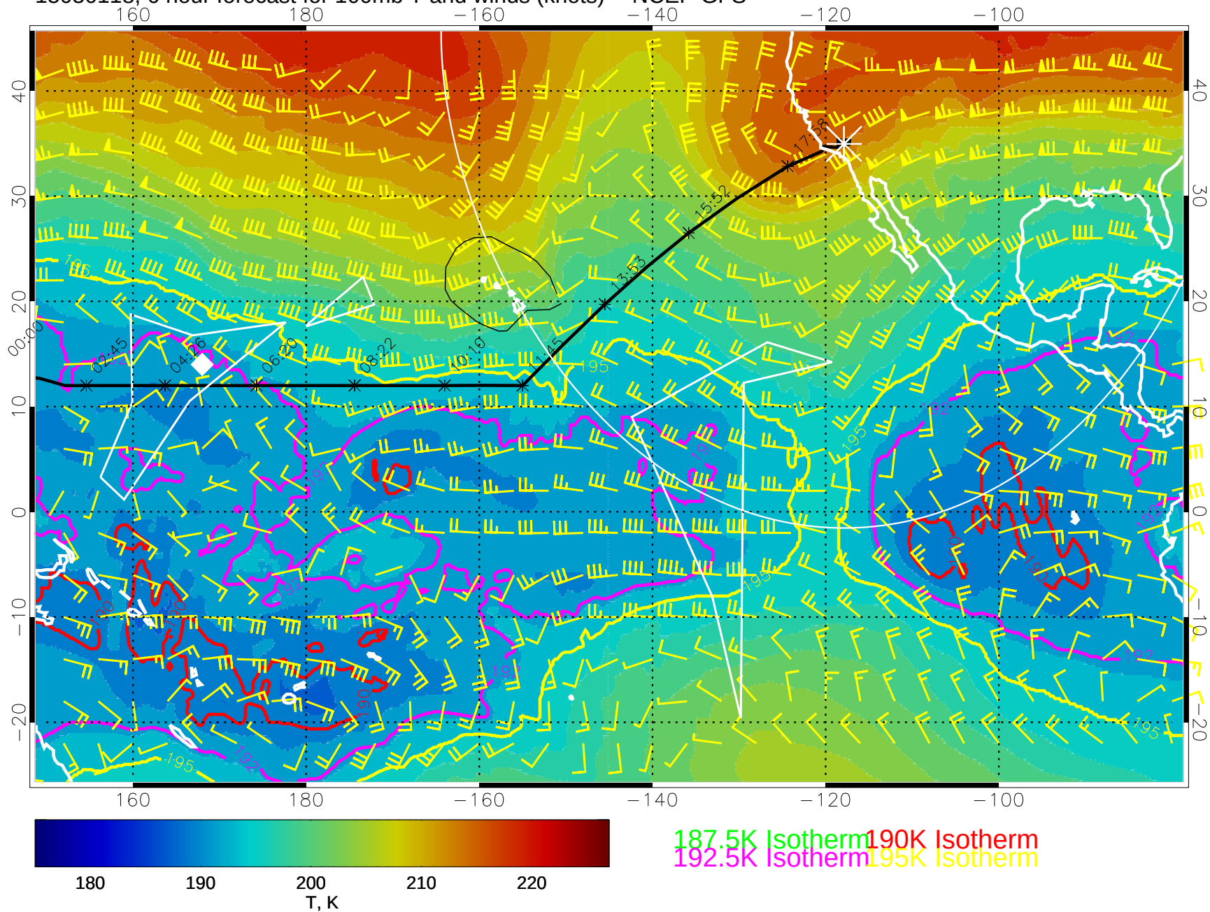
15030118, 6 hour forecast for 100mb T and winds (knots) -- NCEP GFS
