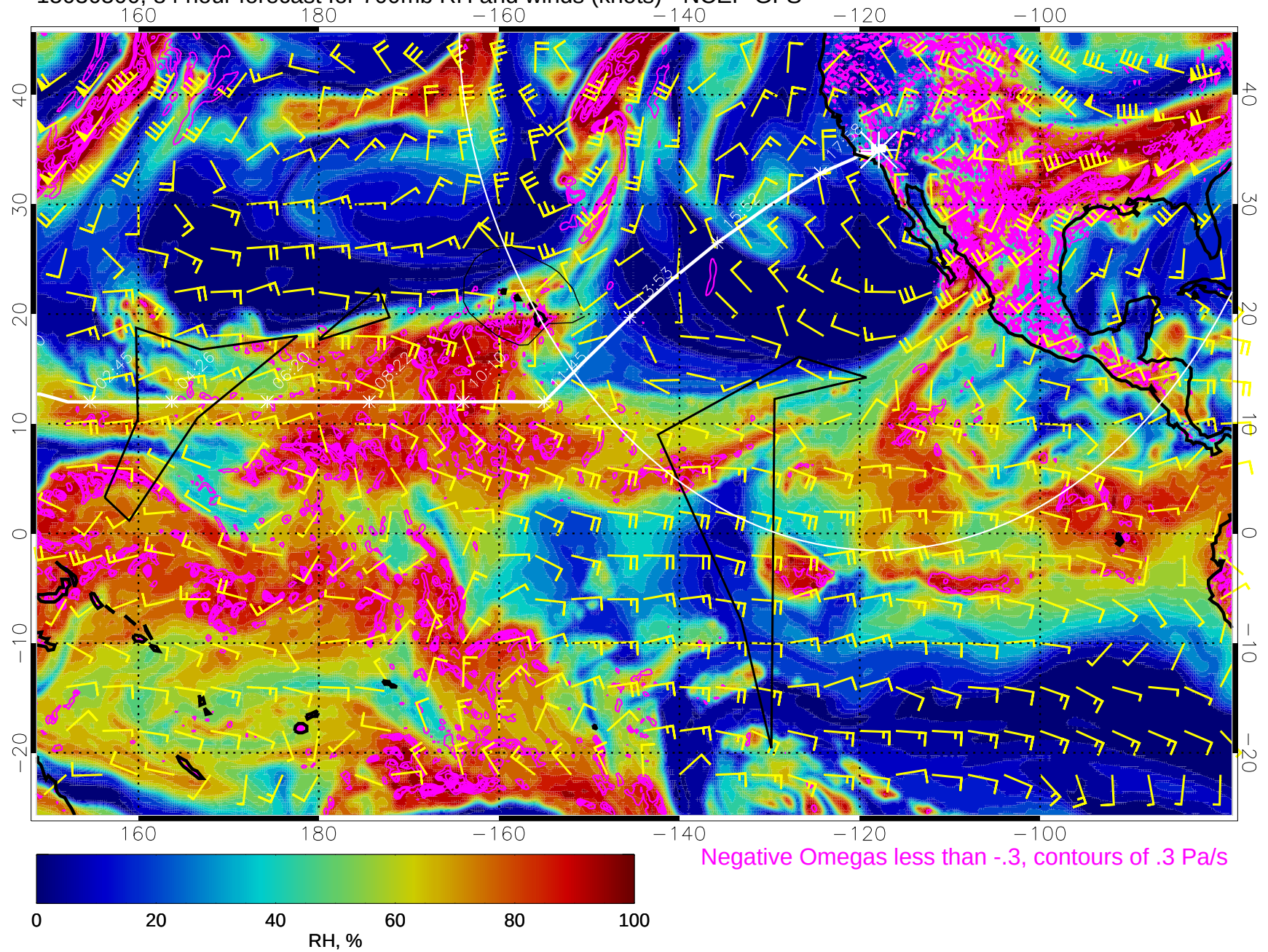
15030500, 84 hour forecast for 700mb RH and winds (knots) - NCEP GFS
