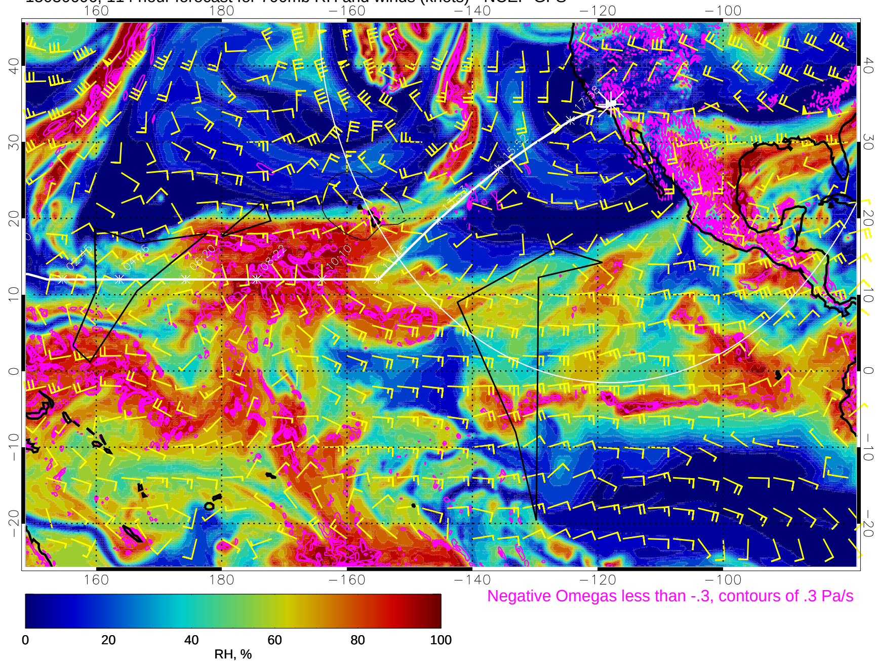
15030606, 114 hour forecast for 700mb RH and winds (knots) - NCEP GFS
