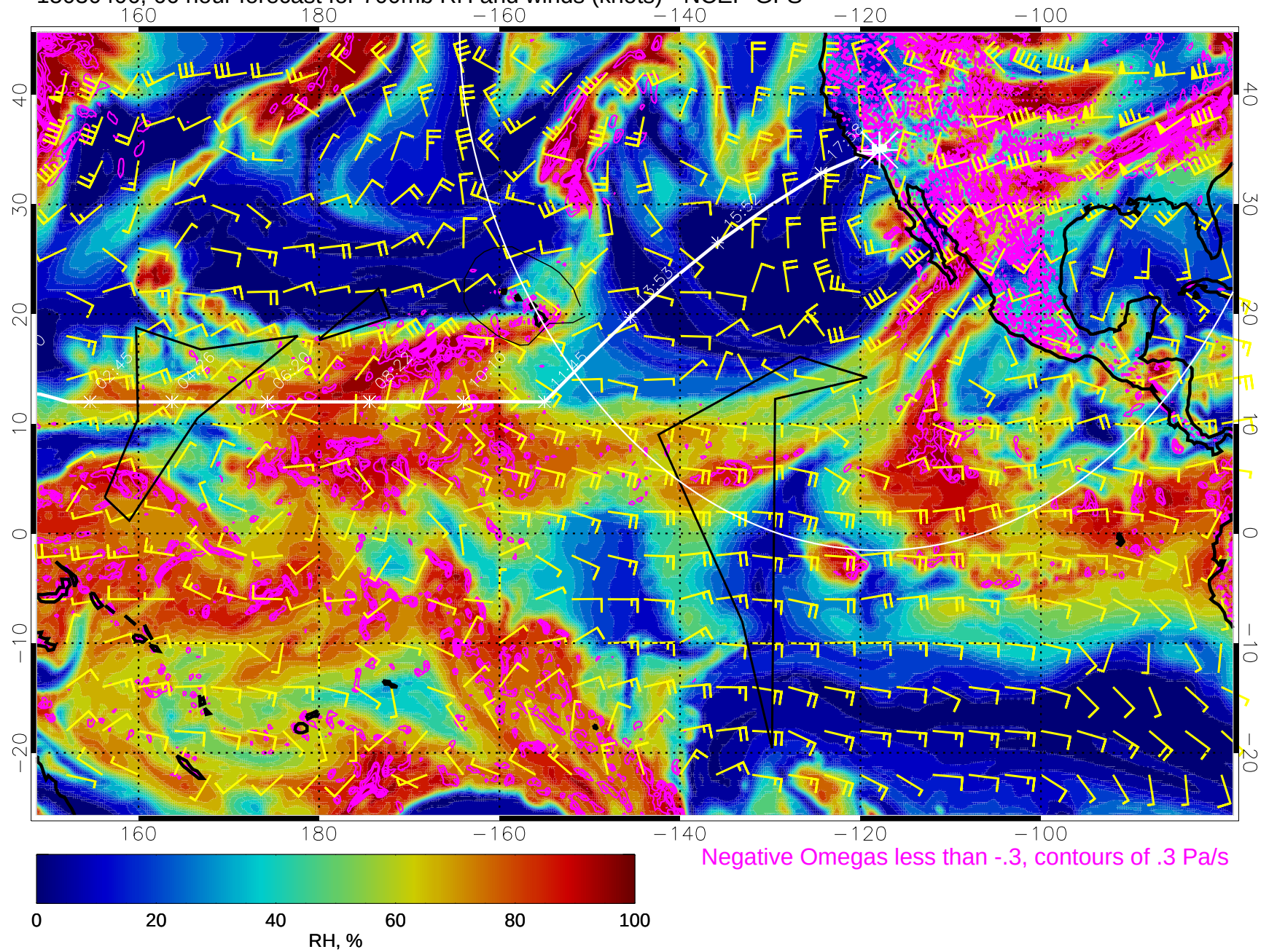
15030406, 66 hour forecast for 700mb RH and winds (knots) - NCEP GFS
