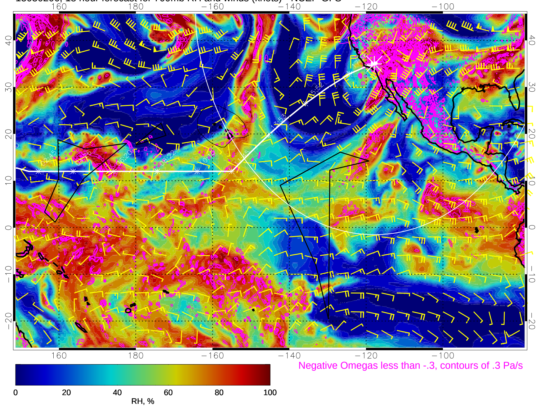
15030206, 18 hour forecast for 700mb RH and winds (knots) - NCEP GFS
