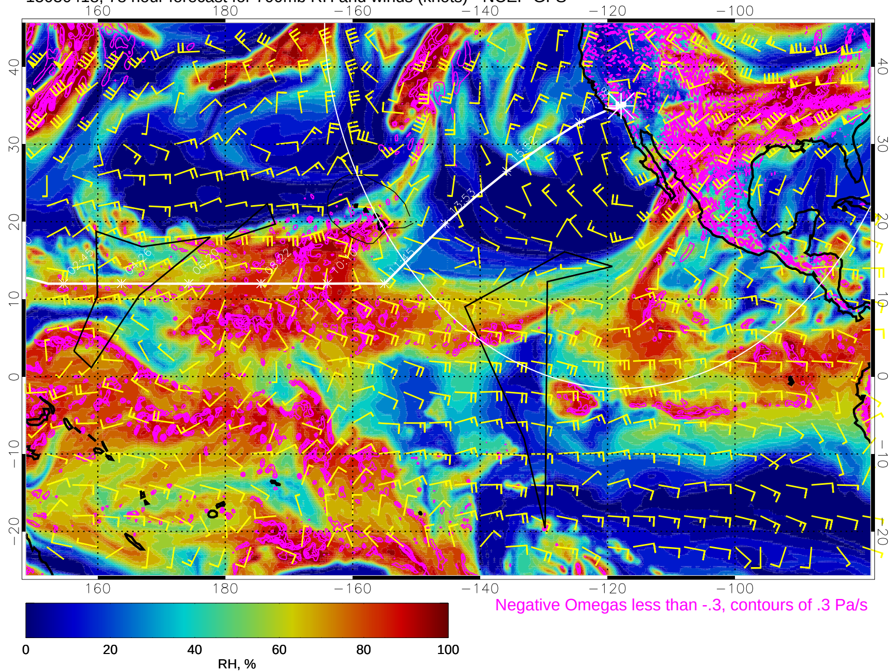
15030418, 78 hour forecast for 700mb RH and winds (knots) - NCEP GFS
