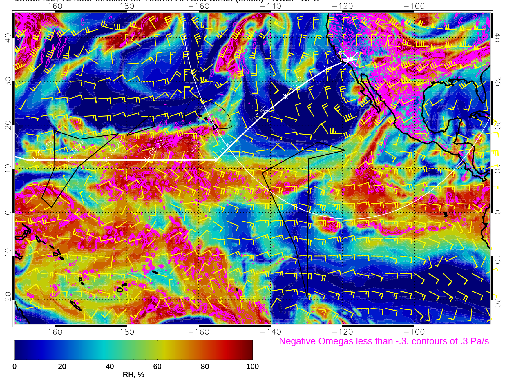
15030412, 72 hour forecast for 700mb RH and winds (knots) - NCEP GFS
