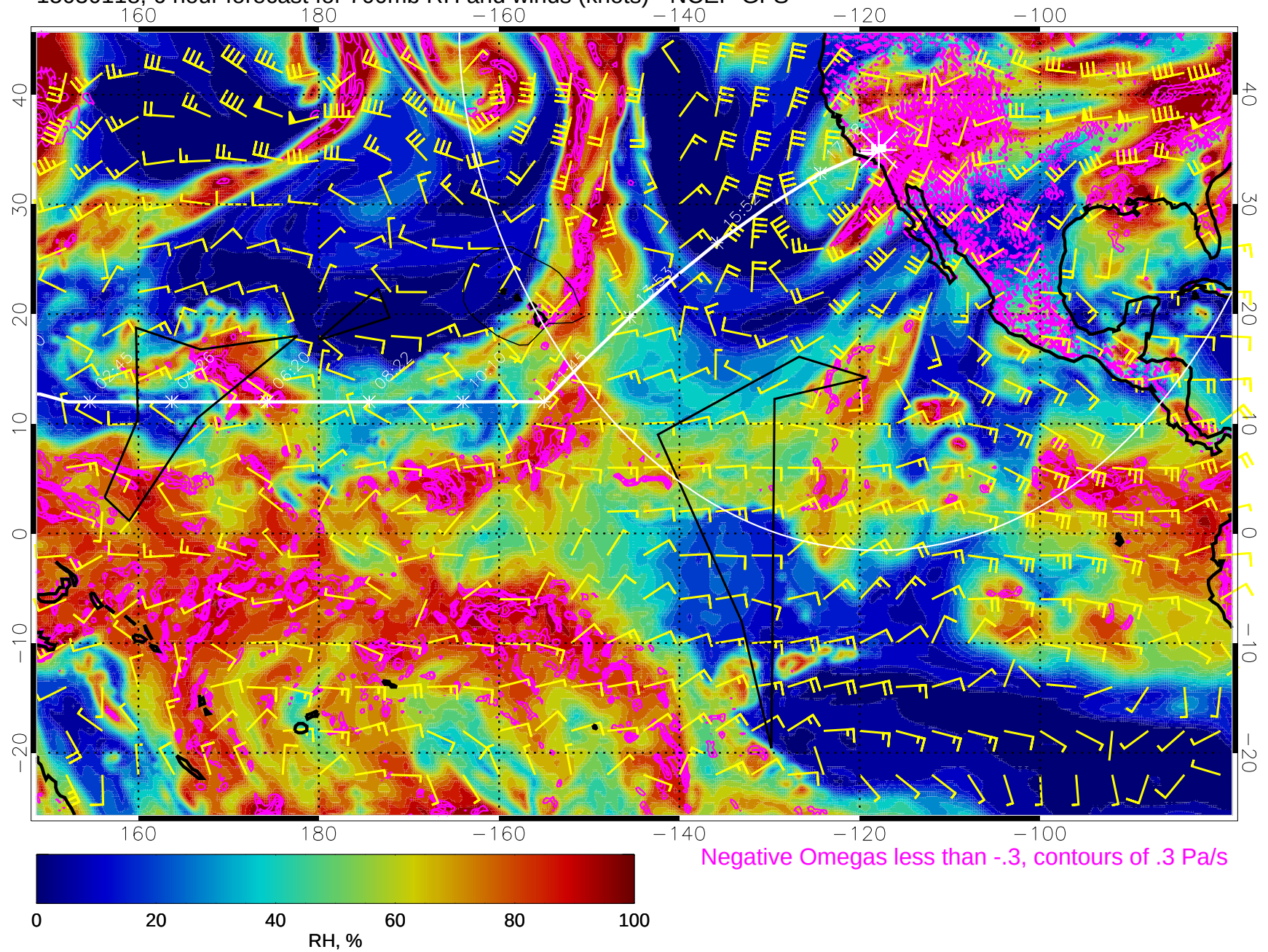
15030118, 6 hour forecast for 700mb RH and winds (knots) - NCEP GFS
