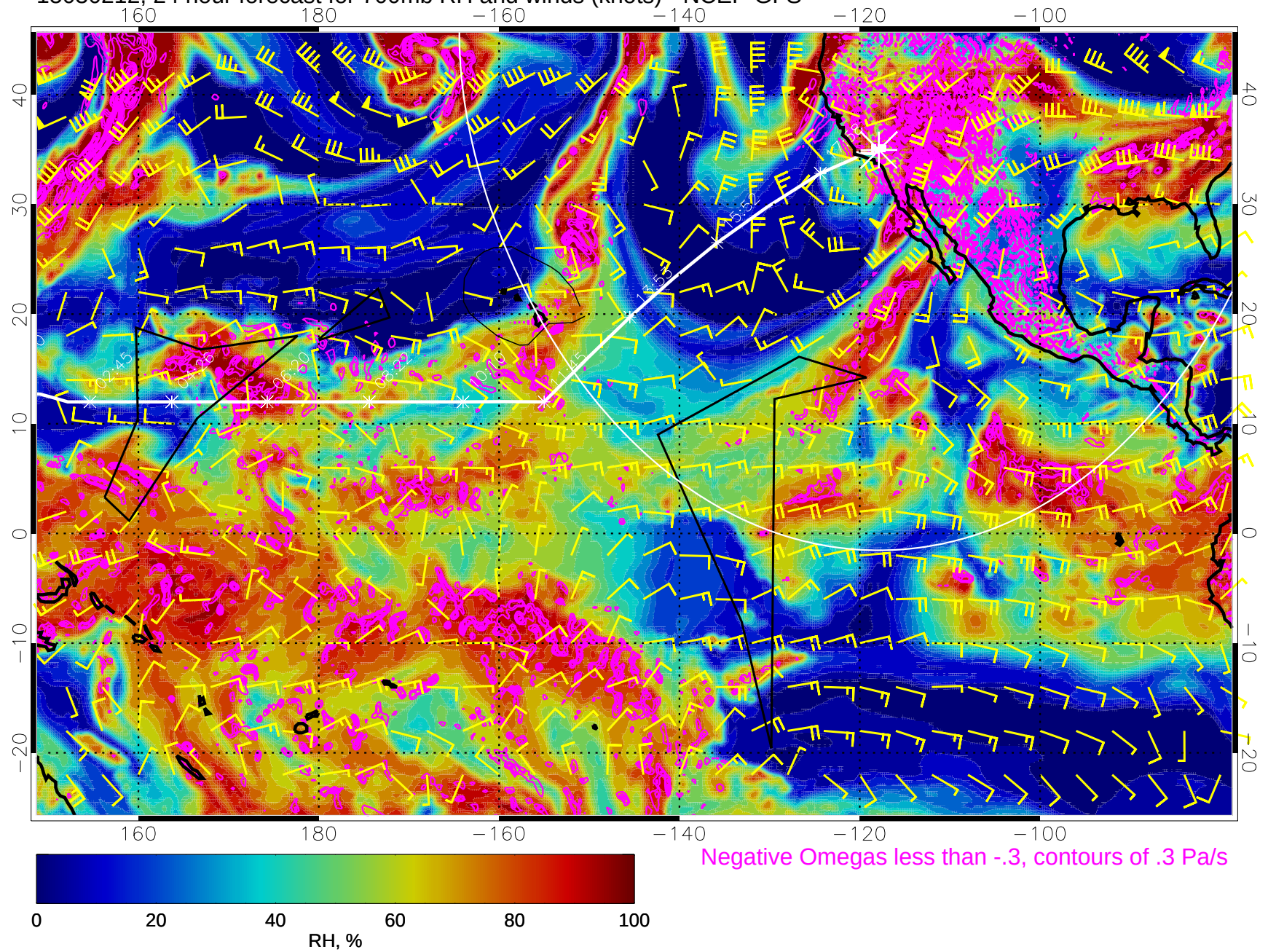
15030212, 24 hour forecast for 700mb RH and winds (knots) - NCEP GFS
