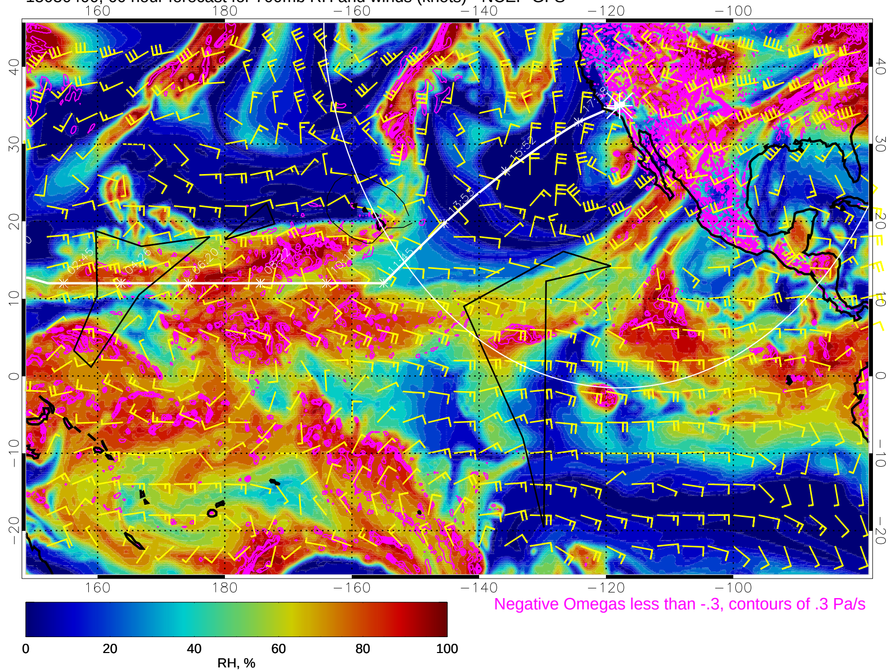
15030400, 60 hour forecast for 700mb RH and winds (knots) - NCEP GFS
