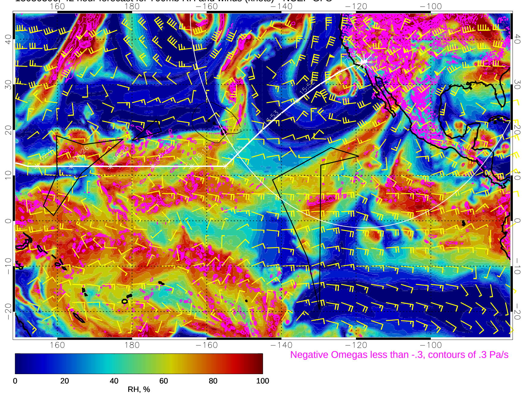
15030306, 42 hour forecast for 700mb RH and winds (knots) - NCEP GFS
