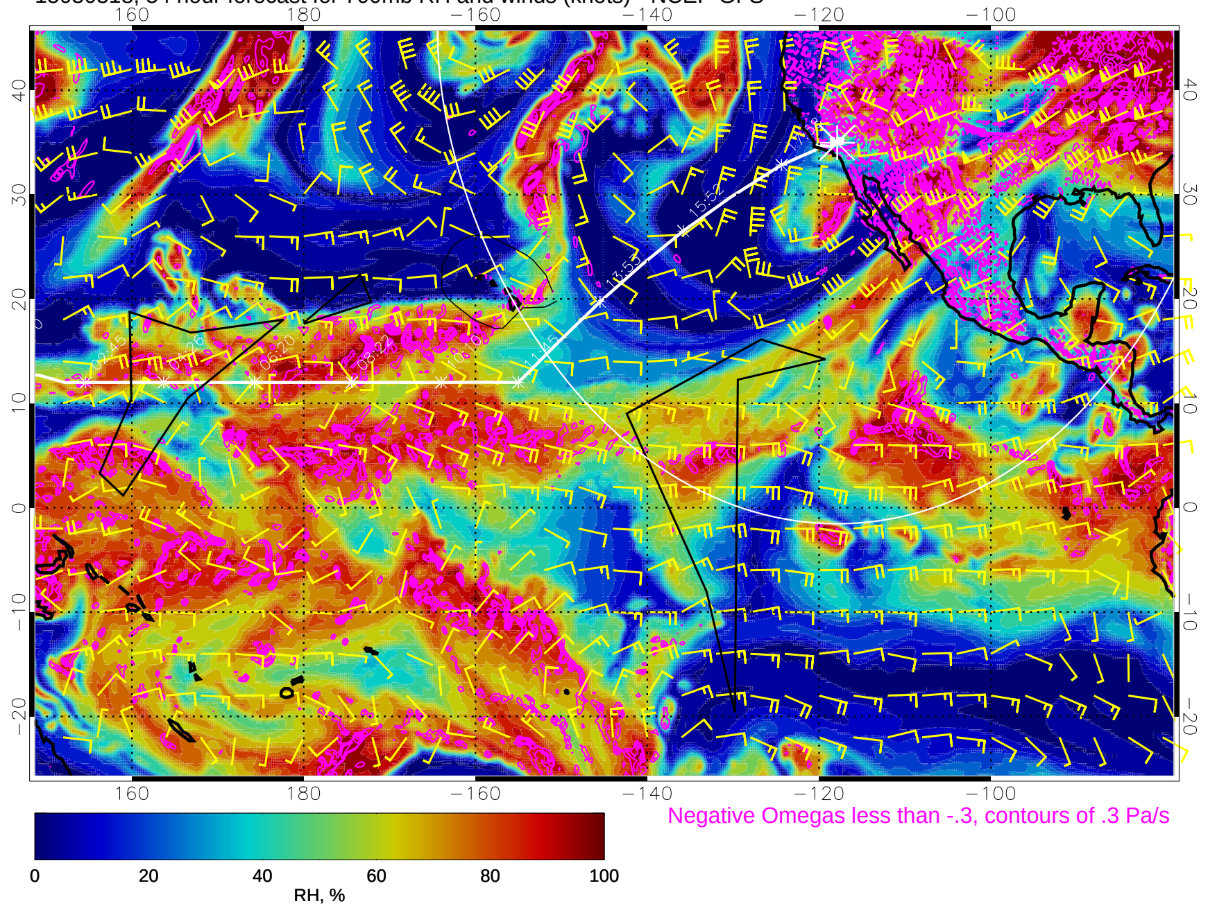
15030318, 54 hour forecast for 700mb RH and winds (knots) - NCEP GFS
