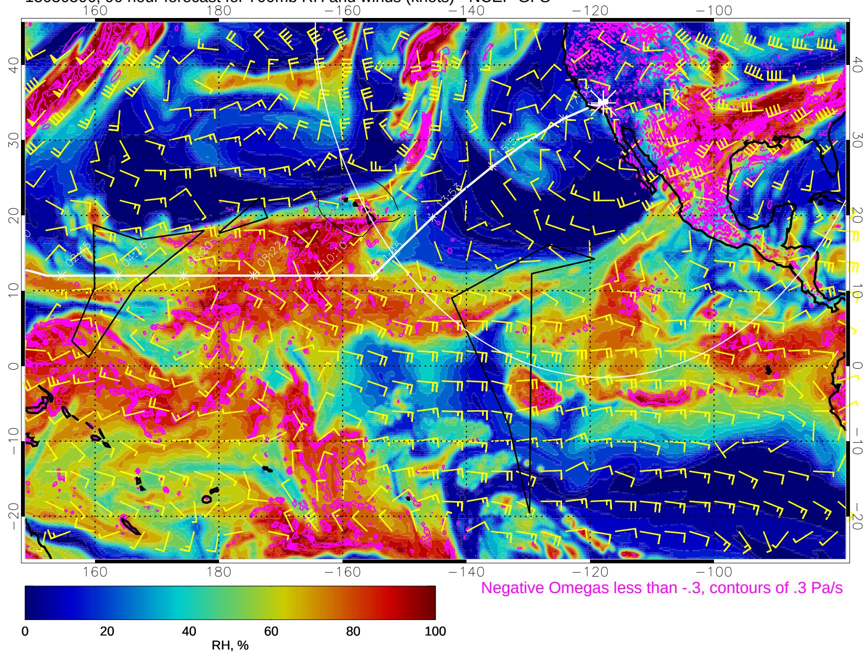
15030506, 90 hour forecast for 700mb RH and winds (knots) - NCEP GFS
