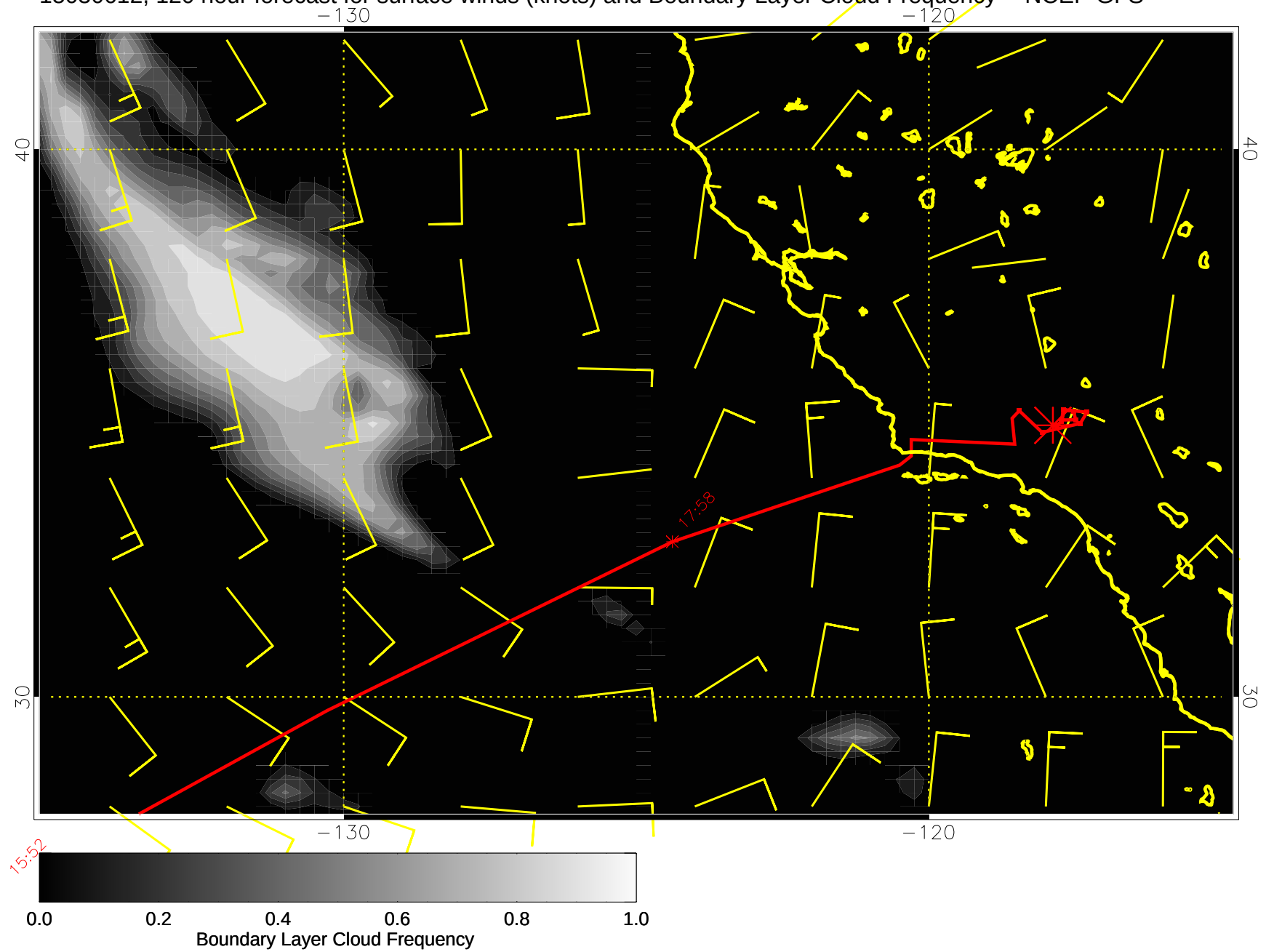
15030612, 120 hour forecast for surface winds (knots) and Boundary Layer Cloud Frequency -- NCEP GFS
