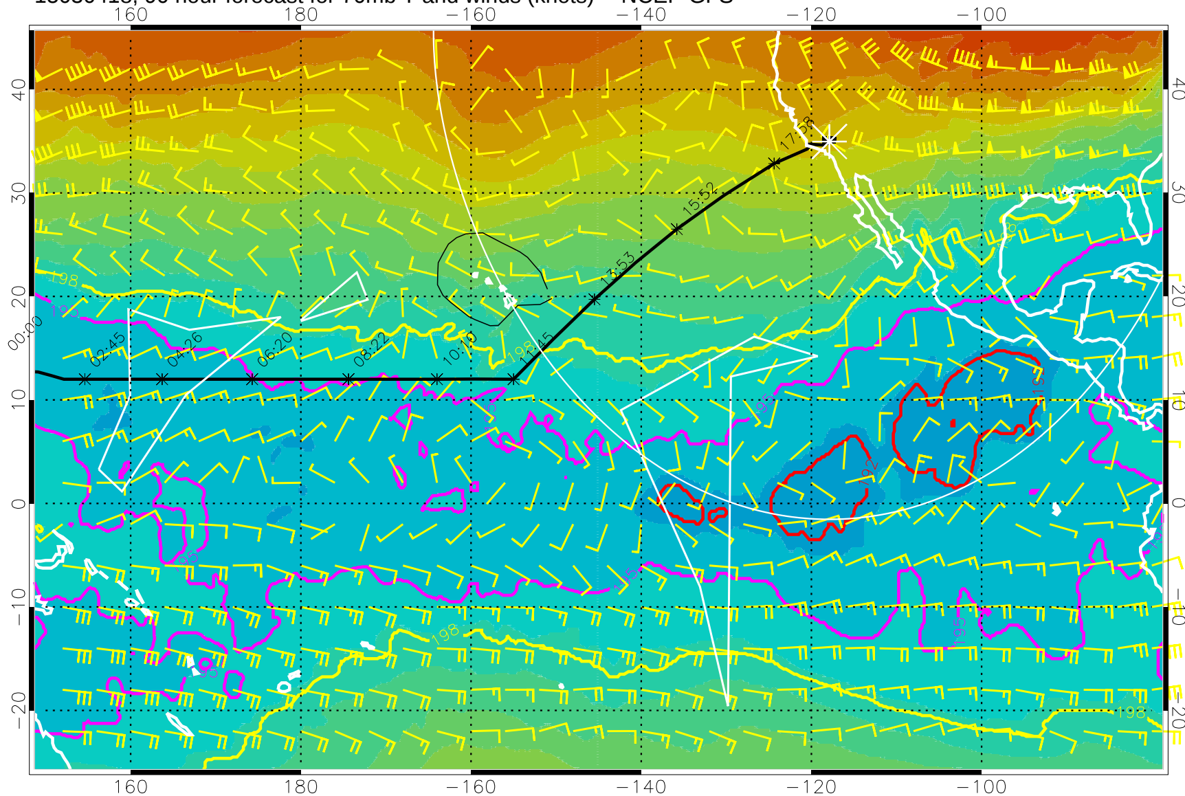
15030418, 90 hour forecast for 70mb T and winds (knots) -- NCEP GFS
