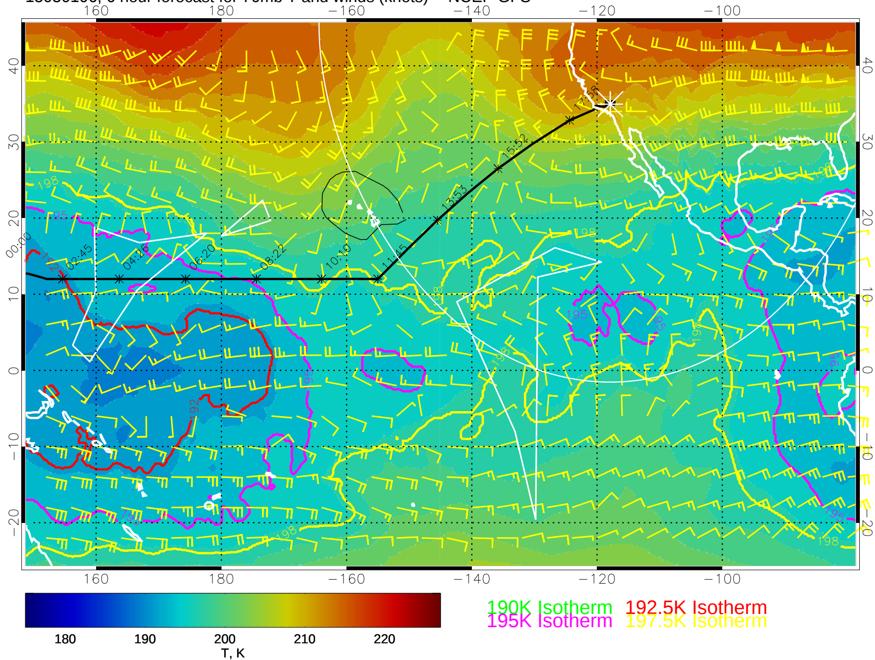
15030106, 6 hour forecast for 70mb T and winds (knots) -- NCEP GFS
