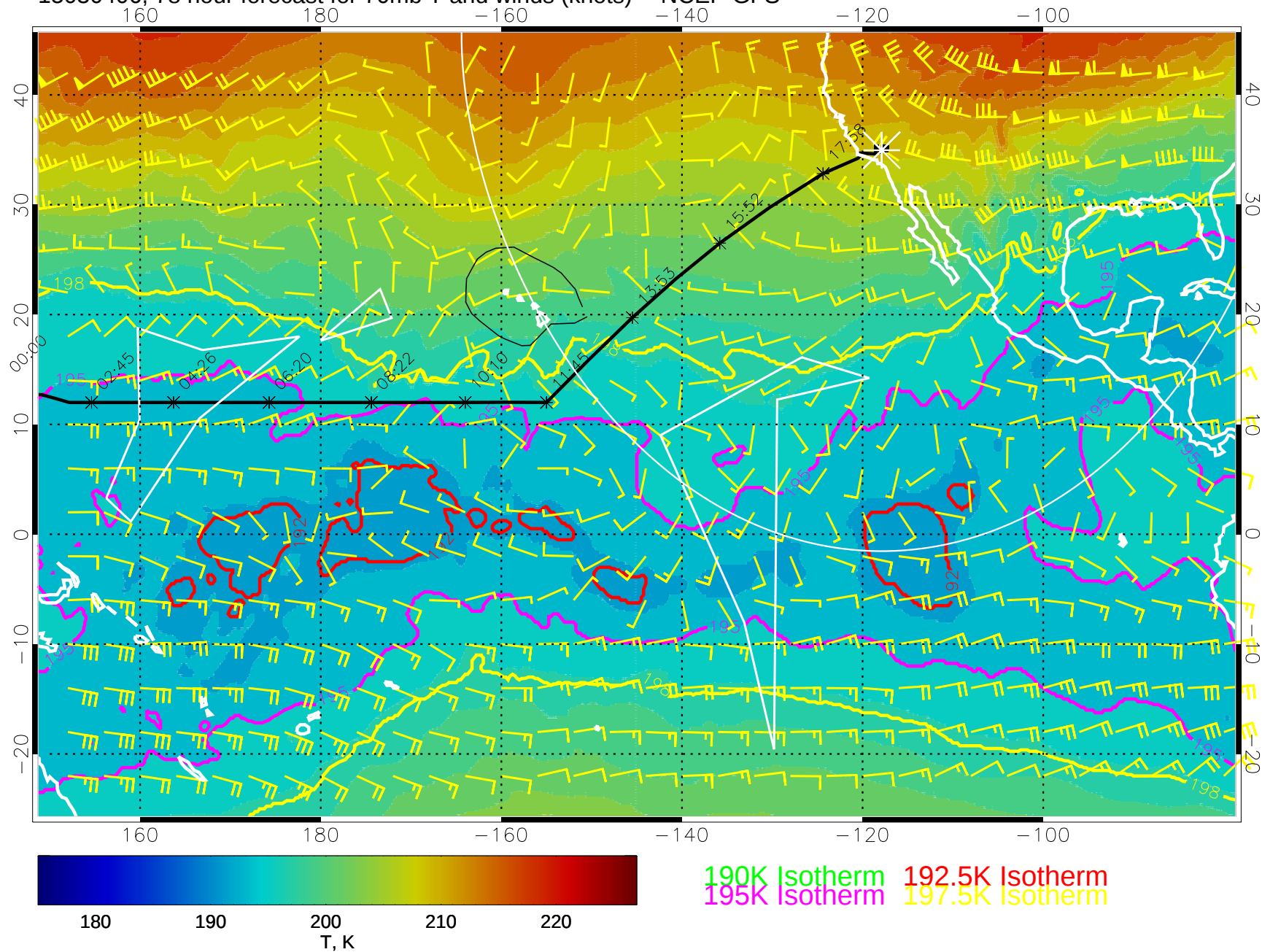
15030406, 78 hour forecast for 70mb T and winds (knots) -- NCEP GFS
