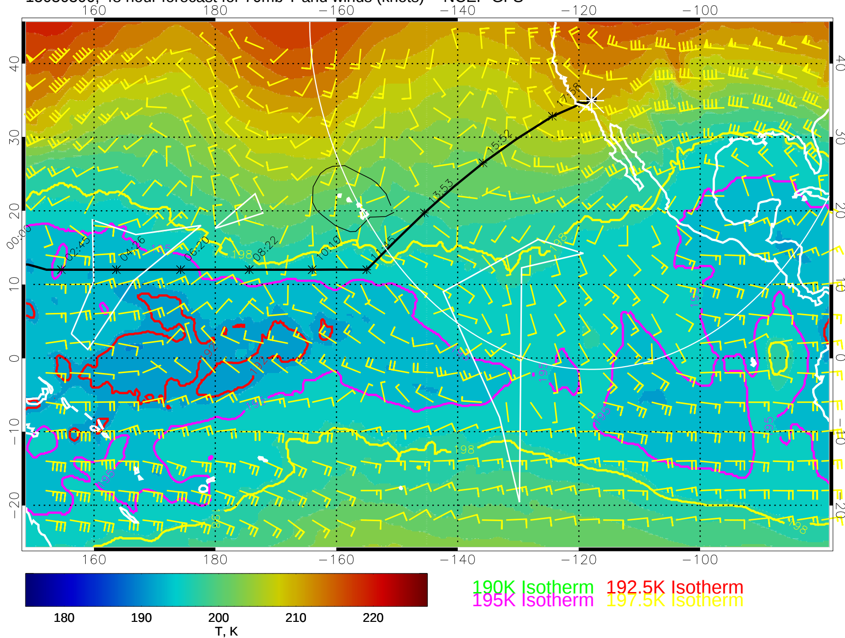
15030300, 48 hour forecast for 70mb T and winds (knots) -- NCEP GFS
