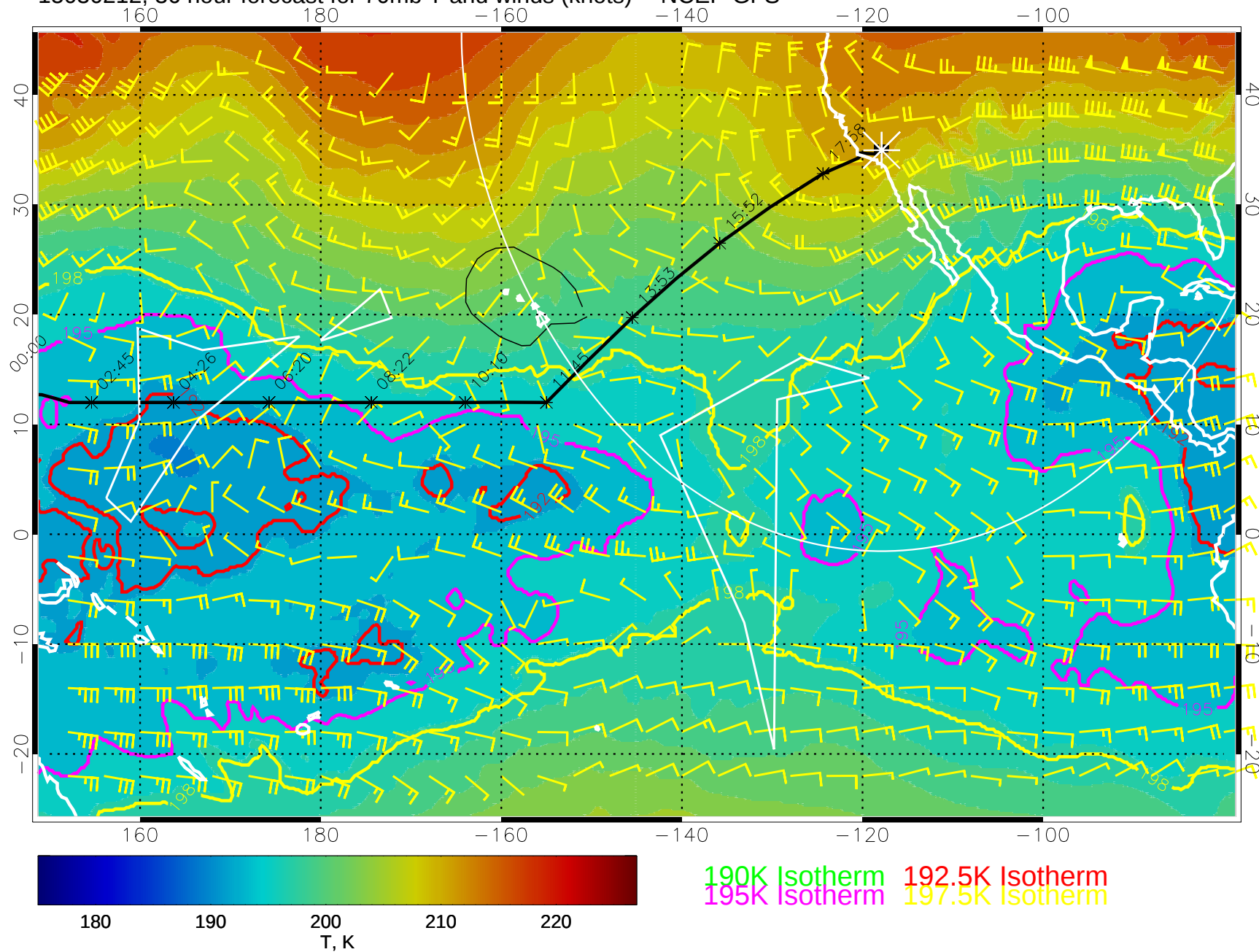
15030212, 36 hour forecast for 70mb T and winds (knots) -- NCEP GFS
