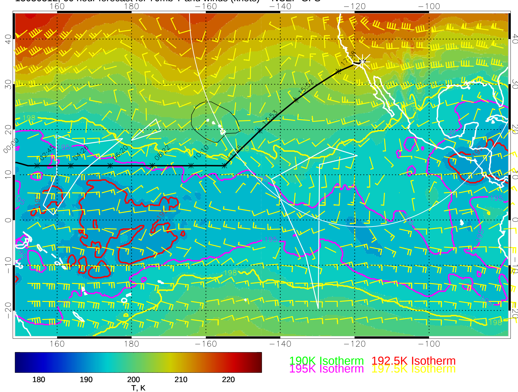
15030312, 60 hour forecast for 70mb T and winds (knots) -- NCEP GFS
