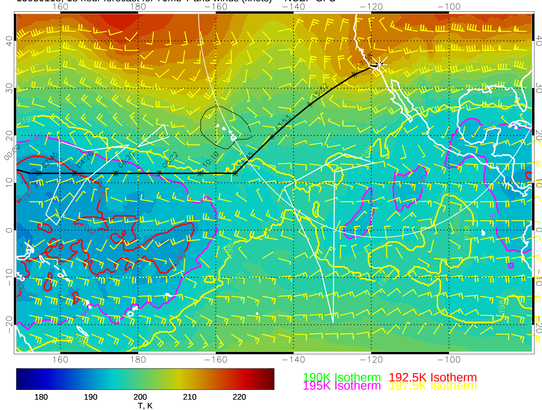
15030118, 18 hour forecast for 70mb T and winds (knots) -- NCEP GFS
