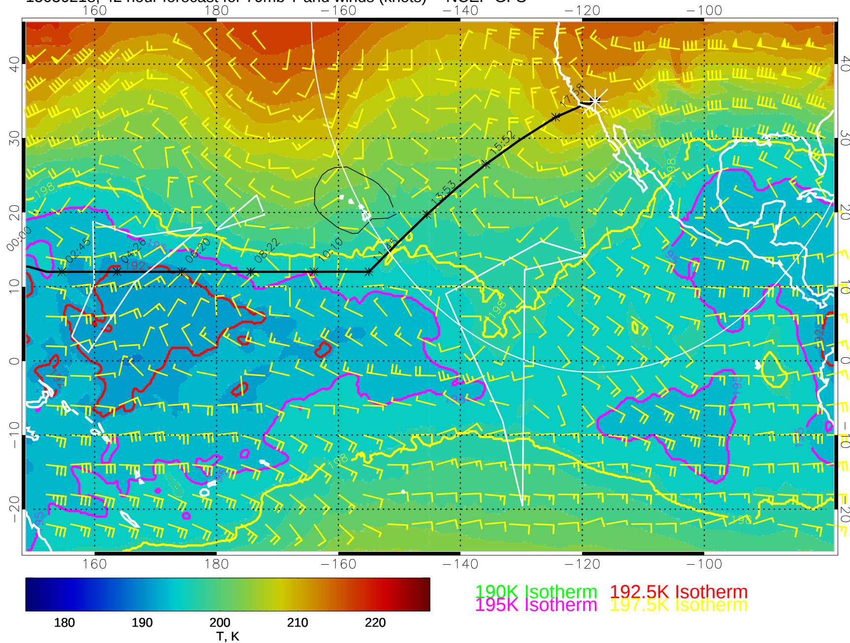
15030218, 42 hour forecast for 70mb T and winds (knots) -- NCEP GFS
