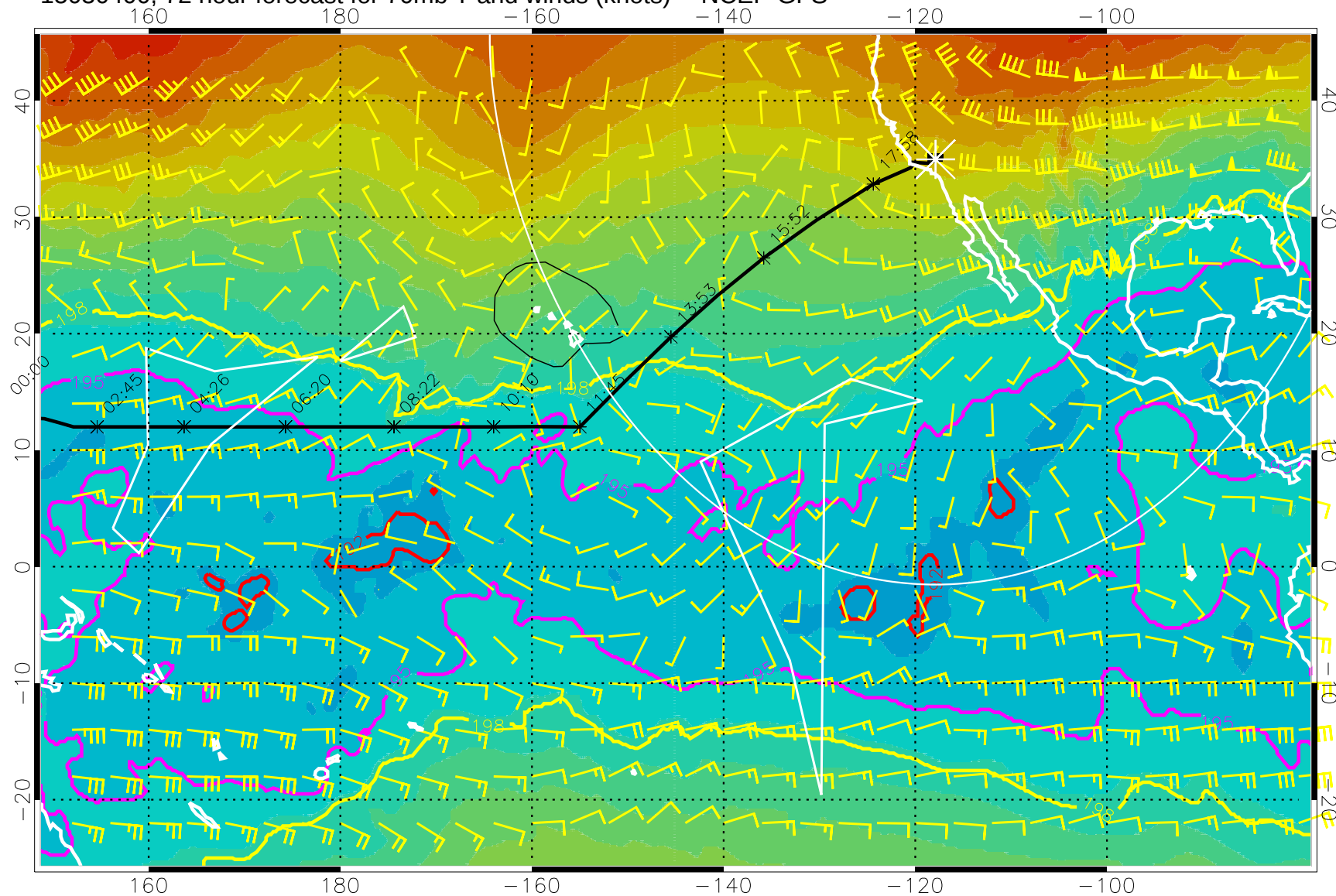
15030400, 72 hour forecast for 70mb T and winds (knots) -- NCEP GFS
