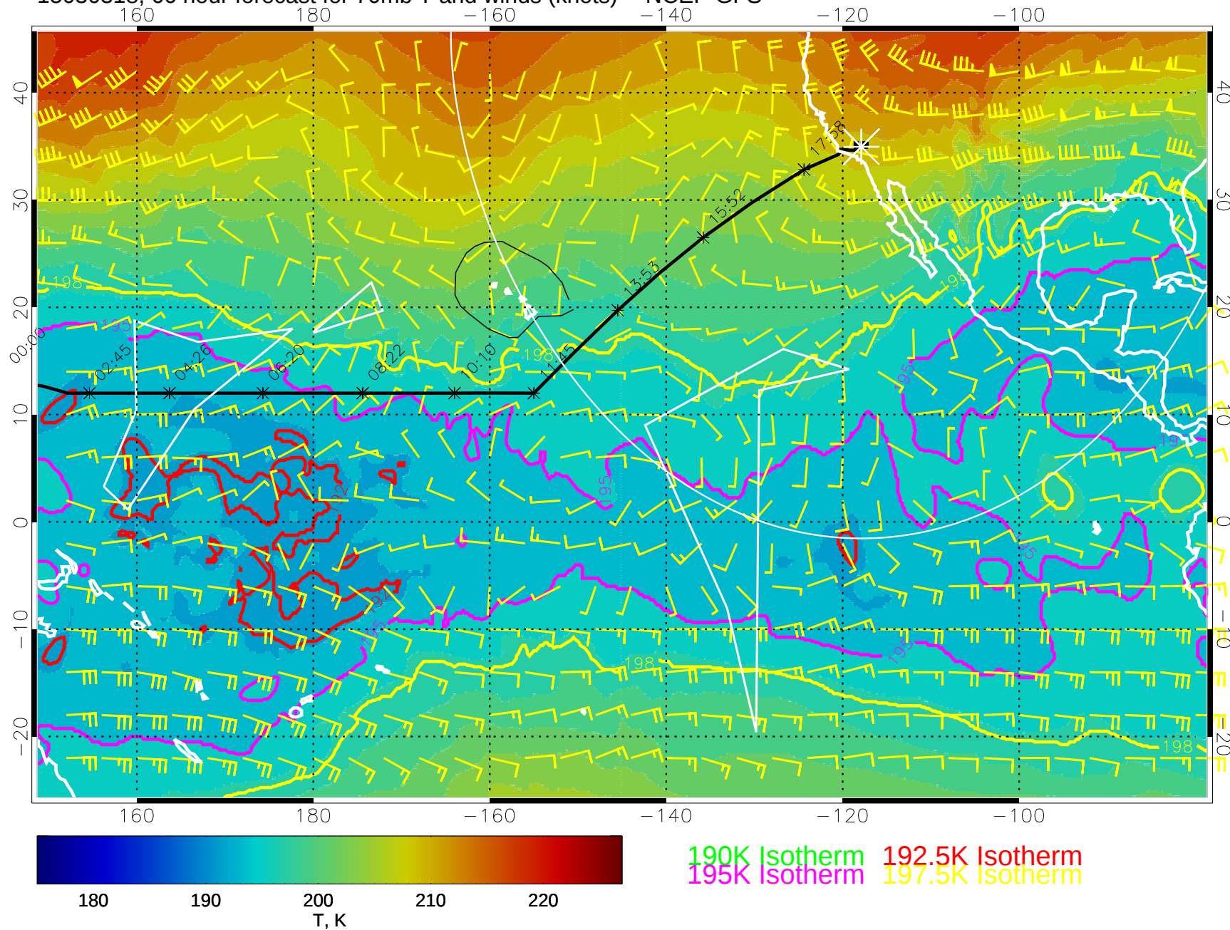
15030318, 66 hour forecast for 70mb T and winds (knots) -- NCEP GFS
