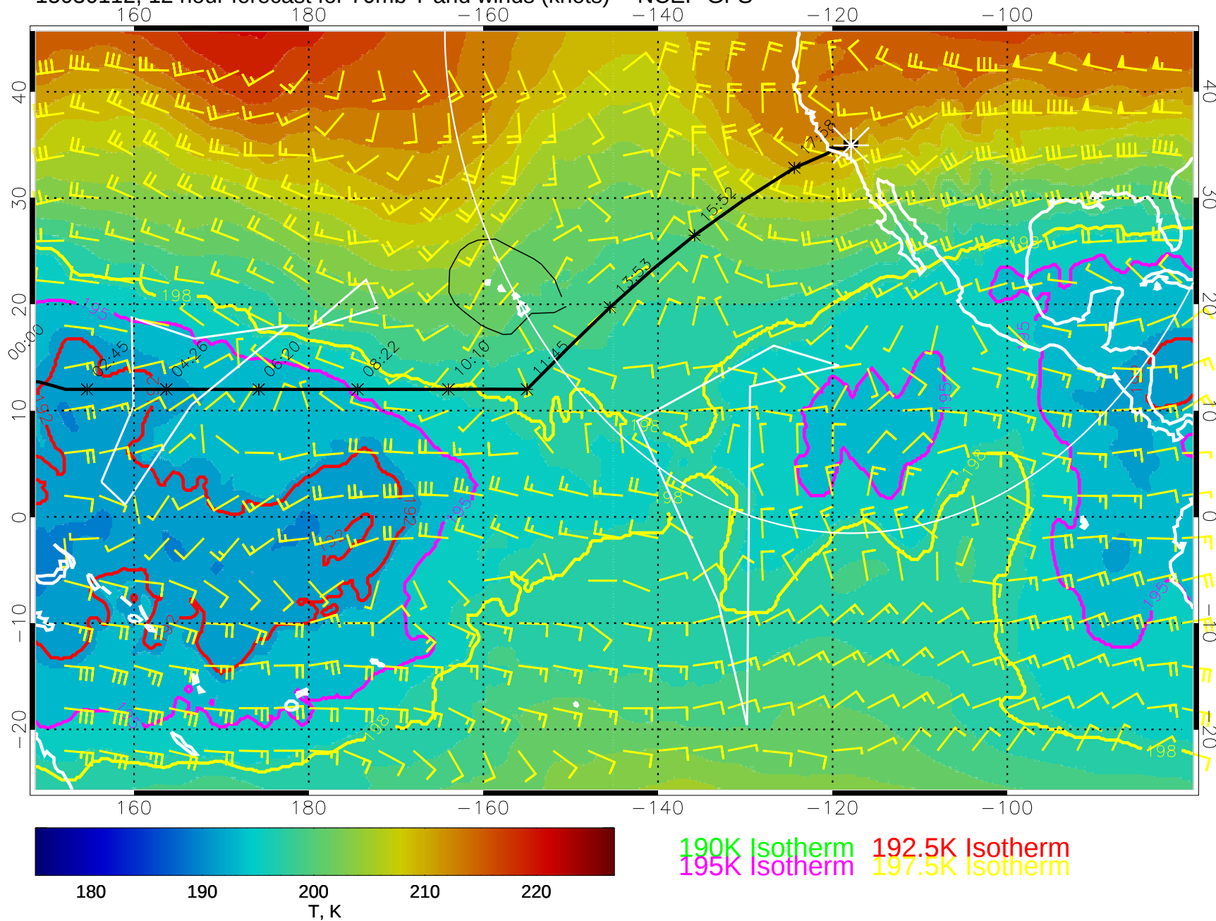
15030112, 12 hour forecast for 70mb T and winds (knots) -- NCEP GFS
