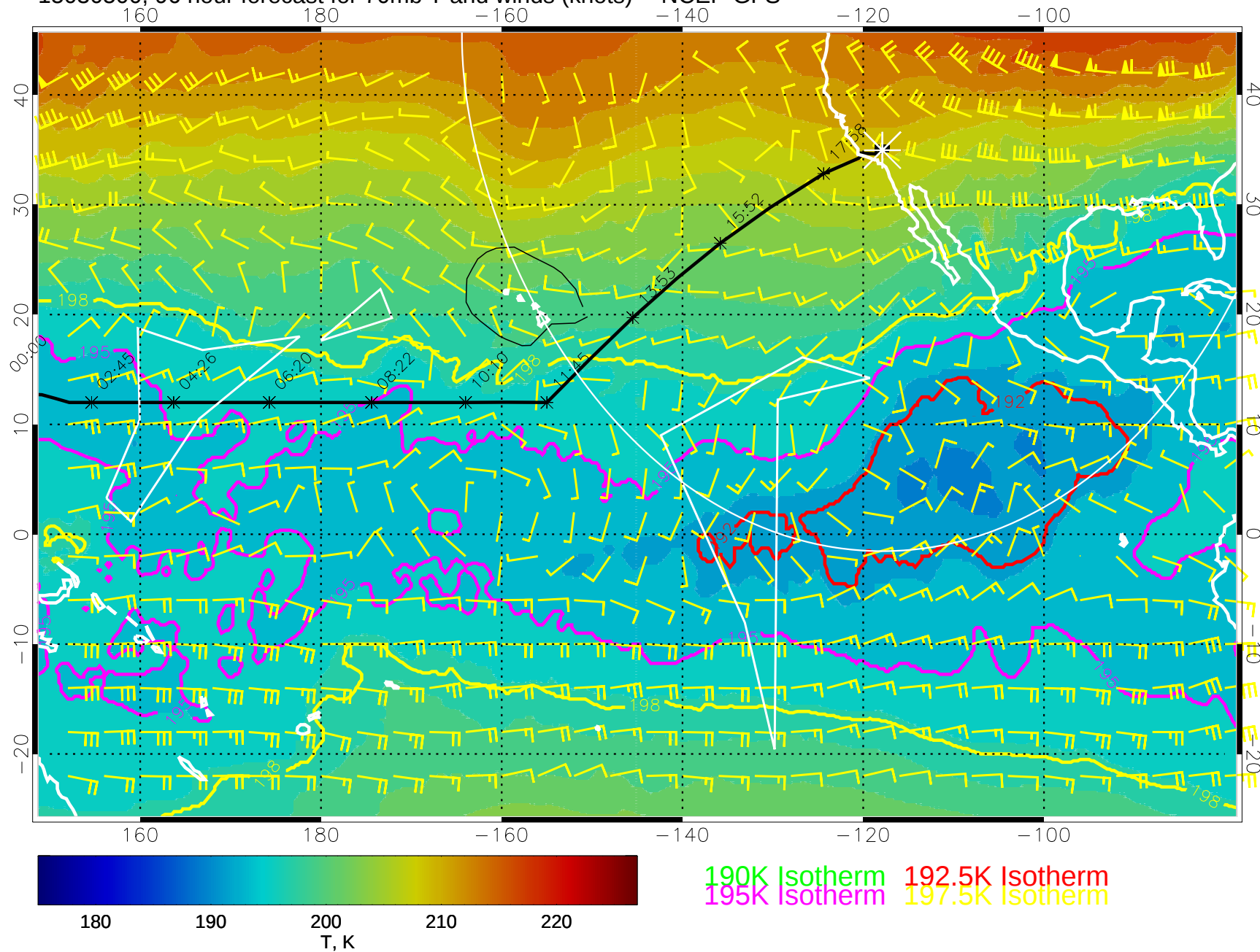
15030500, 96 hour forecast for 70mb T and winds (knots) -- NCEP GFS
