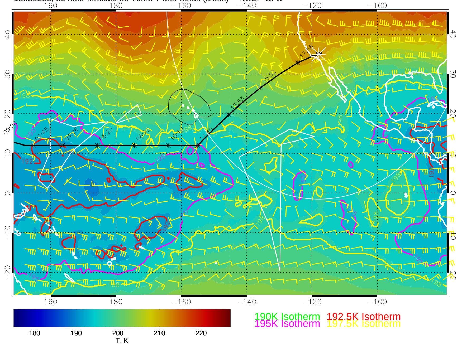
15030206, 30 hour forecast for 70mb T and winds (knots) -- NCEP GFS
