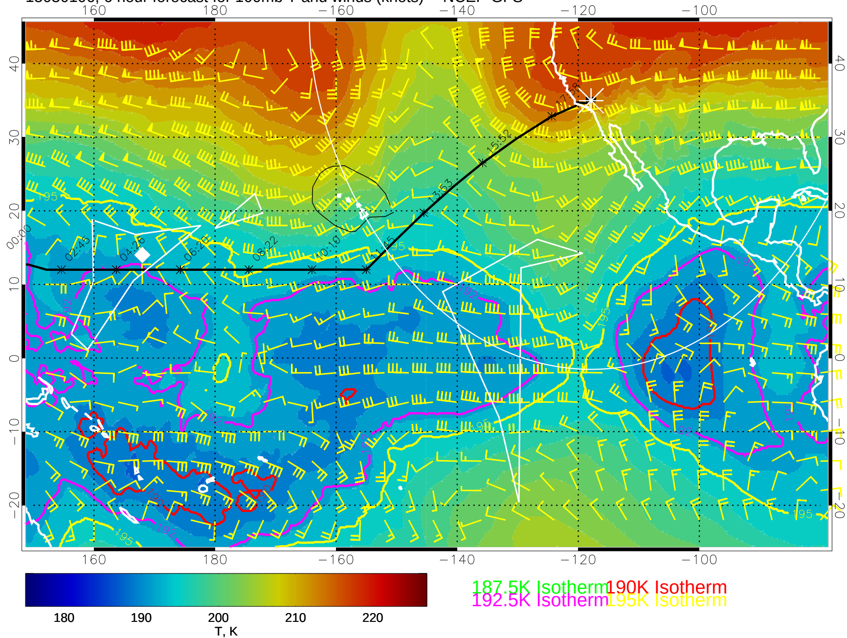
15030106, 6 hour forecast for 100mb T and winds (knots) -- NCEP GFS
