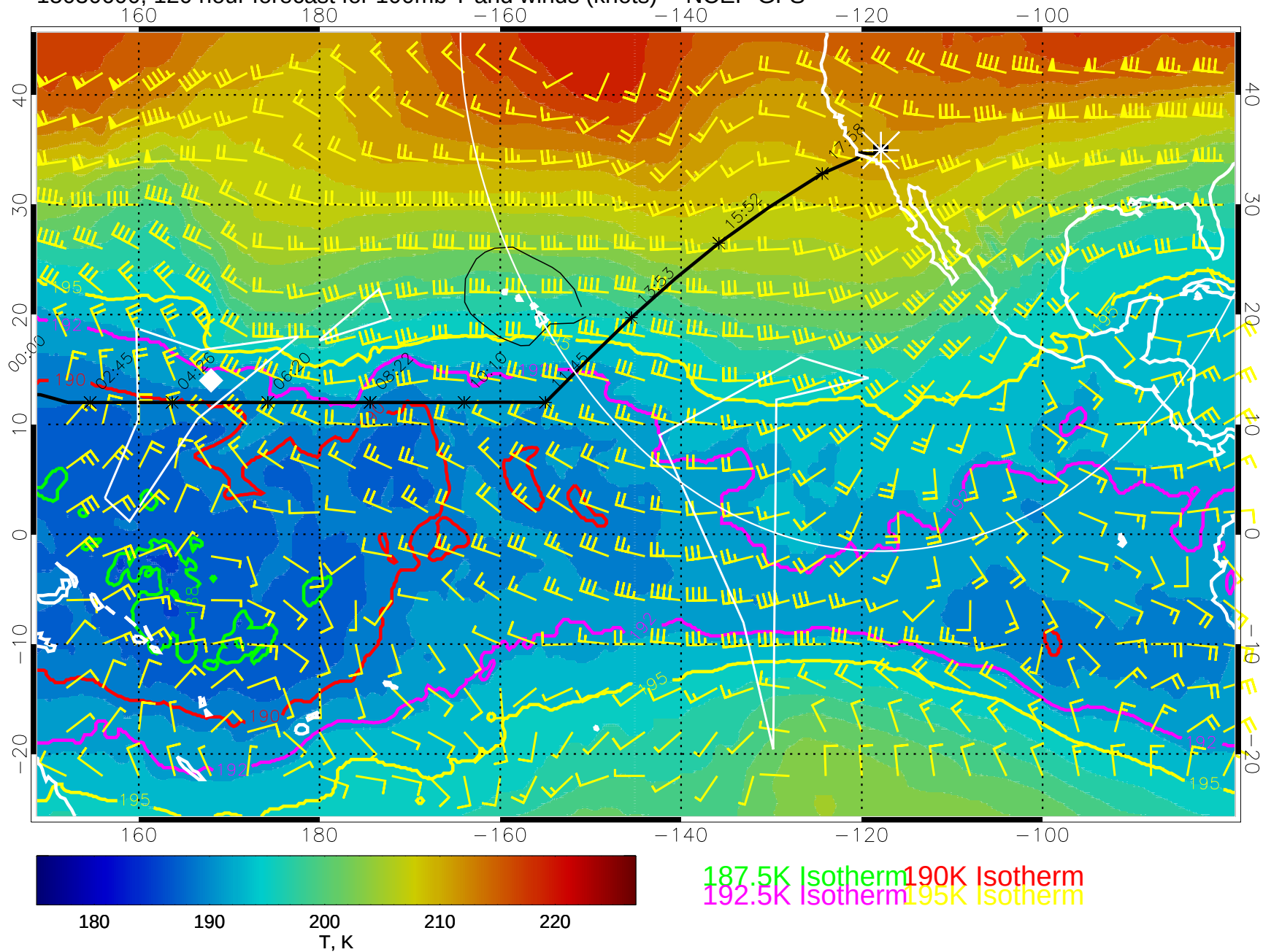
15030600, 120 hour forecast for 100mb T and winds (knots) -- NCEP GFS
