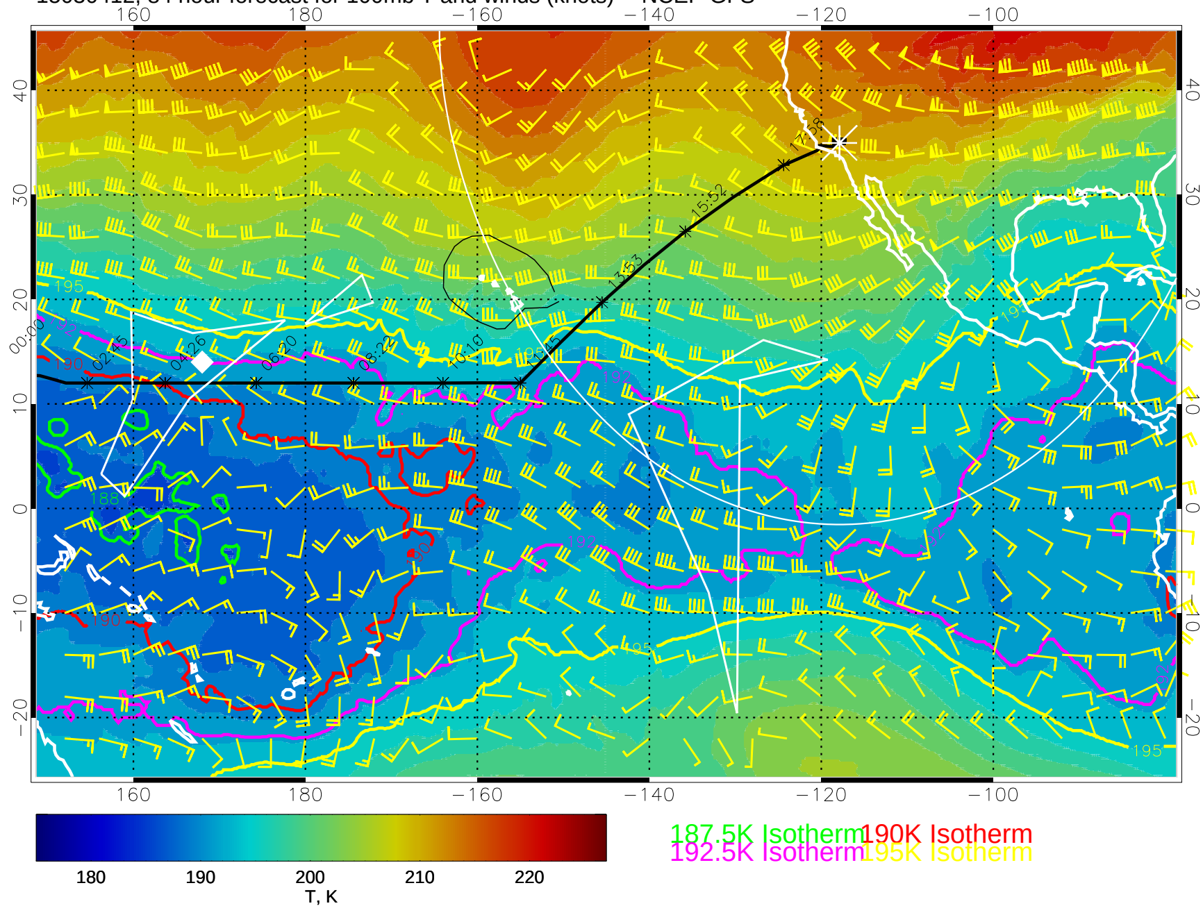
15030412, 84 hour forecast for 100mb T and winds (knots) -- NCEP GFS
