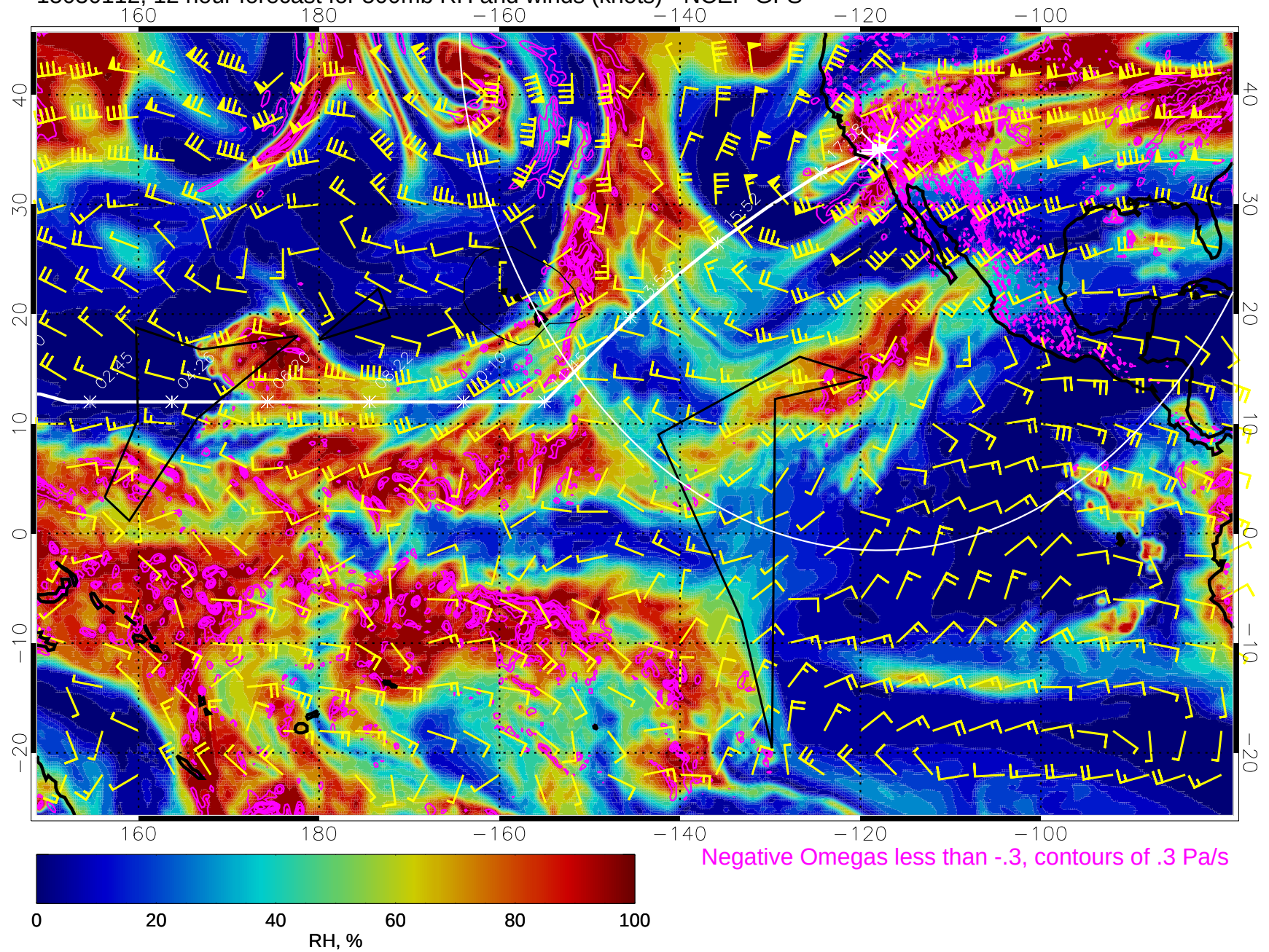
15030112, 12 hour forecast for 500mb RH and winds (knots) - NCEP GFS
