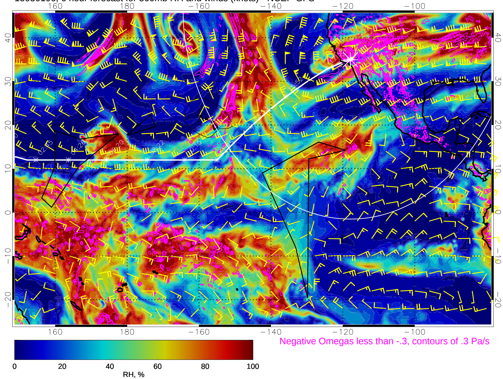
15030106, 6 hour forecast for 500mb RH and winds (knots) - NCEP GFS
