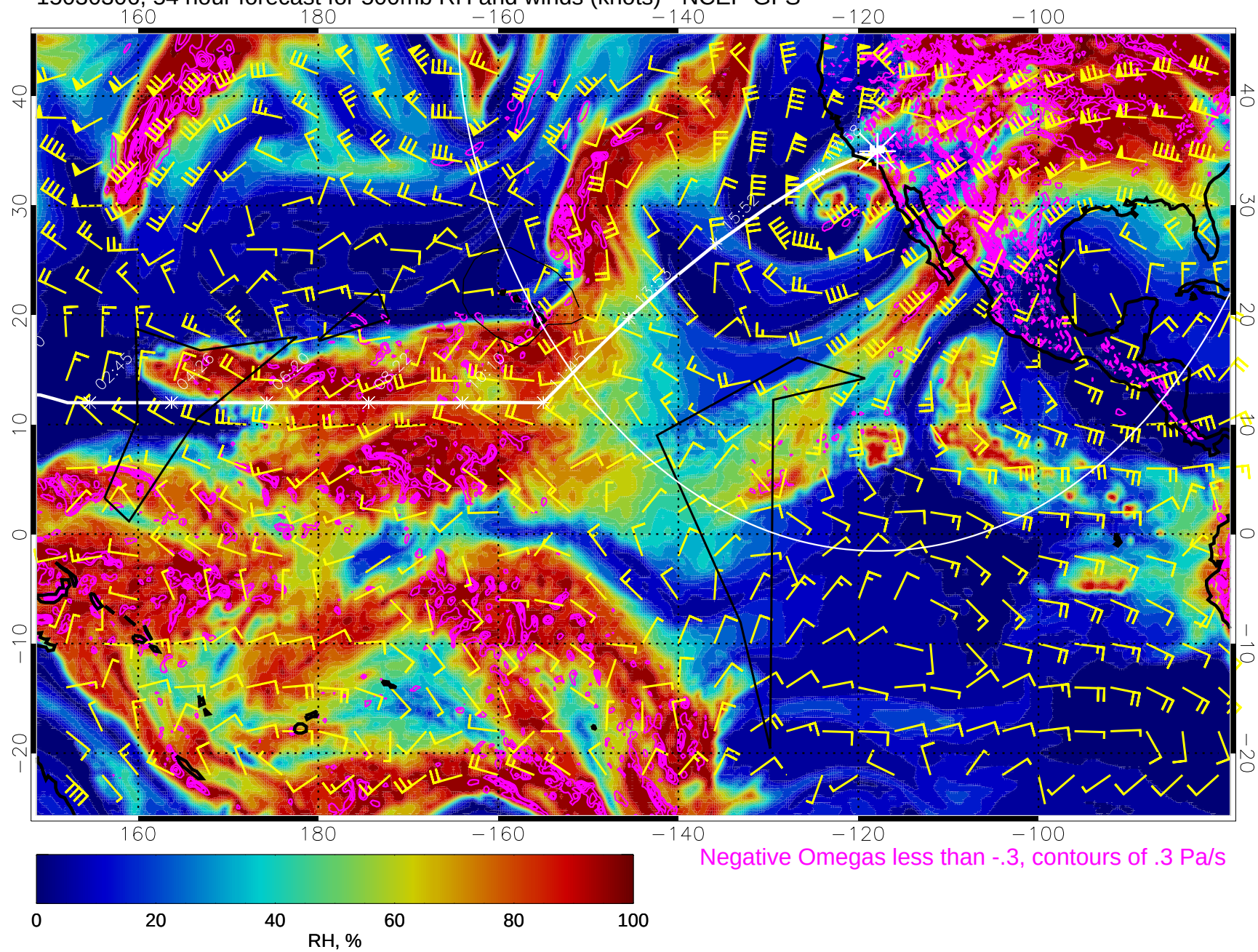
15030306, 54 hour forecast for 500mb RH and winds (knots) - NCEP GFS
