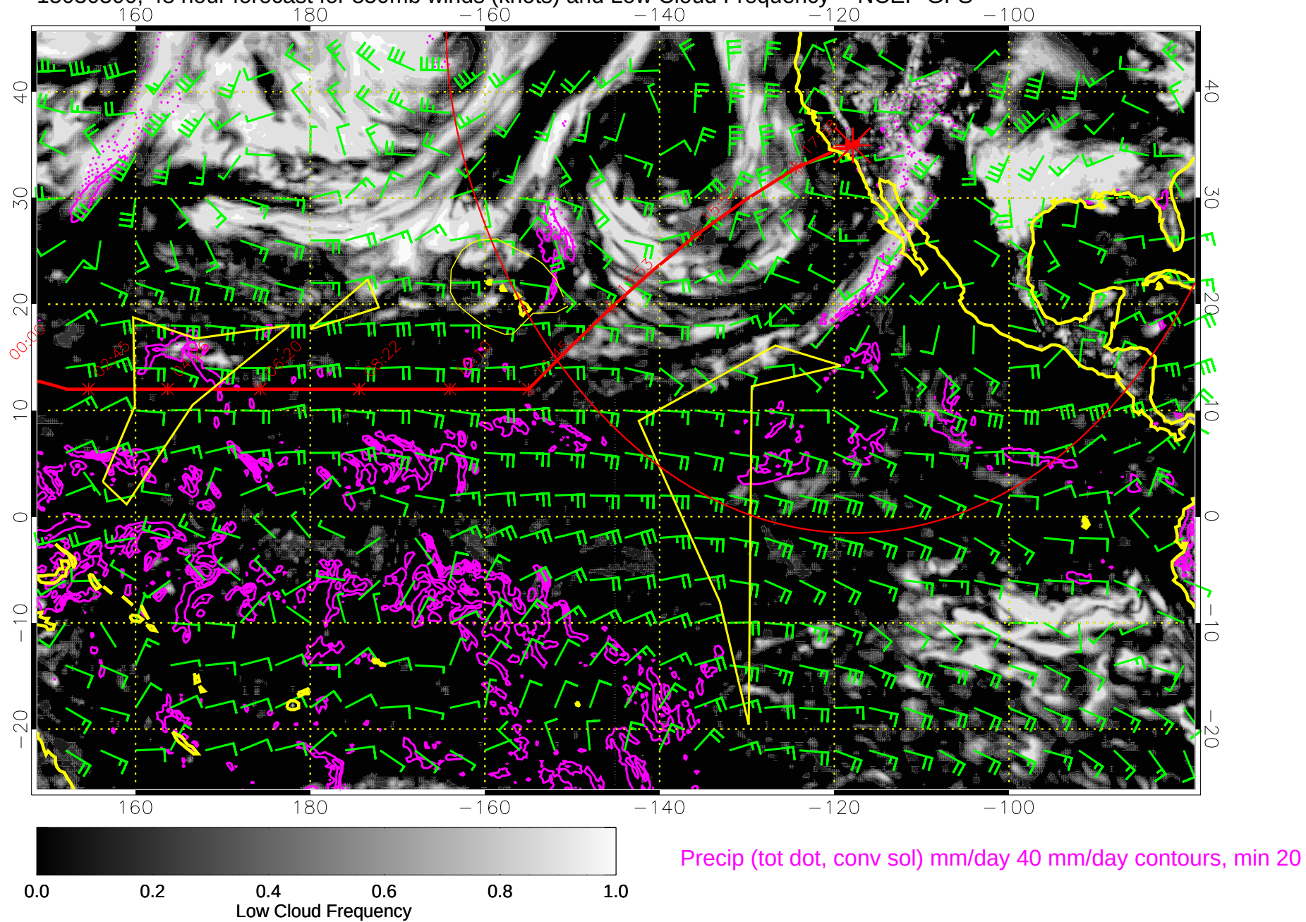
15030300, 48 hour forecast for 850mb winds (knots) and Low Cloud Frequency -- NCEP GFS
