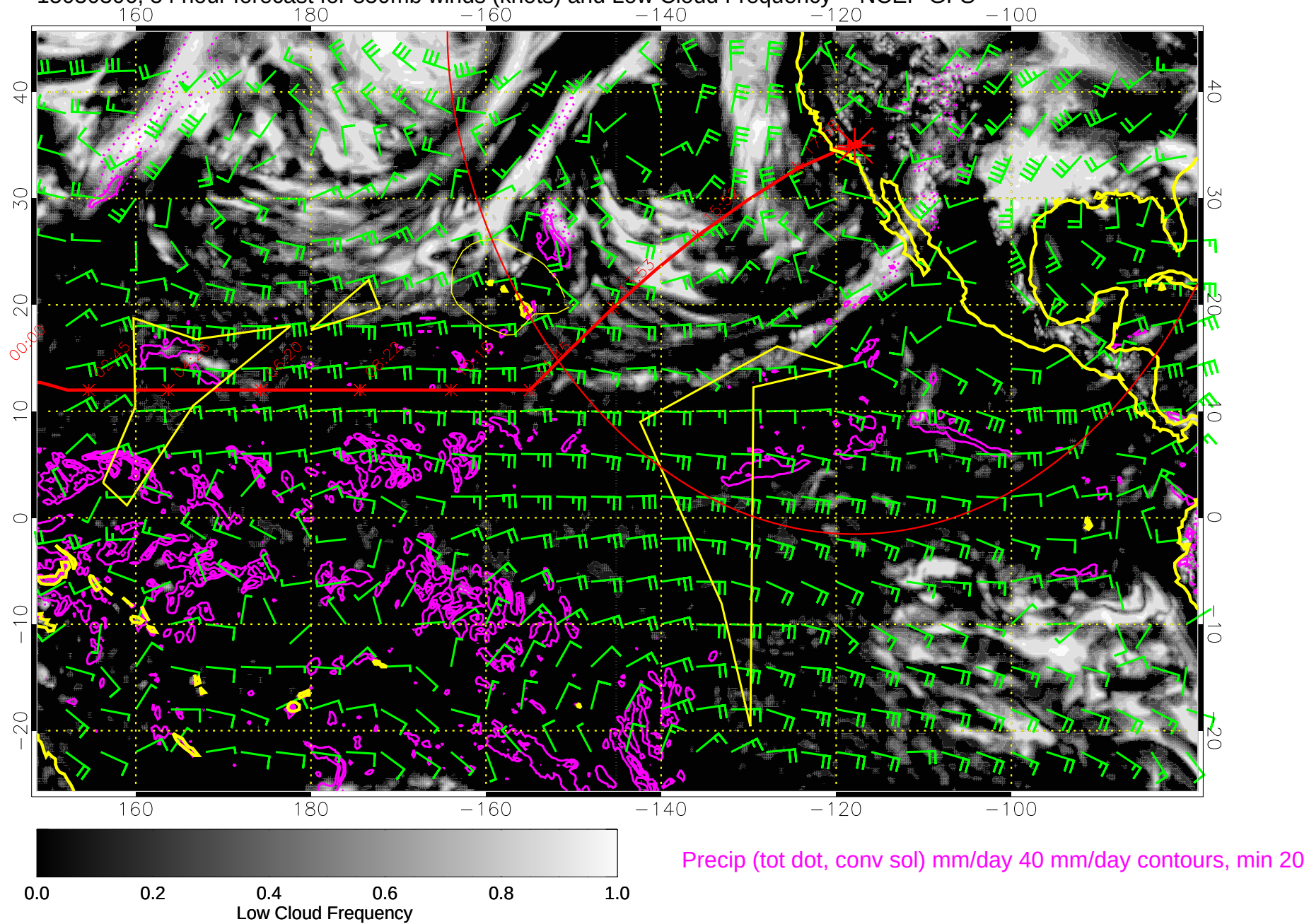
15030306, 54 hour forecast for 850mb winds (knots) and Low Cloud Frequency -- NCEP GFS
