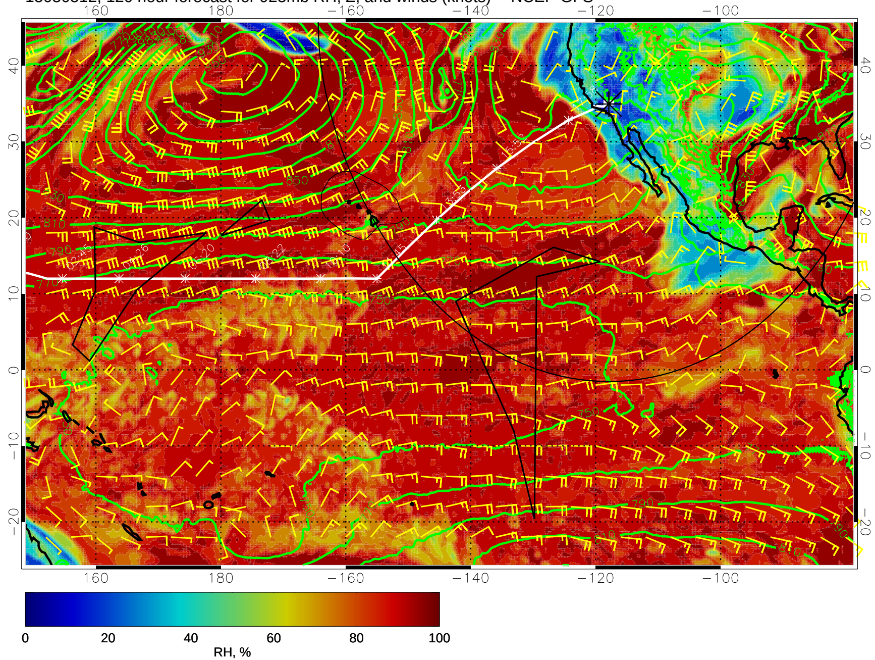
15030512, 120 hour forecast for 925mb RH, Z, and winds (knots) -- NCEP GFS
