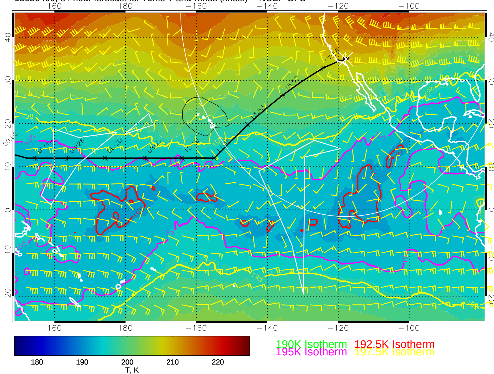
15030400, 84 hour forecast for 70mb T and winds (knots) -- NCEP GFS
