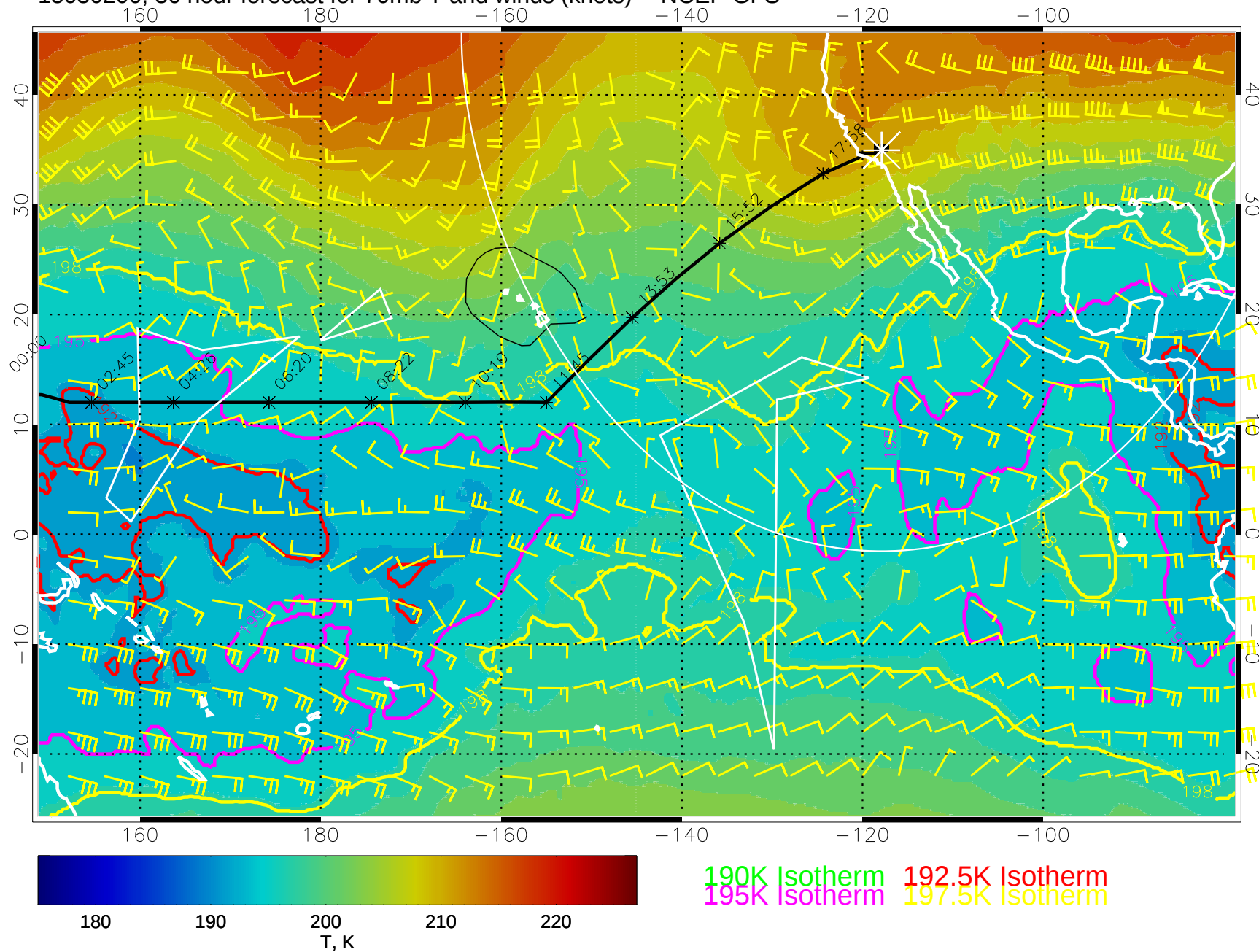
15030200, 36 hour forecast for 70mb T and winds (knots) -- NCEP GFS
