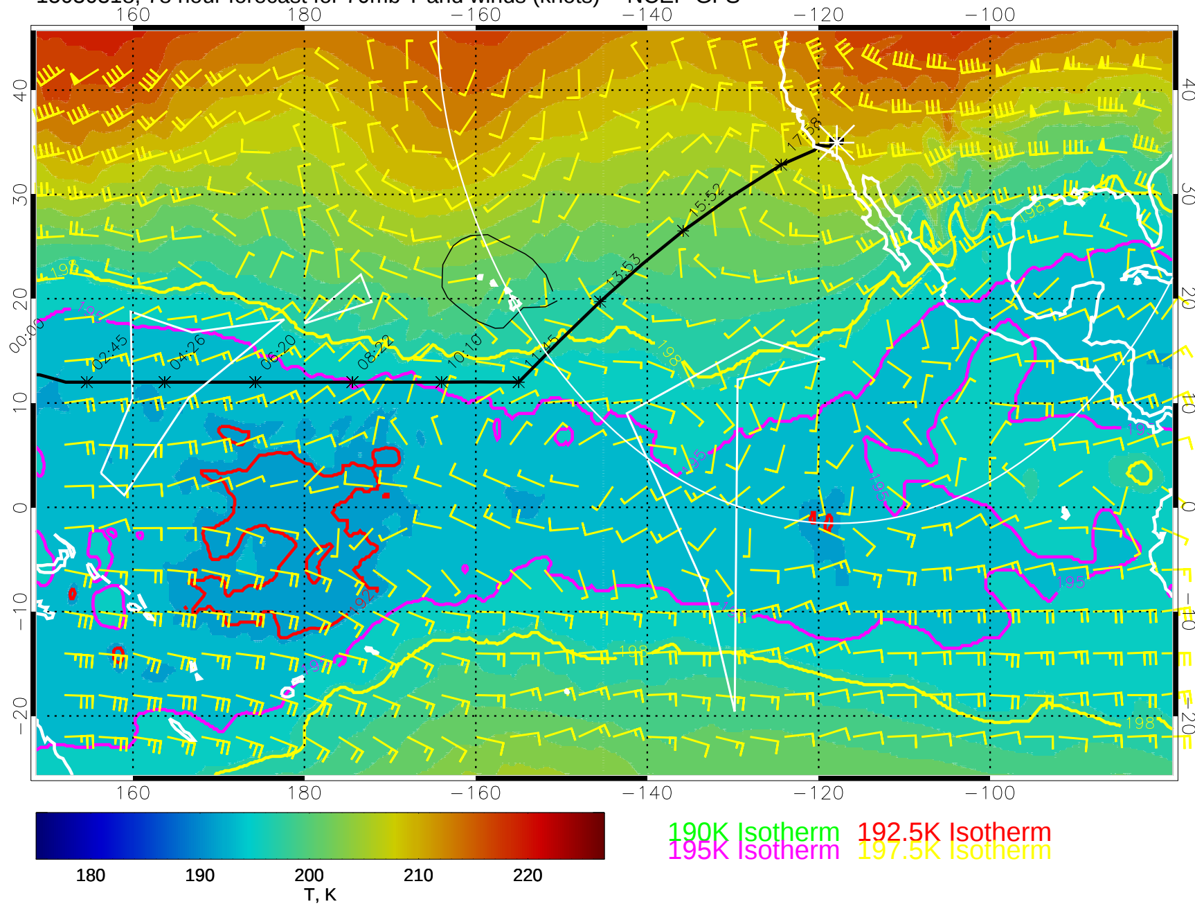
15030318, 78 hour forecast for 70mb T and winds (knots) -- NCEP GFS
