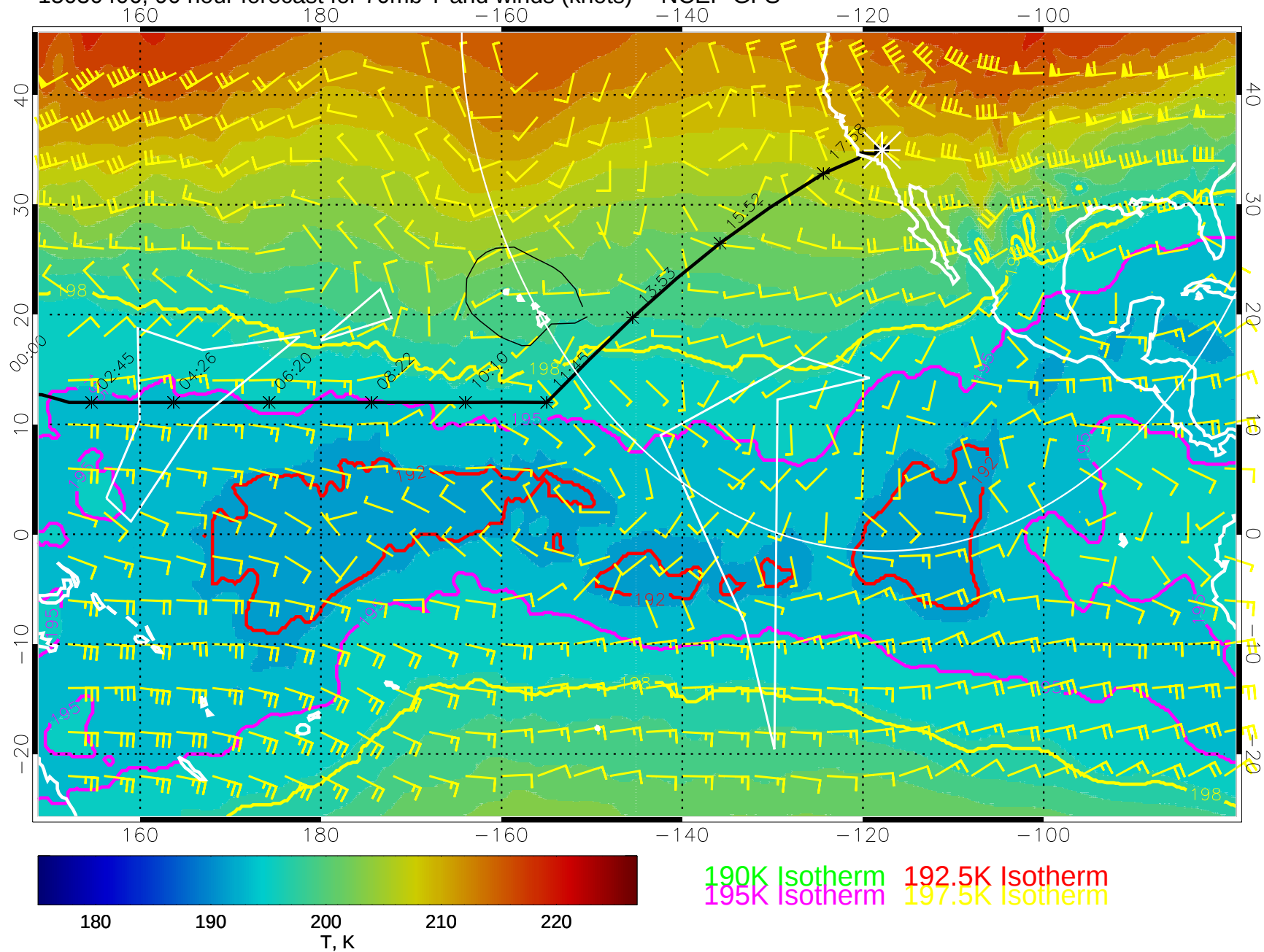
15030406, 90 hour forecast for 70mb T and winds (knots) -- NCEP GFS
