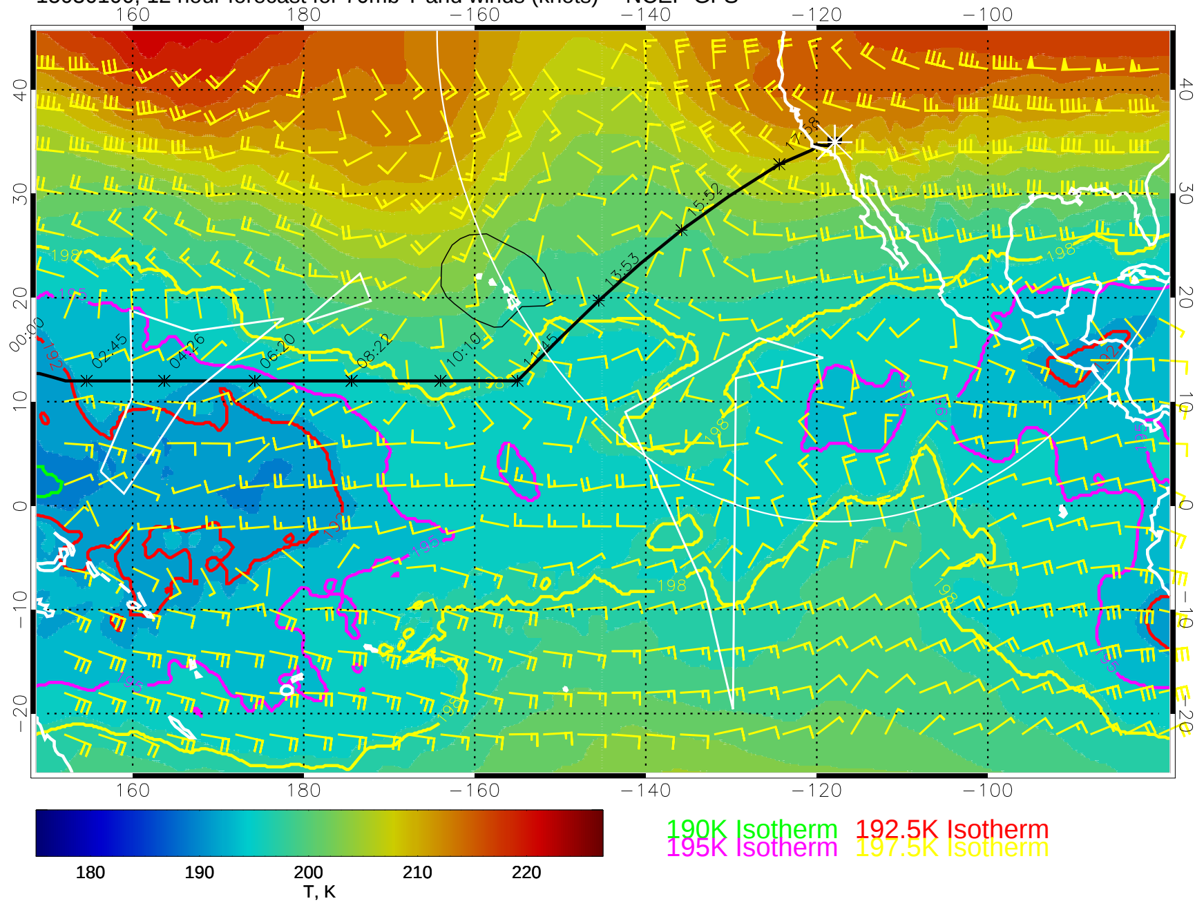
15030100, 12 hour forecast for 70mb T and winds (knots) -- NCEP GFS
