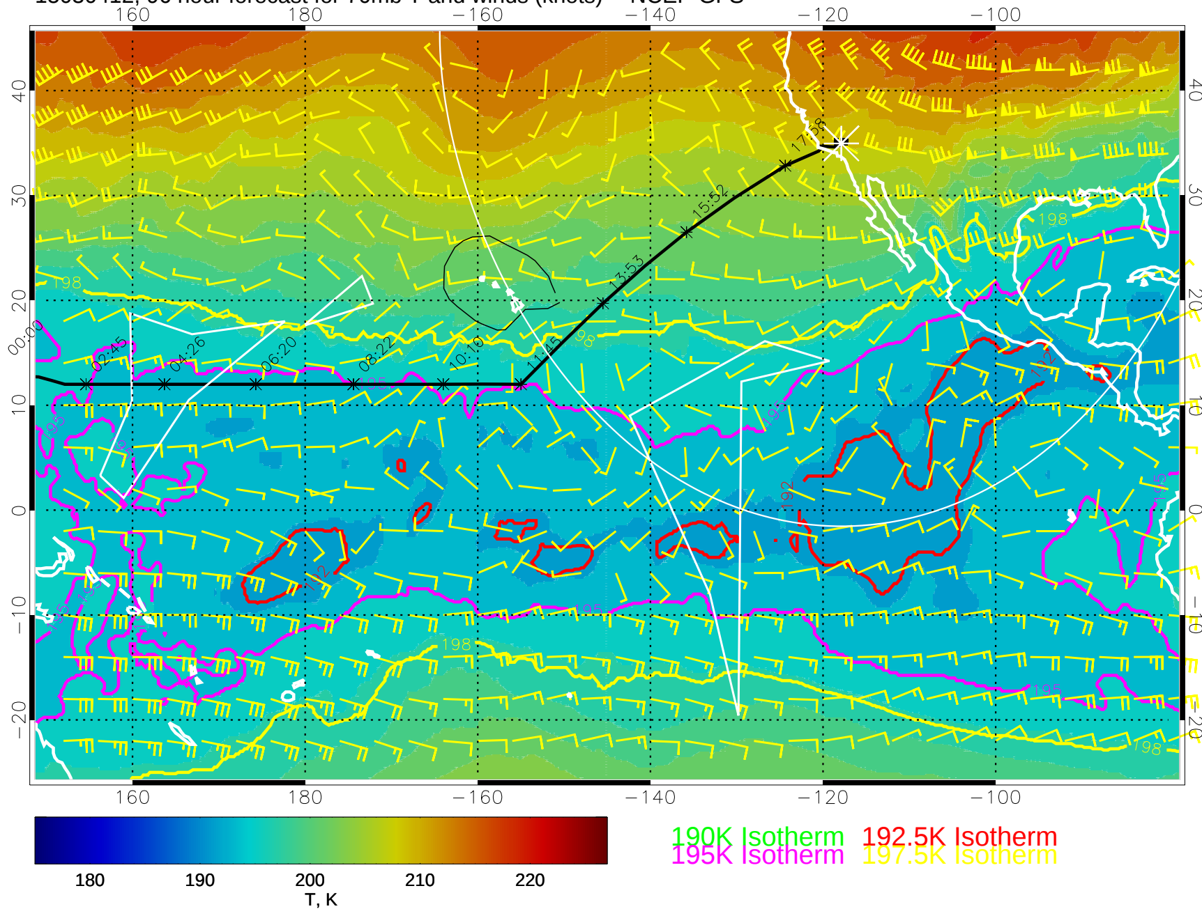
15030412, 96 hour forecast for 70mb T and winds (knots) -- NCEP GFS
