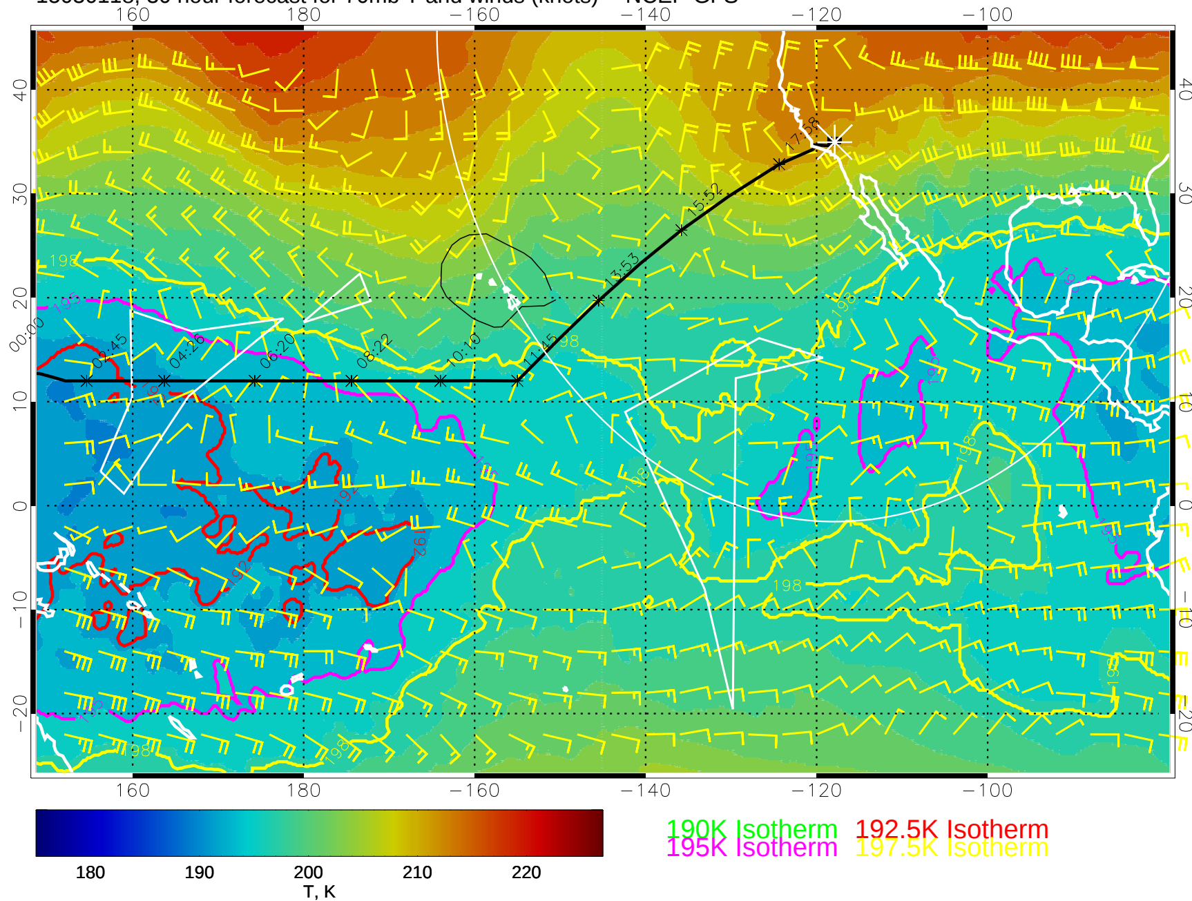
15030118, 30 hour forecast for 70mb T and winds (knots) -- NCEP GFS
