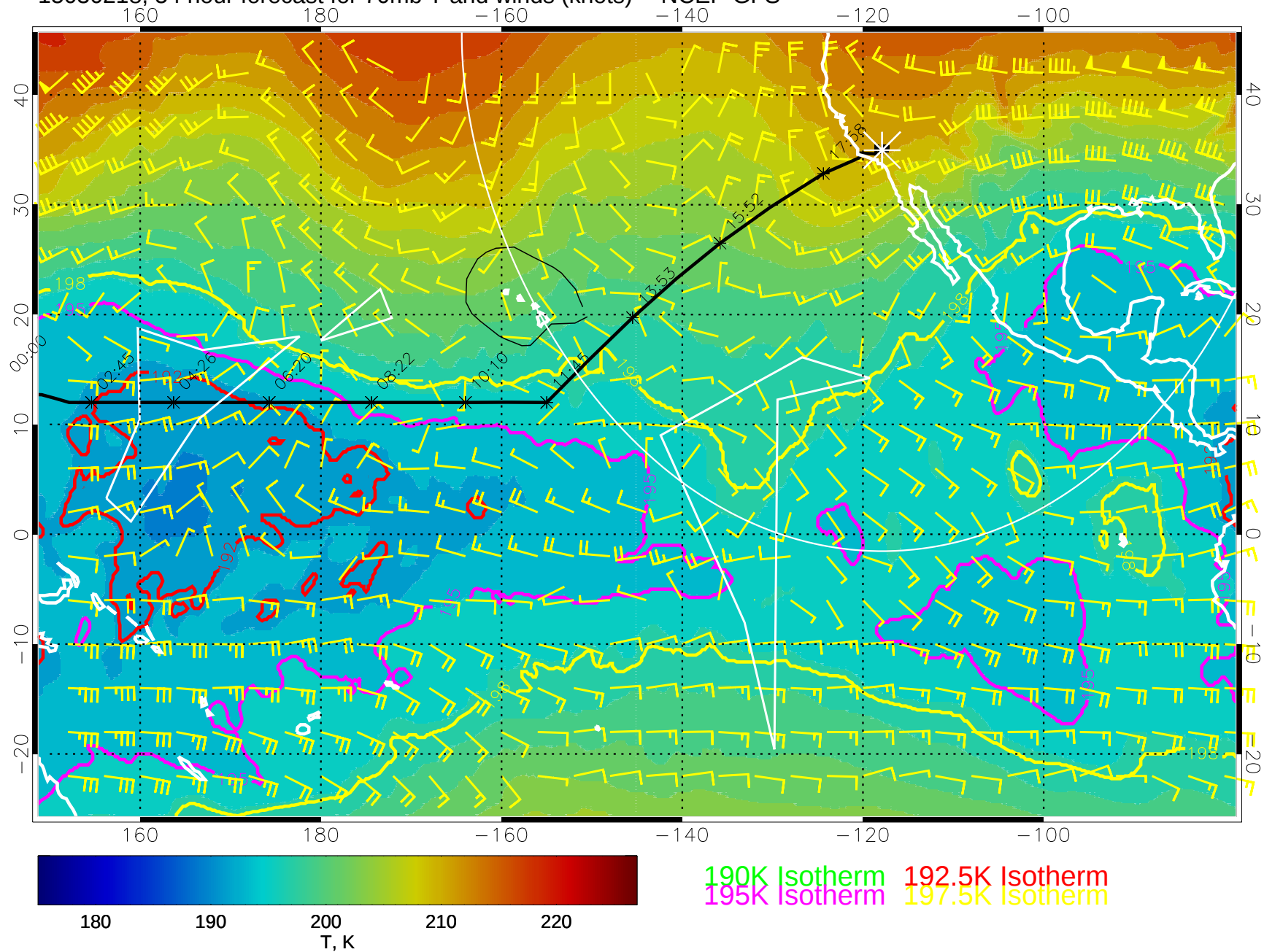
15030218, 54 hour forecast for 70mb T and winds (knots) -- NCEP GFS
