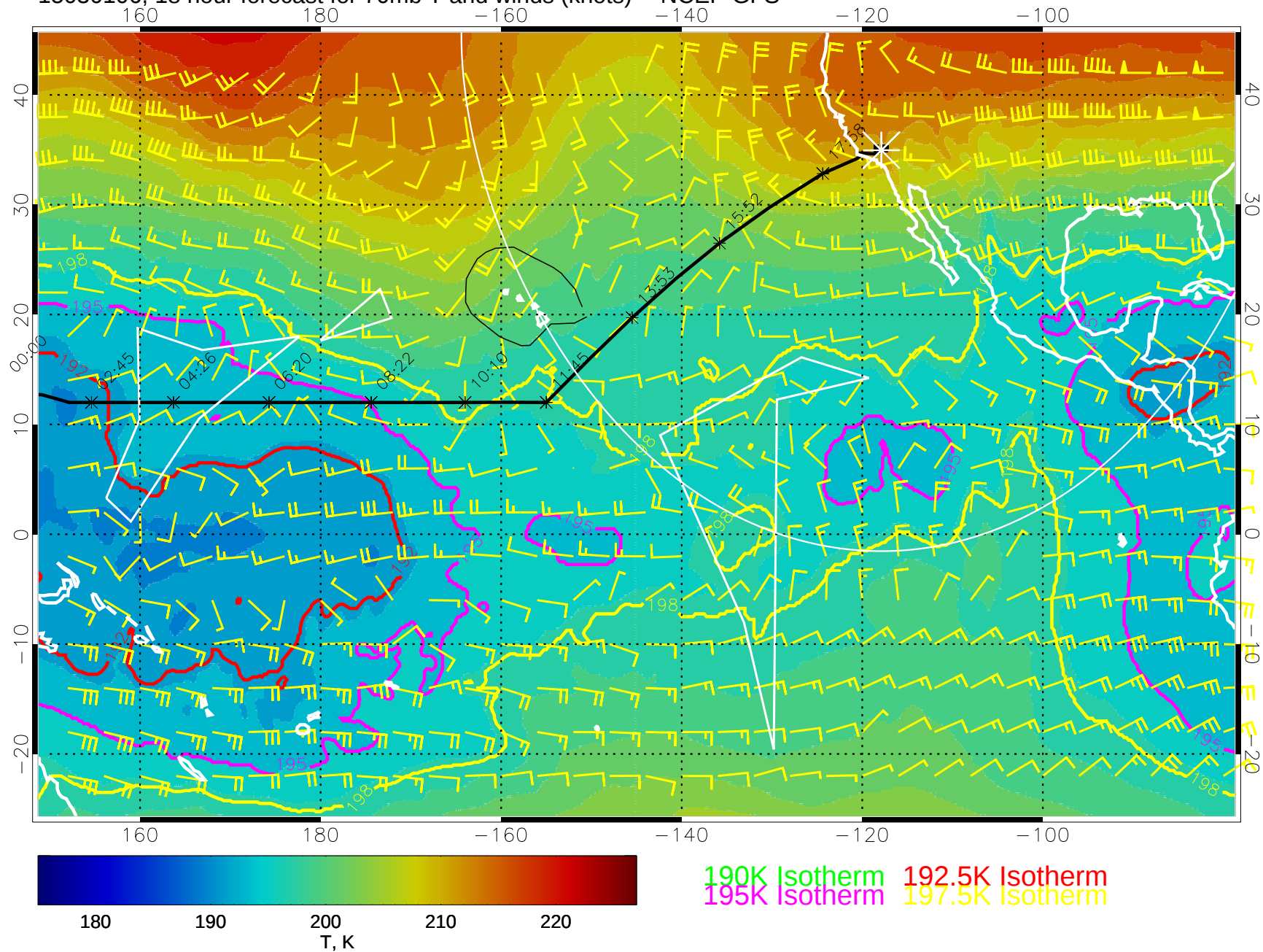
15030106, 18 hour forecast for 70mb T and winds (knots) -- NCEP GFS
