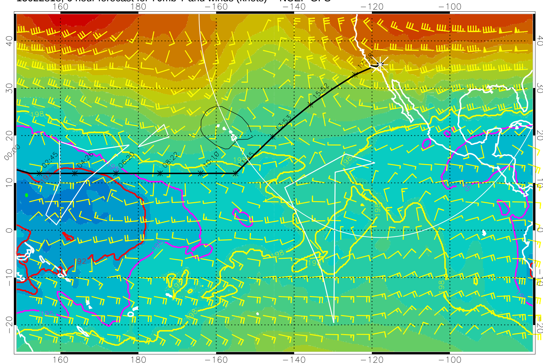
15022818, 6 hour forecast for 70mb T and winds (knots) -- NCEP GFS
