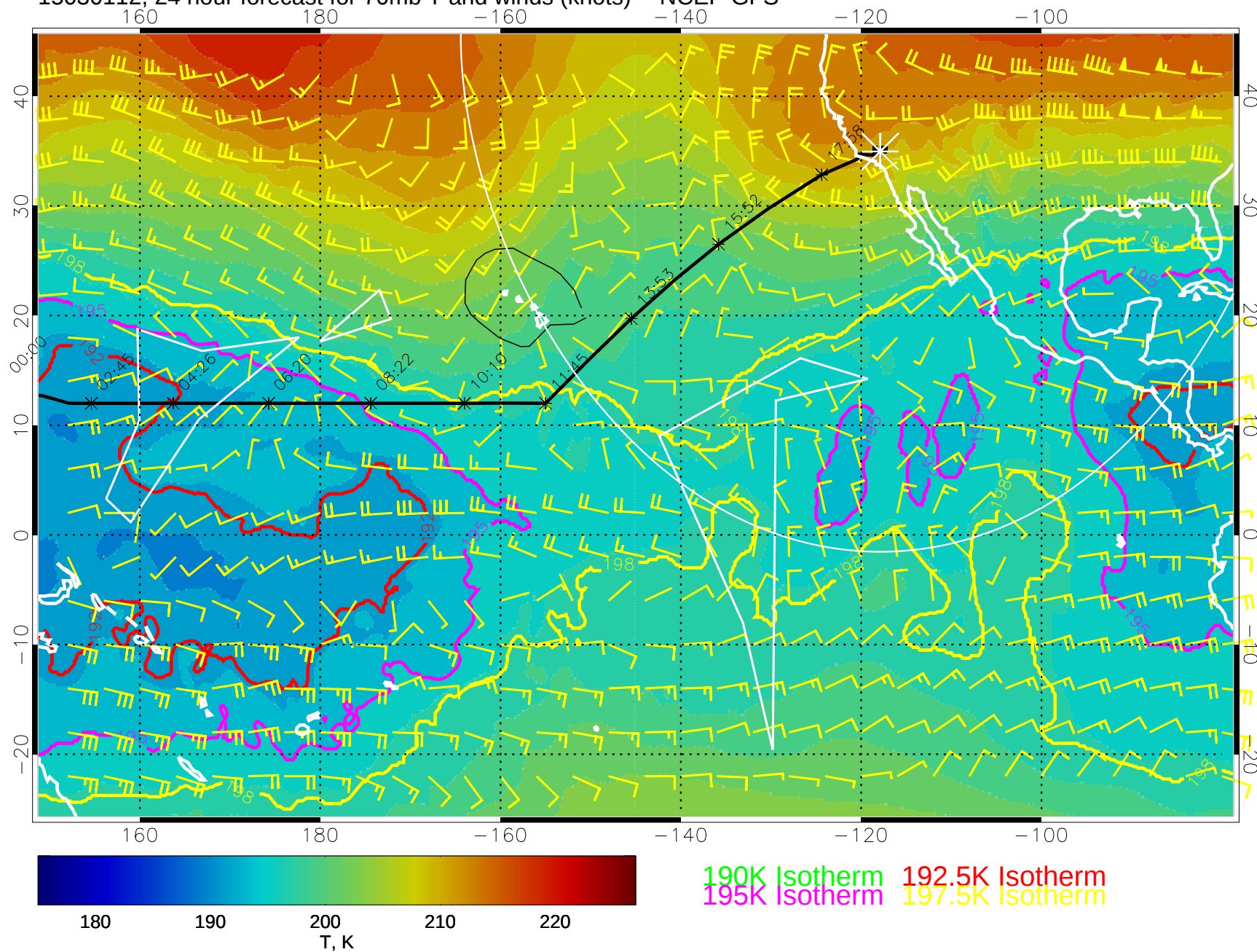
15030112, 24 hour forecast for 70mb T and winds (knots) -- NCEP GFS
