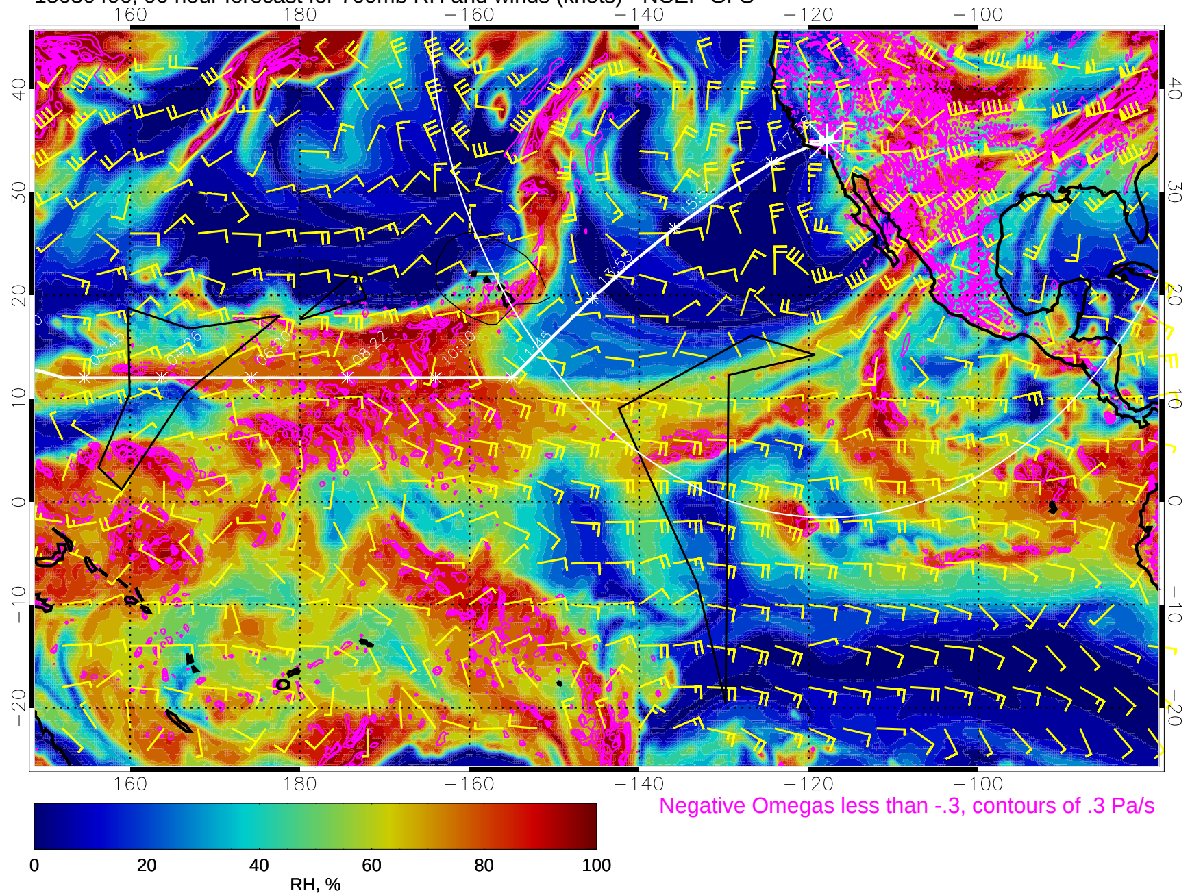
15030406, 90 hour forecast for 700mb RH and winds (knots) - NCEP GFS
