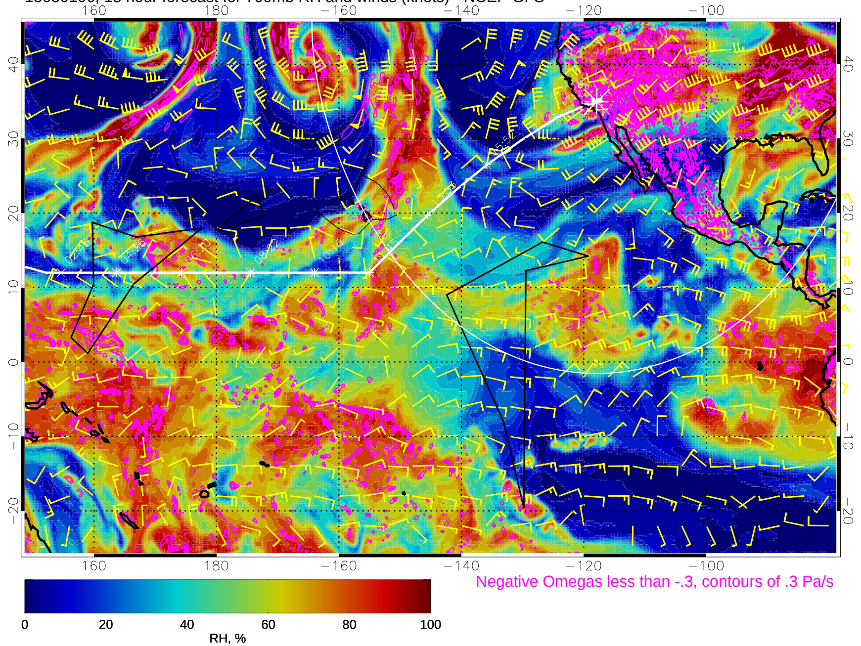
15030106, 18 hour forecast for 700mb RH and winds (knots) - NCEP GFS
