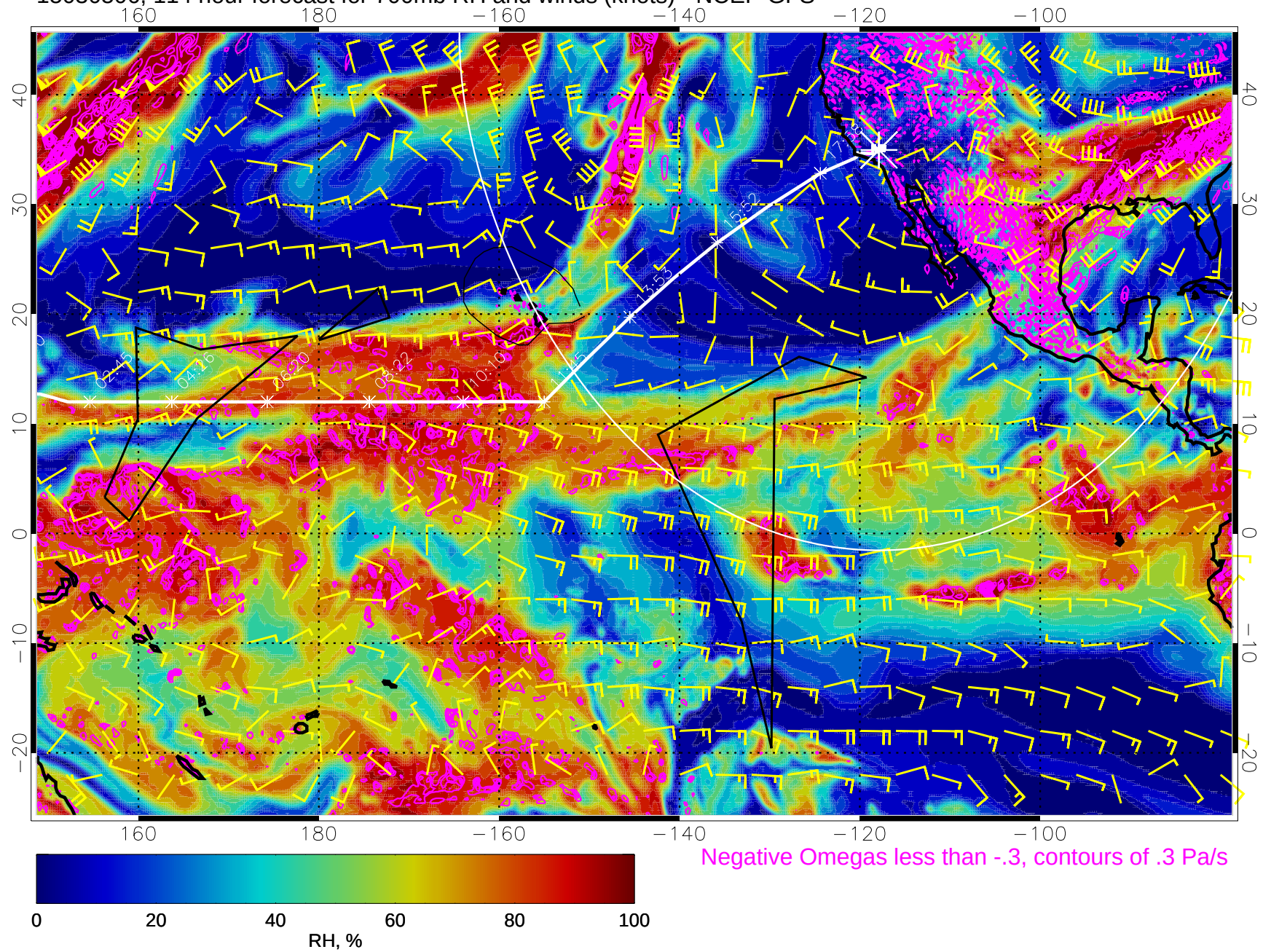
15030506, 114 hour forecast for 700mb RH and winds (knots) - NCEP GFS
