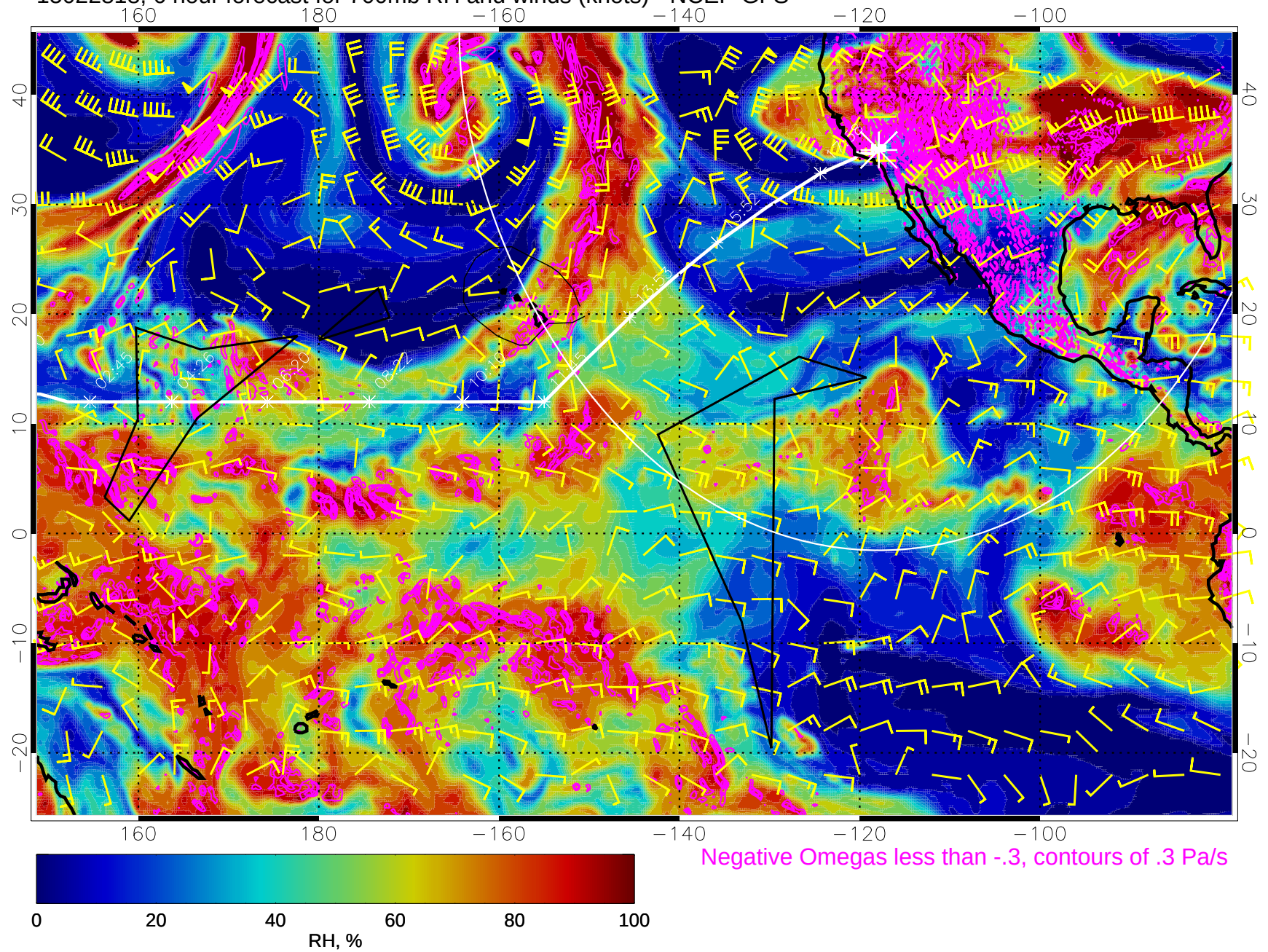
15022818, 6 hour forecast for 700mb RH and winds (knots) - NCEP GFS
