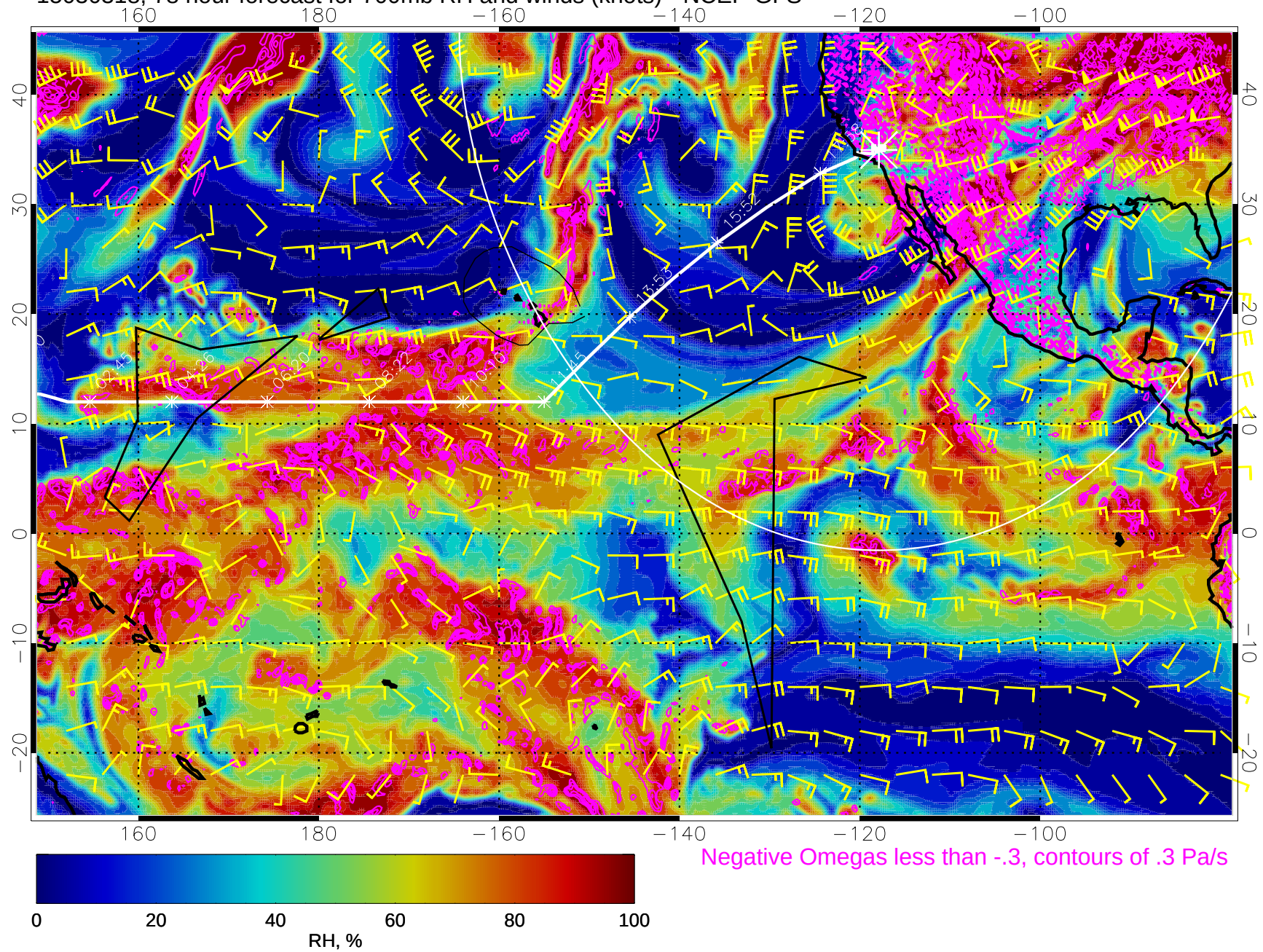
15030318, 78 hour forecast for 700mb RH and winds (knots) - NCEP GFS
