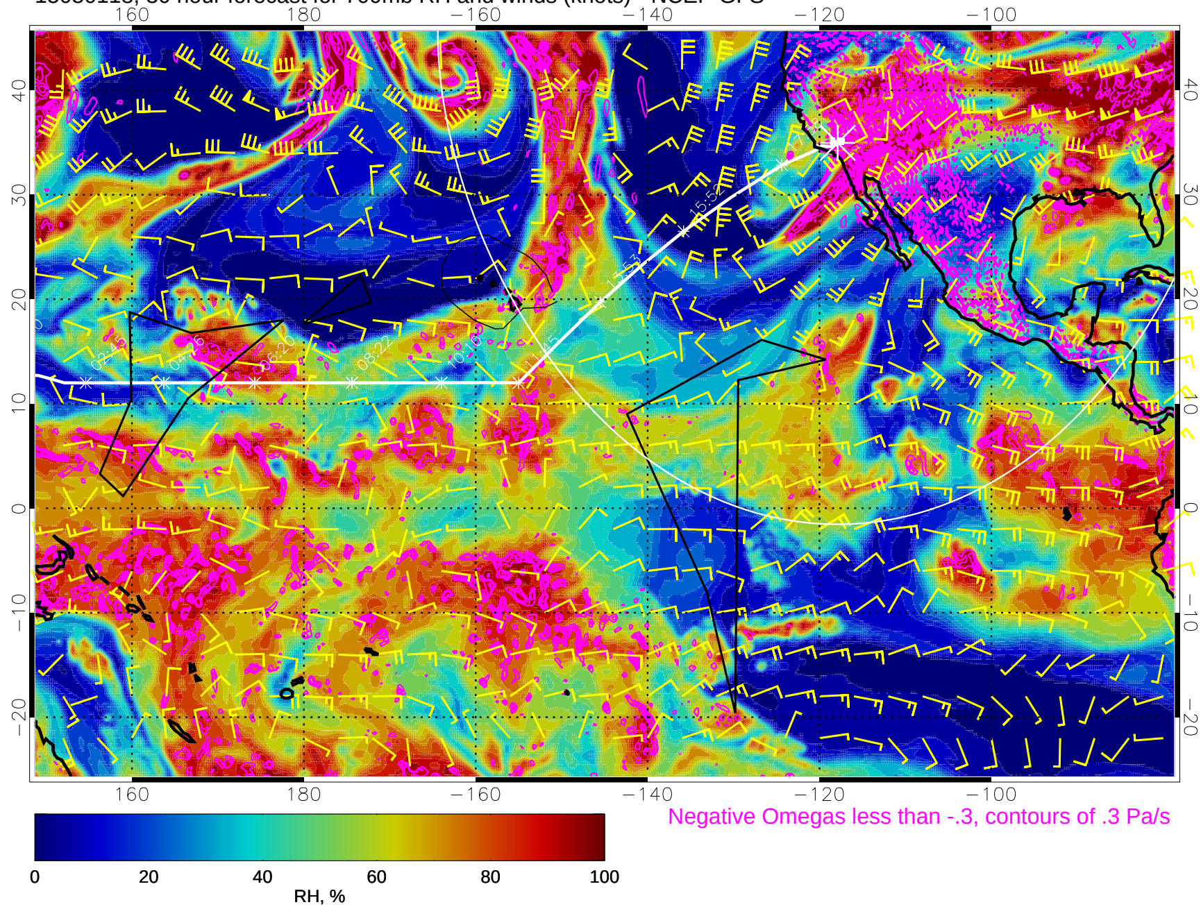
15030118, 30 hour forecast for 700mb RH and winds (knots) - NCEP GFS
