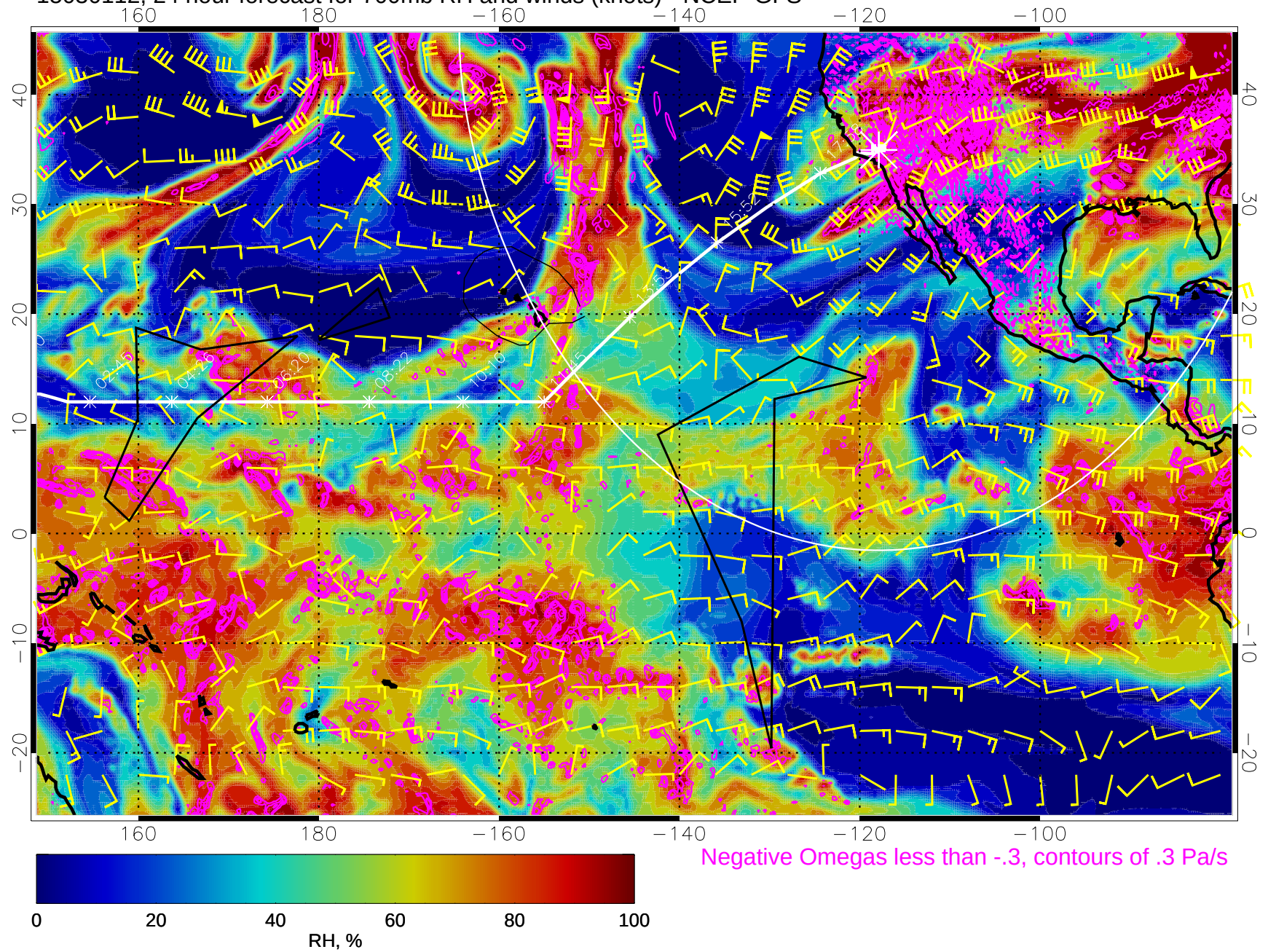
15030112, 24 hour forecast for 700mb RH and winds (knots) - NCEP GFS
