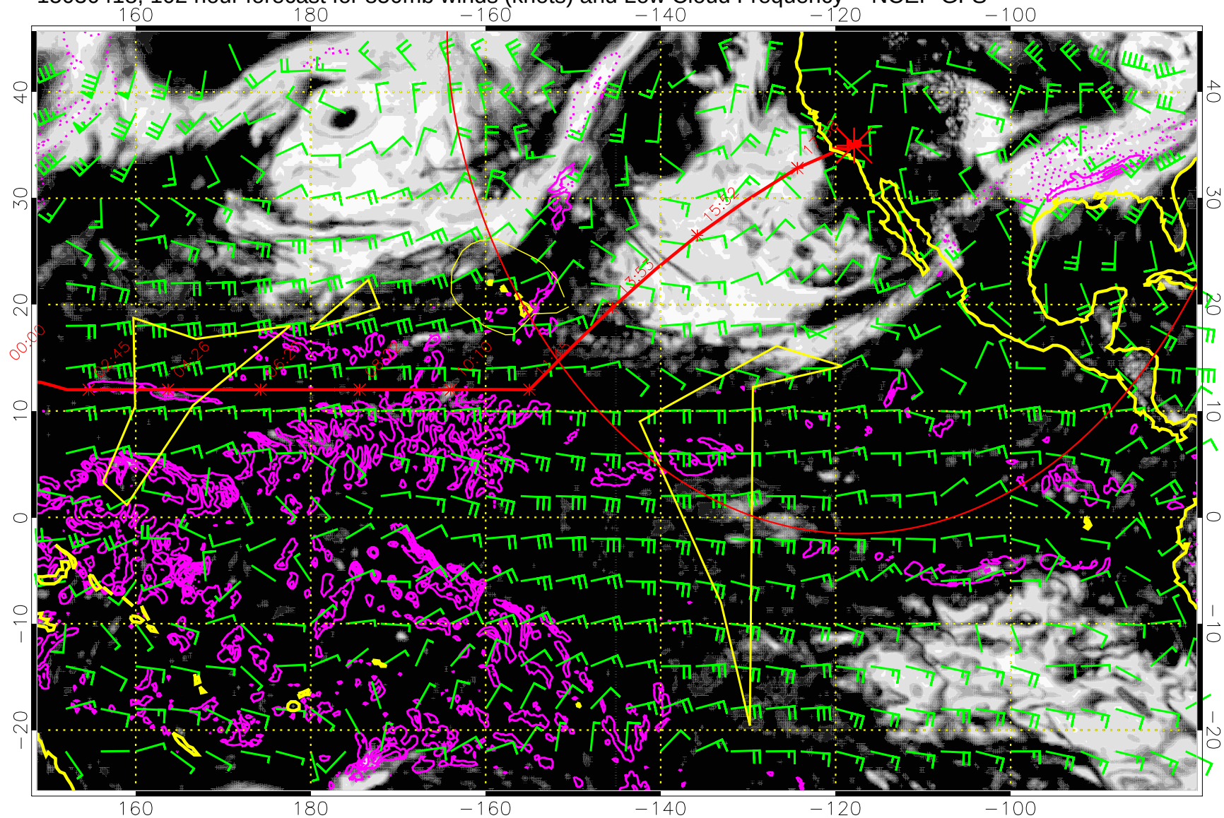
15030418, 102 hour forecast for 850mb winds (knots) and Low Cloud Frequency -- NCEP GFS
