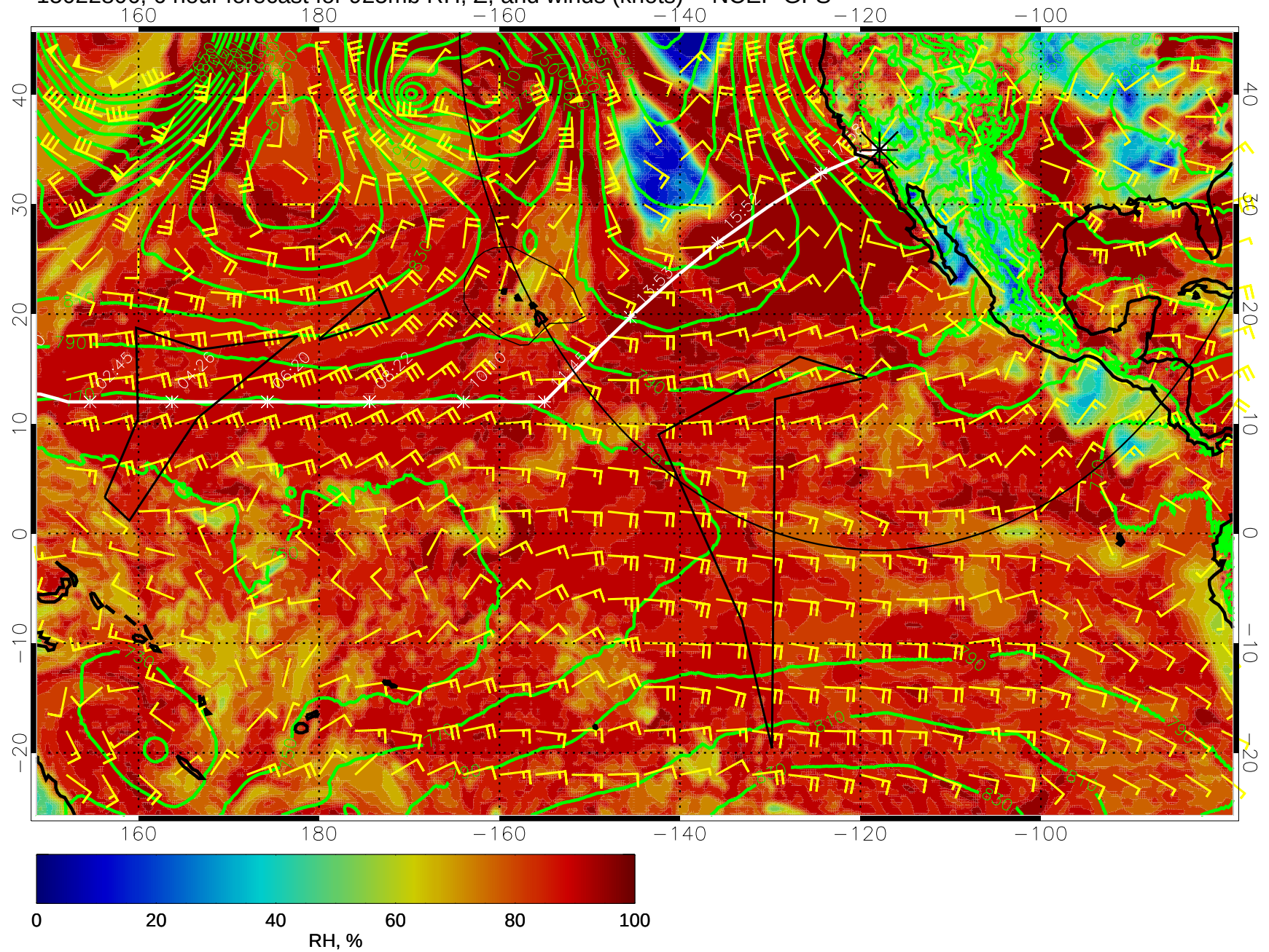
15022806, 6 hour forecast for 925mb RH, Z, and winds (knots) -- NCEP GFS
