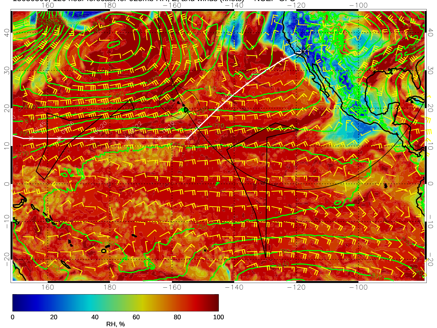
15030500, 120 hour forecast for 925mb RH, Z, and winds (knots) -- NCEP GFS
