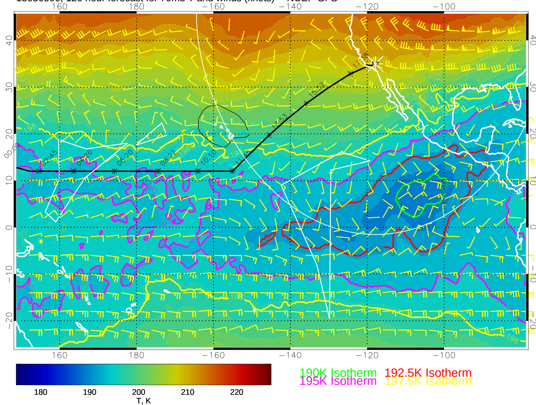
15030500, 120 hour forecast for 70mb T and winds (knots) -- NCEP GFS
