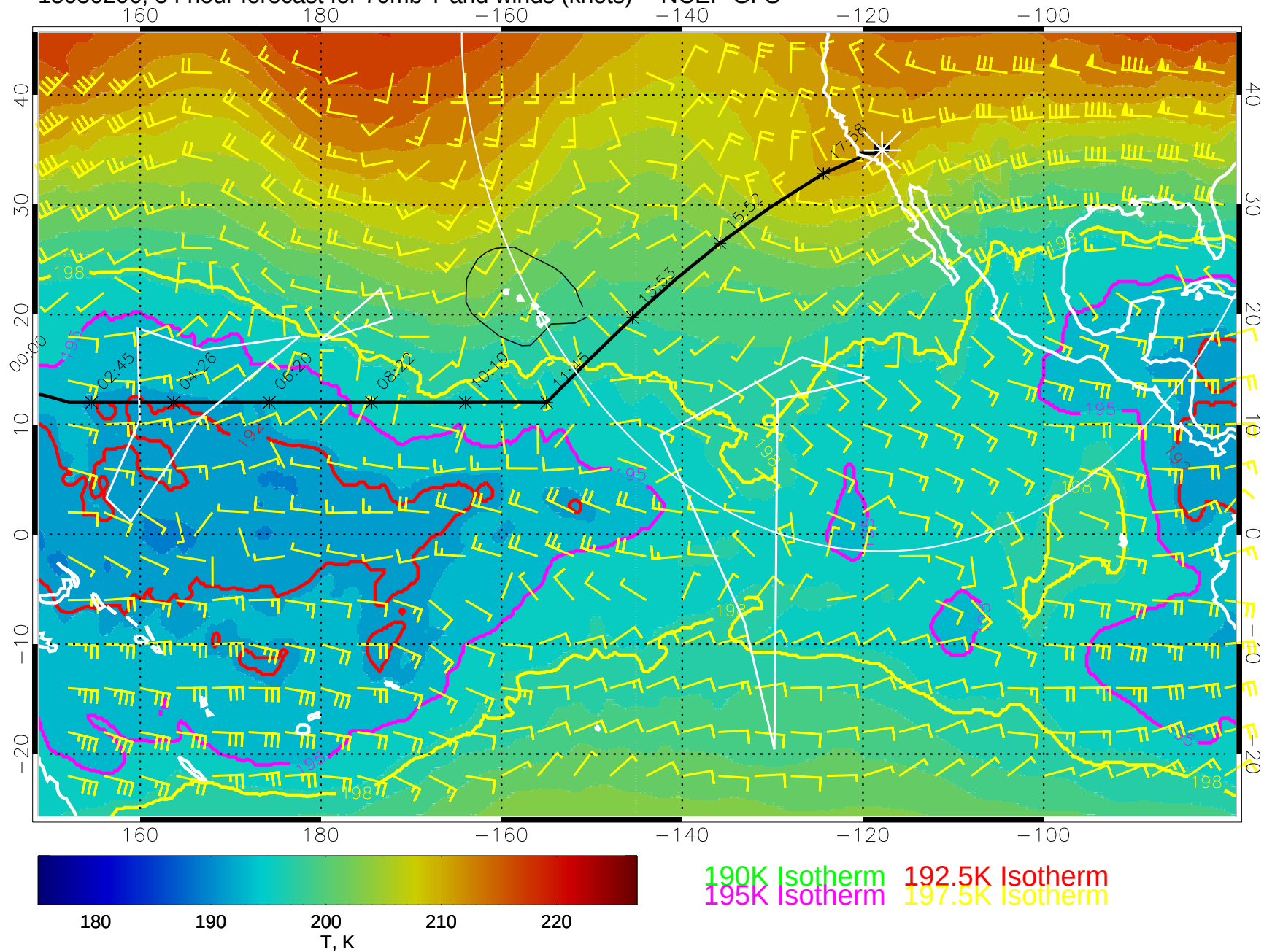
15030206, 54 hour forecast for 70mb T and winds (knots) -- NCEP GFS
