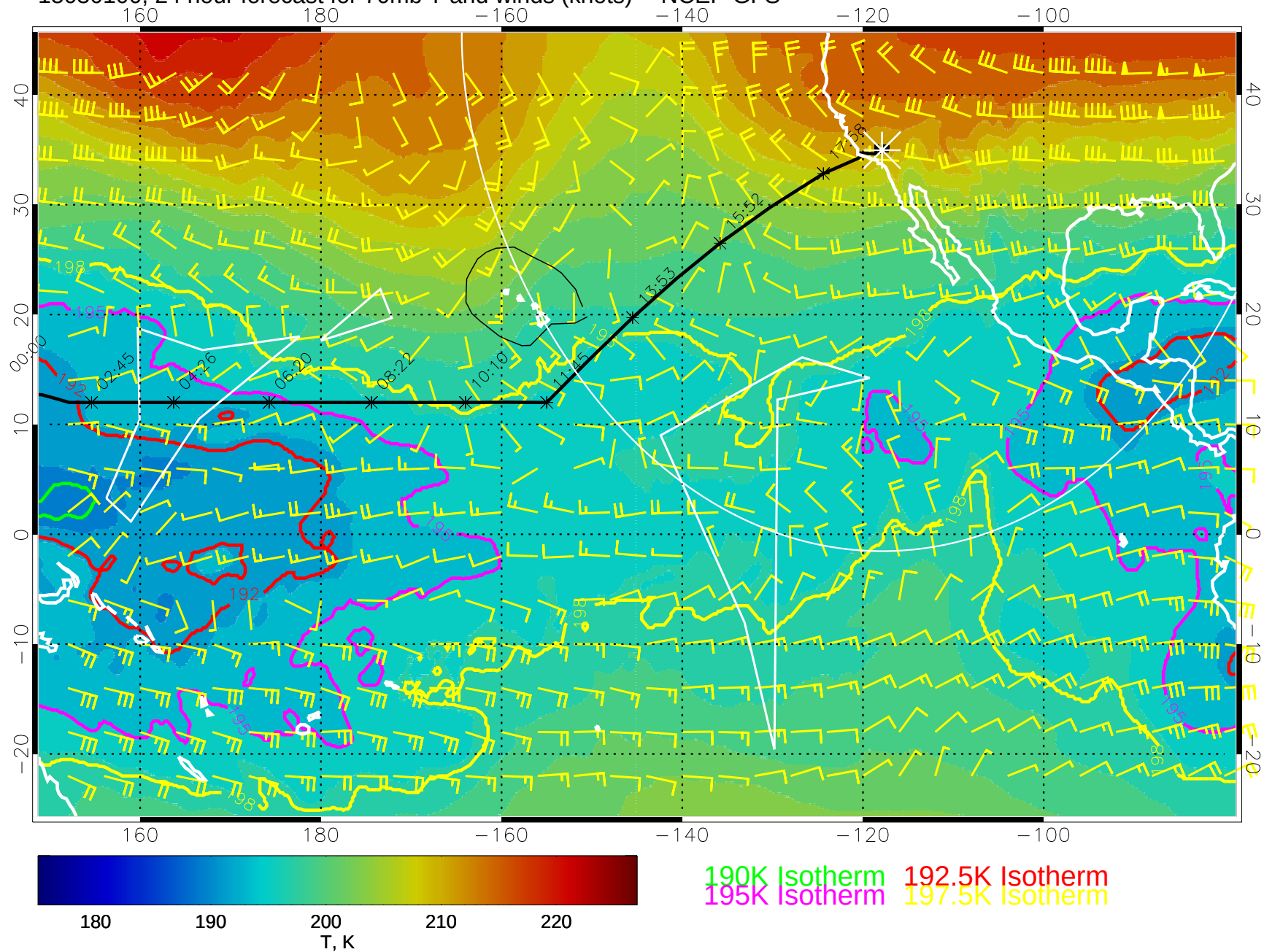
15030100, 24 hour forecast for 70mb T and winds (knots) -- NCEP GFS
