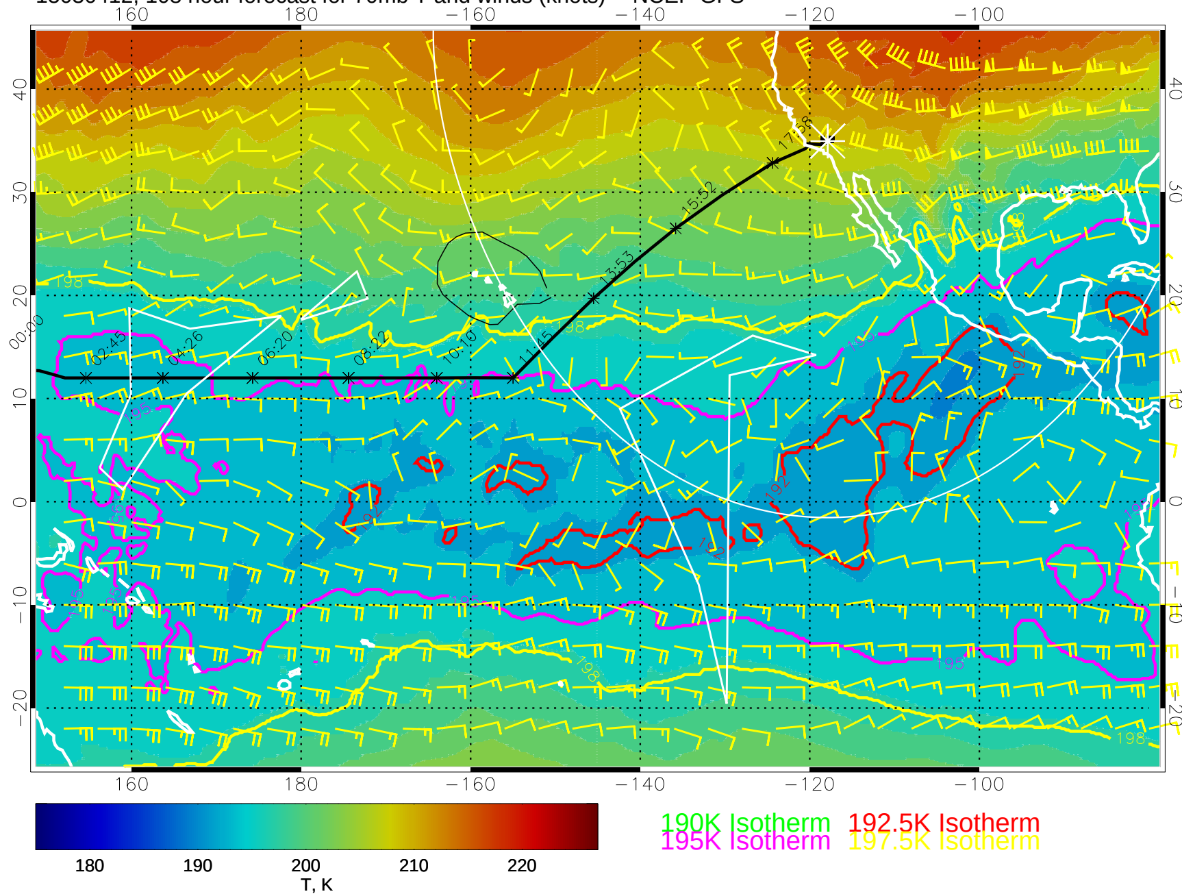
15030412, 108 hour forecast for 70mb T and winds (knots) -- NCEP GFS
