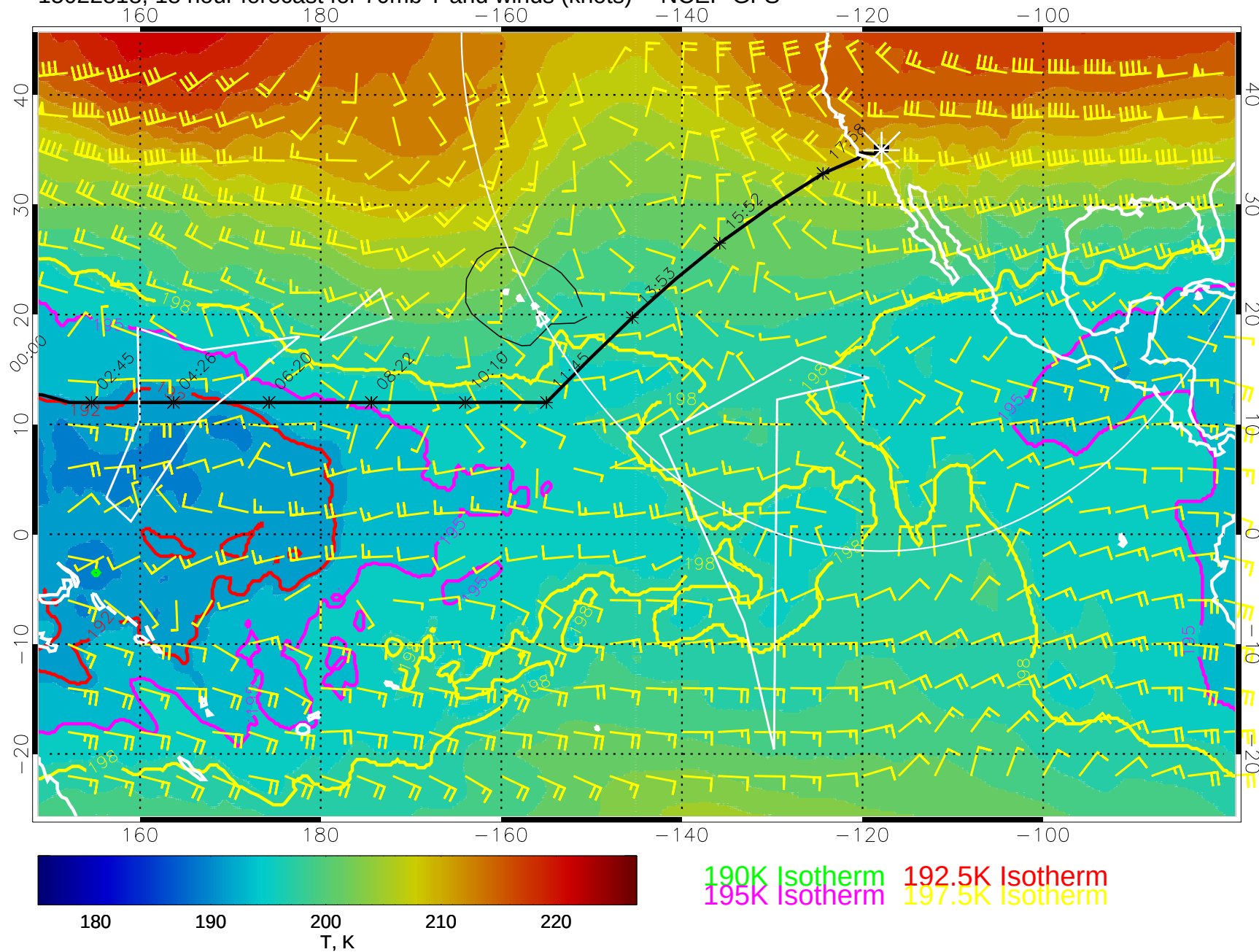
15022818, 18 hour forecast for 70mb T and winds (knots) -- NCEP GFS
