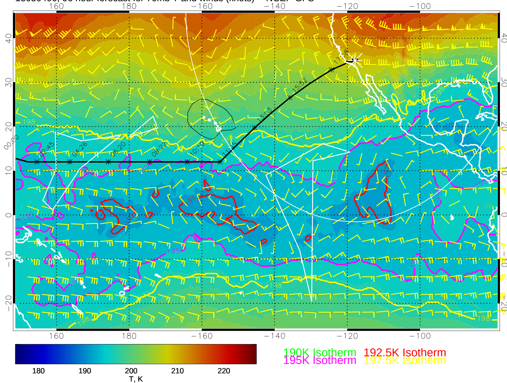
15030400, 96 hour forecast for 70mb T and winds (knots) -- NCEP GFS
