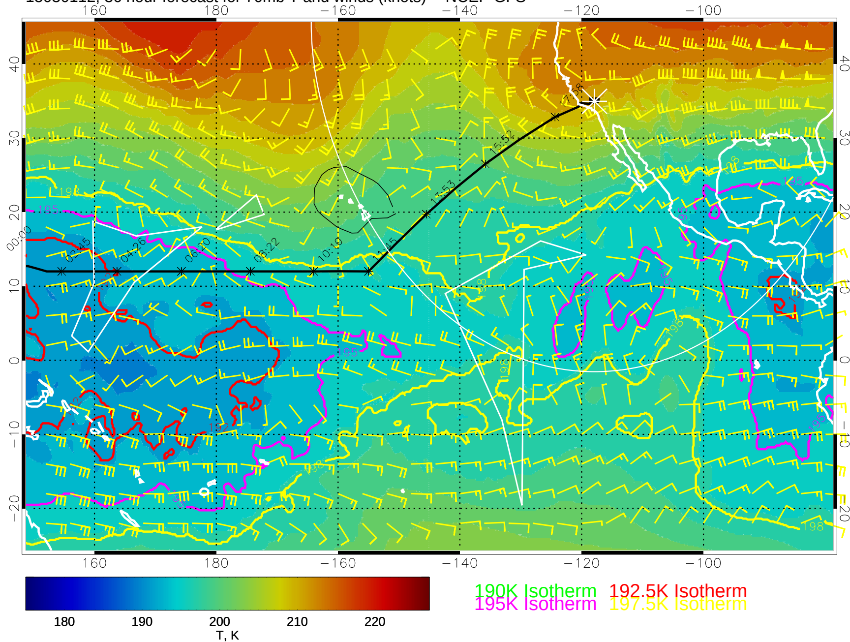
15030112, 36 hour forecast for 70mb T and winds (knots) -- NCEP GFS
