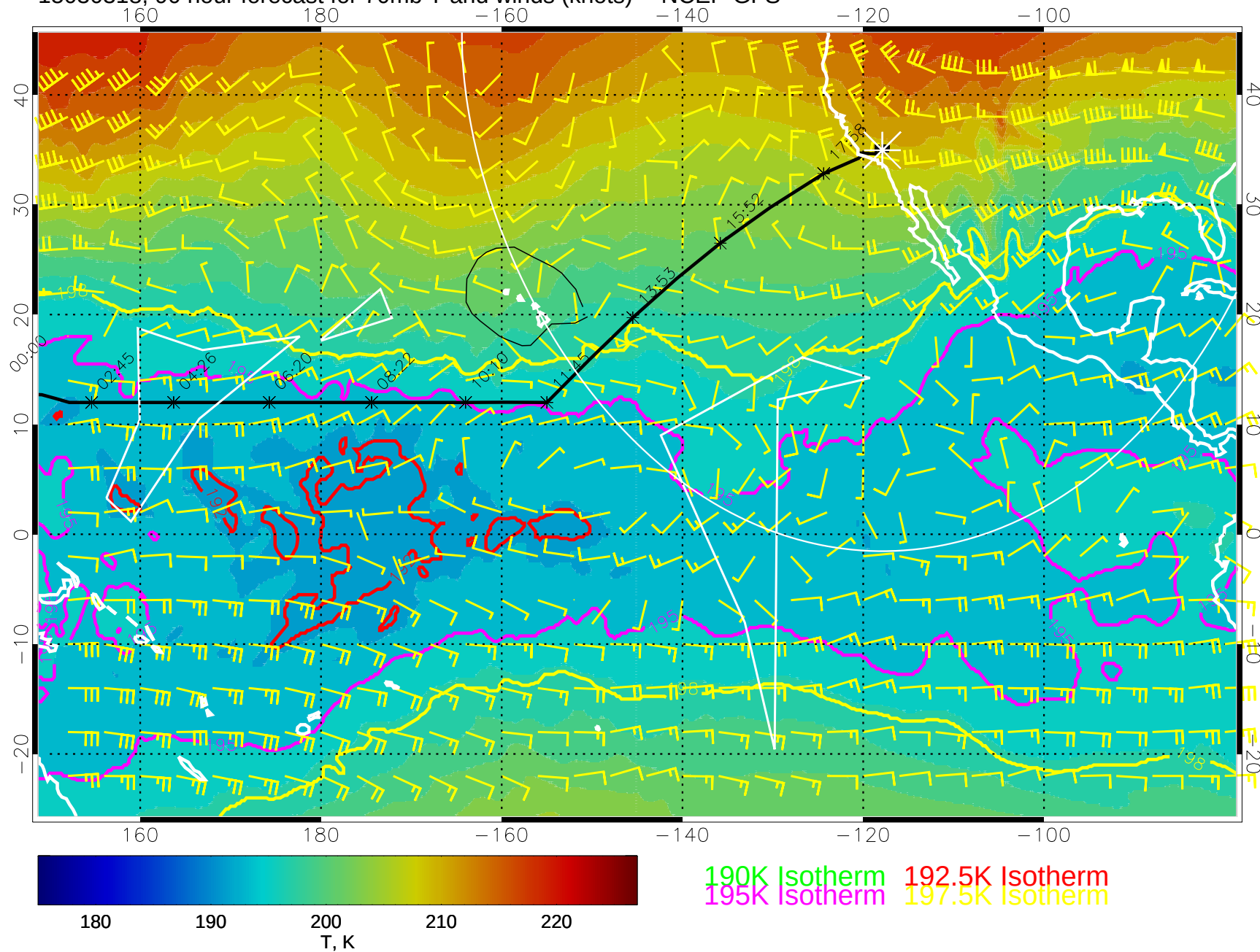
15030318, 90 hour forecast for 70mb T and winds (knots) -- NCEP GFS
