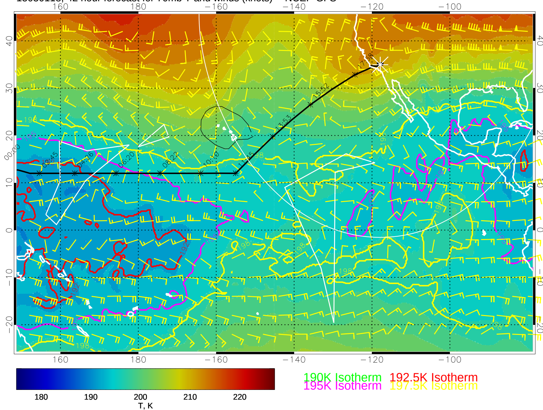
15030118, 42 hour forecast for 70mb T and winds (knots) -- NCEP GFS
