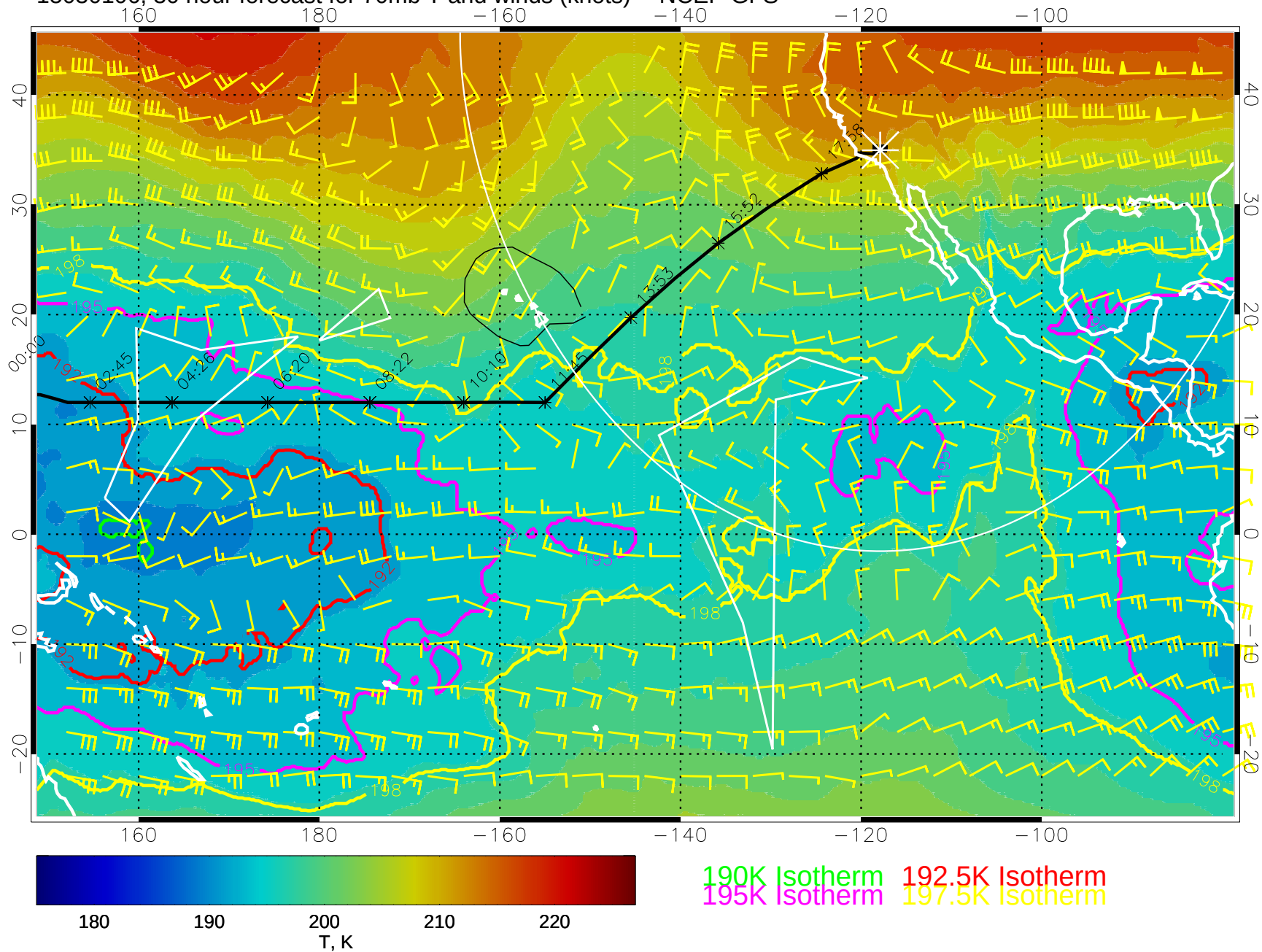
15030106, 30 hour forecast for 70mb T and winds (knots) -- NCEP GFS
