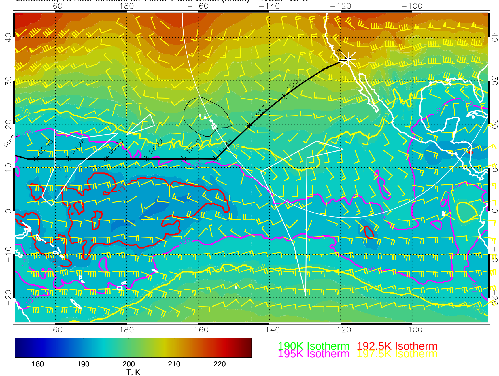
15030306, 78 hour forecast for 70mb T and winds (knots) -- NCEP GFS
