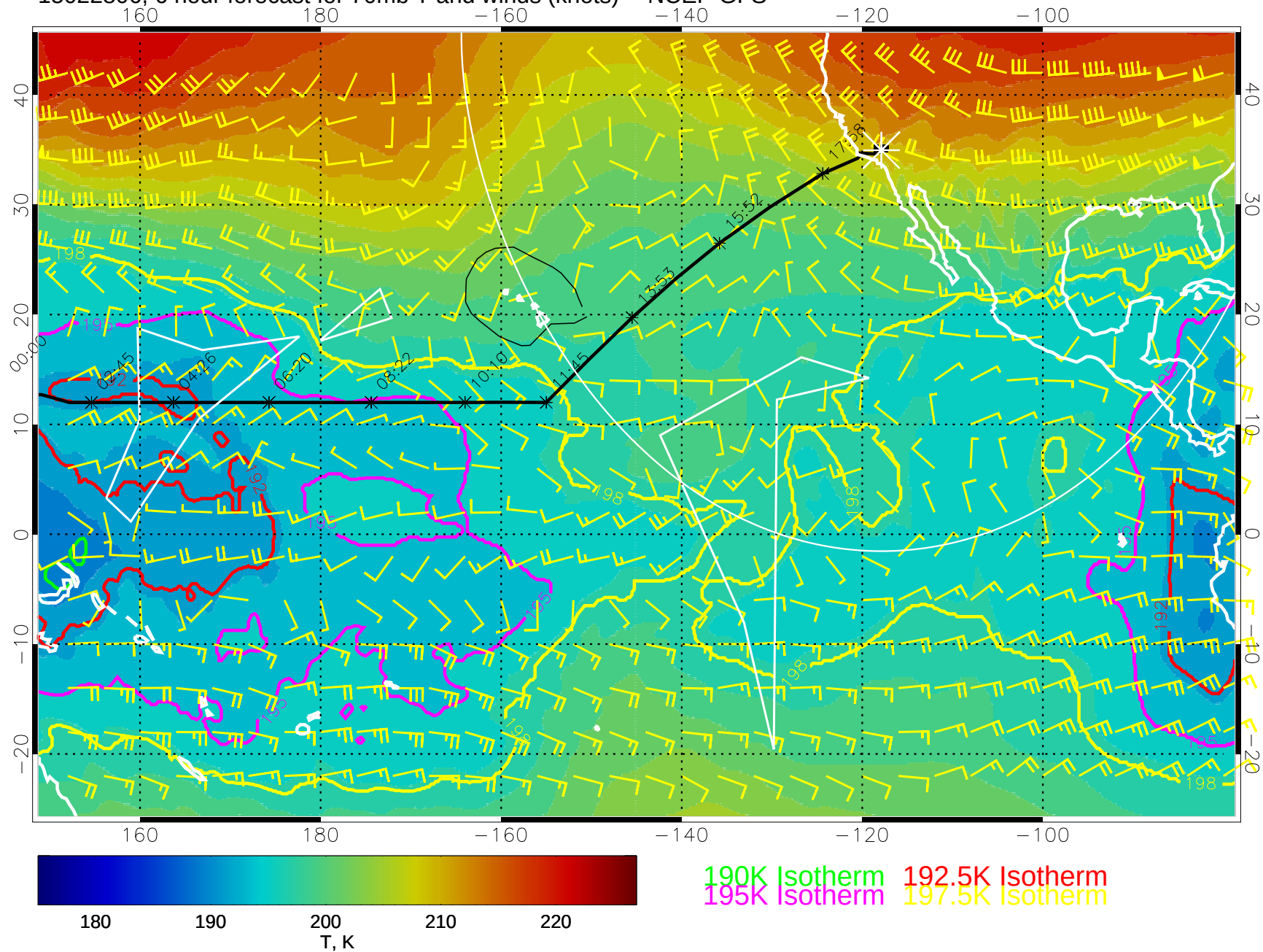
15022806, 6 hour forecast for 70mb T and winds (knots) -- NCEP GFS
