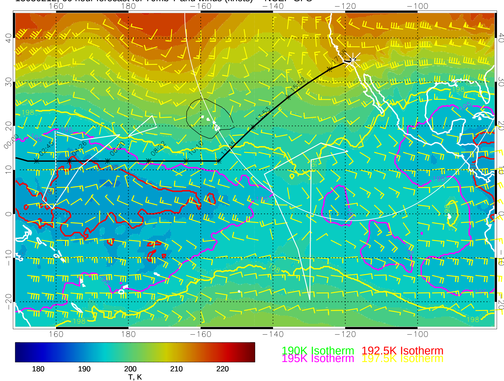
15030212, 60 hour forecast for 70mb T and winds (knots) -- NCEP GFS
