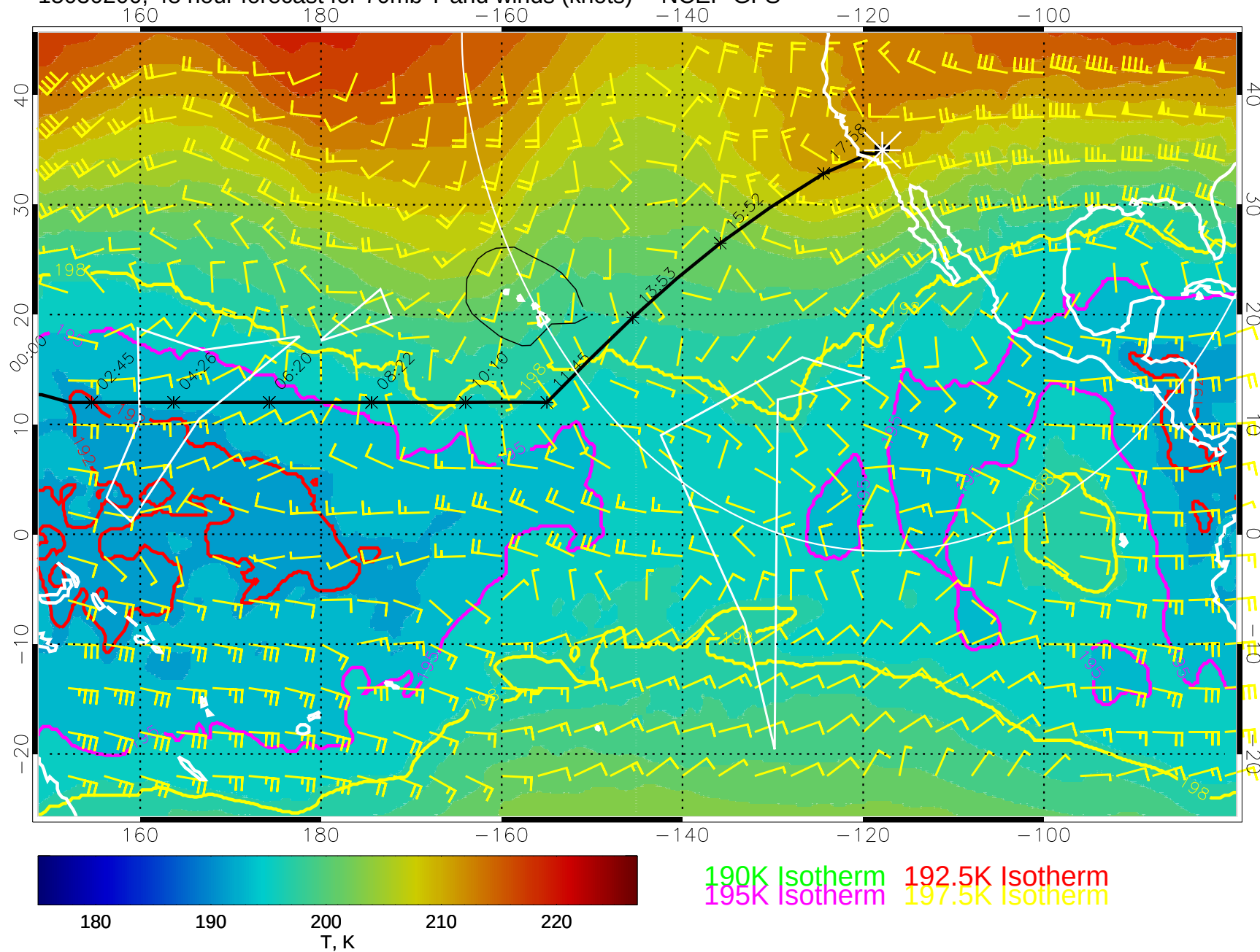
15030200, 48 hour forecast for 70mb T and winds (knots) -- NCEP GFS
