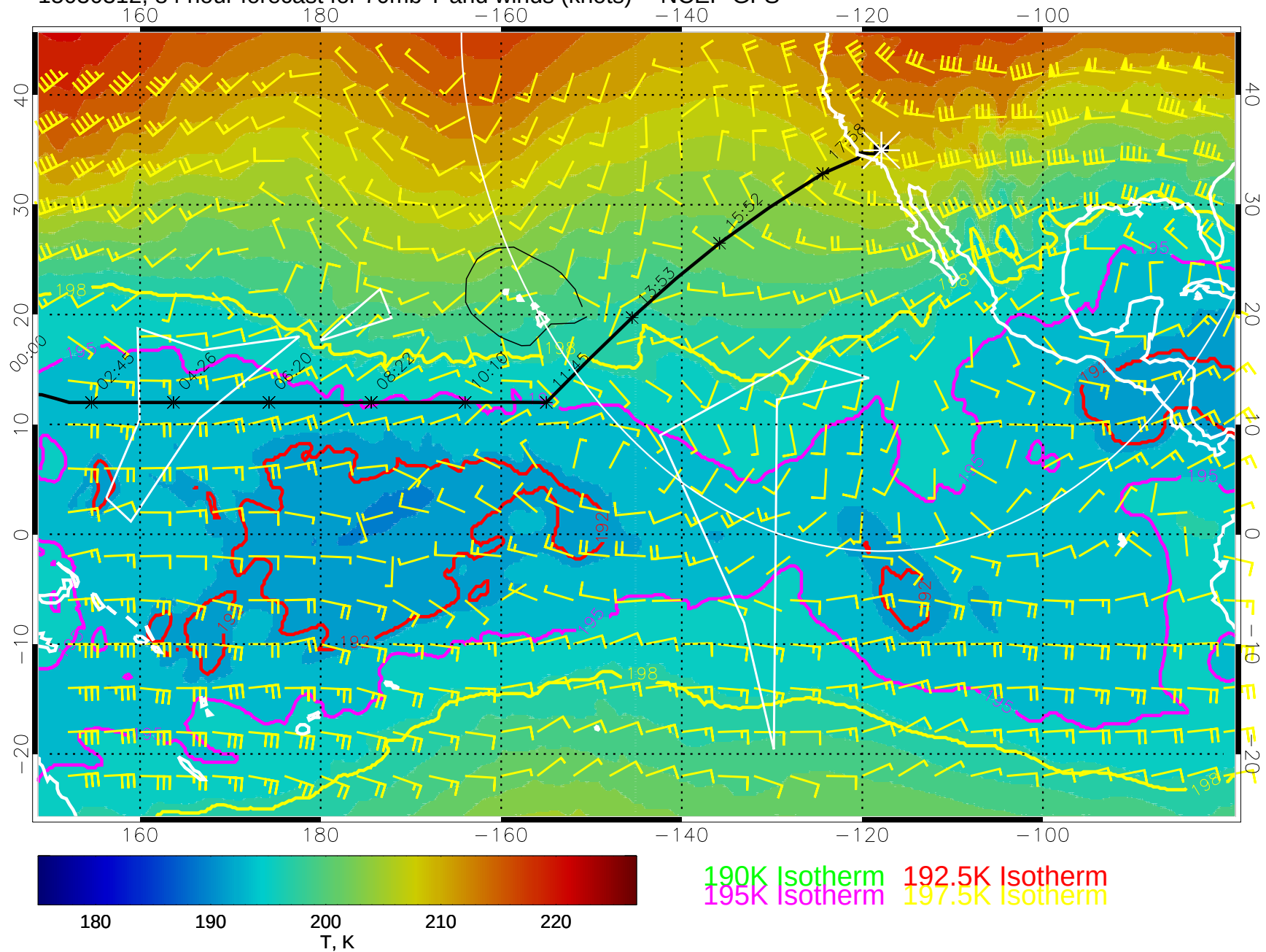
15030312, 84 hour forecast for 70mb T and winds (knots) -- NCEP GFS
