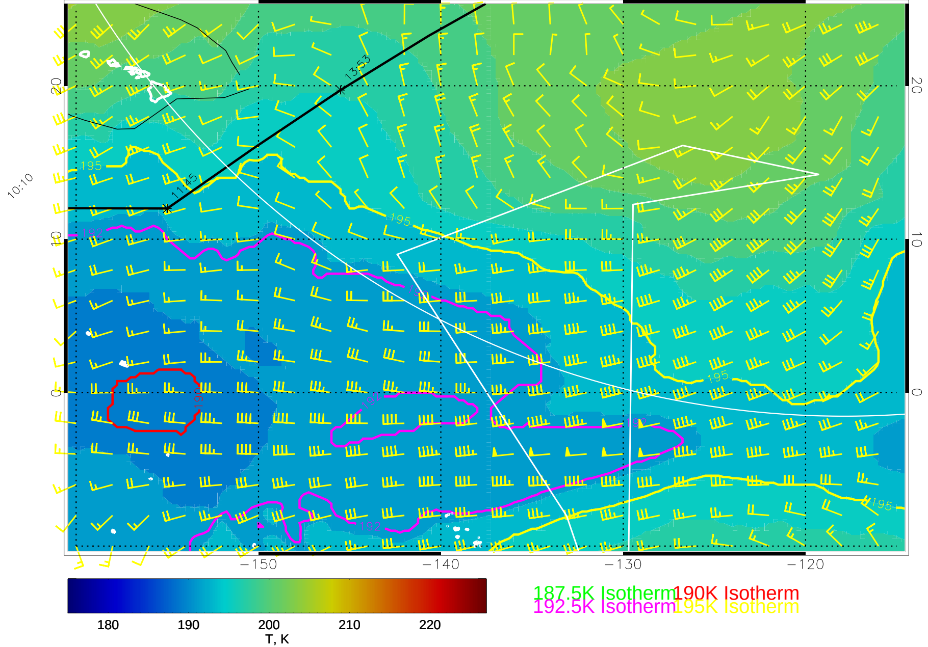
15022818, 18 hour forecast for 100mb T and winds (knots) -- NCEP GFS
