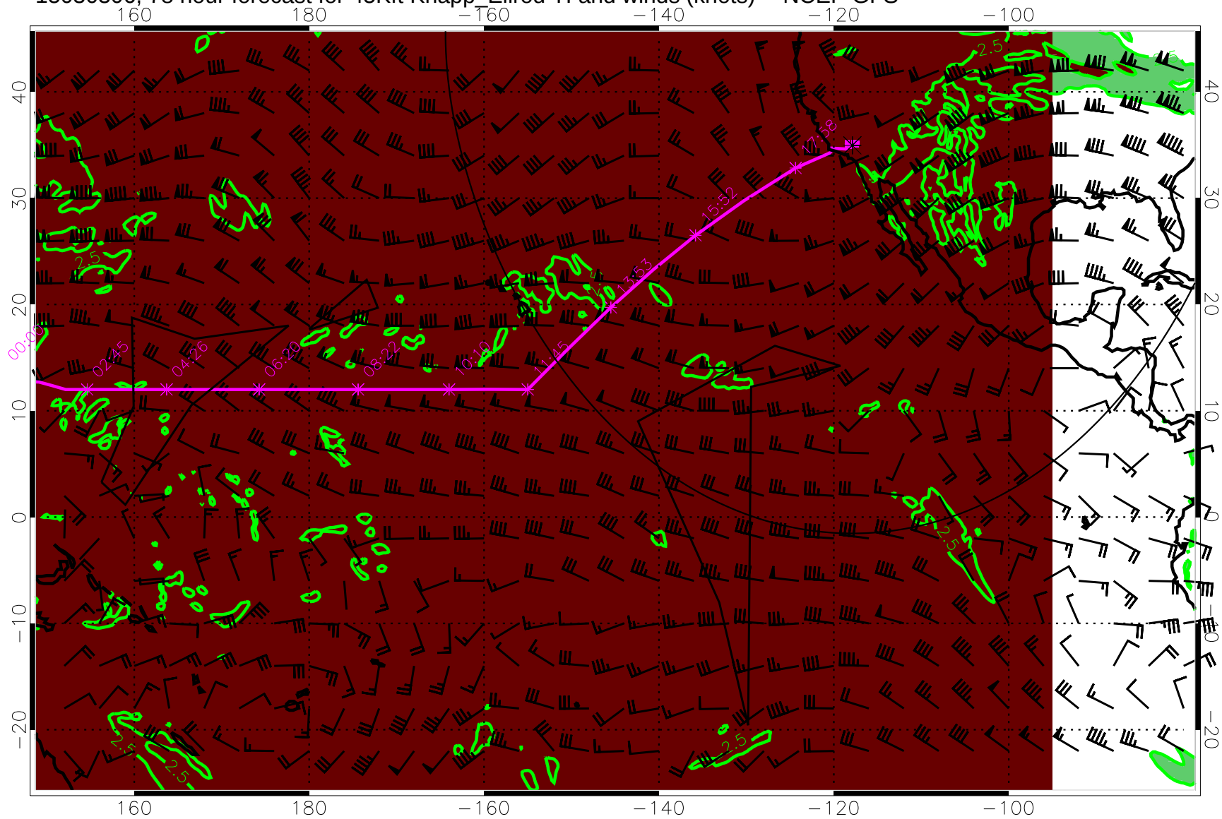
15030306, 78 hour forecast for 45Kft Knapp_Ellrod TI and winds (knots) -- NCEP GFS
