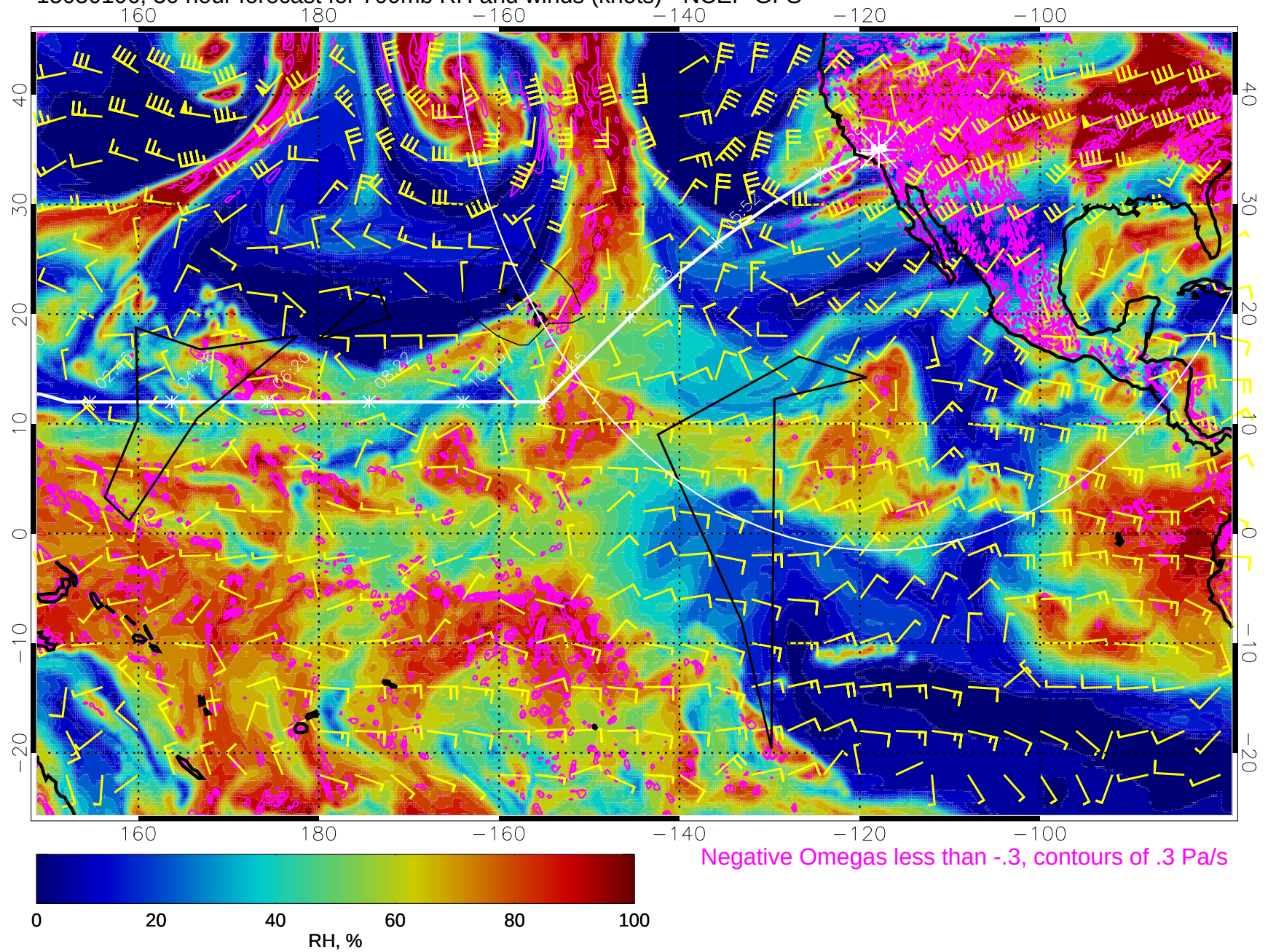
15030106, 30 hour forecast for 700mb RH and winds (knots) - NCEP GFS
