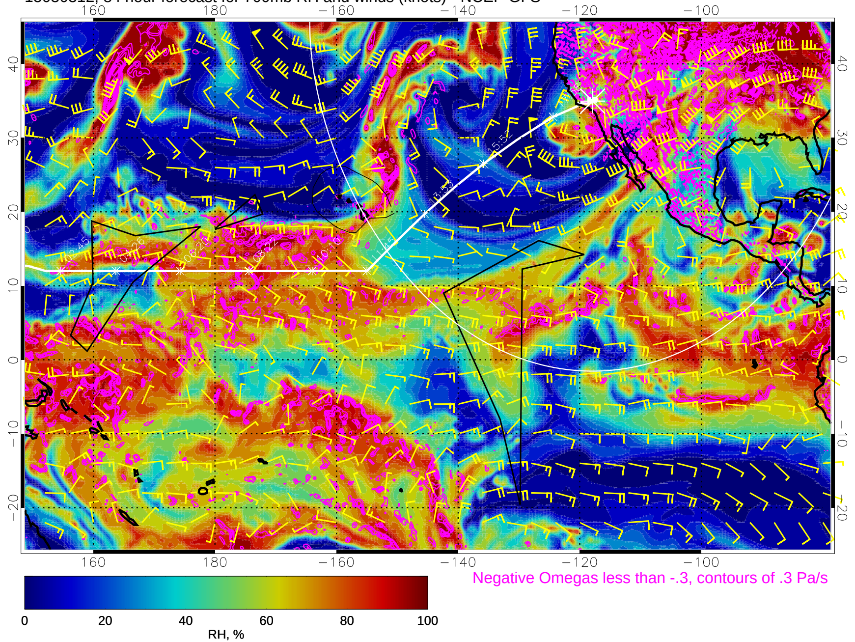
15030312, 84 hour forecast for 700mb RH and winds (knots) - NCEP GFS
