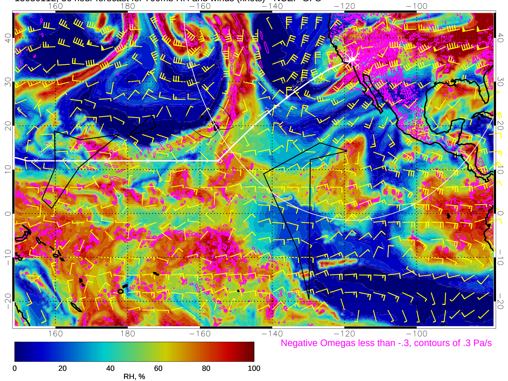
15030112, 36 hour forecast for 700mb RH and winds (knots) - NCEP GFS
