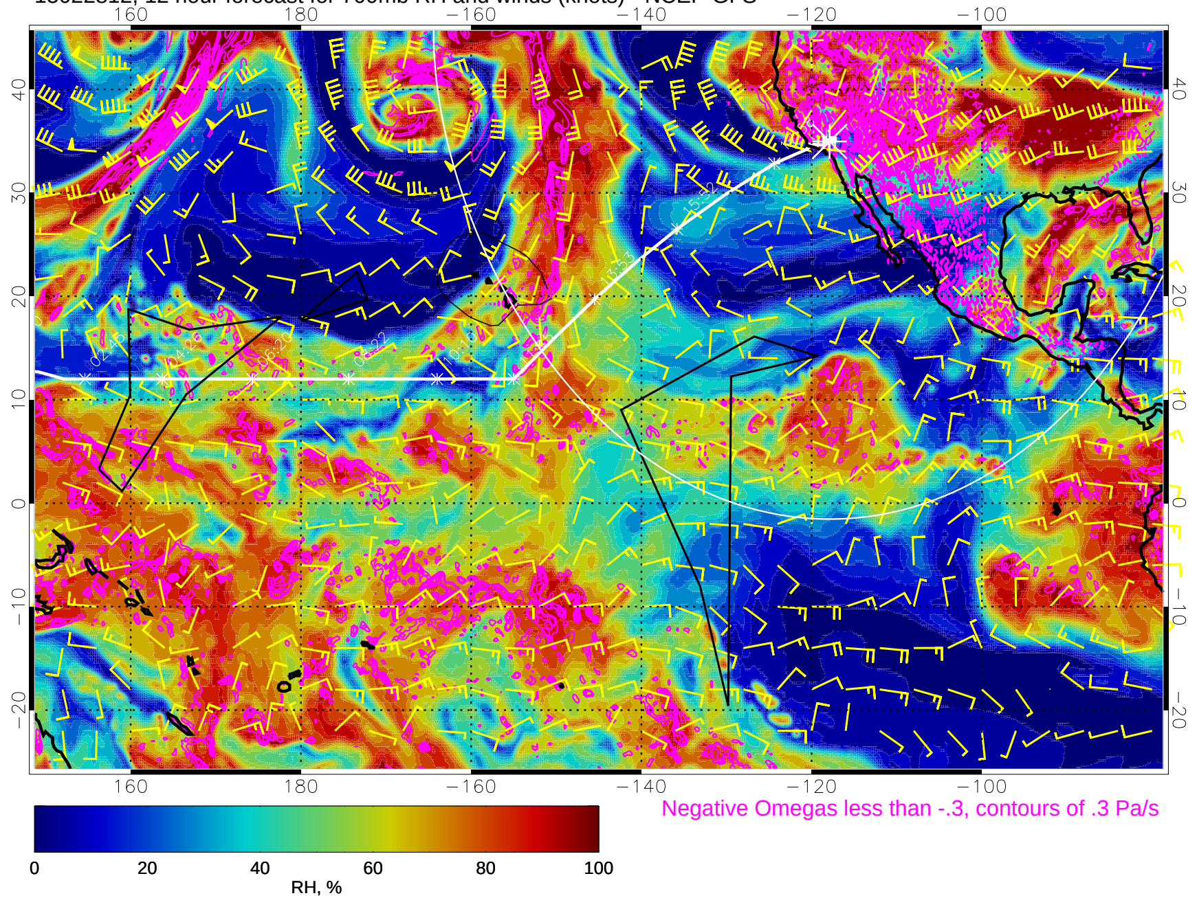
15022812, 12 hour forecast for 700mb RH and winds (knots) - NCEP GFS
