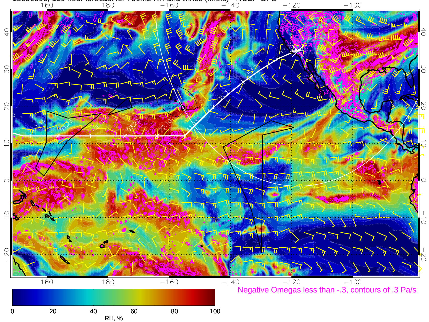
15030500, 120 hour forecast for 700mb RH and winds (knots) - NCEP GFS
