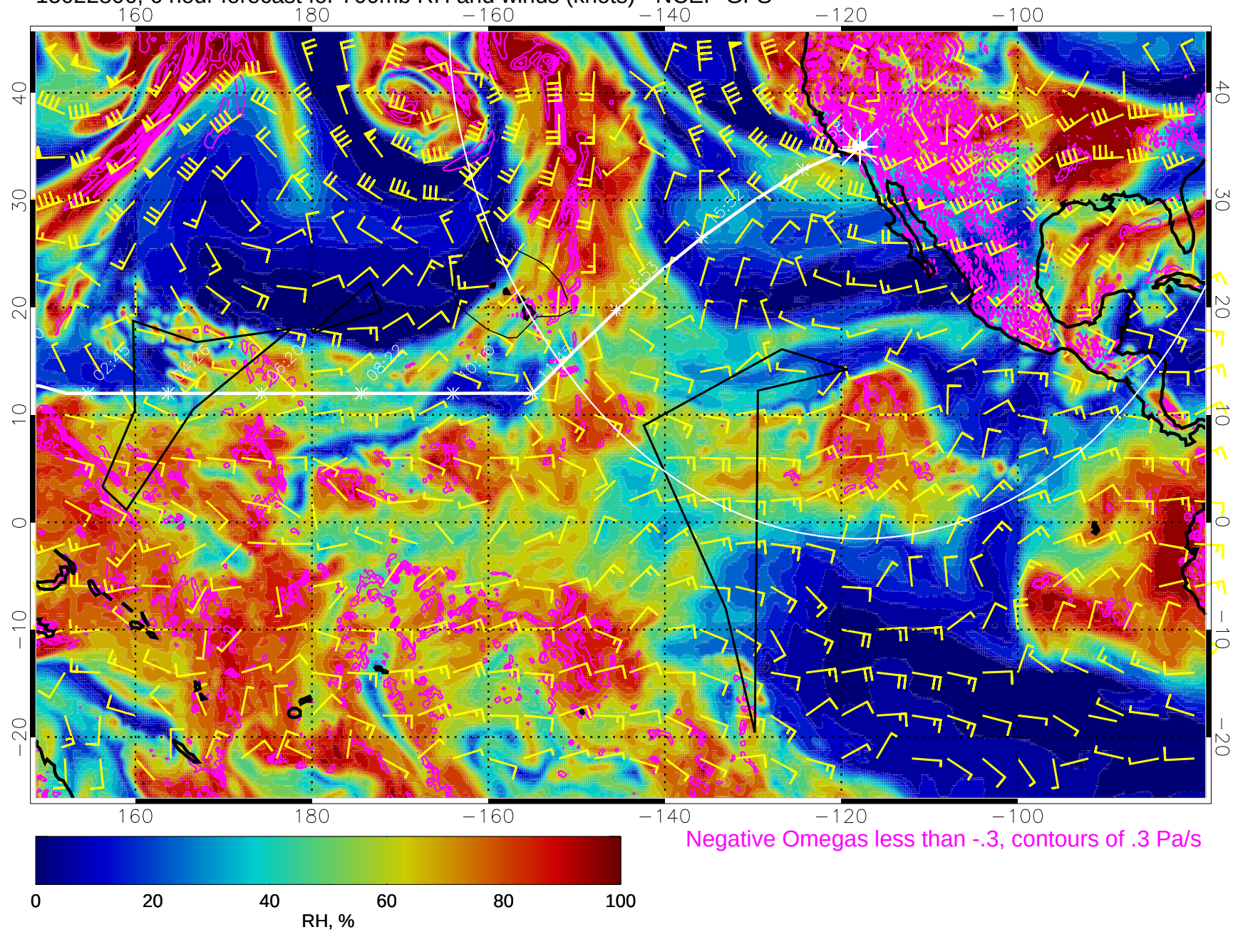
15022806, 6 hour forecast for 700mb RH and winds (knots) - NCEP GFS
