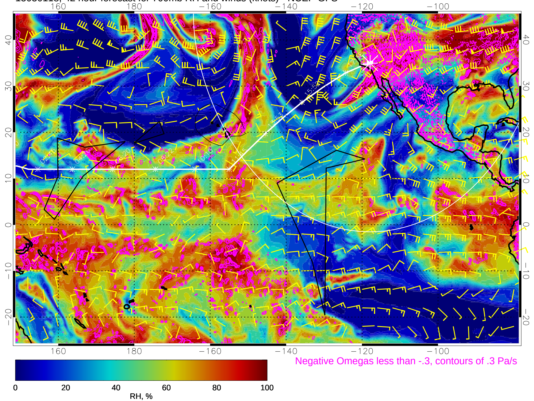
15030118, 42 hour forecast for 700mb RH and winds (knots) - NCEP GFS
