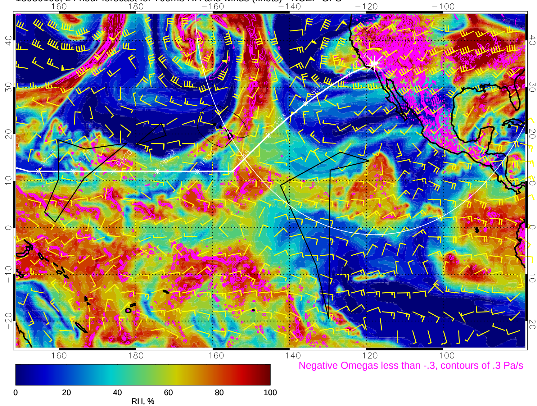
15030100, 24 hour forecast for 700mb RH and winds (knots) - NCEP GFS
