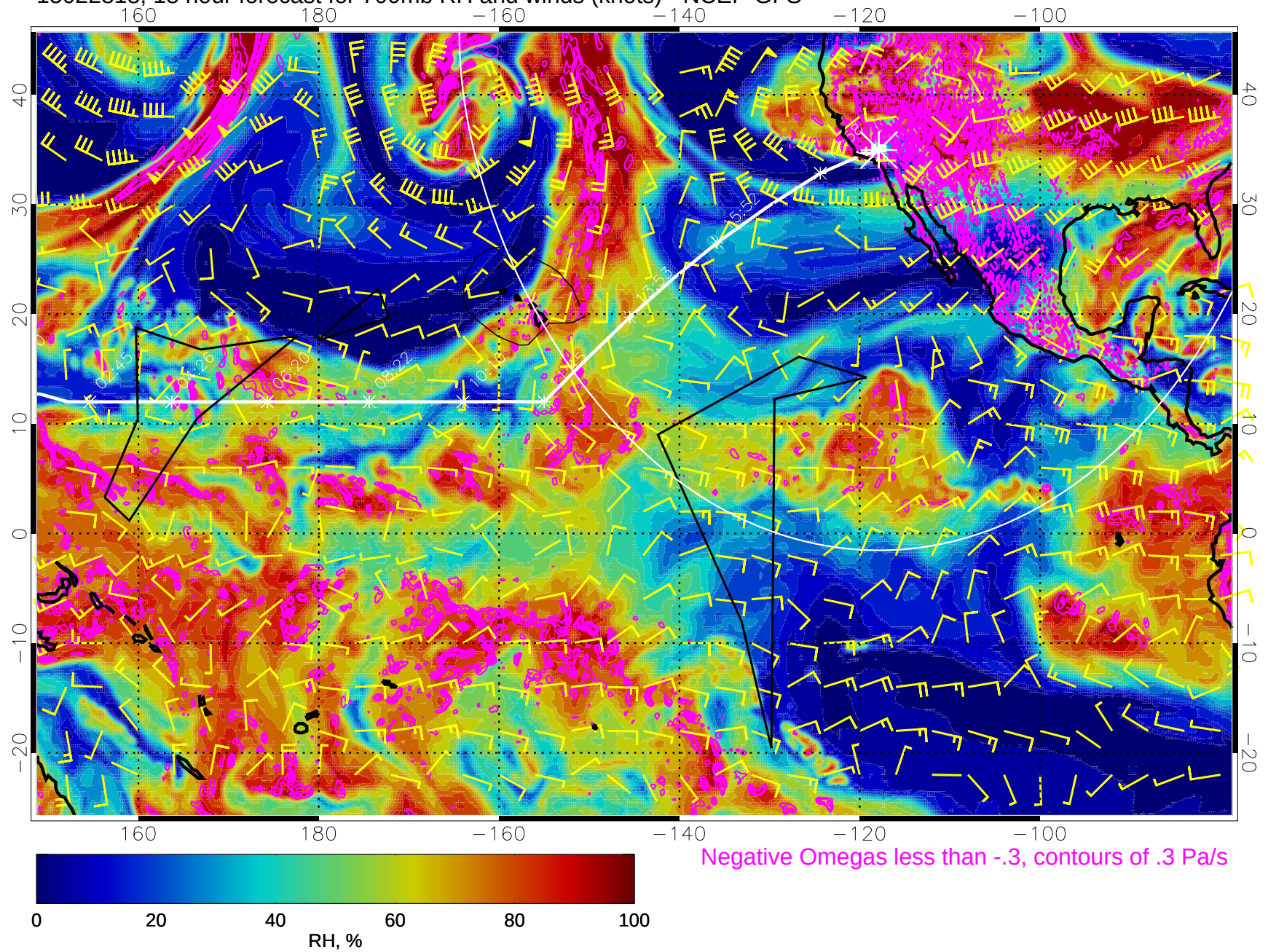
15022818, 18 hour forecast for 700mb RH and winds (knots) - NCEP GFS
