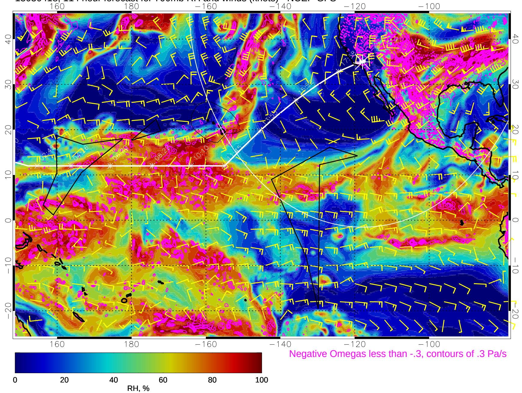
15030418, 114 hour forecast for 700mb RH and winds (knots) - NCEP GFS
