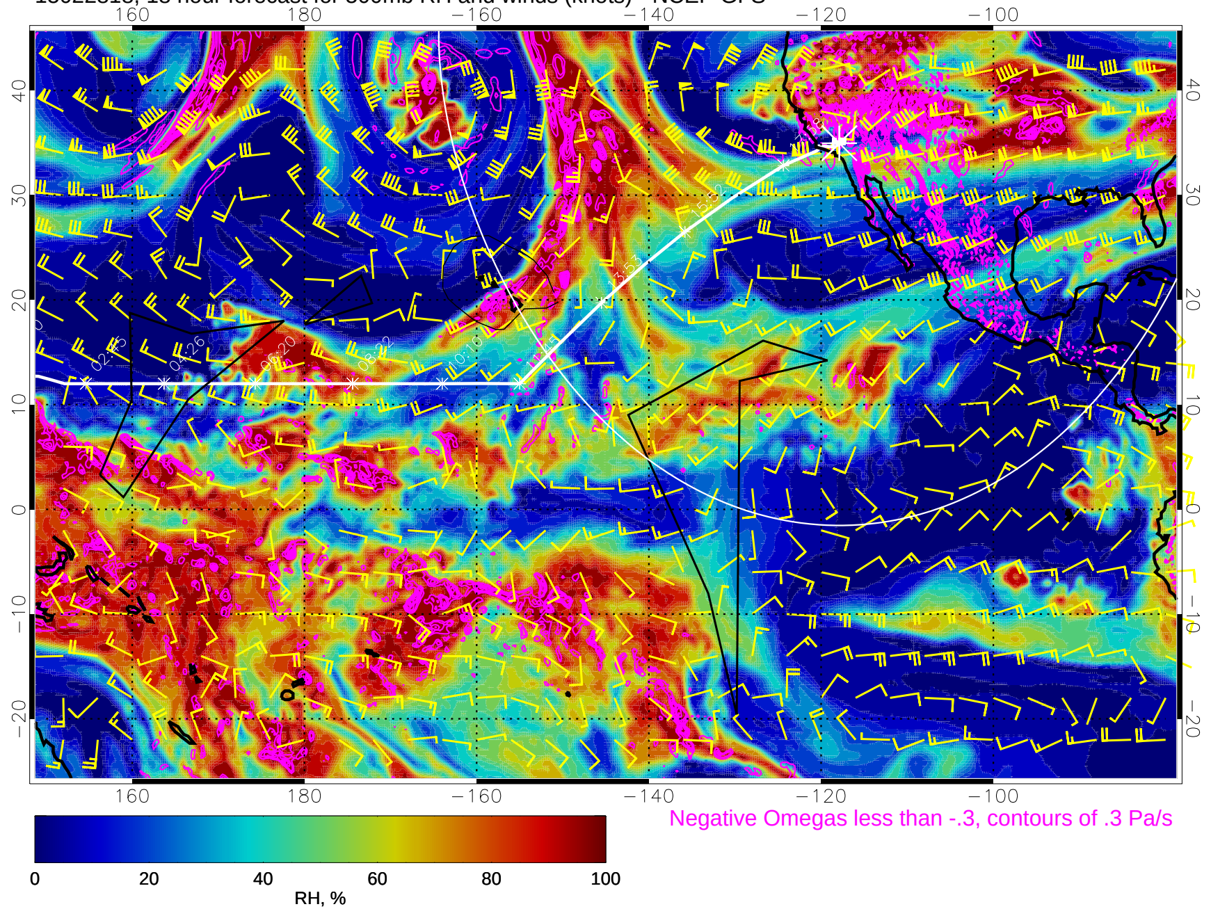
15022818, 18 hour forecast for 500mb RH and winds (knots) - NCEP GFS
