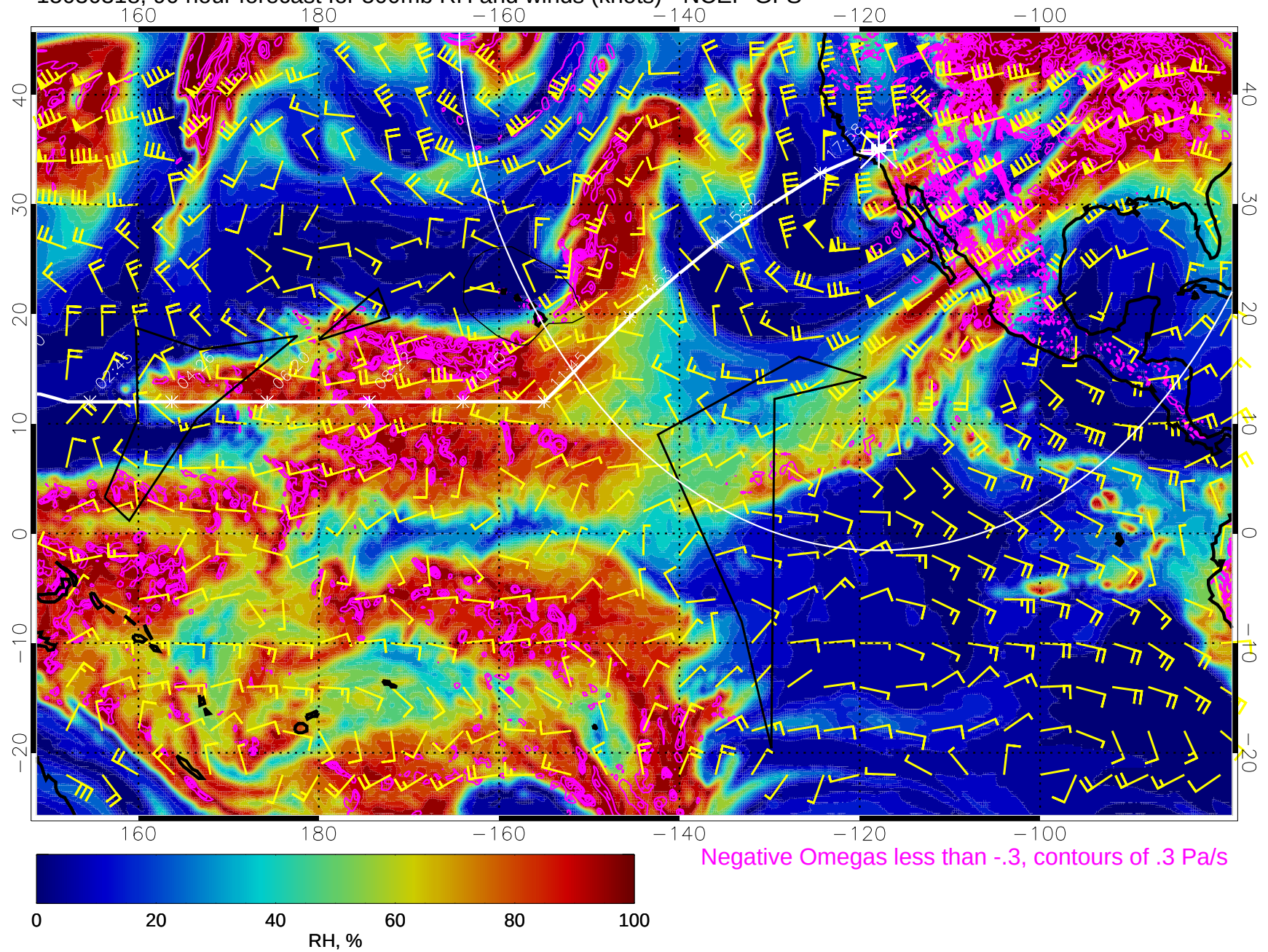
15030318, 90 hour forecast for 500mb RH and winds (knots) - NCEP GFS
