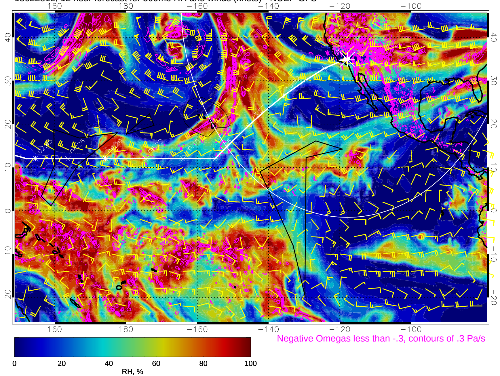
15022812, 12 hour forecast for 500mb RH and winds (knots) - NCEP GFS
