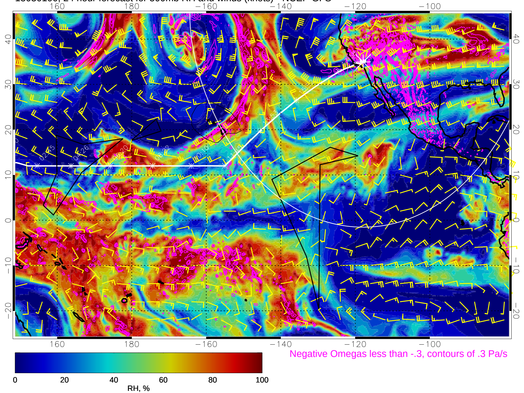
15030100, 24 hour forecast for 500mb RH and winds (knots) - NCEP GFS
