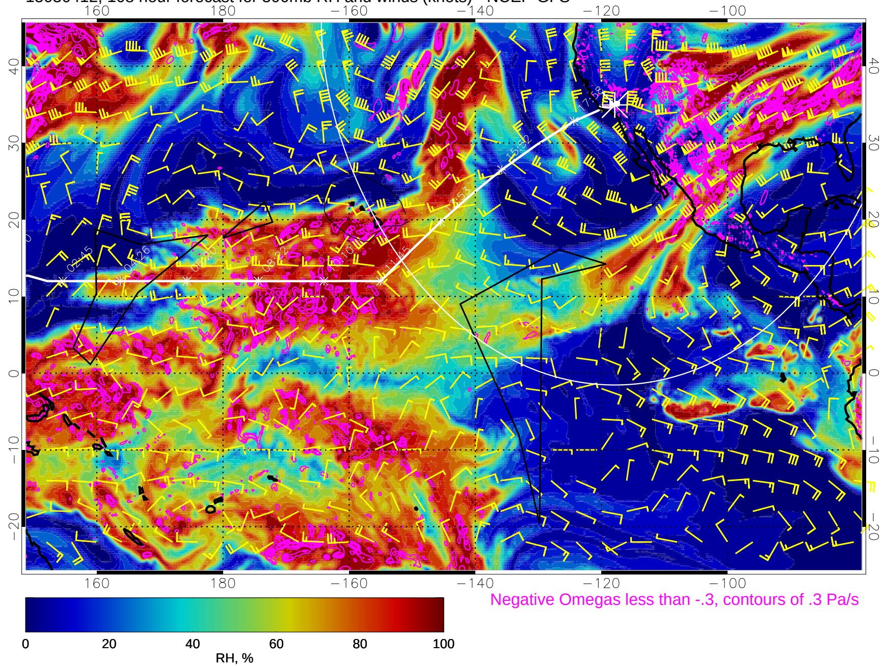
15030412, 108 hour forecast for 500mb RH and winds (knots) - NCEP GFS
