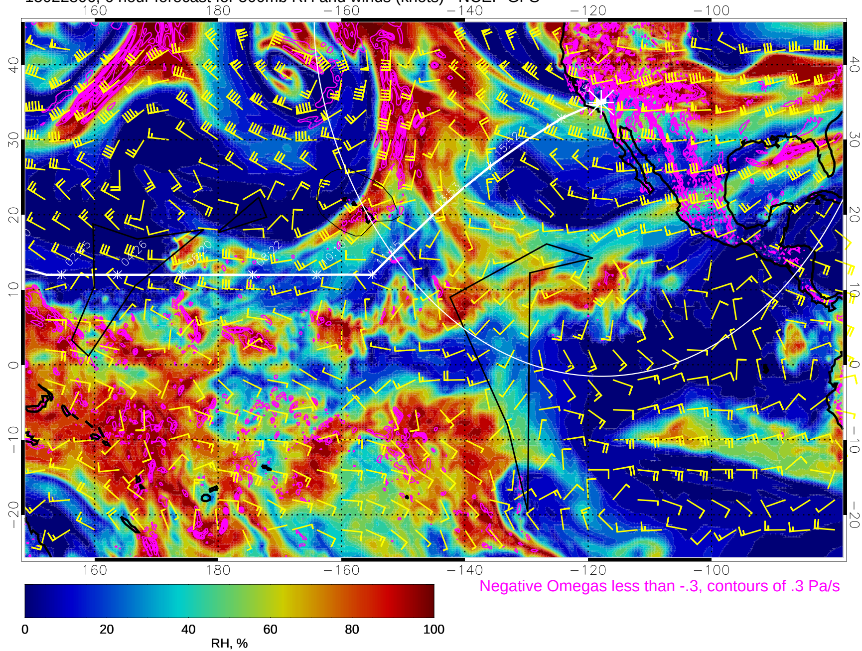
15022806, 6 hour forecast for 500mb RH and winds (knots) - NCEP GFS
