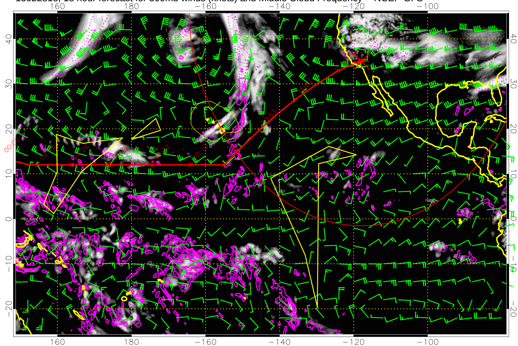
15022818, 18 hour forecast for 500mb winds (knots) and Middle Cloud Frequency -- NCEP GFS
