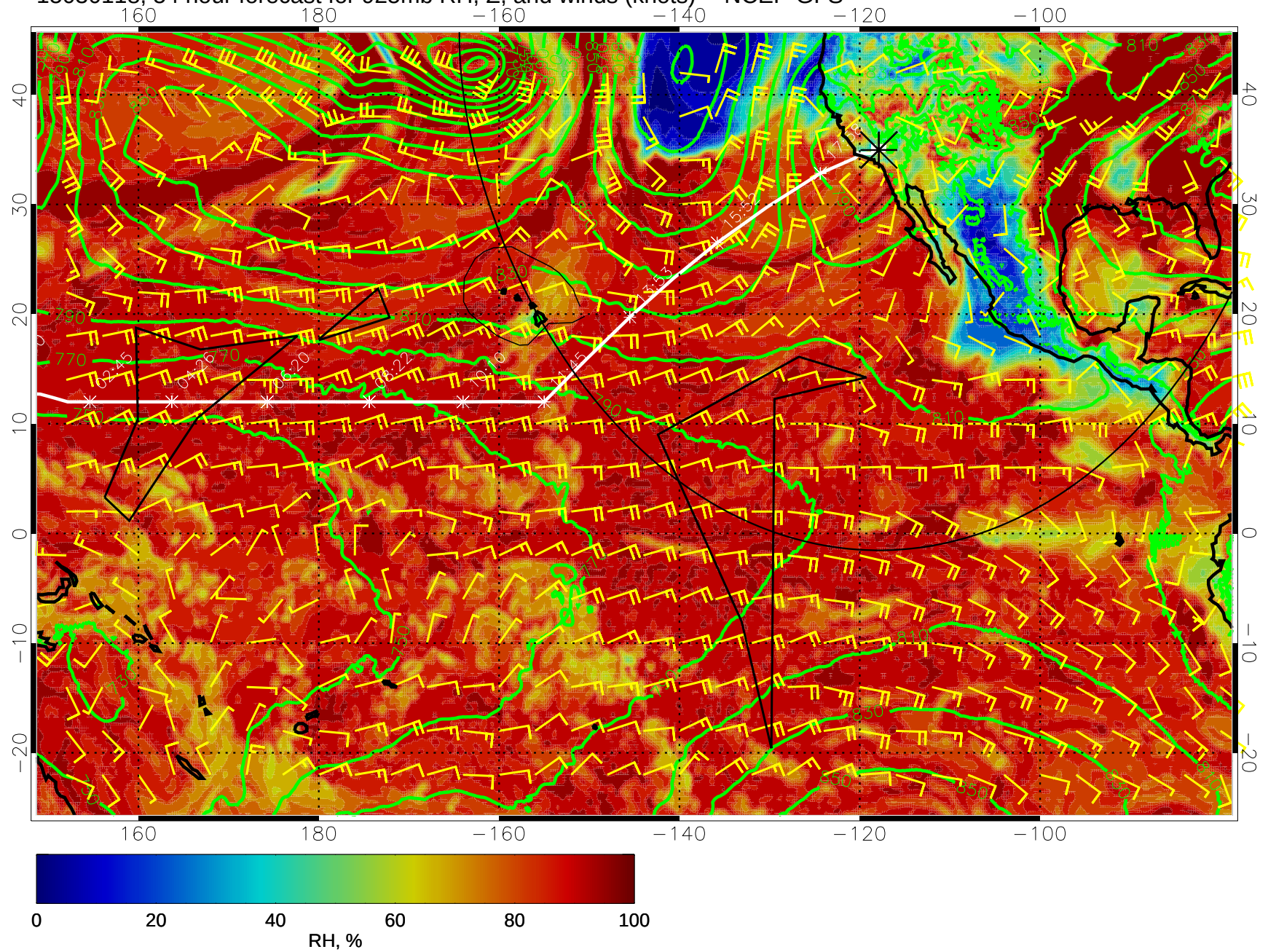
15030118, 54 hour forecast for 925mb RH, Z, and winds (knots) -- NCEP GFS
