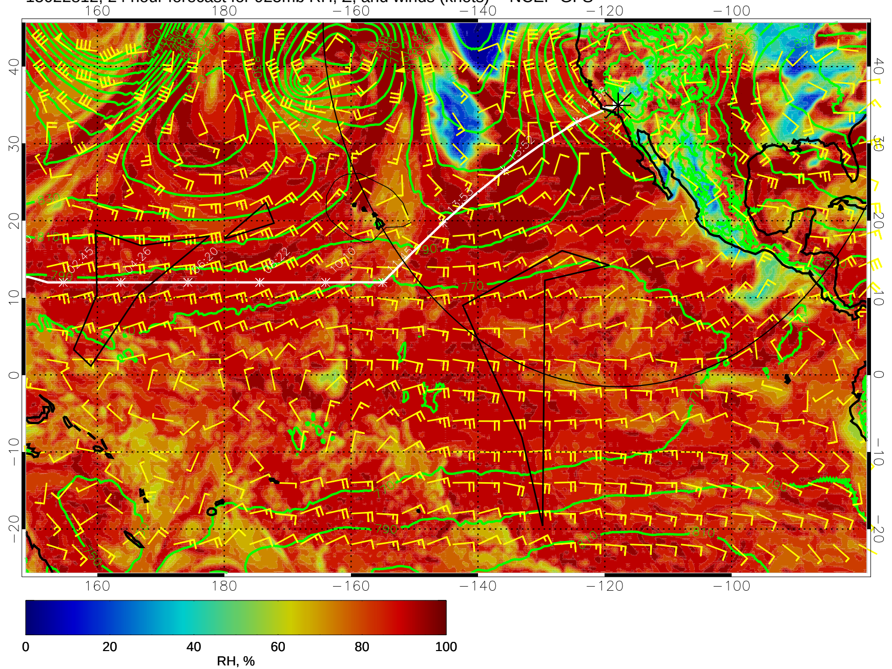
15022812, 24 hour forecast for 925mb RH, Z, and winds (knots) -- NCEP GFS
