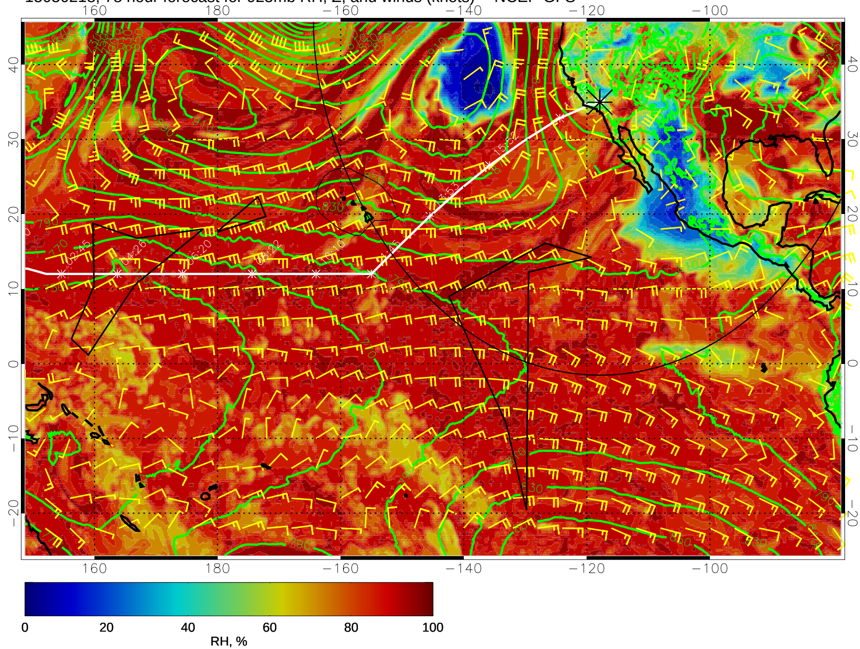
15030218, 78 hour forecast for 925mb RH, Z, and winds (knots) -- NCEP GFS
