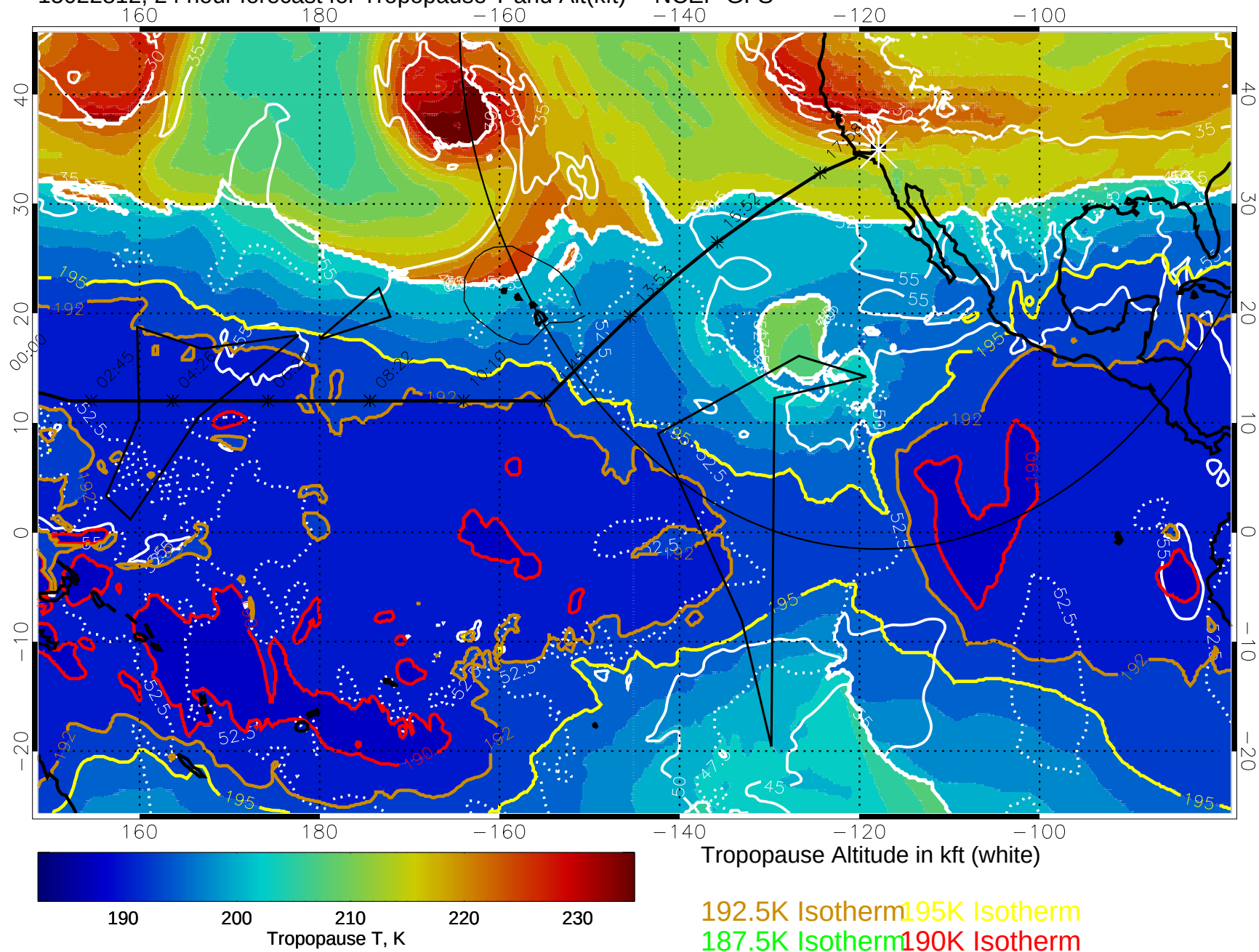
15022812, 24 hour forecast for Tropopause T and Alt(kft) -- NCEP GFS
