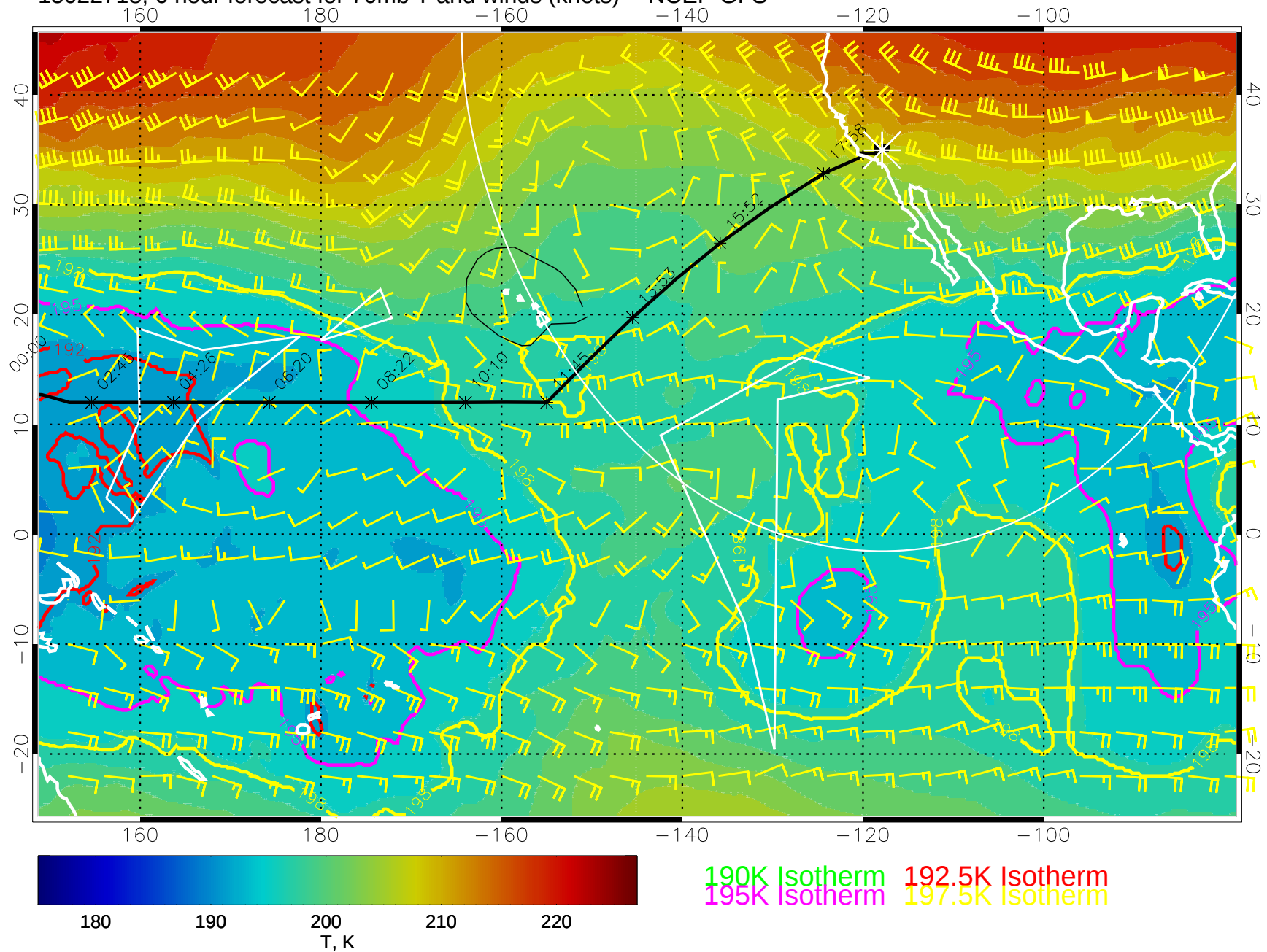
15022718, 6 hour forecast for 70mb T and winds (knots) -- NCEP GFS
