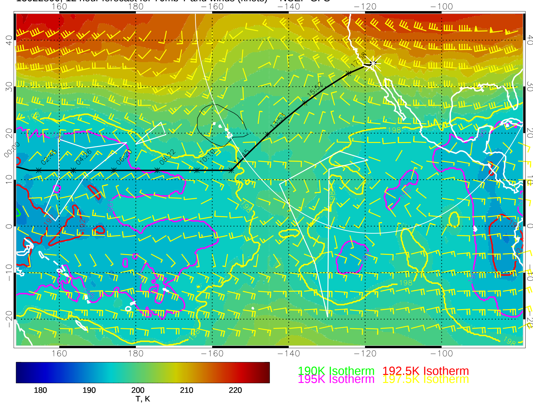
15022800, 12 hour forecast for 70mb T and winds (knots) -- NCEP GFS
