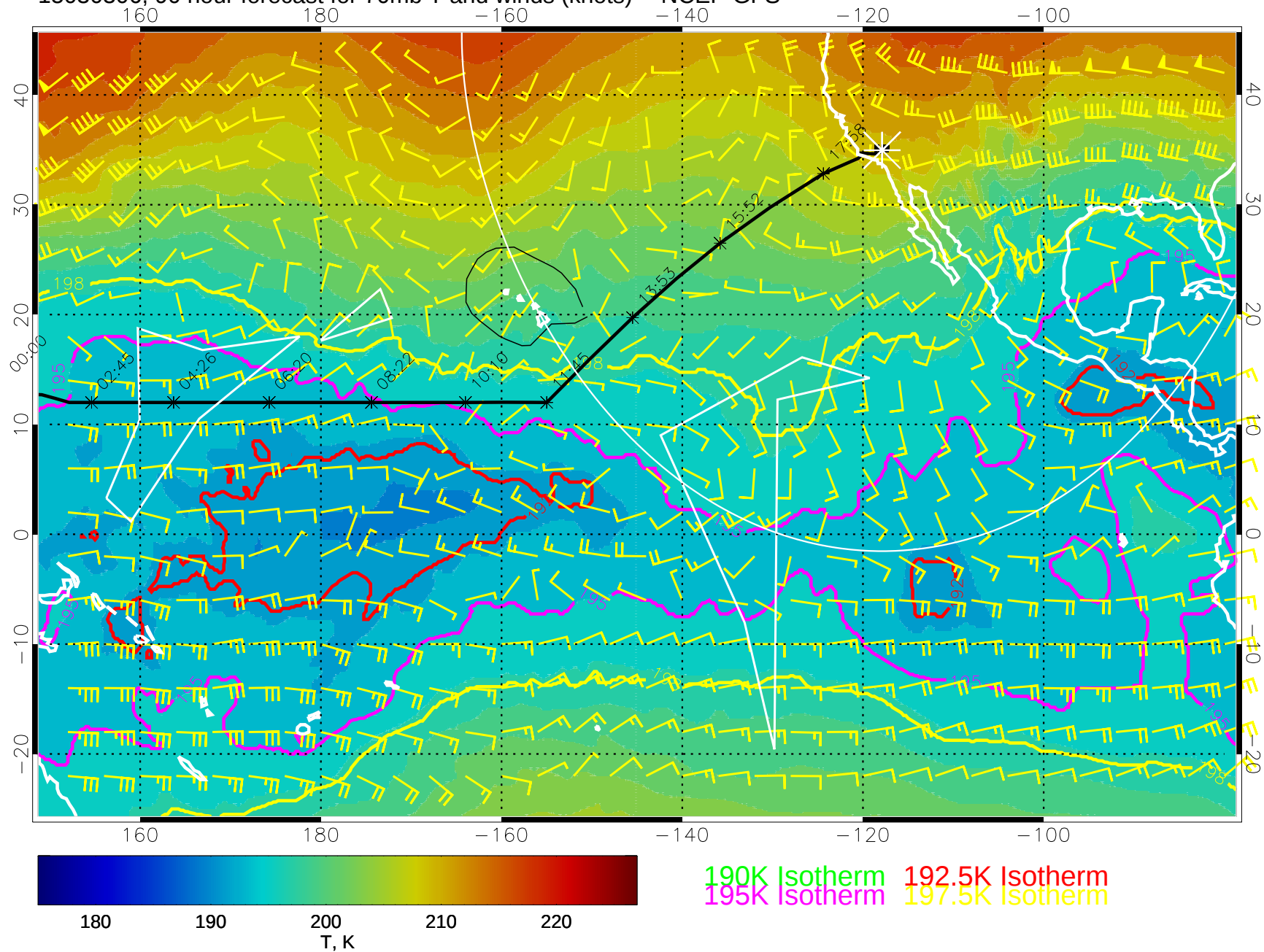
15030306, 90 hour forecast for 70mb T and winds (knots) -- NCEP GFS
