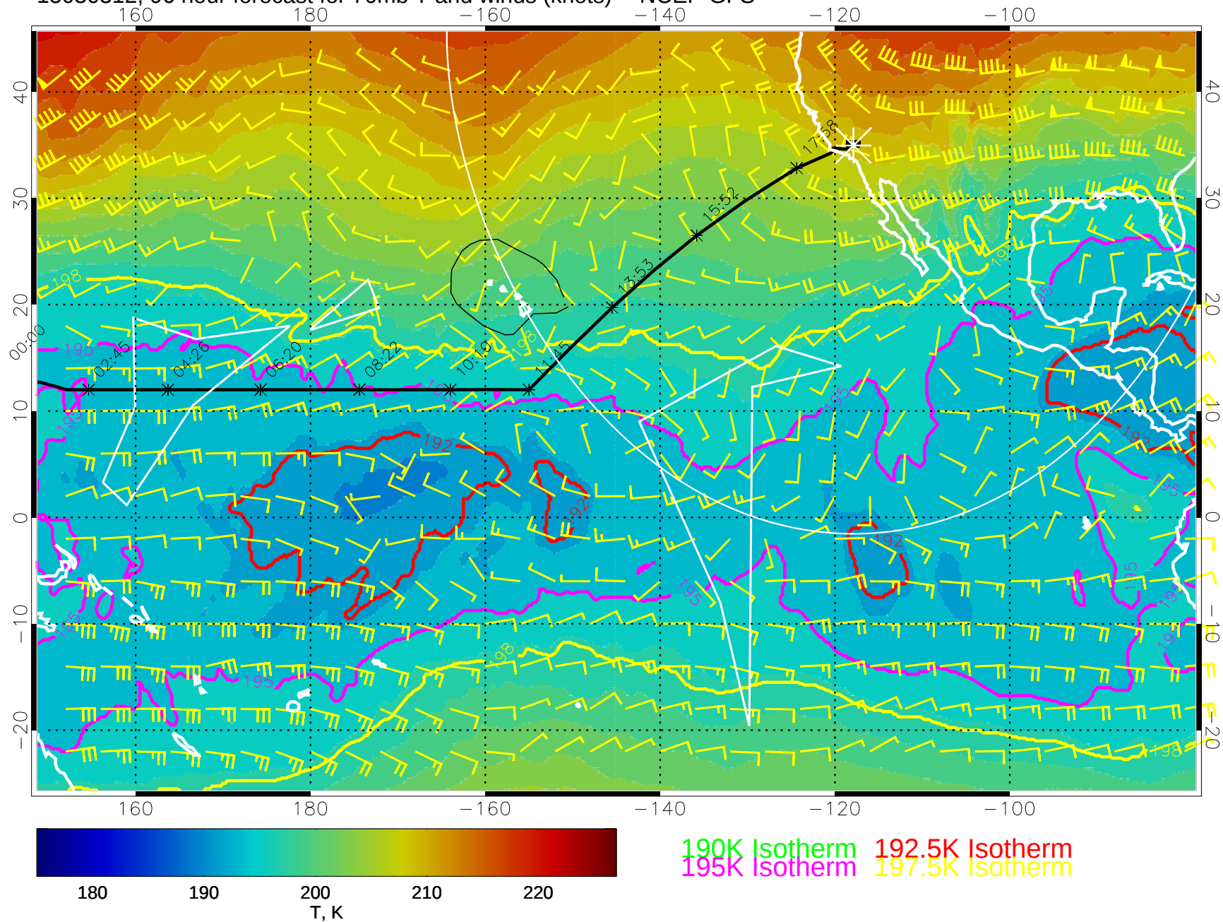
15030312, 96 hour forecast for 70mb T and winds (knots) -- NCEP GFS
