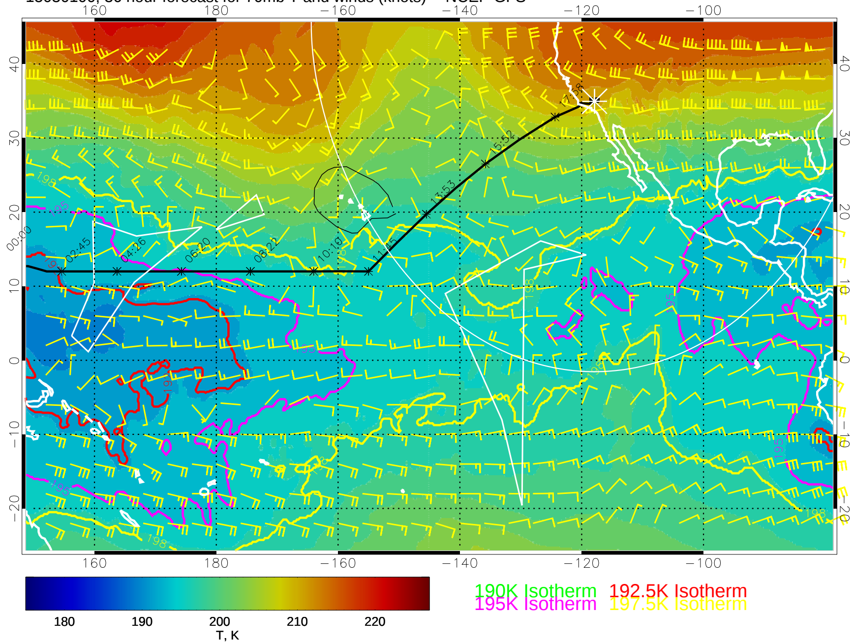
15030100, 36 hour forecast for 70mb T and winds (knots) -- NCEP GFS
