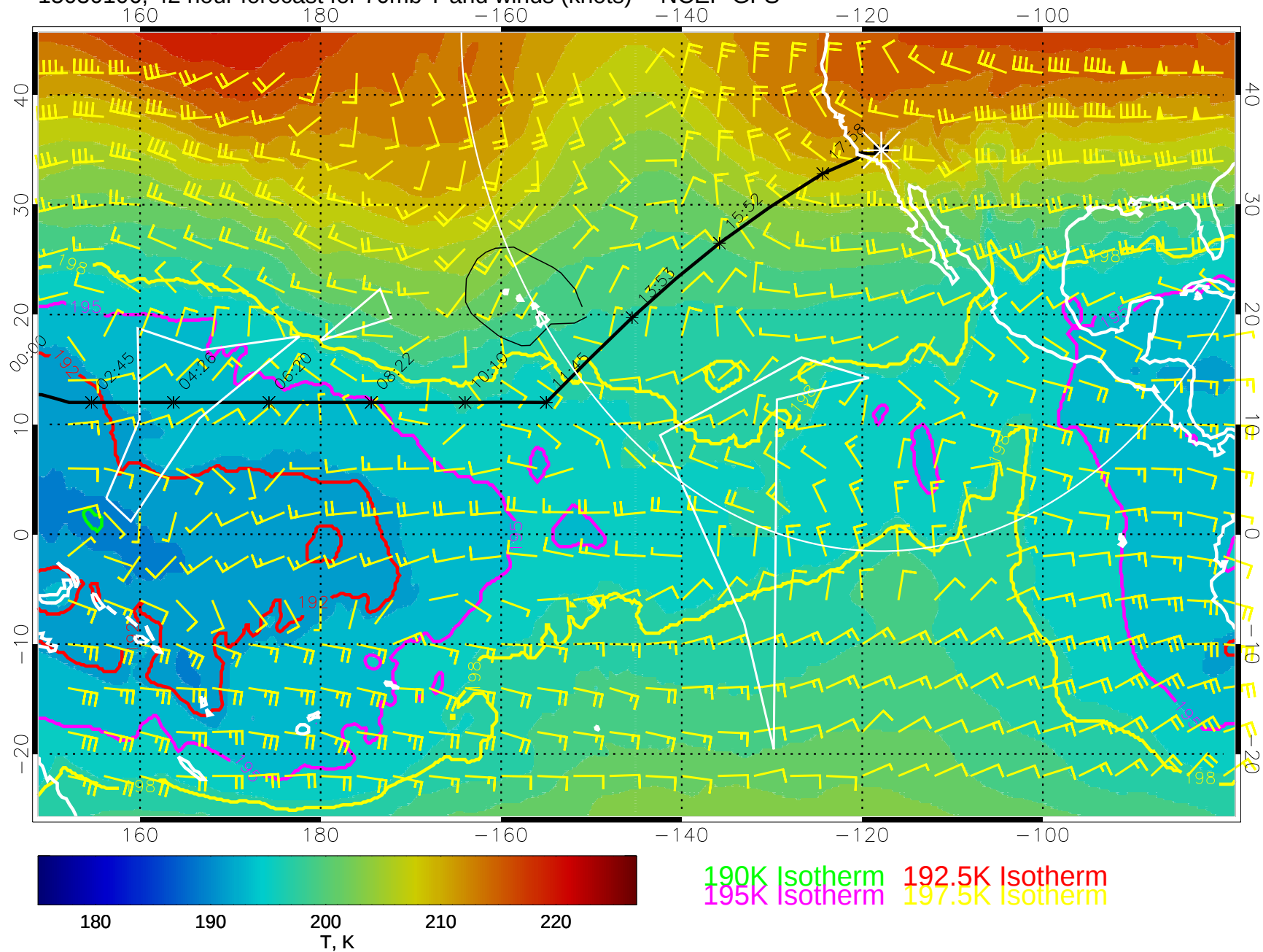
15030106, 42 hour forecast for 70mb T and winds (knots) -- NCEP GFS
