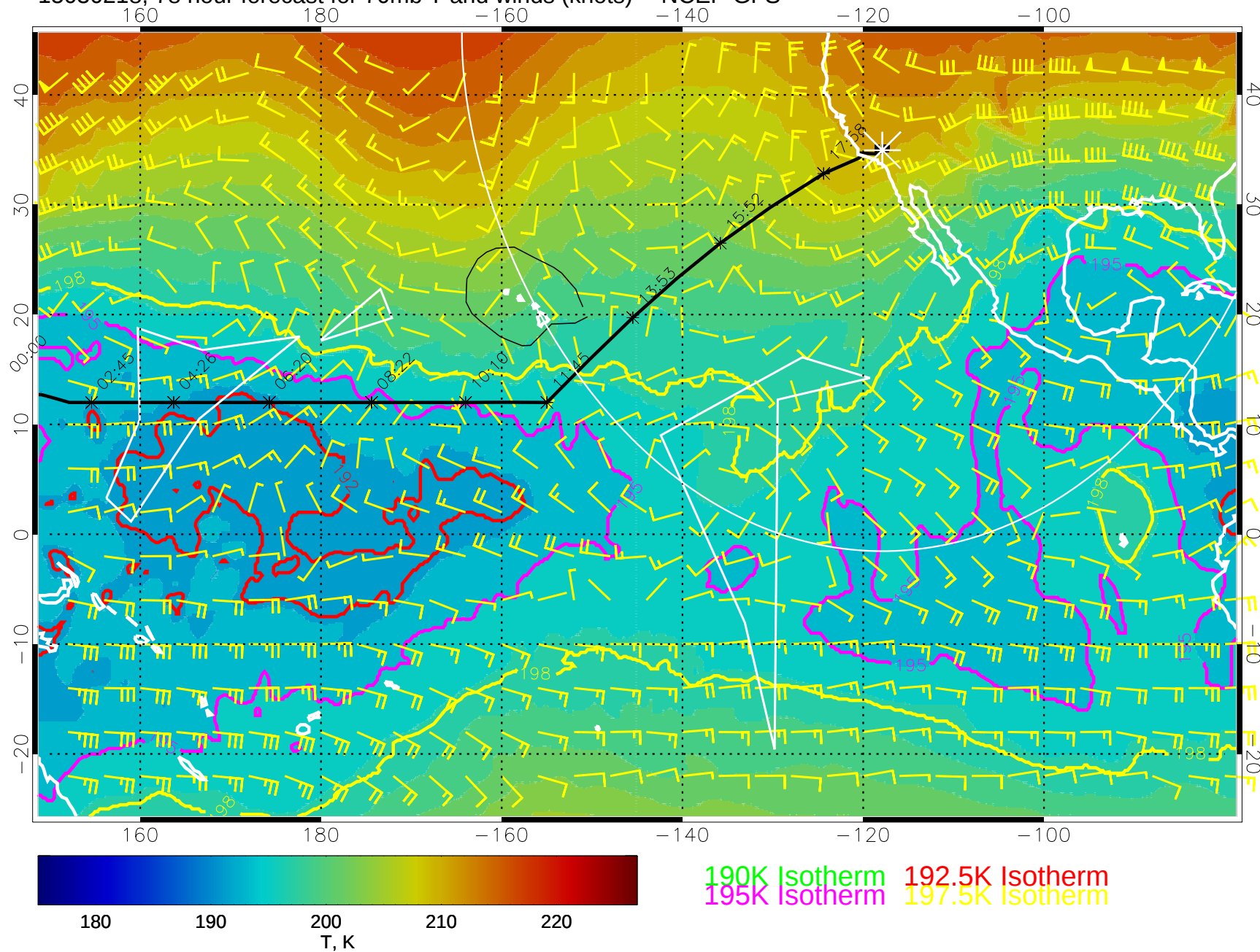
15030218, 78 hour forecast for 70mb T and winds (knots) -- NCEP GFS
