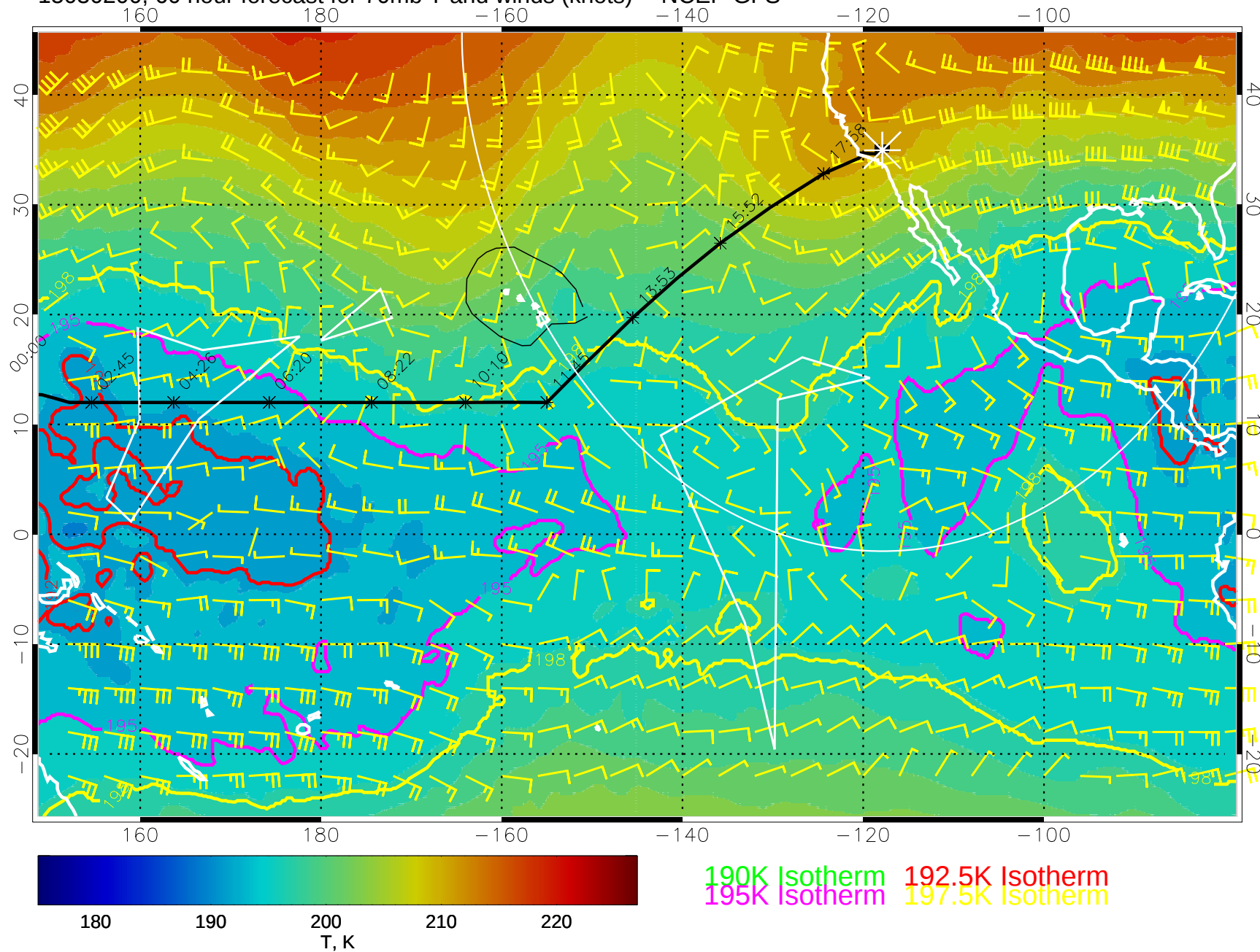
15030200, 60 hour forecast for 70mb T and winds (knots) -- NCEP GFS
