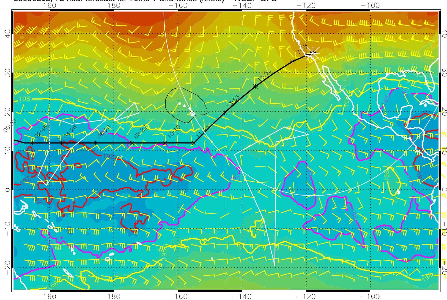
15030212, 72 hour forecast for 70mb T and winds (knots) -- NCEP GFS
