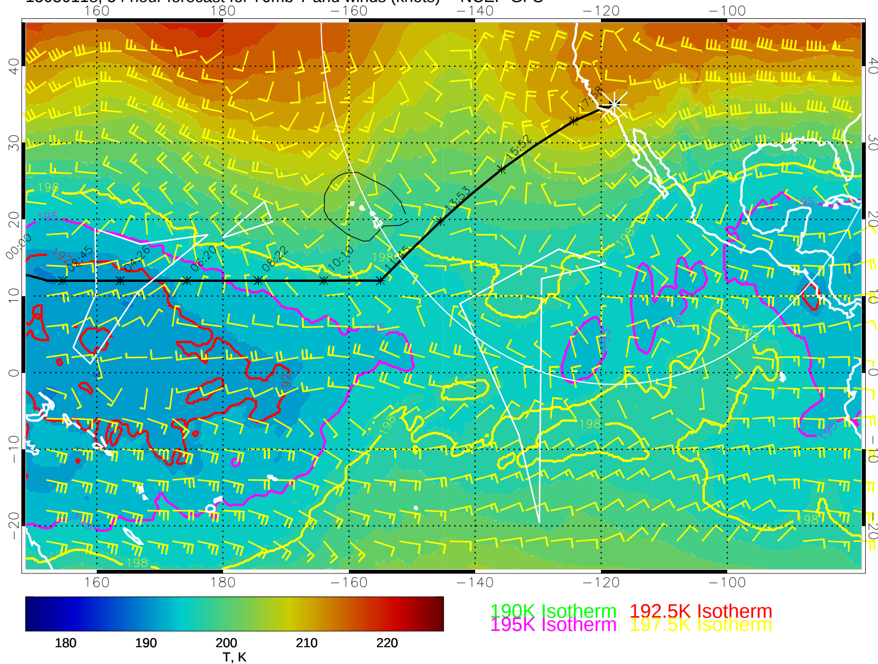
15030118, 54 hour forecast for 70mb T and winds (knots) -- NCEP GFS
