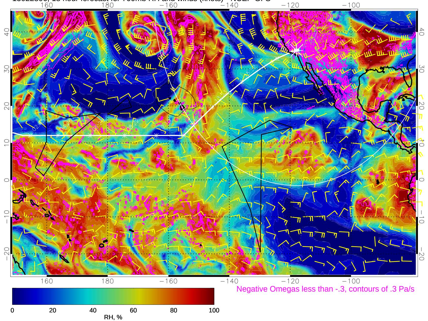
15022806, 18 hour forecast for 700mb RH and winds (knots) - NCEP GFS
