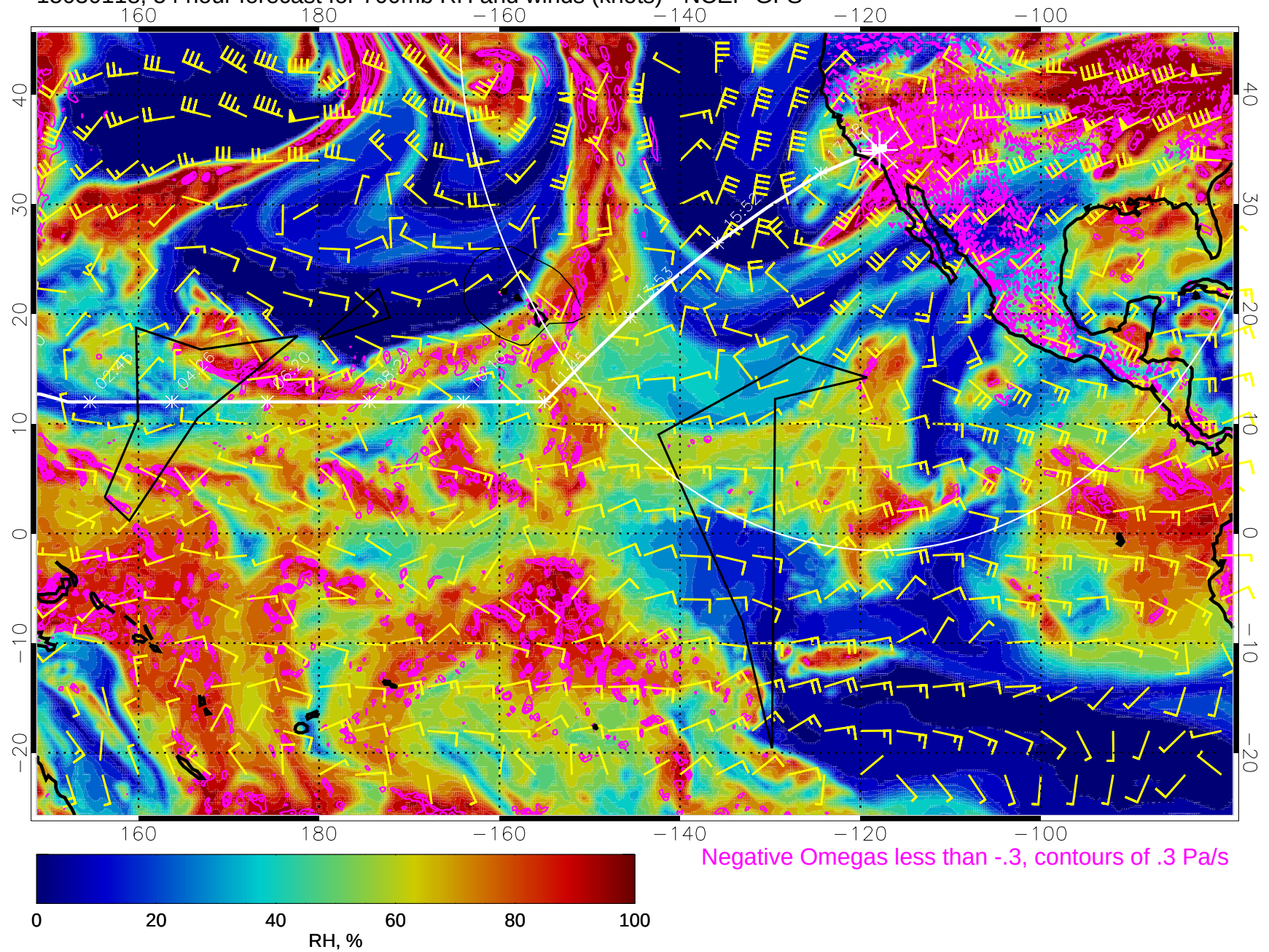
15030118, 54 hour forecast for 700mb RH and winds (knots) - NCEP GFS
