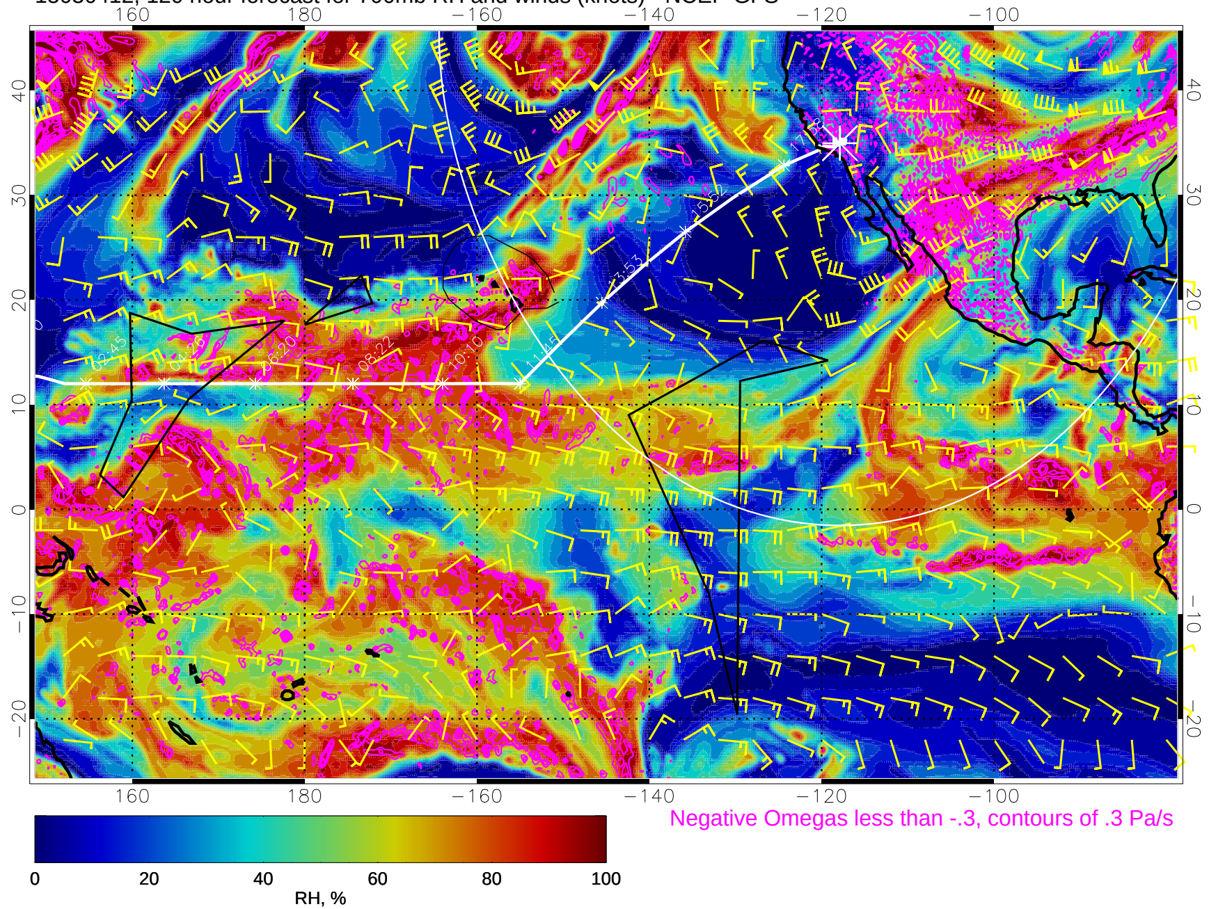
15030412, 120 hour forecast for 700mb RH and winds (knots) - NCEP GFS
