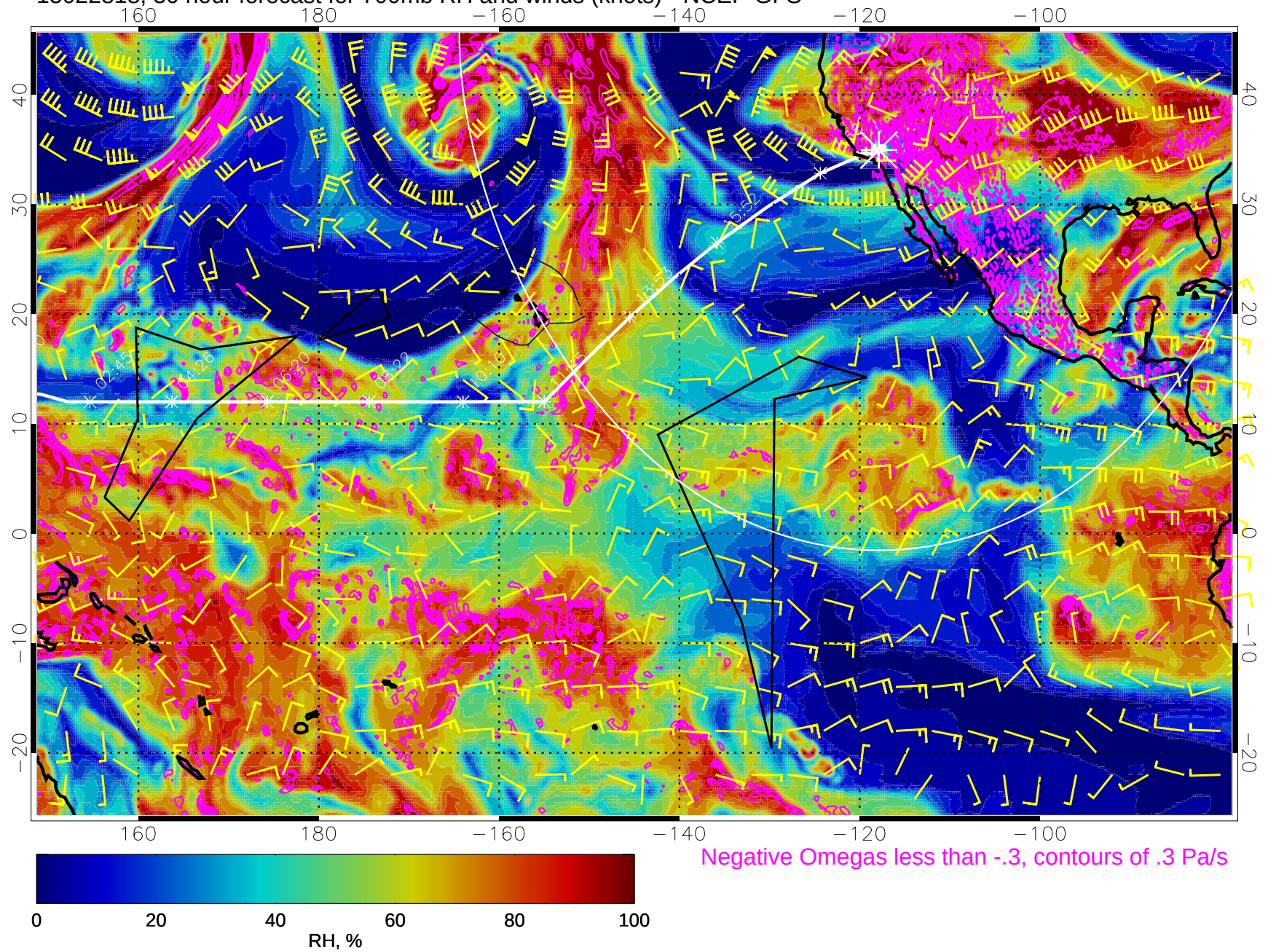
15022818, 30 hour forecast for 700mb RH and winds (knots) - NCEP GFS
