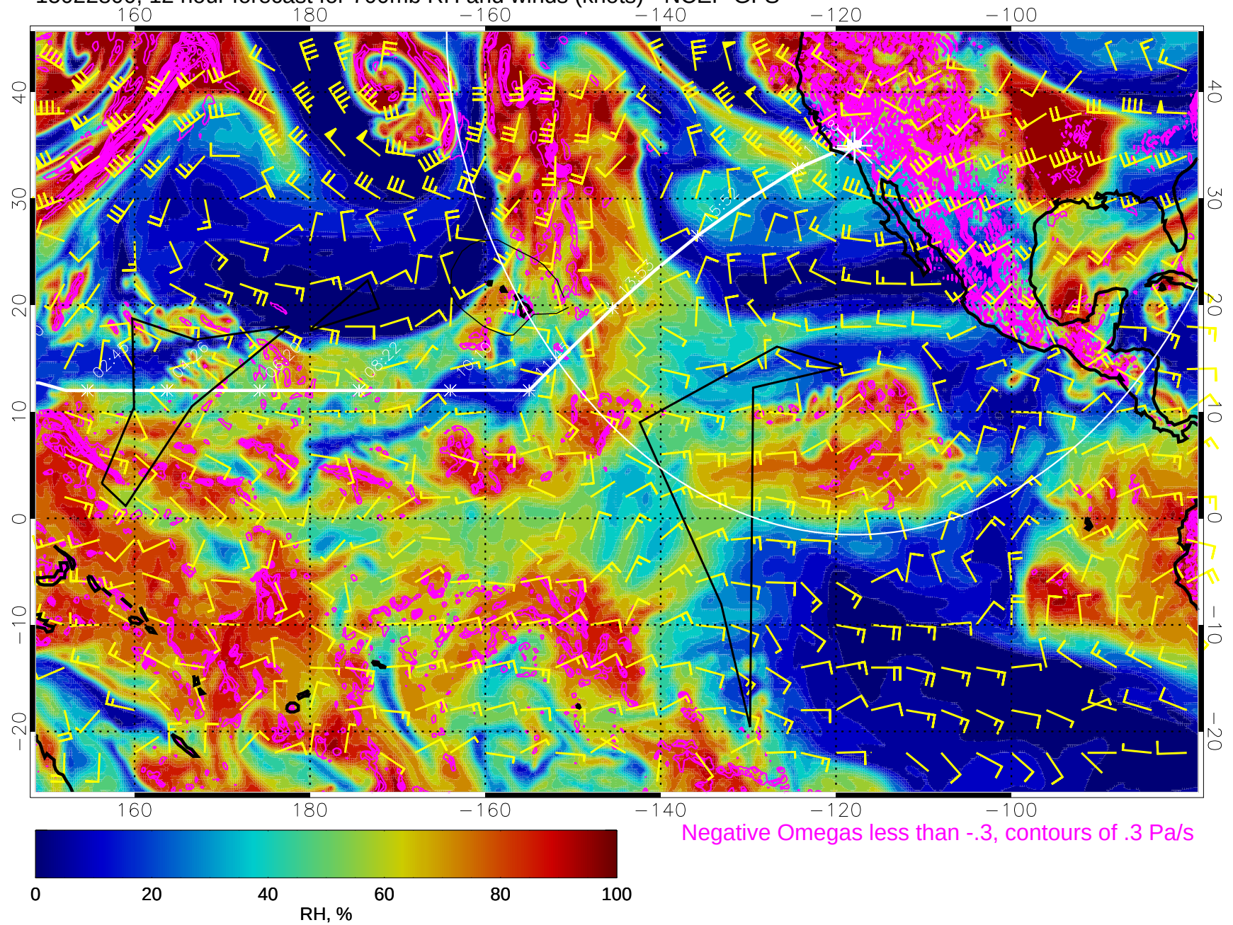
15022800, 12 hour forecast for 700mb RH and winds (knots) - NCEP GFS
