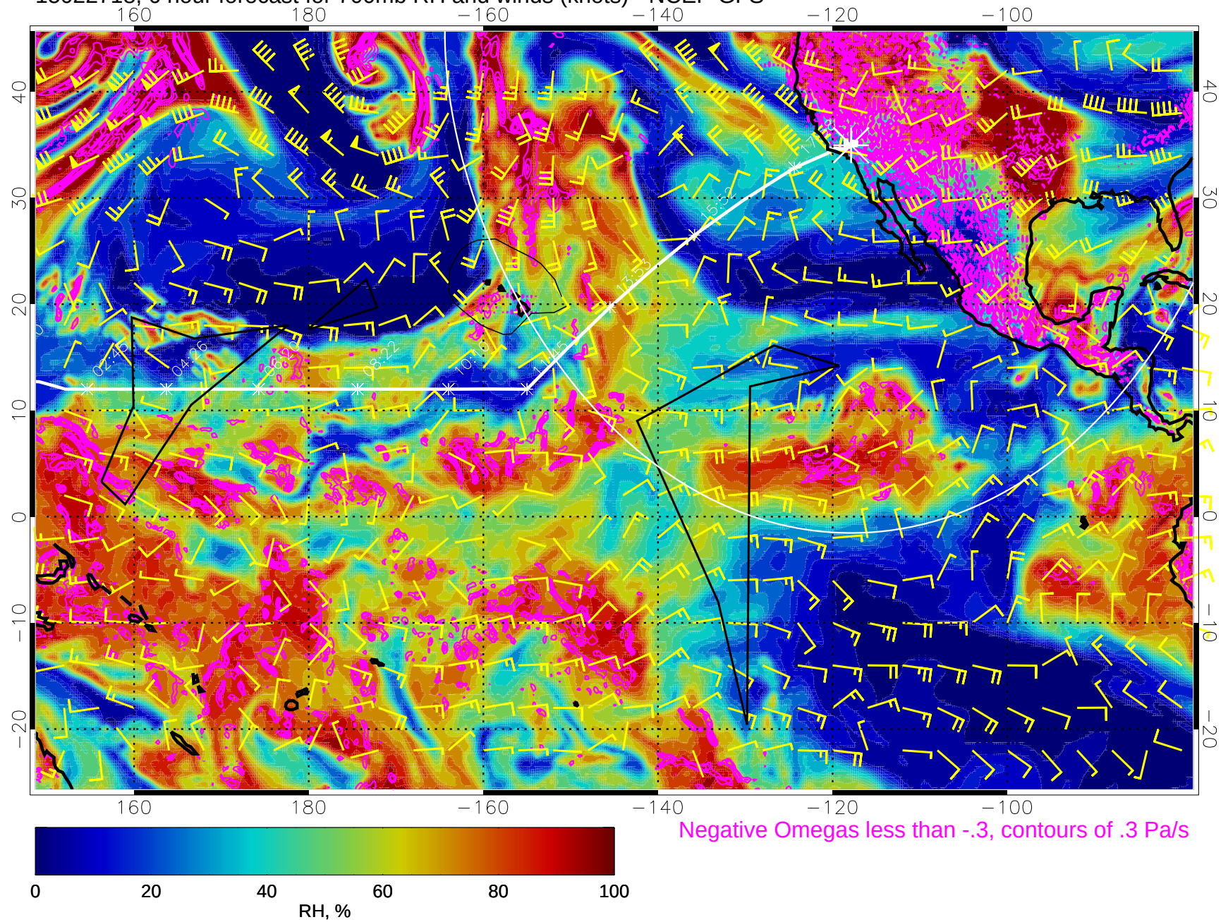
15022718, 6 hour forecast for 700mb RH and winds (knots) - NCEP GFS
