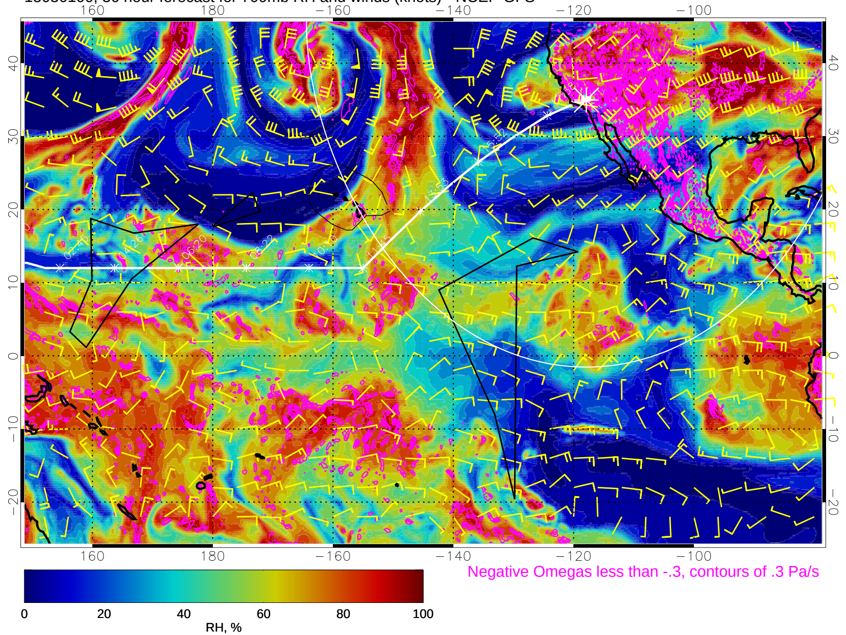
15030100, 36 hour forecast for 700mb RH and winds (knots) - NCEP GFS
