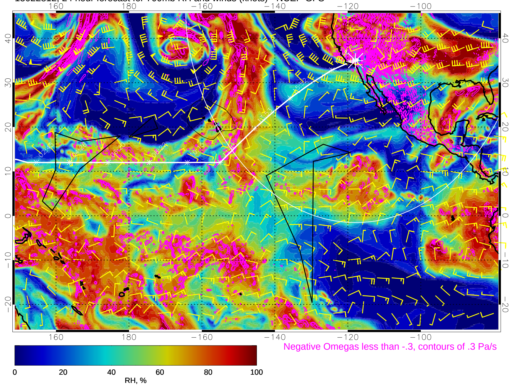
15022812, 24 hour forecast for 700mb RH and winds (knots) - NCEP GFS
