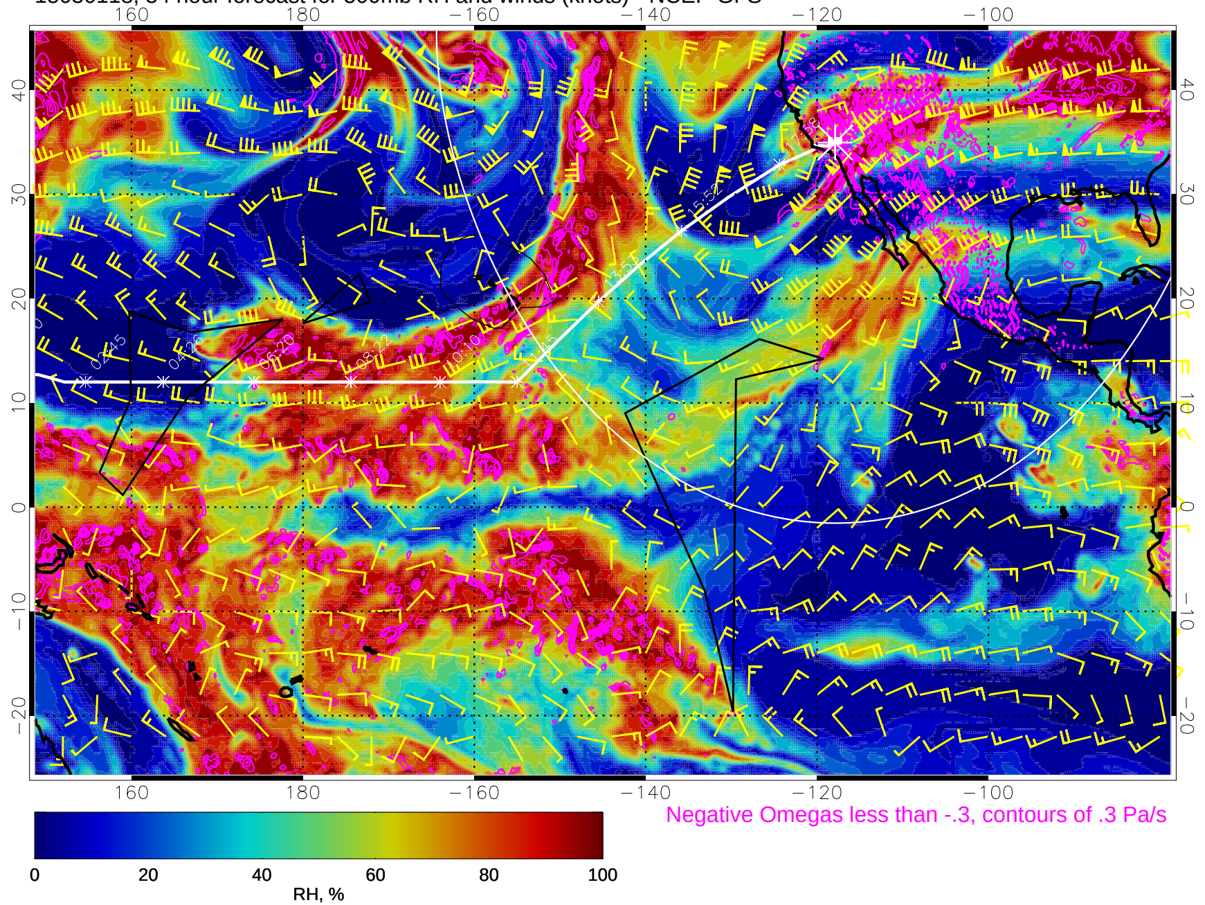
15030118, 54 hour forecast for 500mb RH and winds (knots) - NCEP GFS
