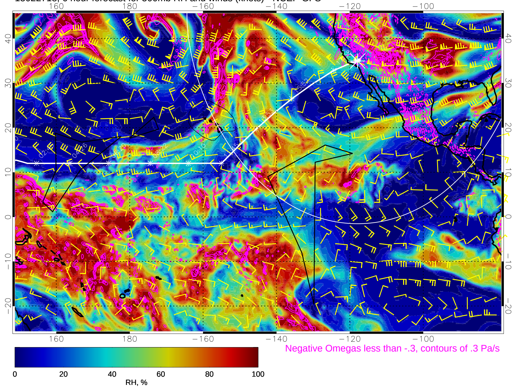
15022718, 6 hour forecast for 500mb RH and winds (knots) - NCEP GFS
