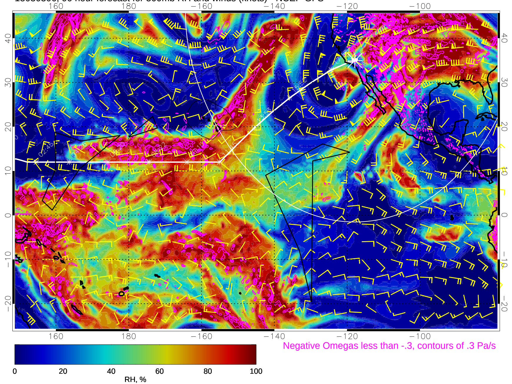
15030306, 90 hour forecast for 500mb RH and winds (knots) - NCEP GFS
