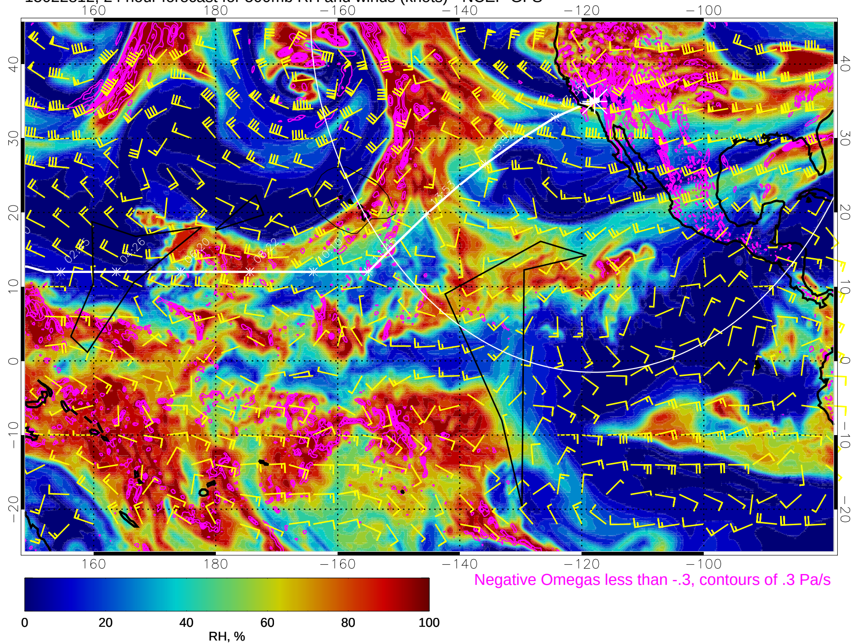
15022812, 24 hour forecast for 500mb RH and winds (knots) - NCEP GFS
