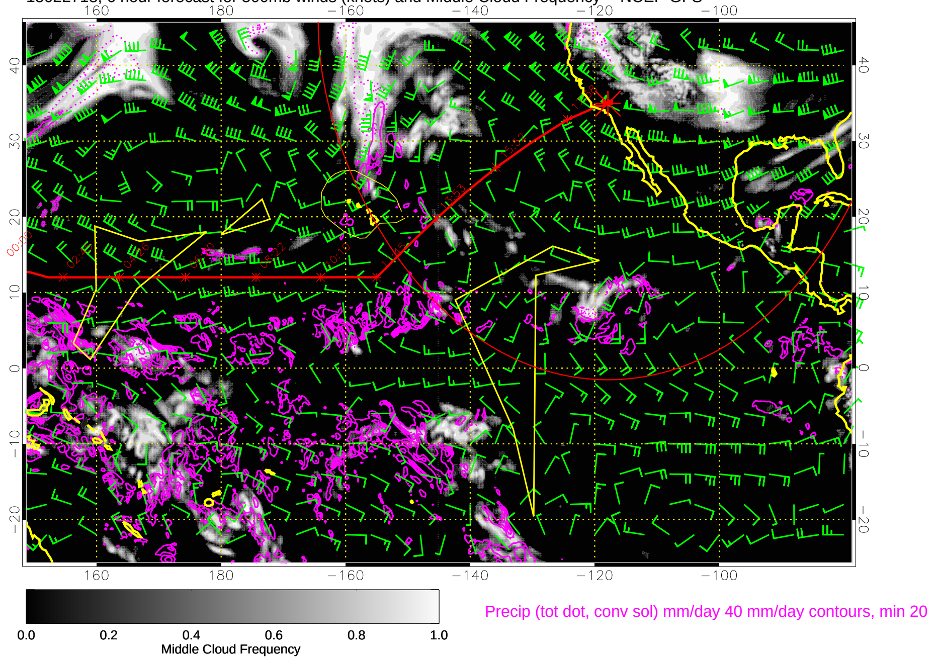
15022718, 6 hour forecast for 500mb winds (knots) and Middle Cloud Frequency -- NCEP GFS
