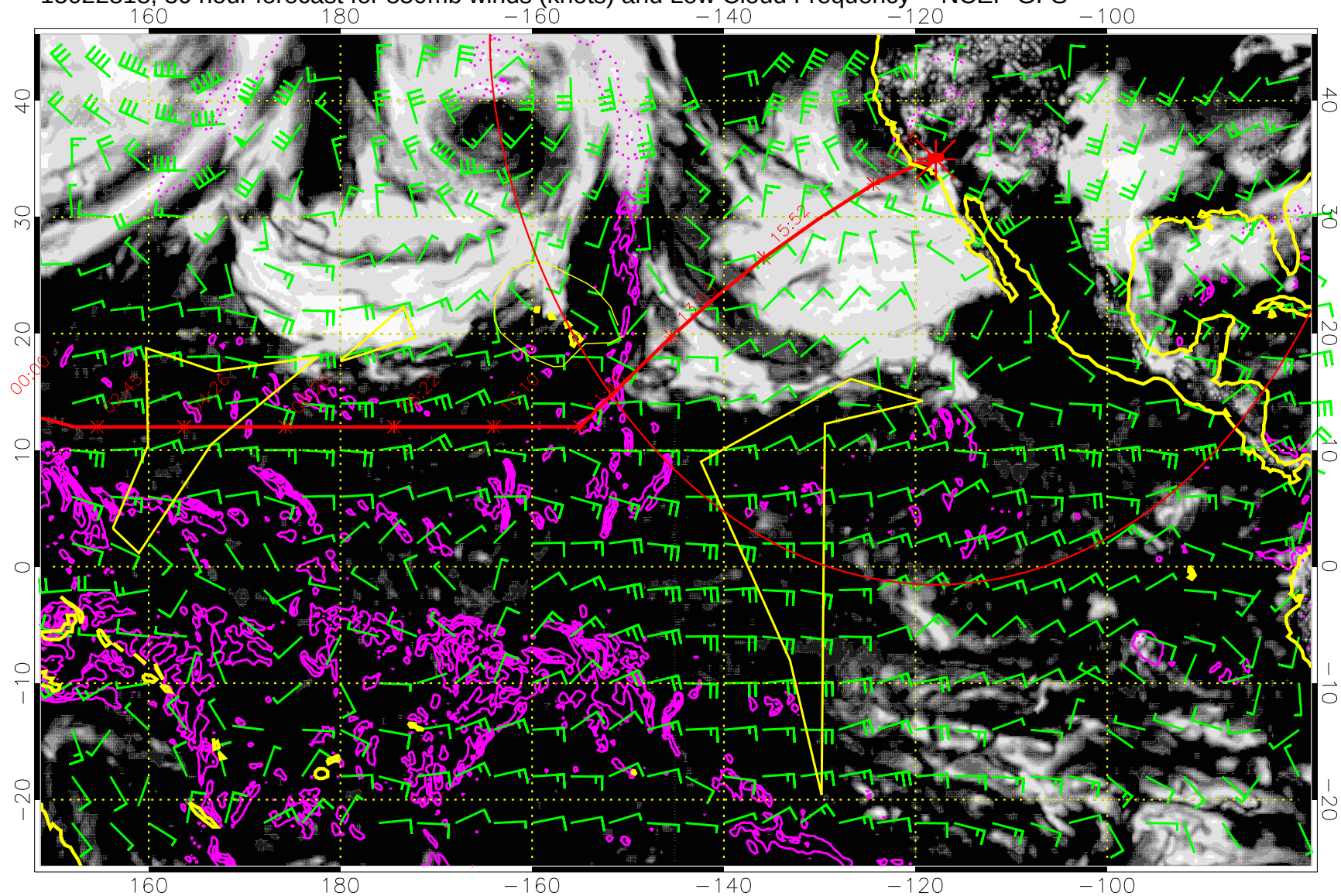
15022818, 30 hour forecast for 850mb winds (knots) and Low Cloud Frequency -- NCEP GFS
