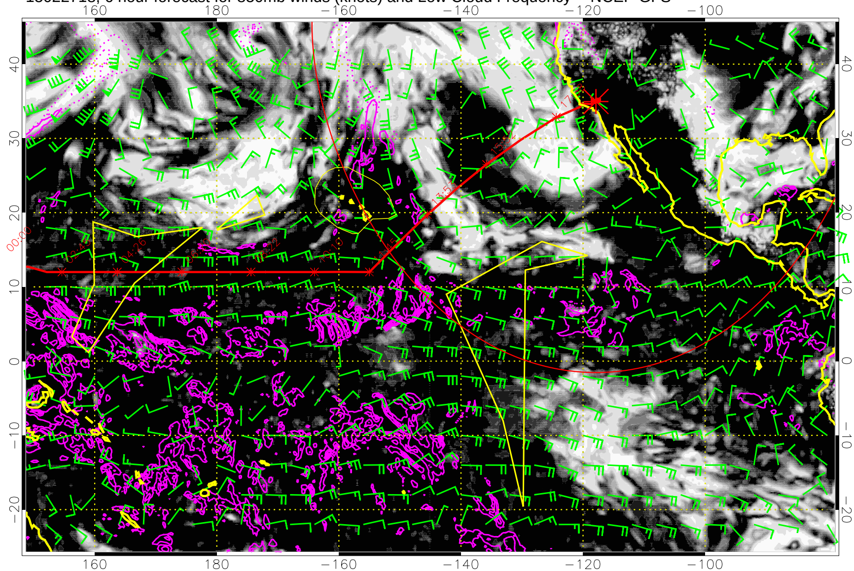
15022718, 6 hour forecast for 850mb winds (knots) and Low Cloud Frequency -- NCEP GFS
