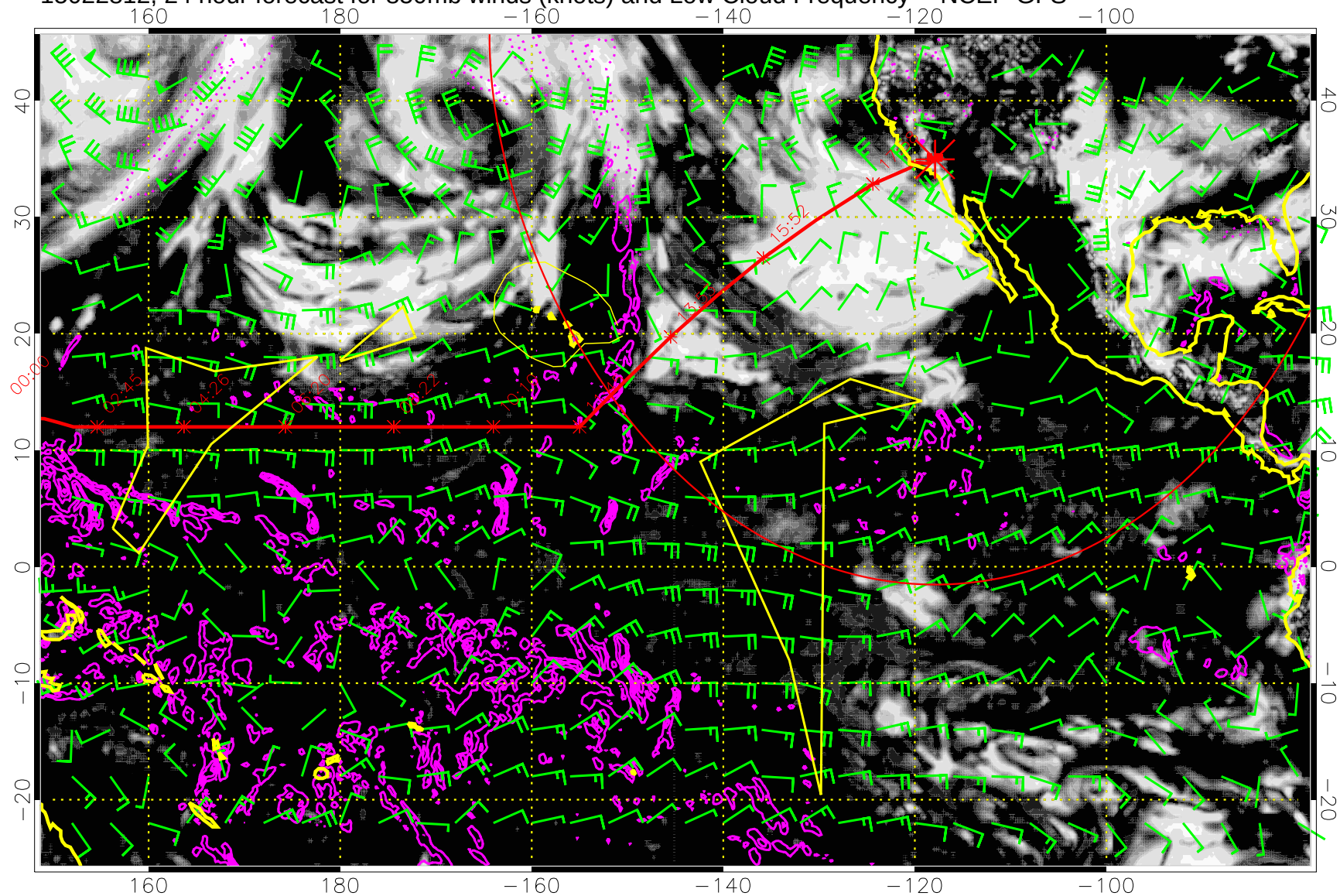
15022812, 24 hour forecast for 850mb winds (knots) and Low Cloud Frequency -- NCEP GFS
