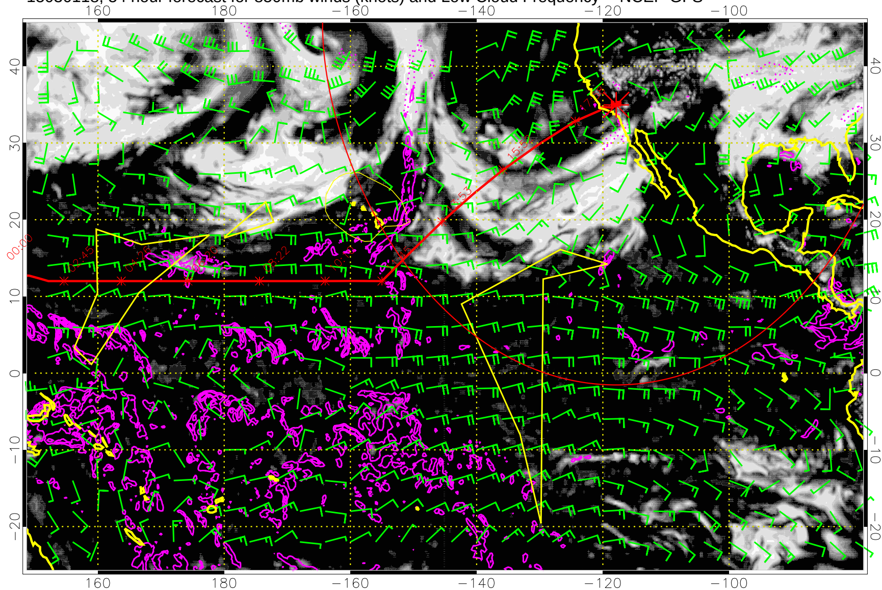
15030118, 54 hour forecast for 850mb winds (knots) and Low Cloud Frequency -- NCEP GFS
