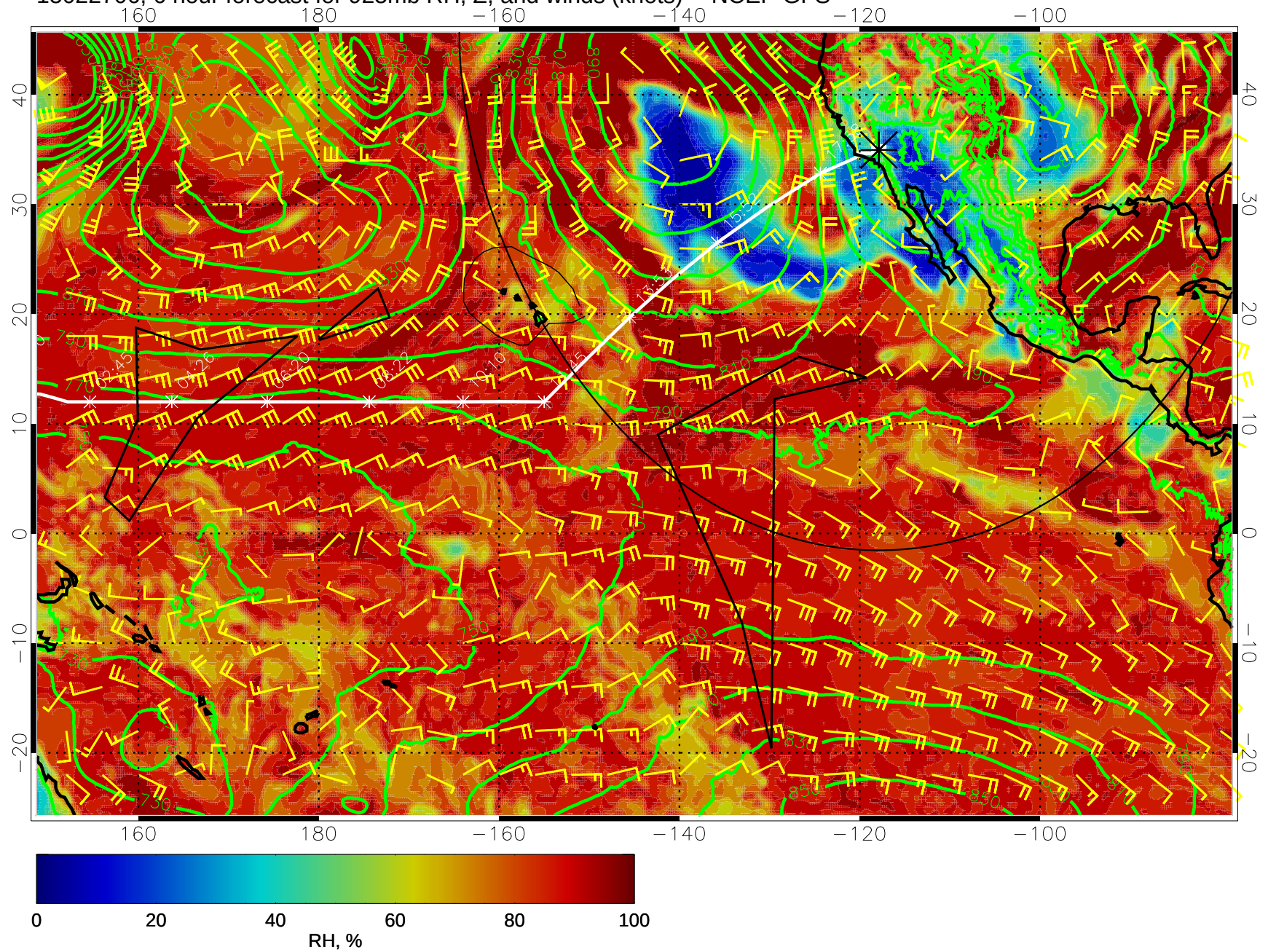
15022706, 6 hour forecast for 925mb RH, Z, and winds (knots) -- NCEP GFS
