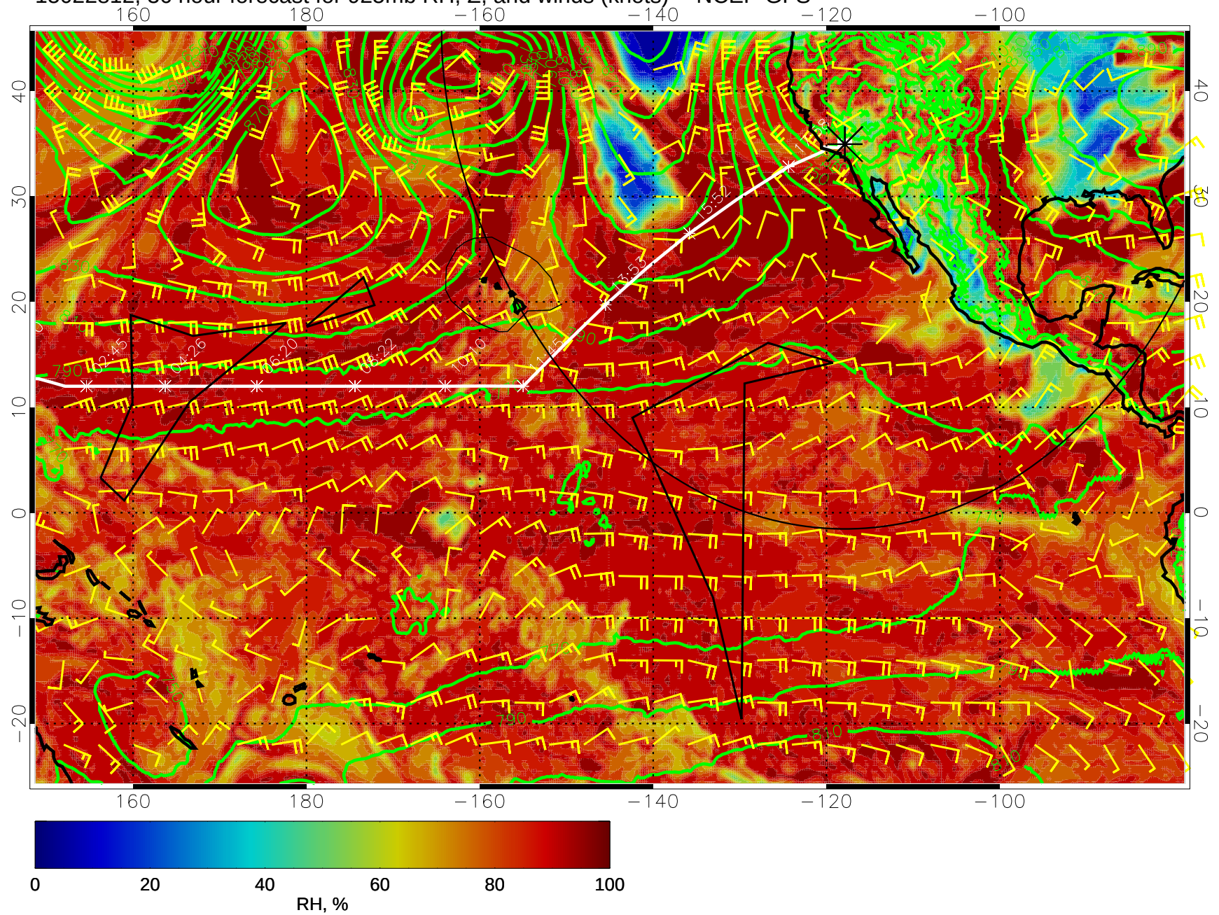
15022812, 36 hour forecast for 925mb RH, Z, and winds (knots) -- NCEP GFS
