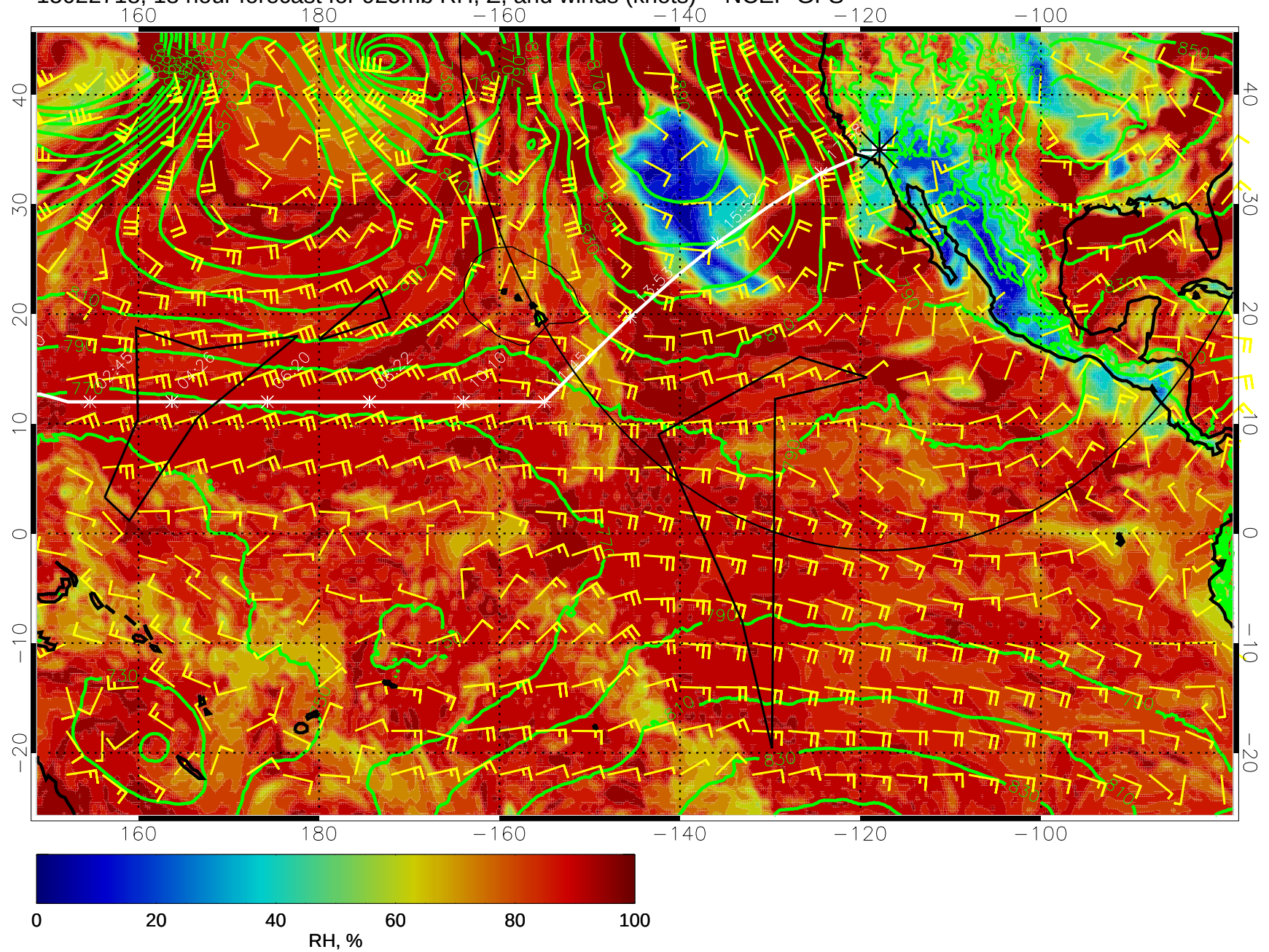
15022718, 18 hour forecast for 925mb RH, Z, and winds (knots) -- NCEP GFS
