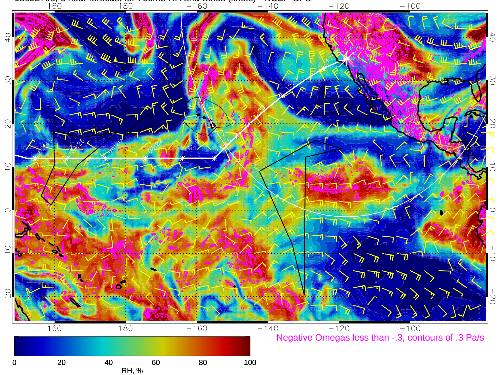
15022706, 6 hour forecast for 700mb RH and winds (knots) - NCEP GFS
