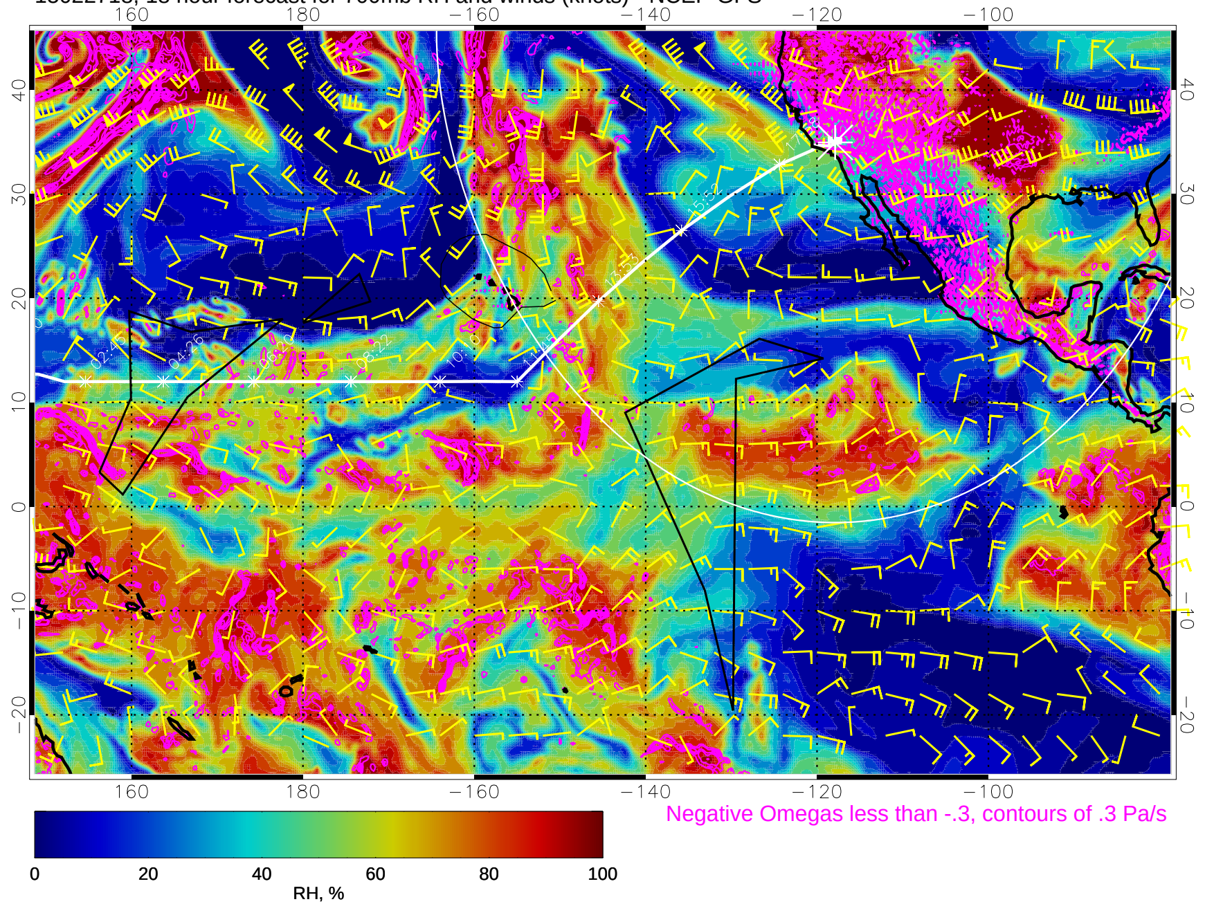
15022718, 18 hour forecast for 700mb RH and winds (knots) - NCEP GFS
