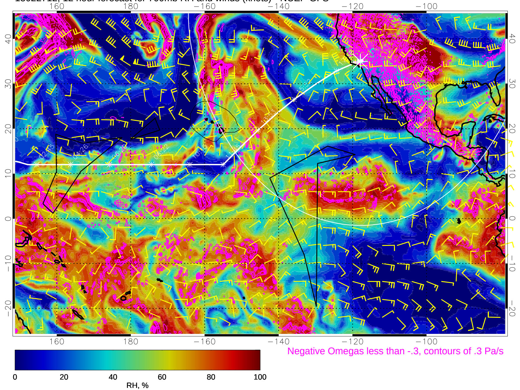
15022712, 12 hour forecast for 700mb RH and winds (knots) - NCEP GFS
