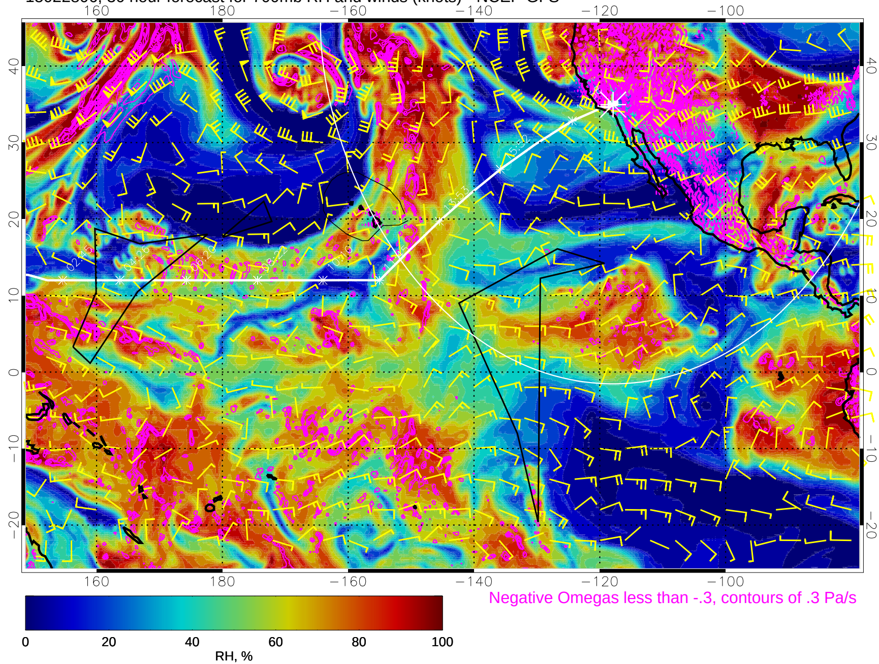
15022806, 30 hour forecast for 700mb RH and winds (knots) - NCEP GFS
