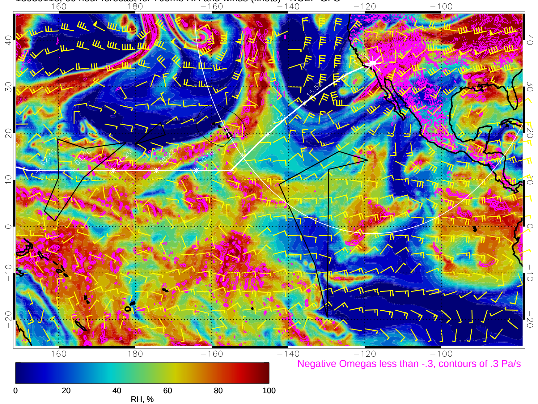
15030118, 66 hour forecast for 700mb RH and winds (knots) - NCEP GFS
