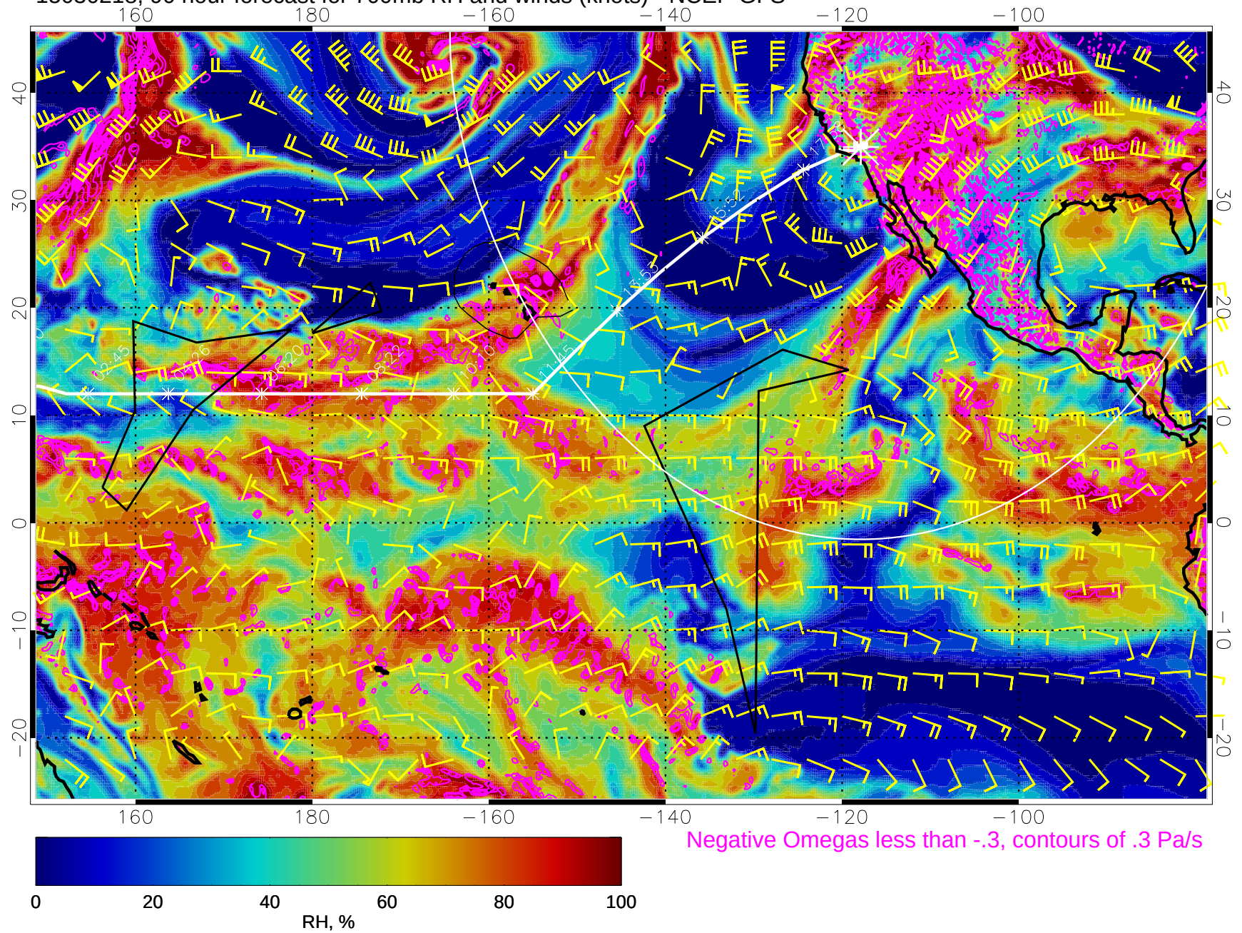
15030218, 90 hour forecast for 700mb RH and winds (knots) - NCEP GFS
