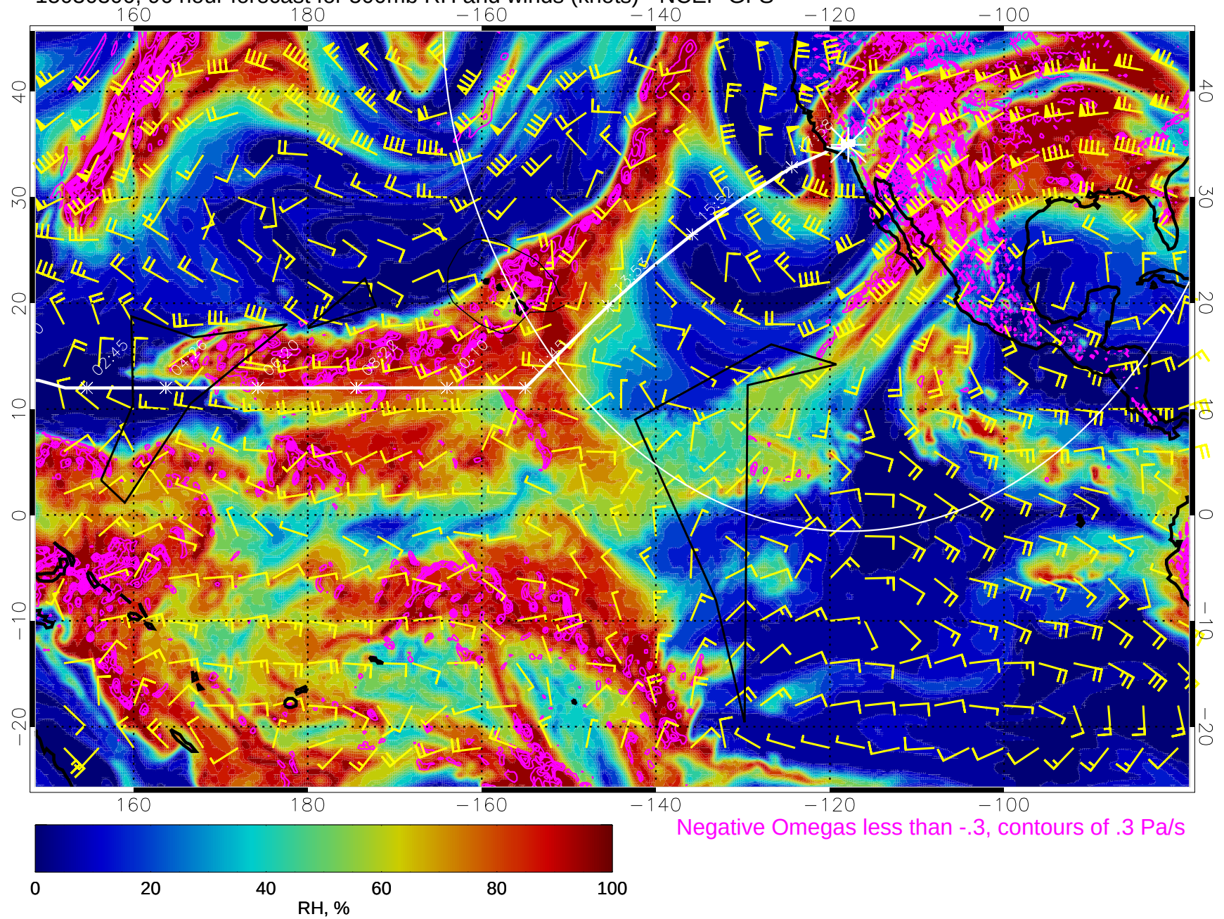
15030300, 96 hour forecast for 500mb RH and winds (knots) - NCEP GFS
