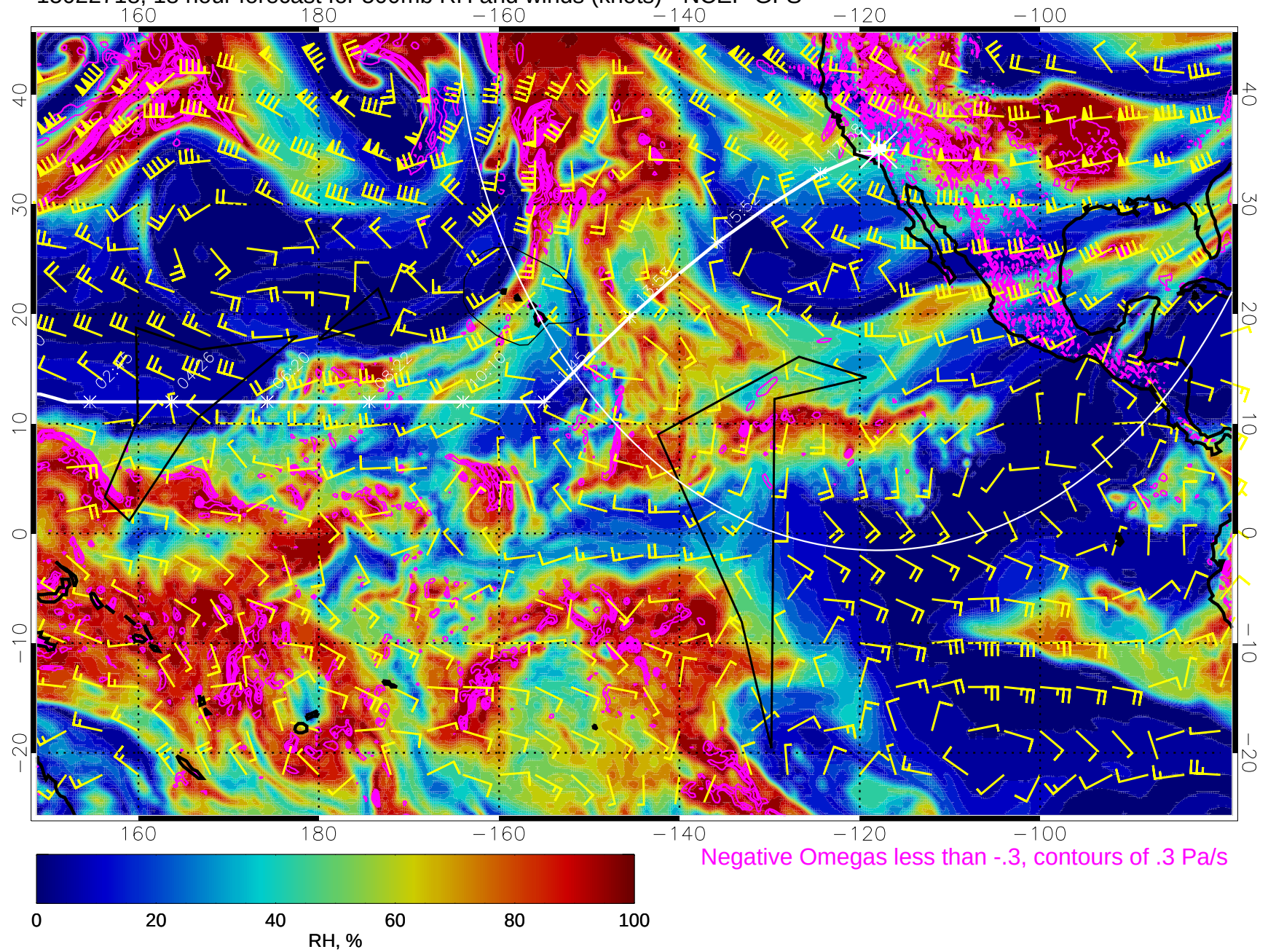
15022718, 18 hour forecast for 500mb RH and winds (knots) - NCEP GFS
