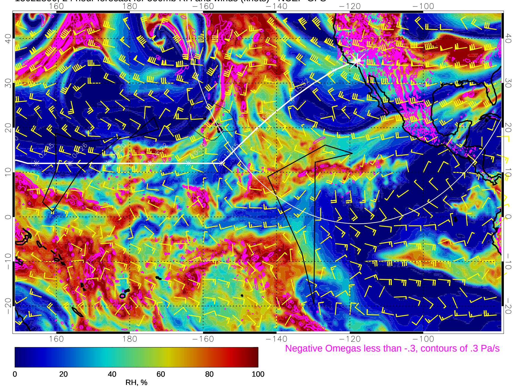
15022800, 24 hour forecast for 500mb RH and winds (knots) - NCEP GFS
