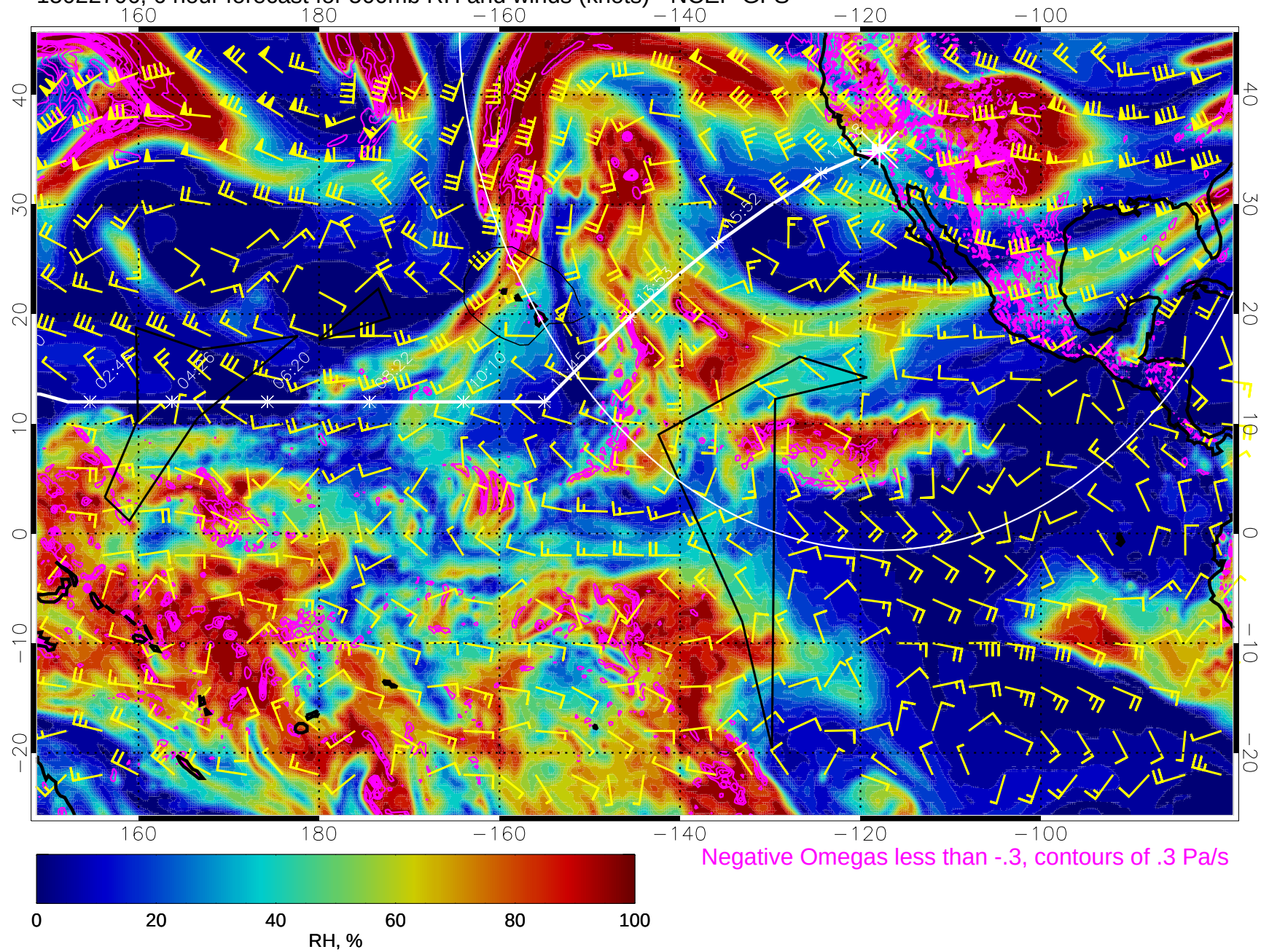
15022706, 6 hour forecast for 500mb RH and winds (knots) - NCEP GFS
