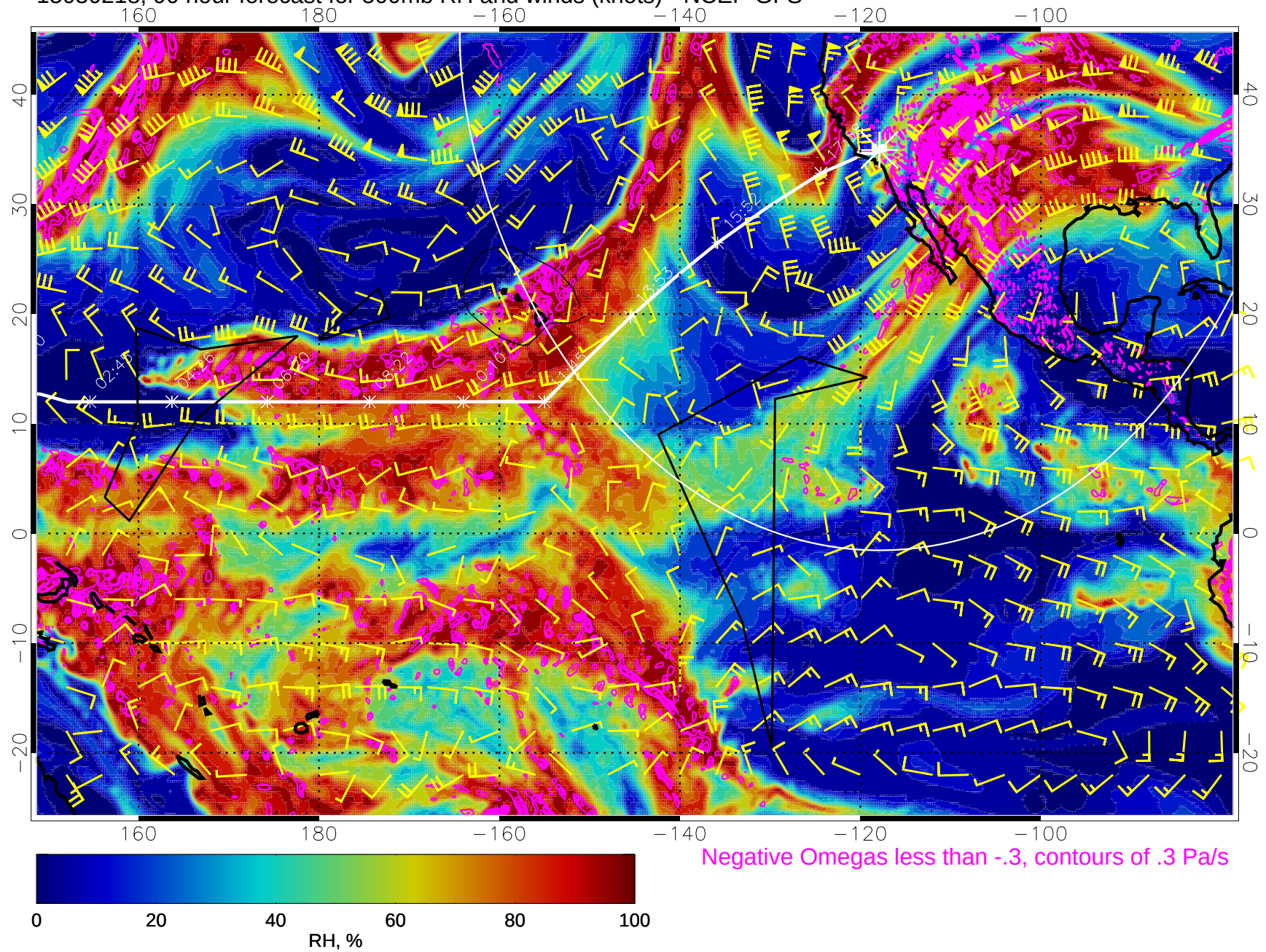
15030218, 90 hour forecast for 500mb RH and winds (knots) - NCEP GFS
