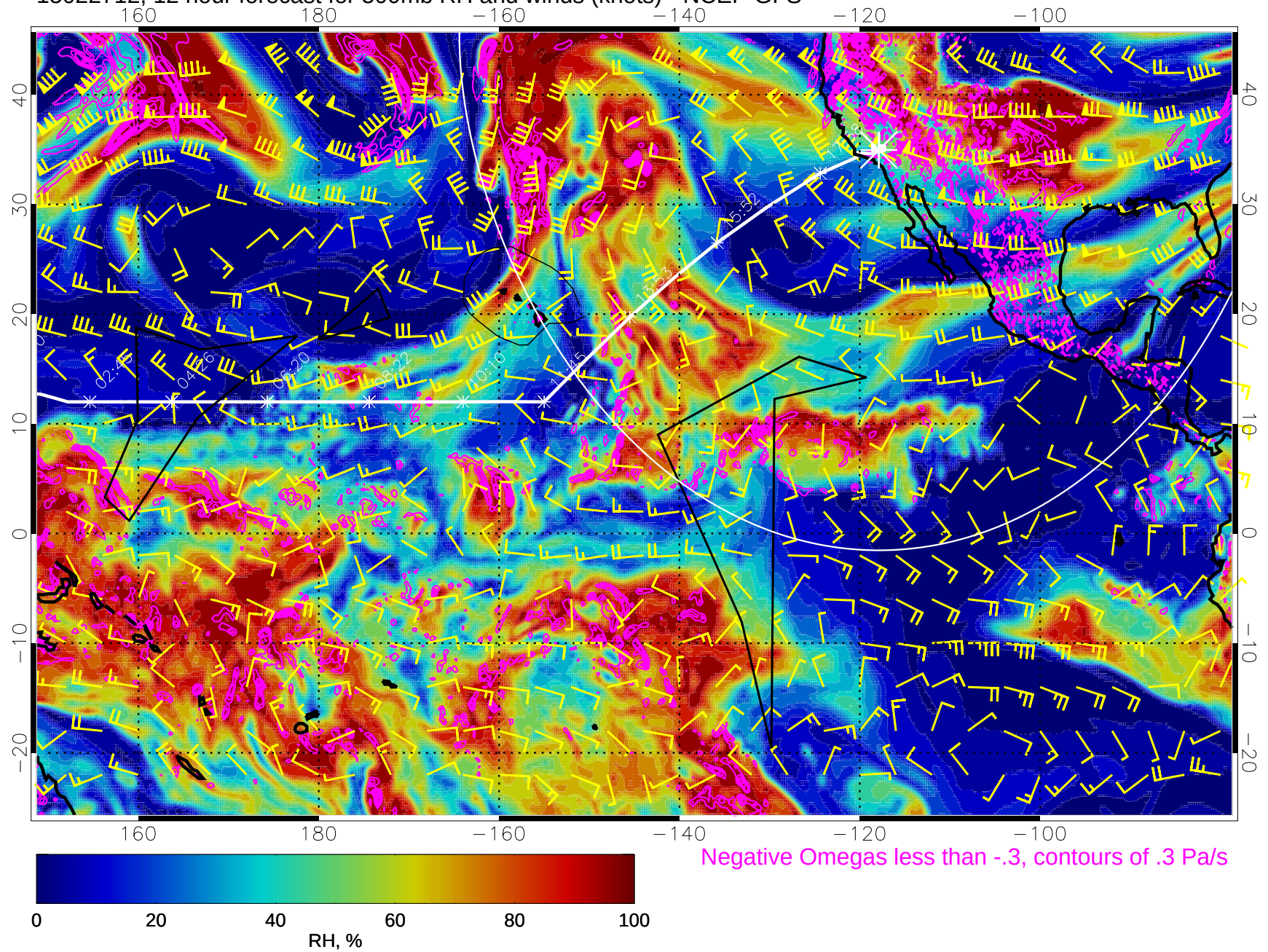
15022712, 12 hour forecast for 500mb RH and winds (knots) - NCEP GFS
