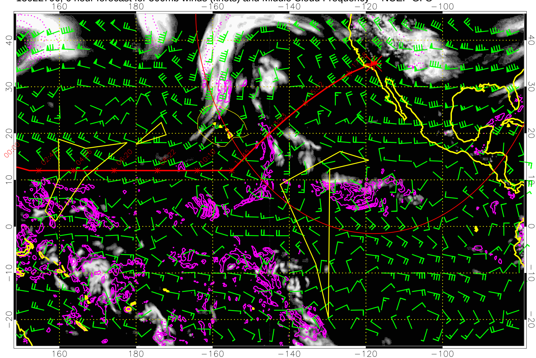
15022706, 6 hour forecast for 500mb winds (knots) and Middle Cloud Frequency -- NCEP GFS
