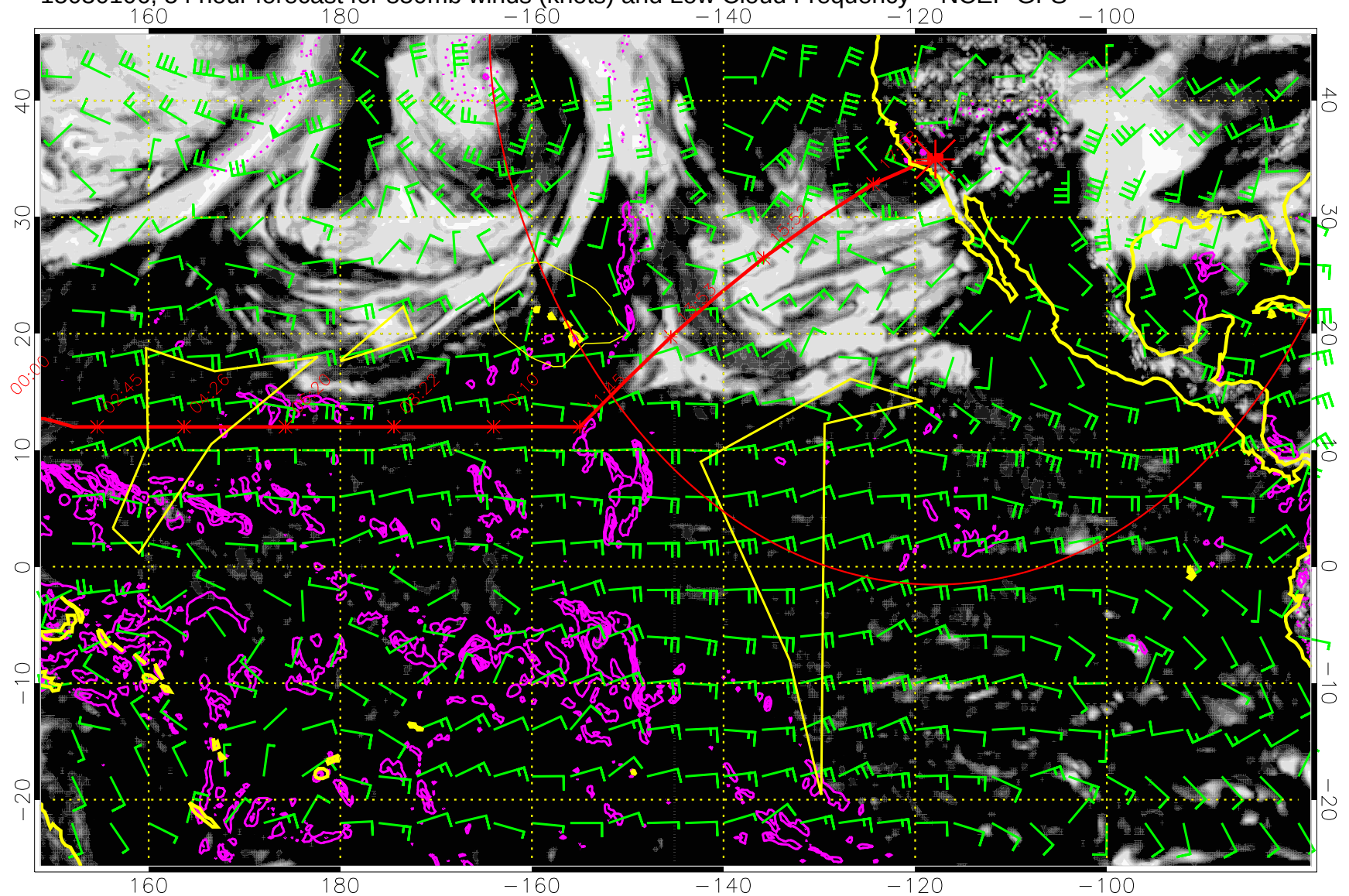
15030106, 54 hour forecast for 850mb winds (knots) and Low Cloud Frequency -- NCEP GFS
