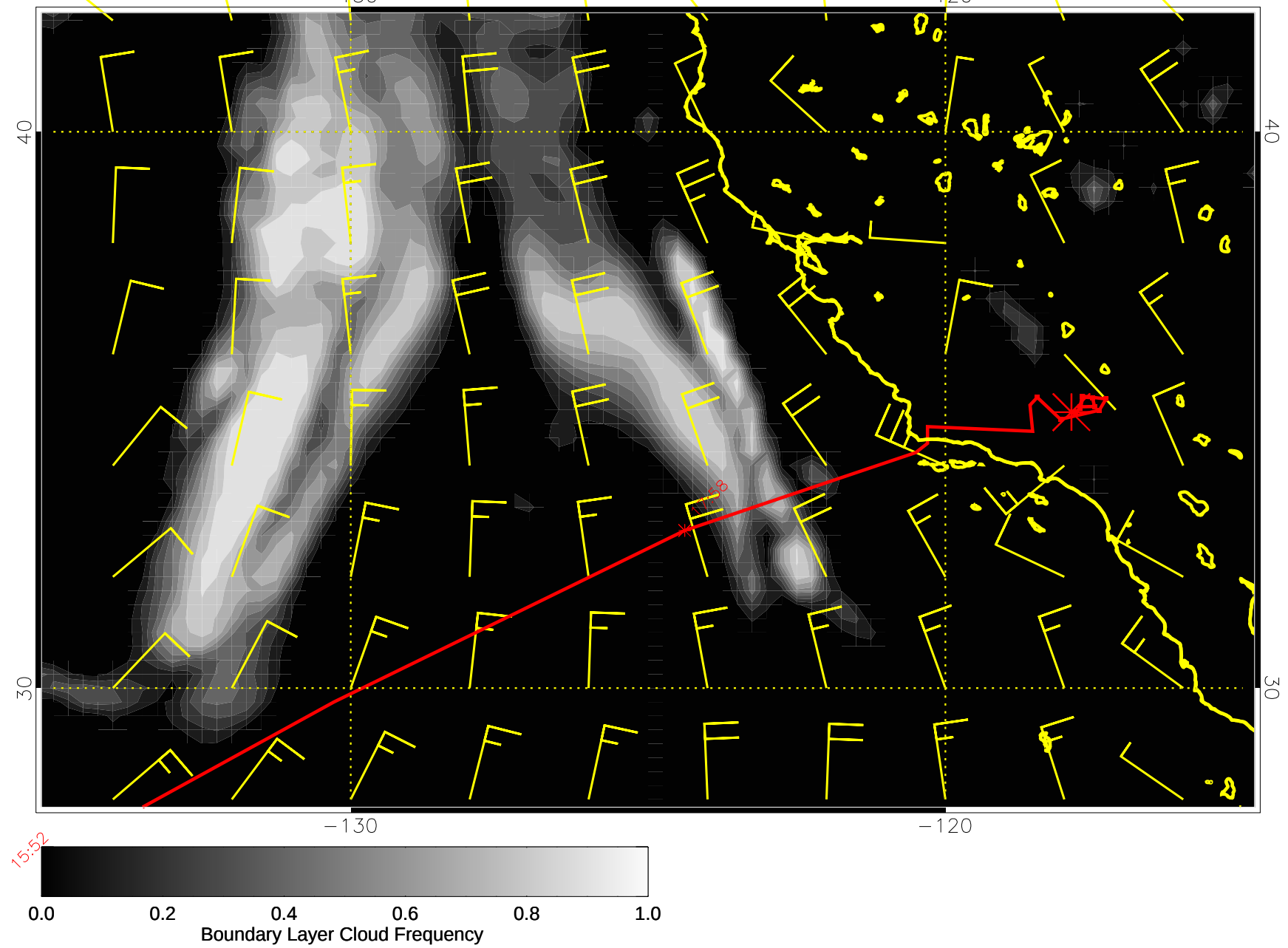
15030400, 120 hour forecast for surface winds (knots) and Boundary Layer Cloud Frequency -- NCEP GFS
