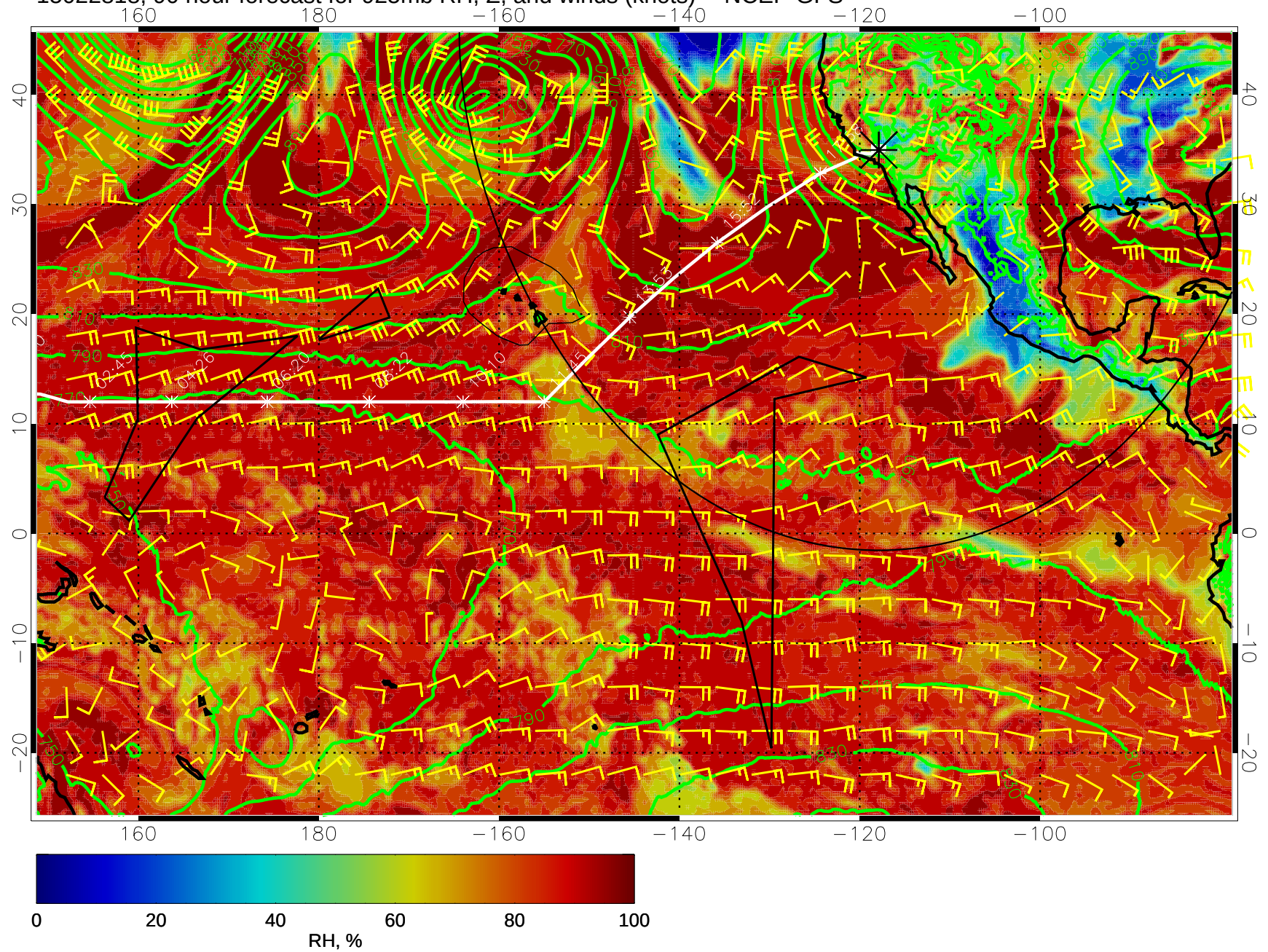
15022818, 90 hour forecast for 925mb RH, Z, and winds (knots) -- NCEP GFS
