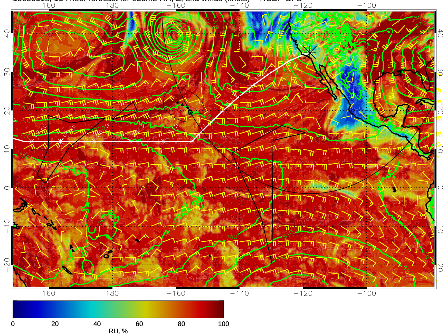
15030118, 114 hour forecast for 925mb RH, Z, and winds (knots) -- NCEP GFS
