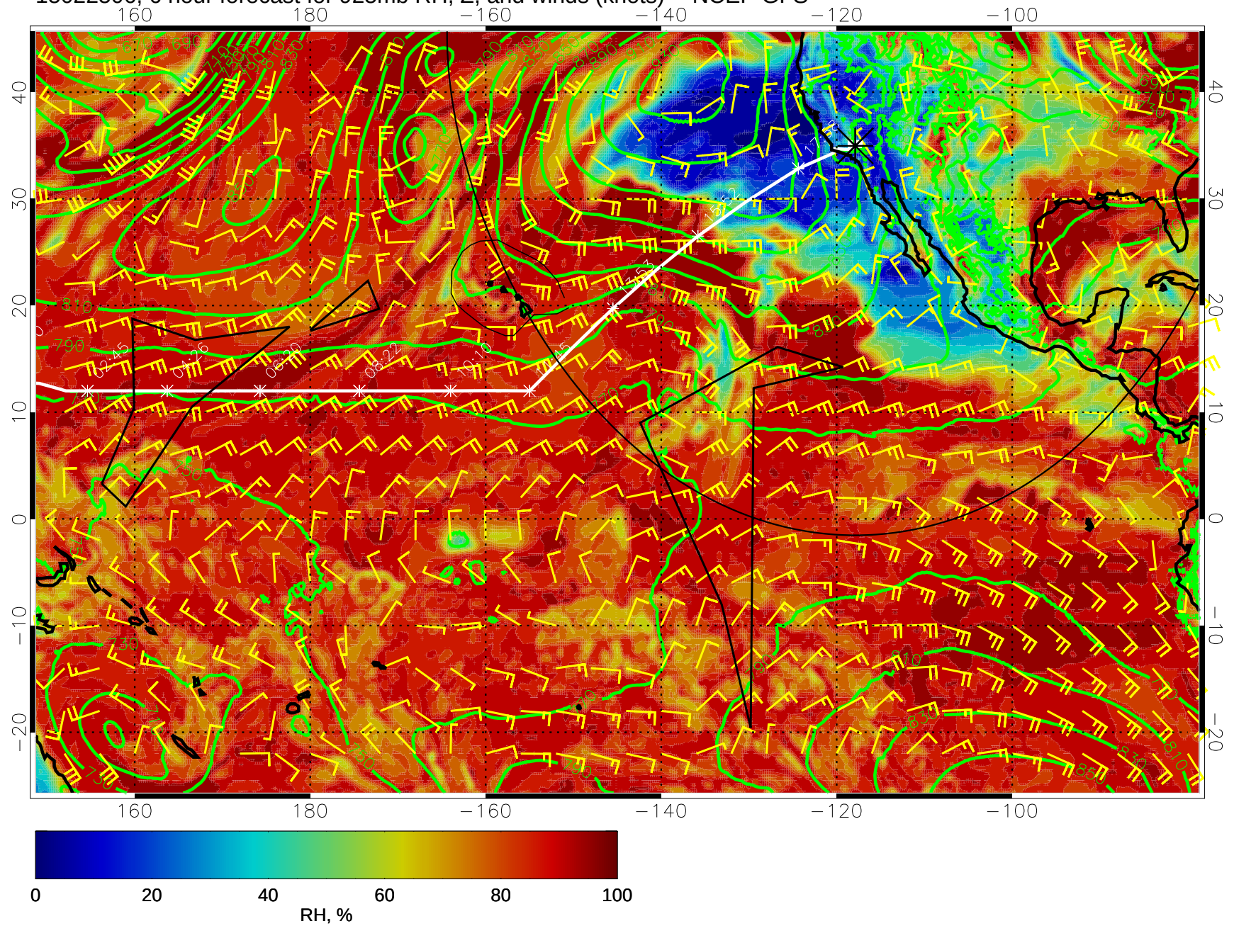
15022506, 6 hour forecast for 925mb RH, Z, and winds (knots) -- NCEP GFS
