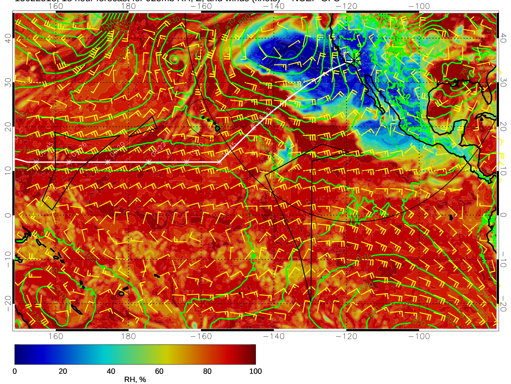
15022518, 18 hour forecast for 925mb RH, Z, and winds (knots) -- NCEP GFS
