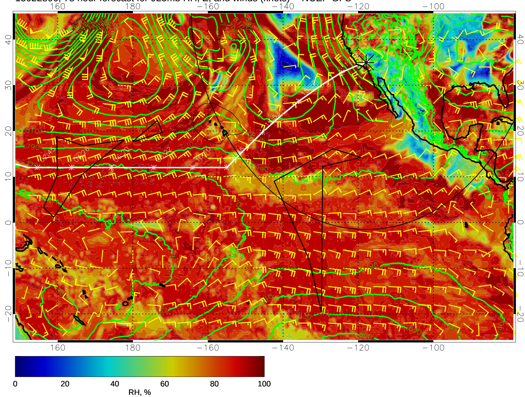
15022806, 78 hour forecast for 925mb RH, Z, and winds (knots) -- NCEP GFS
