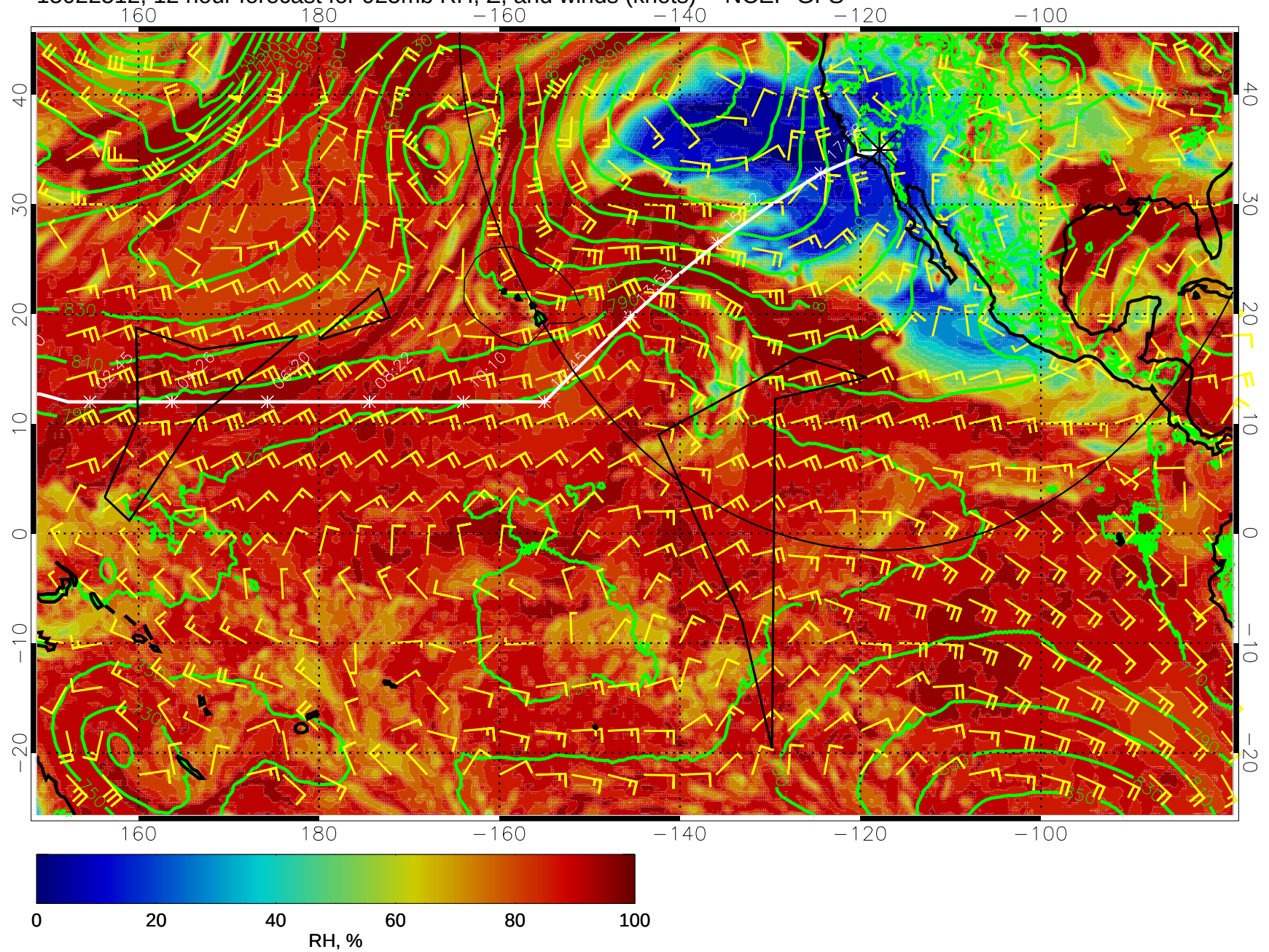
15022512, 12 hour forecast for 925mb RH, Z, and winds (knots) -- NCEP GFS
