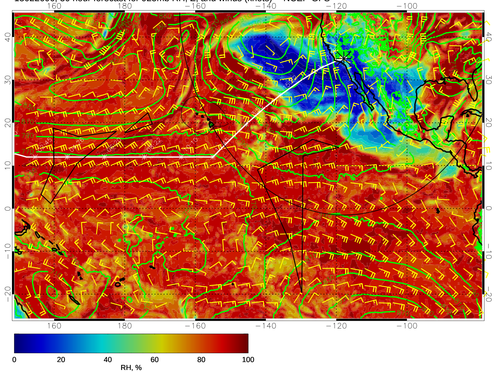
15022606, 30 hour forecast for 925mb RH, Z, and winds (knots) -- NCEP GFS
