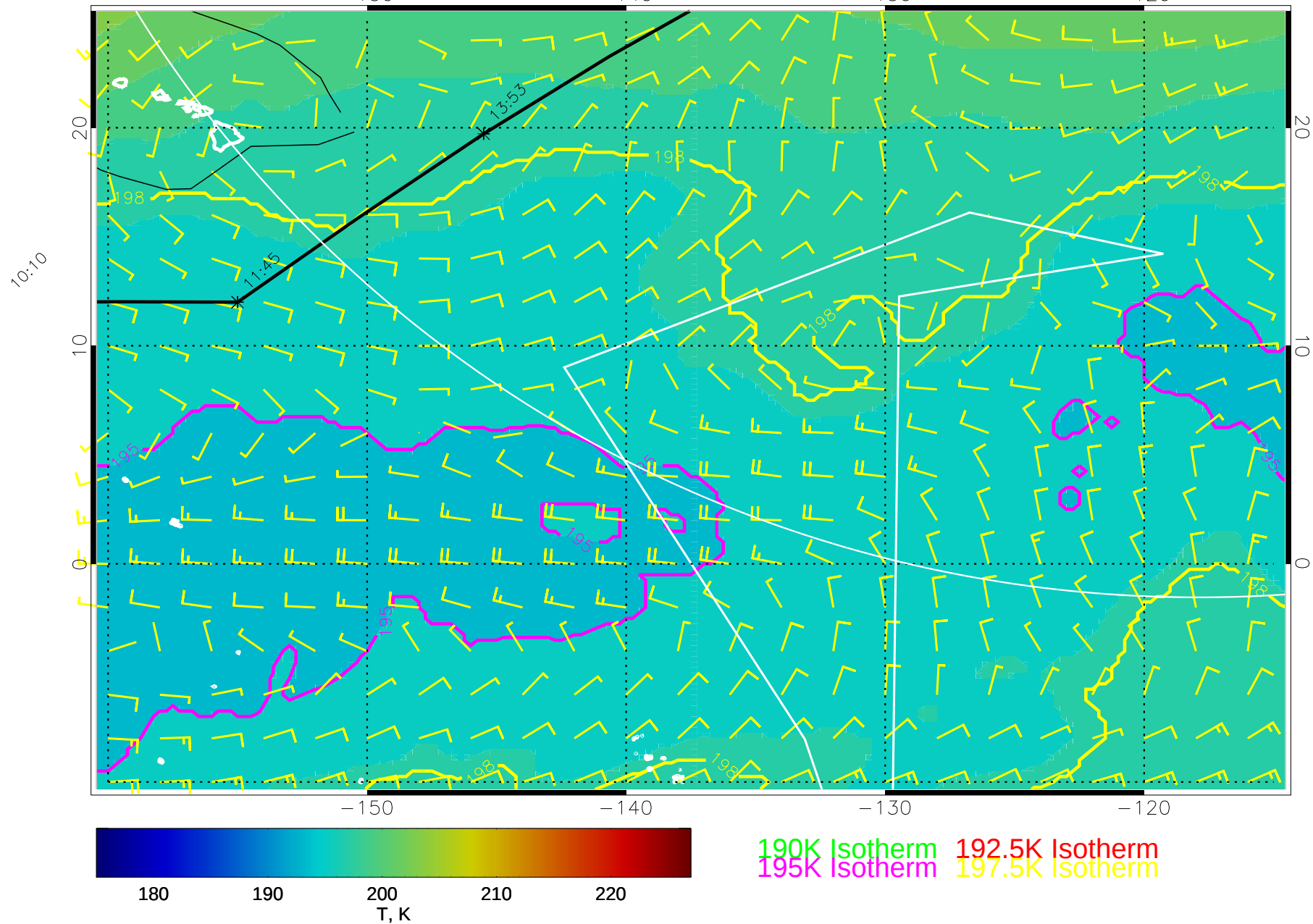
15030106, 102 hour forecast for 70mb T and winds (knots) -- NCEP GFS
