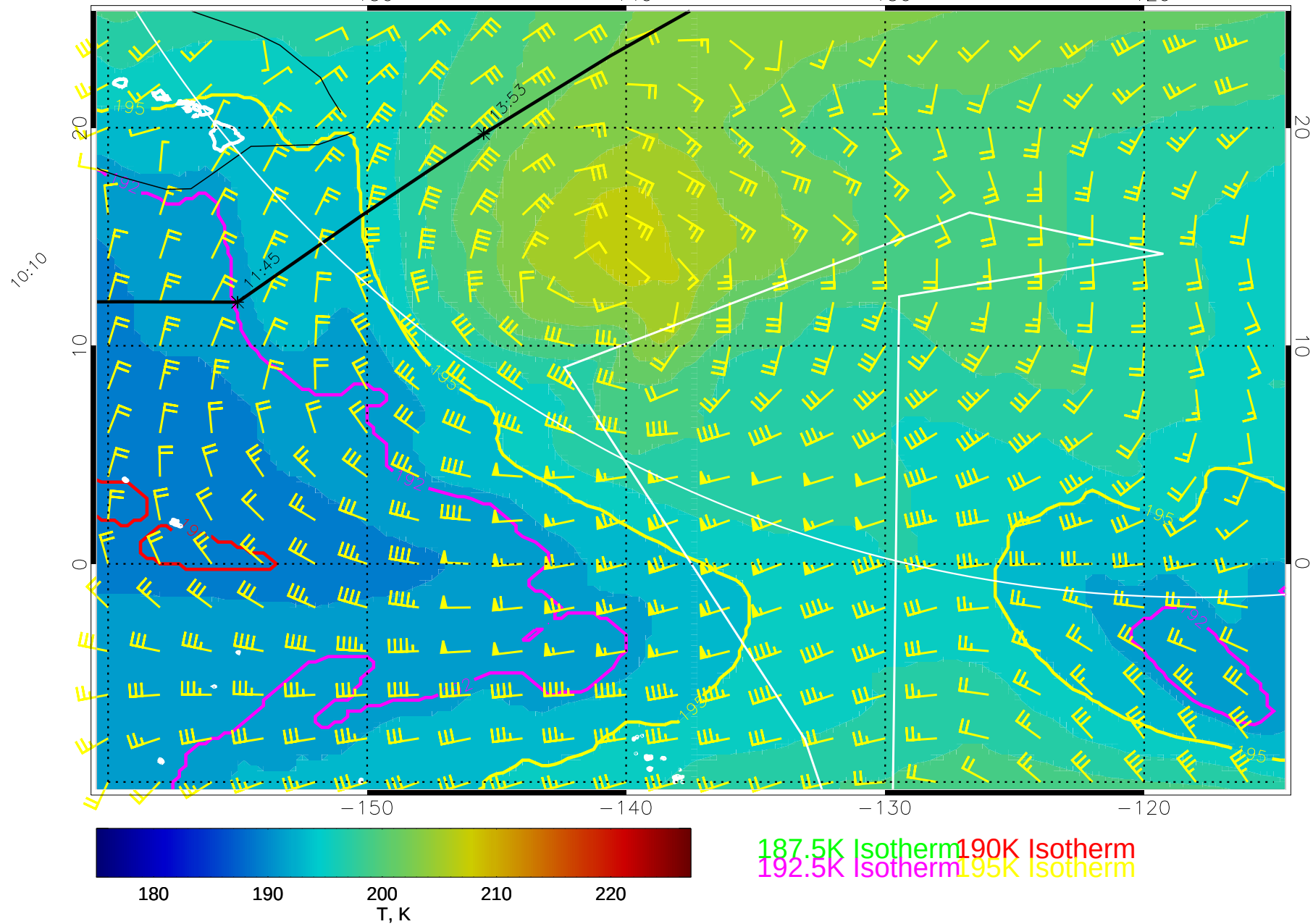
15022506, 6 hour forecast for 100mb T and winds (knots) -- NCEP GFS
