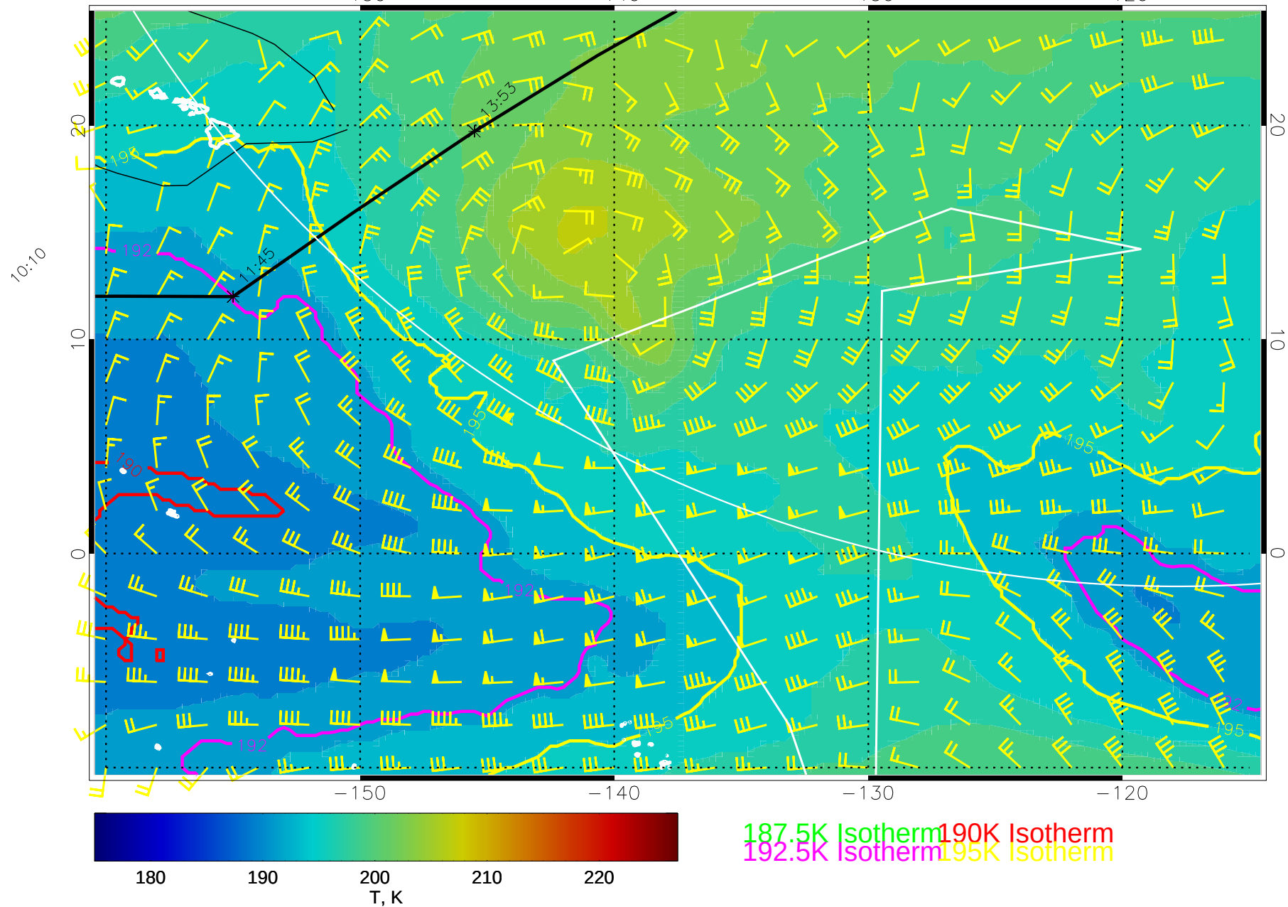
15022512, 12 hour forecast for 100mb T and winds (knots) -- NCEP GFS
